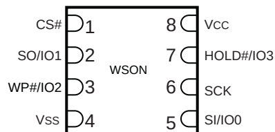
Figure 29. 8-Contact WSON (5 mm x 6 mm) Package / 8-Contact USON (4 mm x 4 mm) Package
