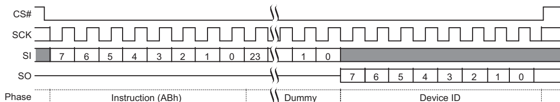
Figure 55. Read Electronic Signature (RES ABh) Command Sequence
