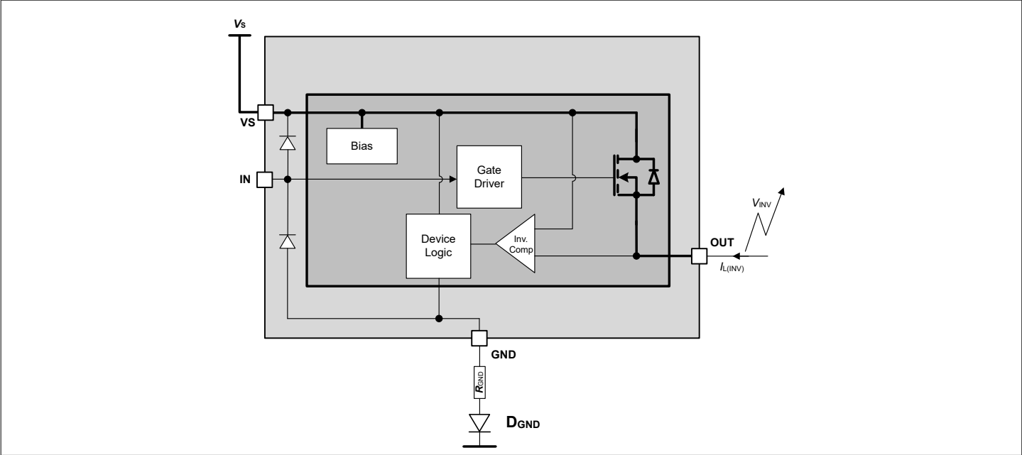
Figure 12 Inverse current circuitry ITS4035S-EP-D
