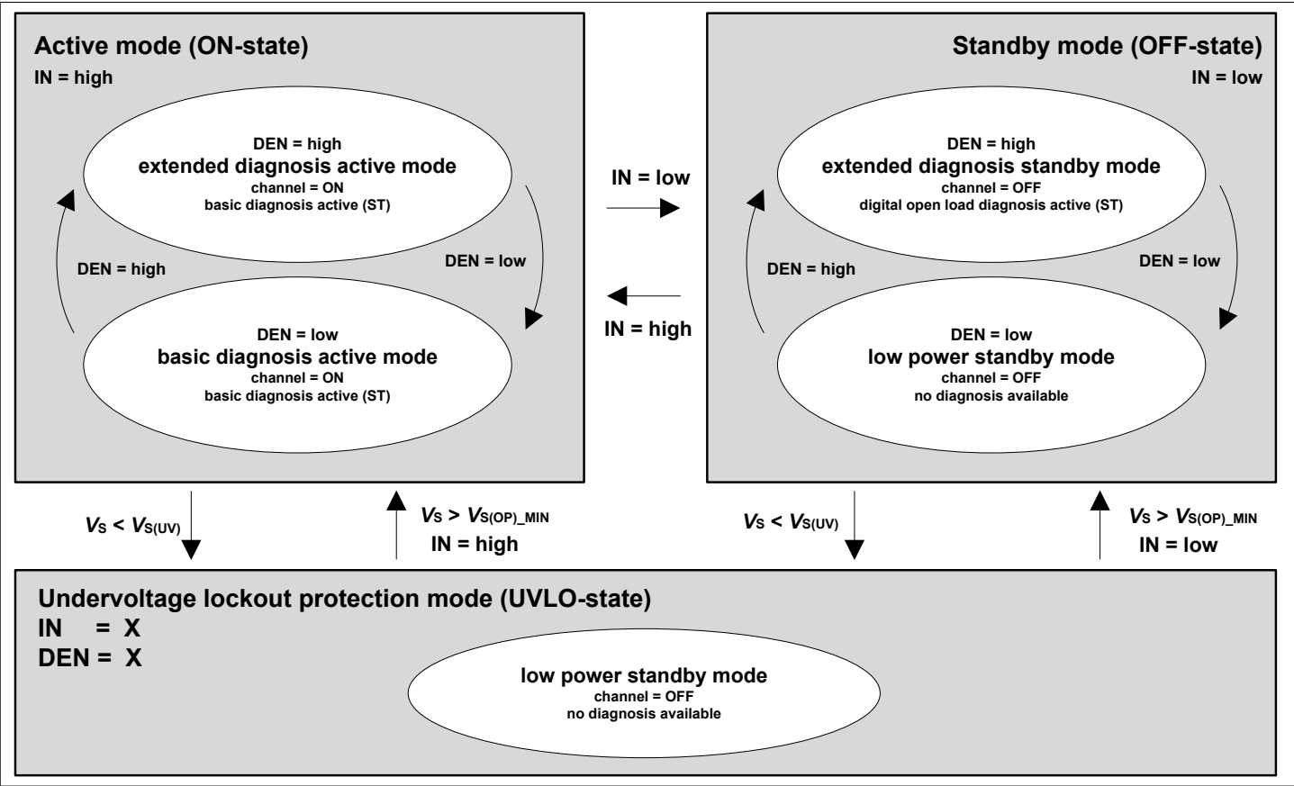
Figure 6 State diagram ITS4035S-EP-D
