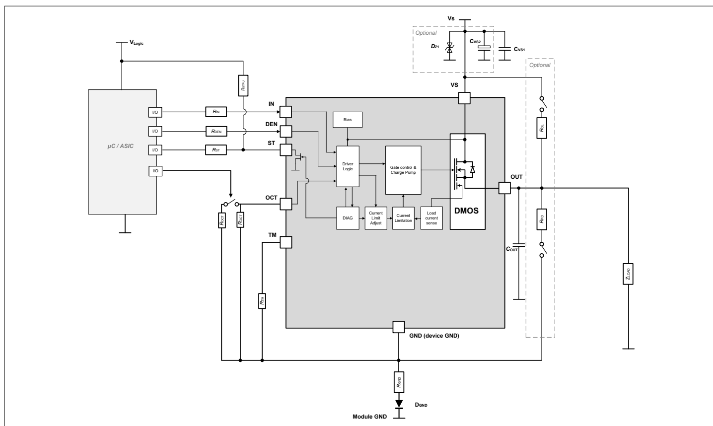
Figure 26 Application diagram with ITS4035S-EP-D controlled by logic levels [μC] with dynamic inrush current control
