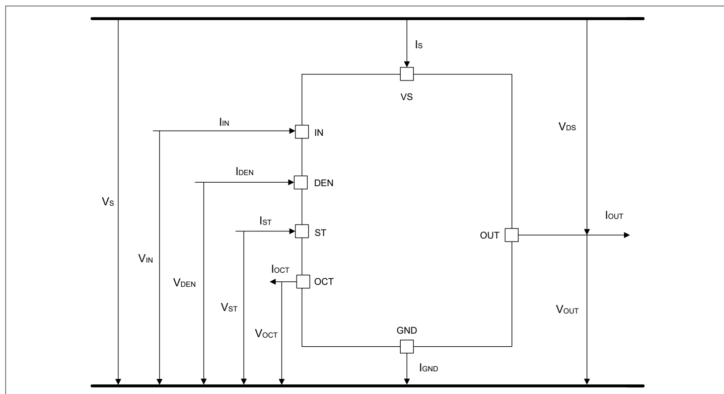
Figure 3 Voltage and current definitions
