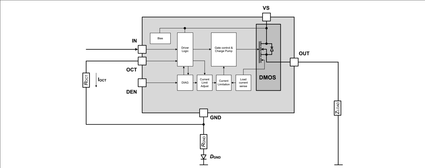
Figure 19 Adjustment of Current Limit threshold with external resistor R_{OCT}
