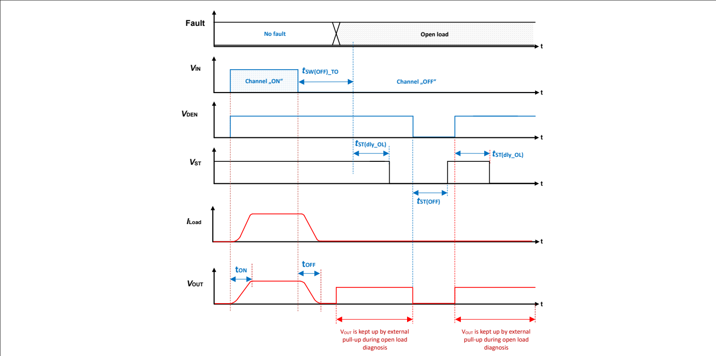
Figure 22 Behavior and timings of the extended diagnostic capabilities (the usage of a DEN - controlled switchable pull-up resistor from OUT to V_S in OFF-state is assumed)
