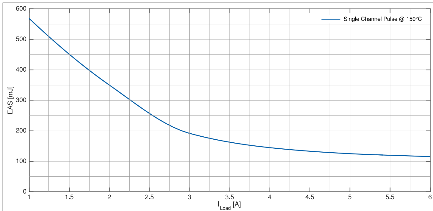
Figure 11 Maximum energy dissipation single pulse; V_S = 28 V
