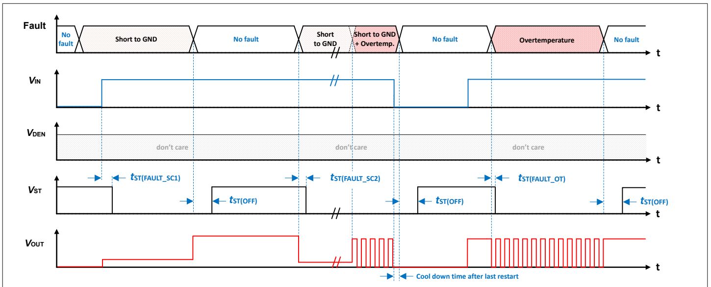
Figure 21 Behavior and timings of basic diagnosis
