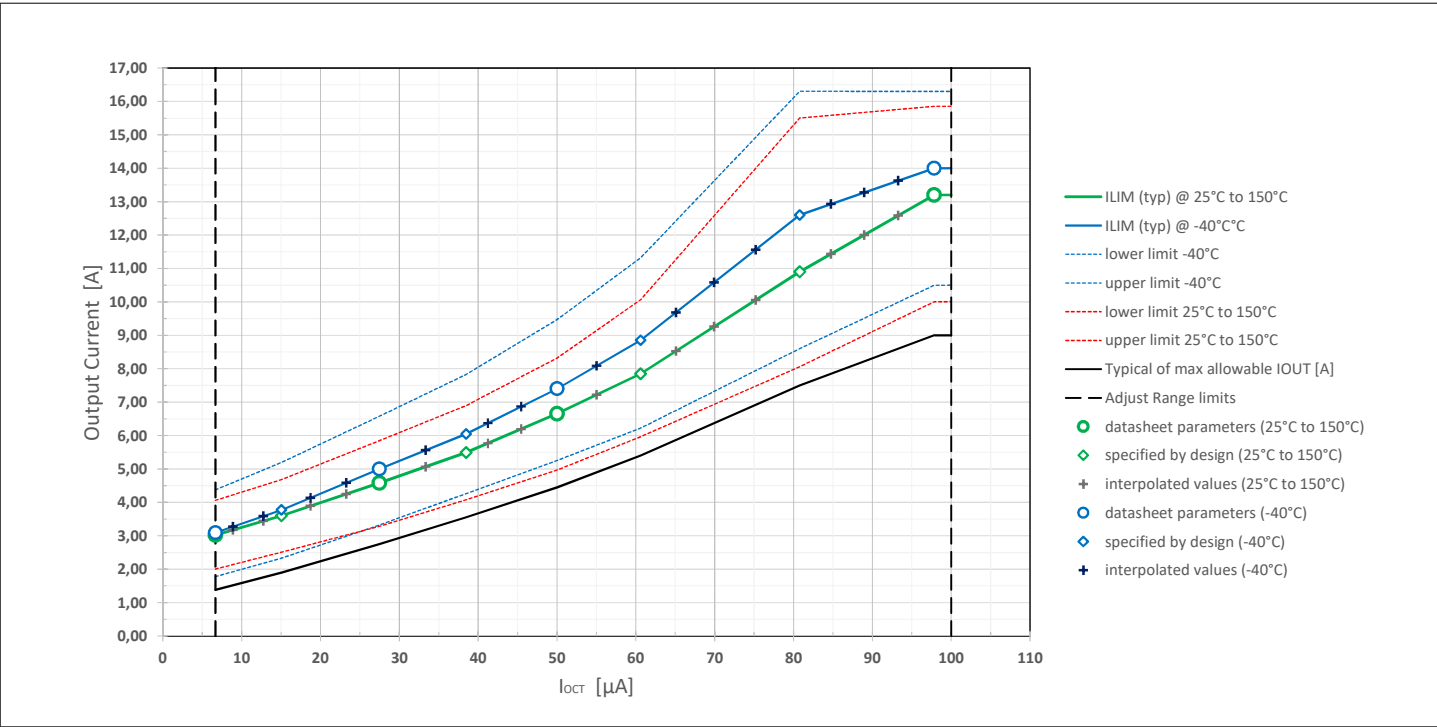
Figure 27 Current limitation threshold I_{LIM(th,adj)} as function of I_{OCT} and related limitation values for different temperatures
