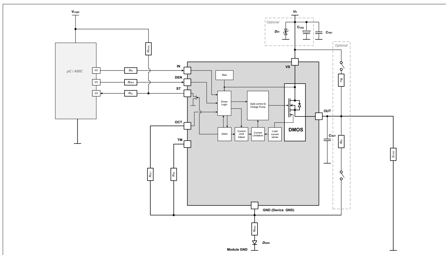
Figure 25 Application diagram with ITS4035S-EP-D
