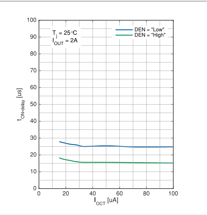
Turn on delay time t_{ON\_delay} to V_{OUT} = 10\% versus current limit adjust current I_{OCT}
