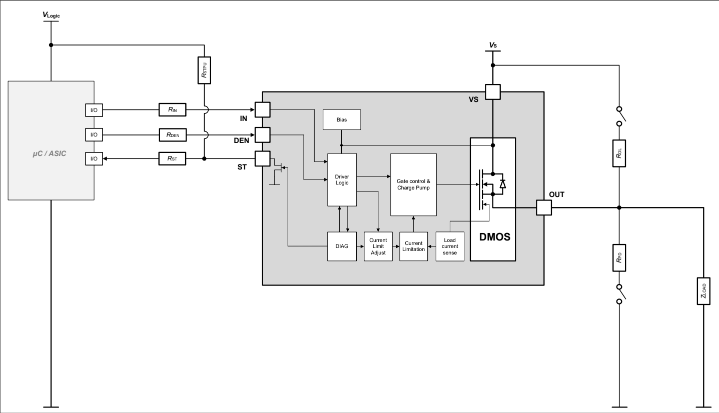
Figure 23 Overview: usage of diagnosis
