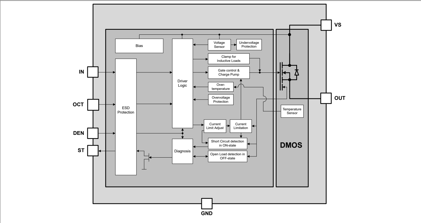
Figure 1 Block diagram ITS4035S-EP-D
