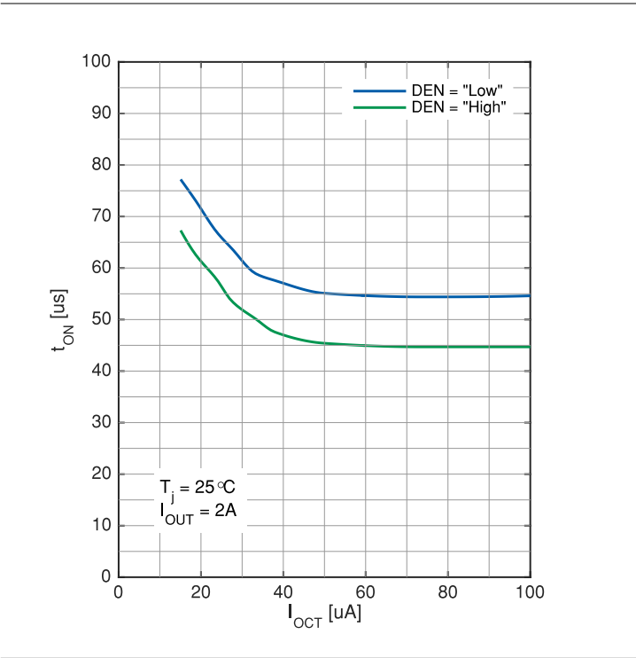
Turn on time t_{ON} to V_{OUT} = 90\% versus current limit adjust current I_{OCT}
