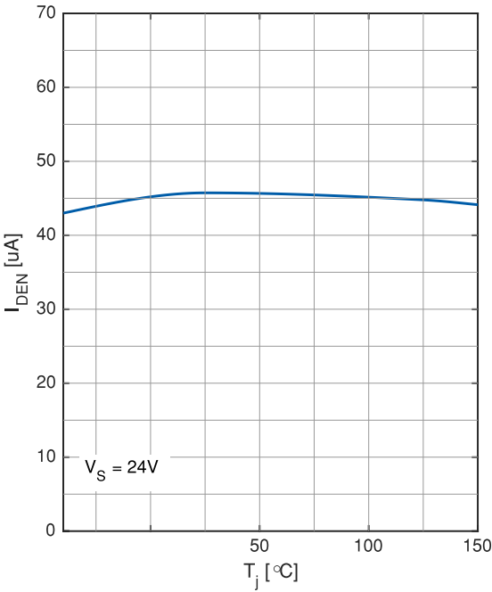
Input pin current I_{\text{DEN(H)}} versus Junction temperature T_j
