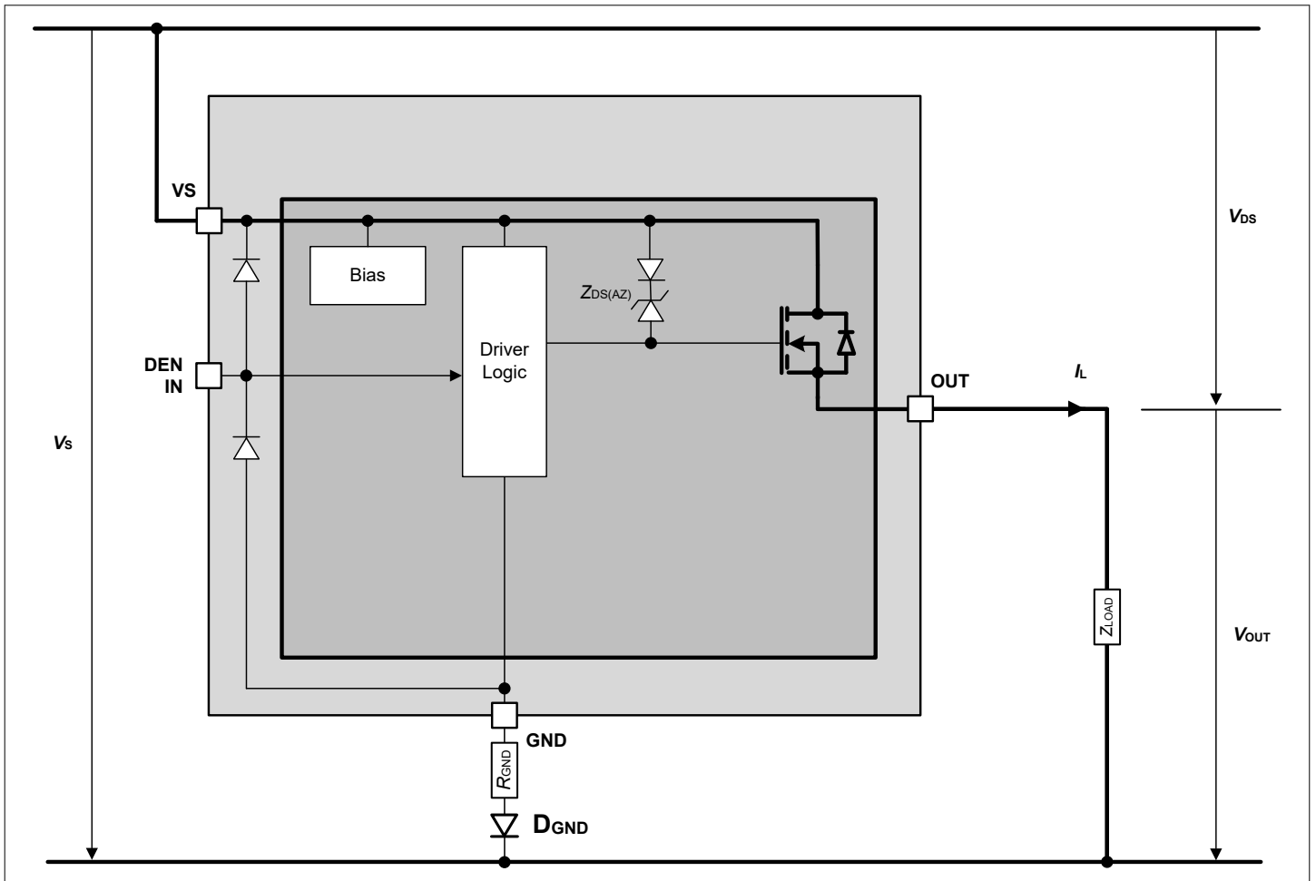
Figure 9 Output clamp ITS4035S-EP-D
