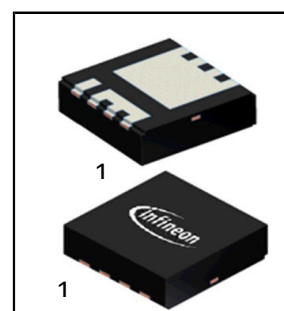
PG-TSDSON-8-33
