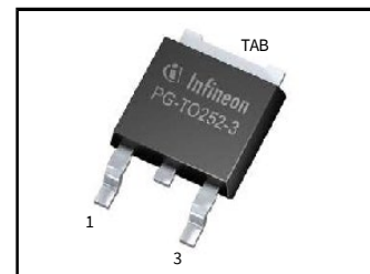
PG-TO252-3-313
