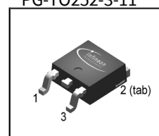
PG-TO252-3-11
