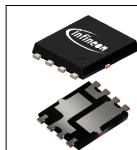
PG-TDSON-8-56
