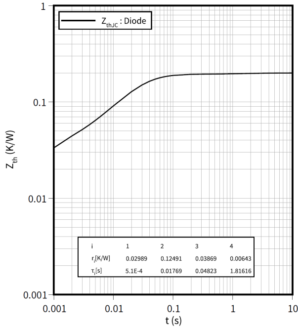
Transient thermal impedance, Diode, Inverter Z_{th} = f(t)
