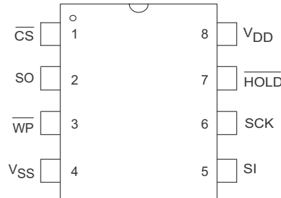
Figure 1. 8-pin PDIP pinout
