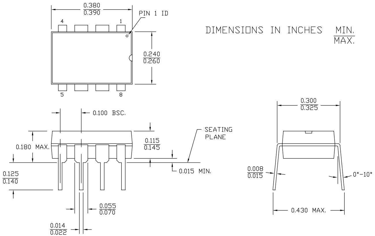
Figure 19. 8-pin PDIP (300 Mils) Package Outline, 51-85075
