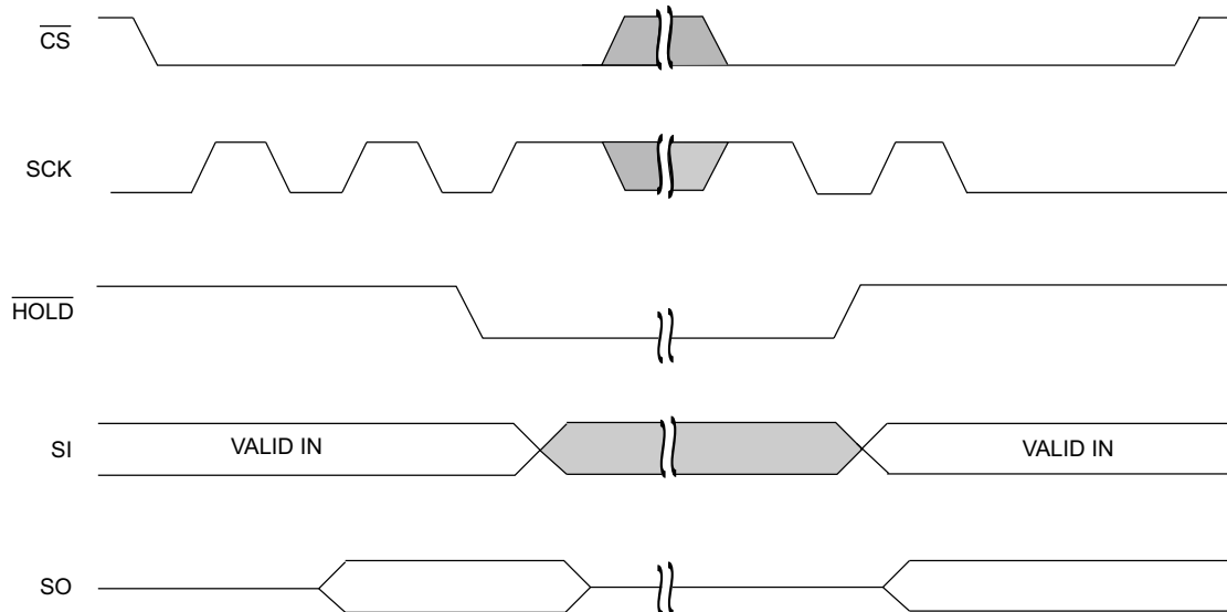
Figure 12. \overline{HOLD} Operation [2]
