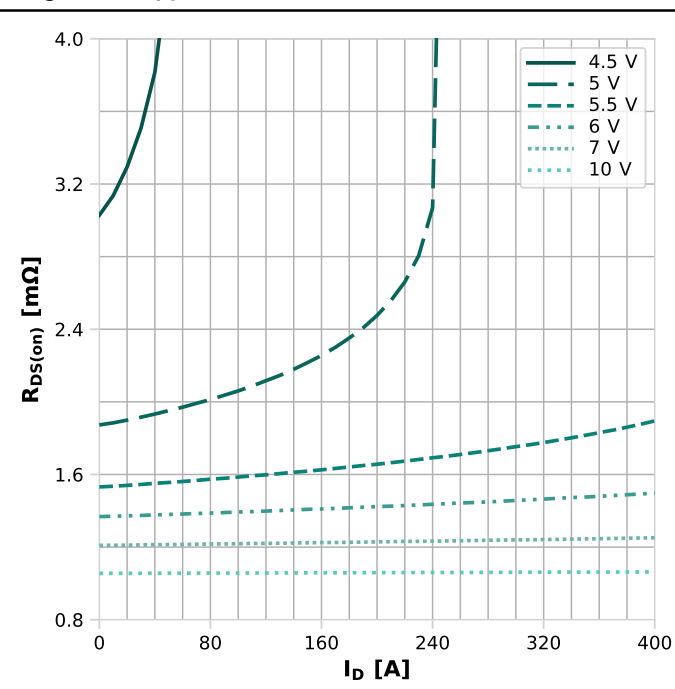
Diagram 6: Typ. drain-source on-state resistance
