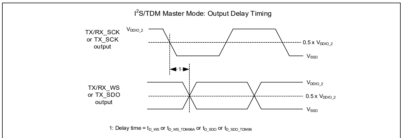
Figure 46 Master output delay
