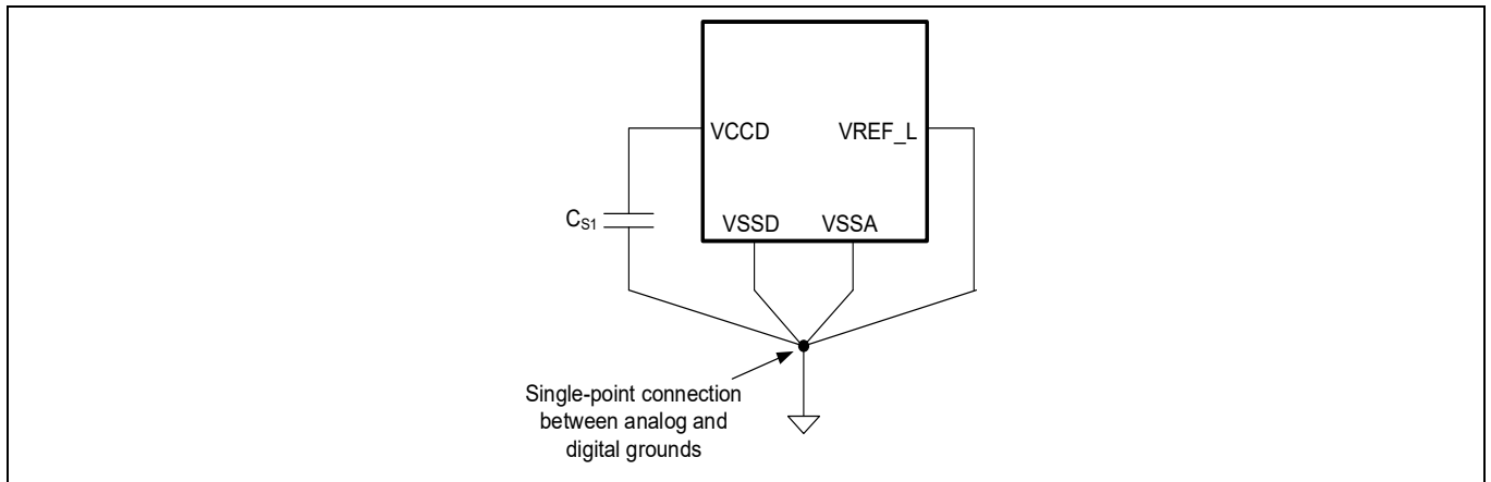
Figure 15 Smoothing capacitor
