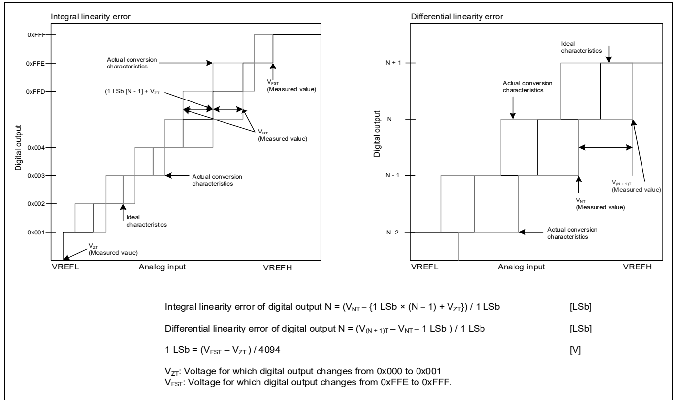
Figure 18 Integral and differential linearity errors
