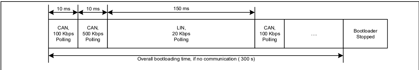
Figure 63 Bootloading sequence
