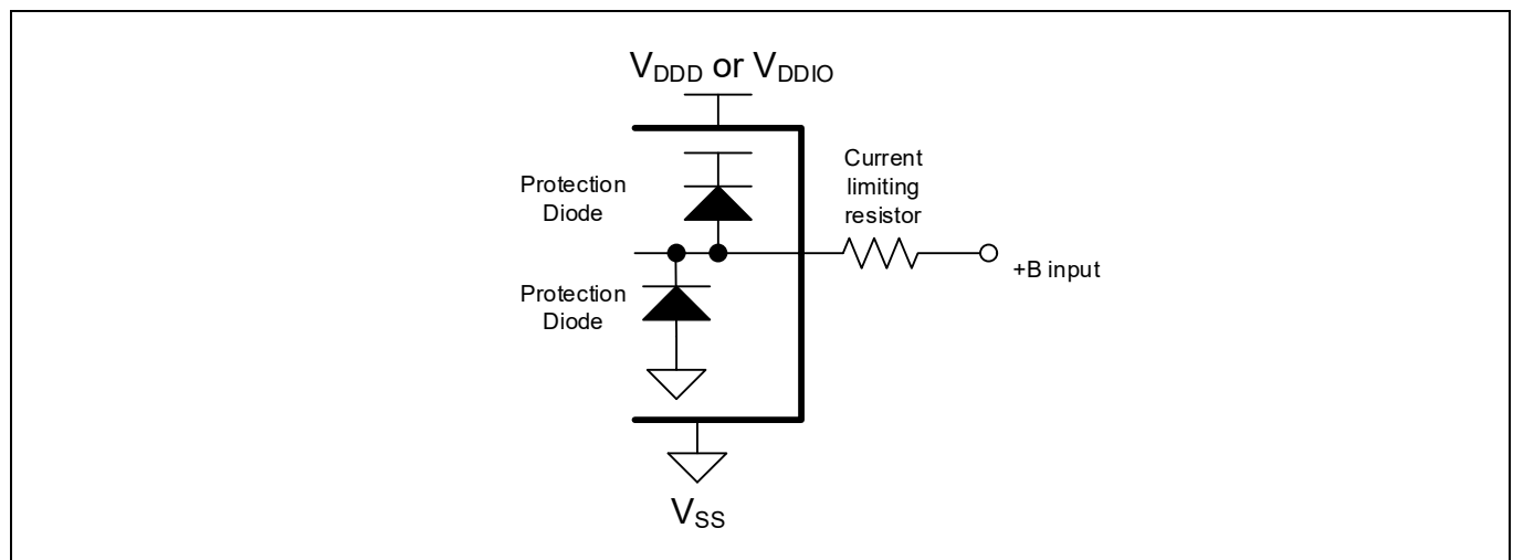
Figure 14 Example of a recommended circuit [54]
