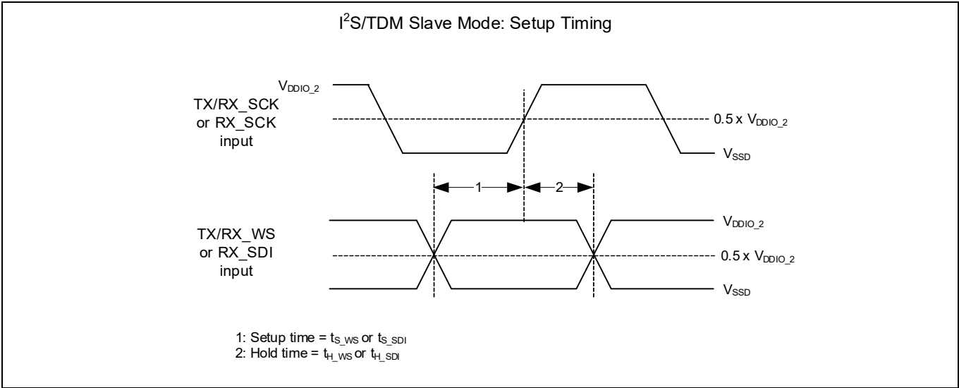
Figure 50 Slave setup
