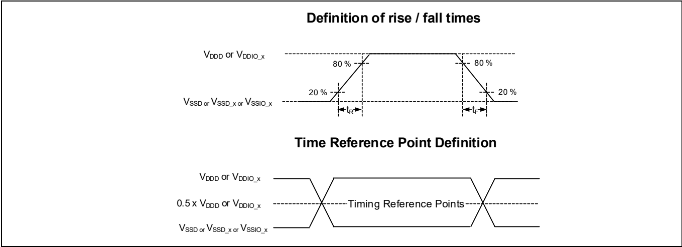
Figure 20 AC timings specifications
