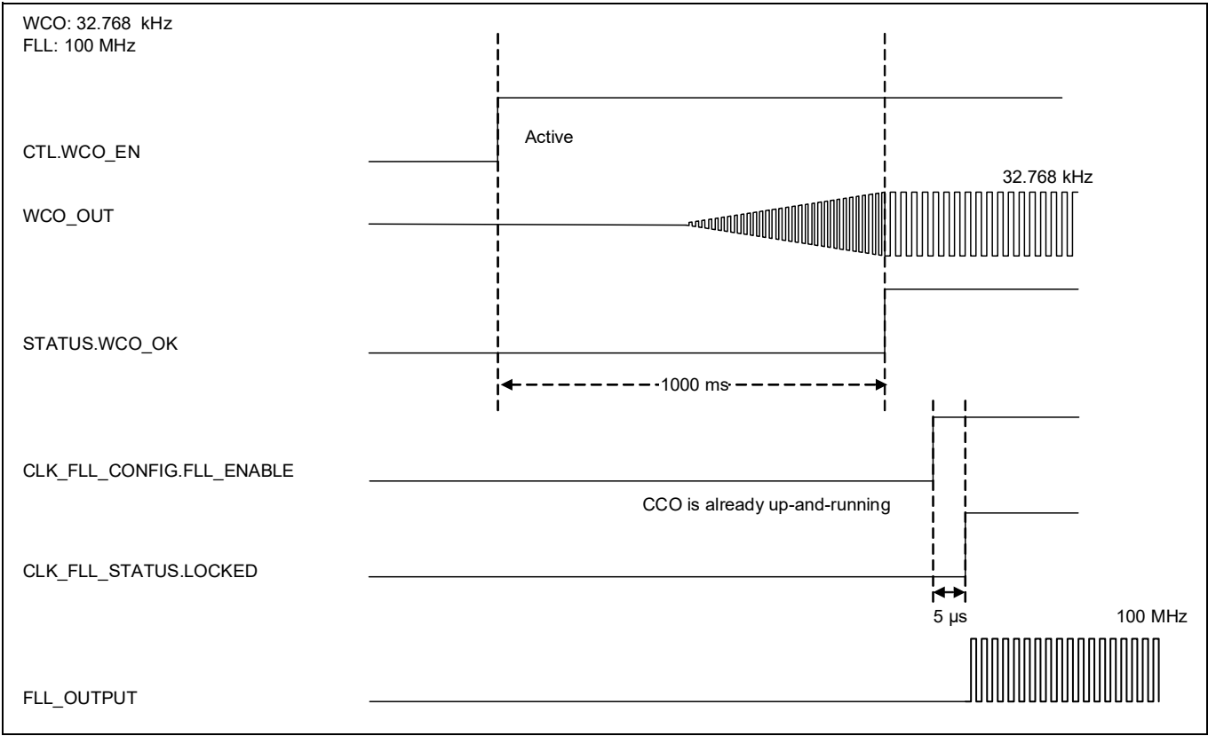
Figure 38 WCO to FLL diagram
