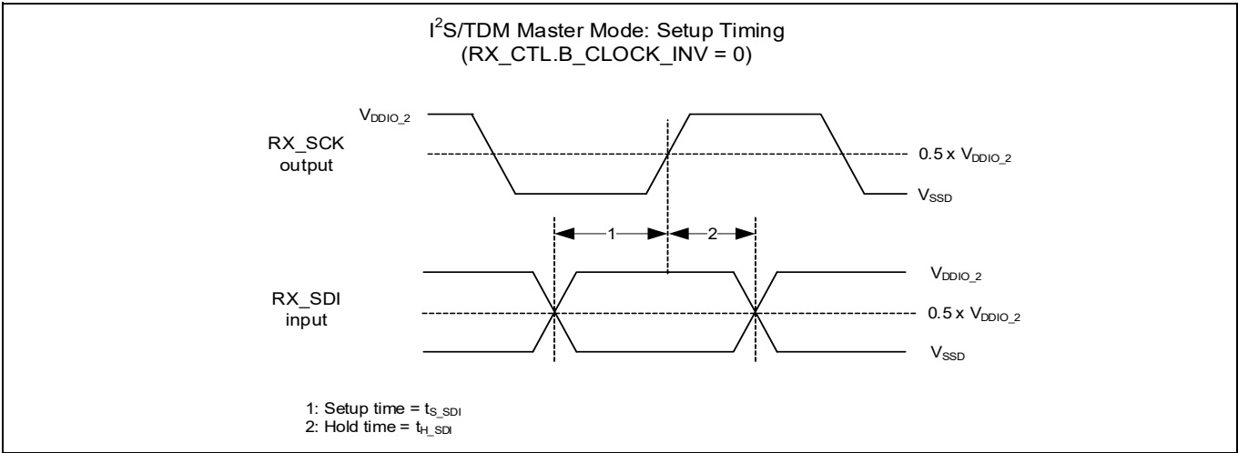
Figure 47 Master setup without clock inversion
