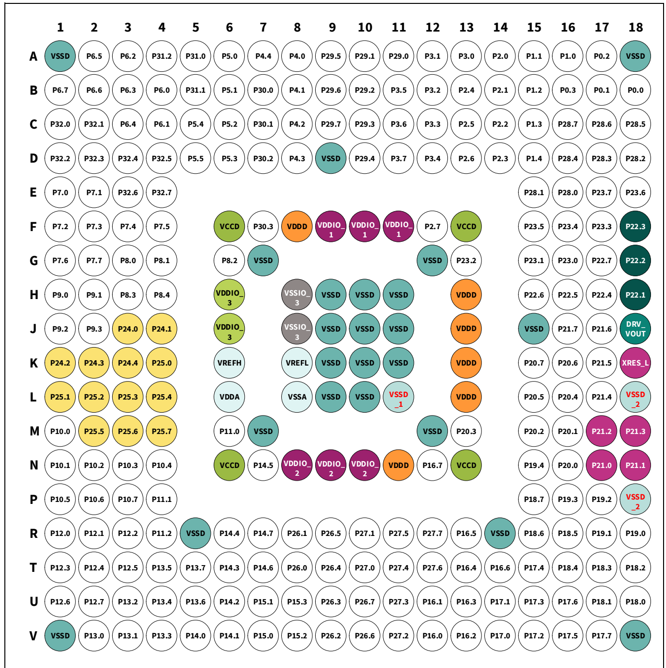
Figure 11 272-BGA ball map
