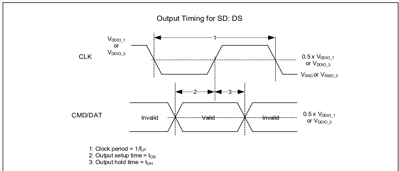
Figure 43 SD default speed output timing
