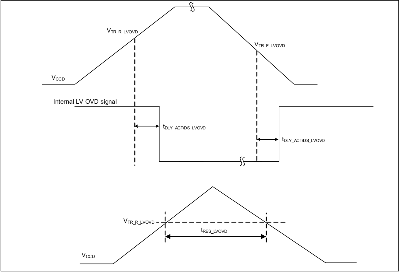
Figure 32 Low-voltage OVD specifications
