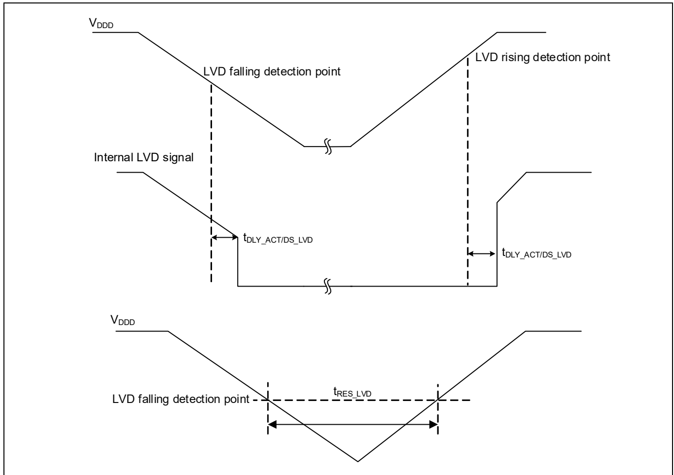
Figure 33 LVD specifications
