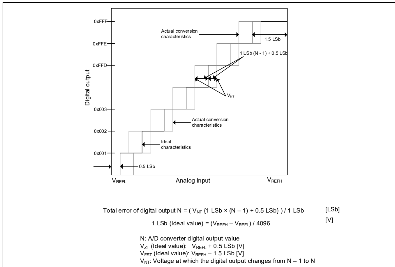
Figure 17 ADC characteristics and error descriptions
