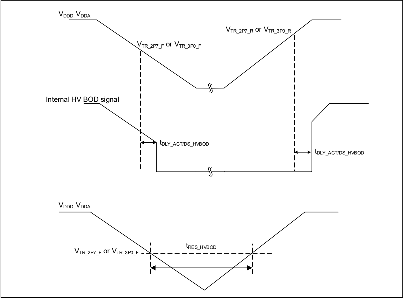
Figure 29 High-voltage BOD specifications
