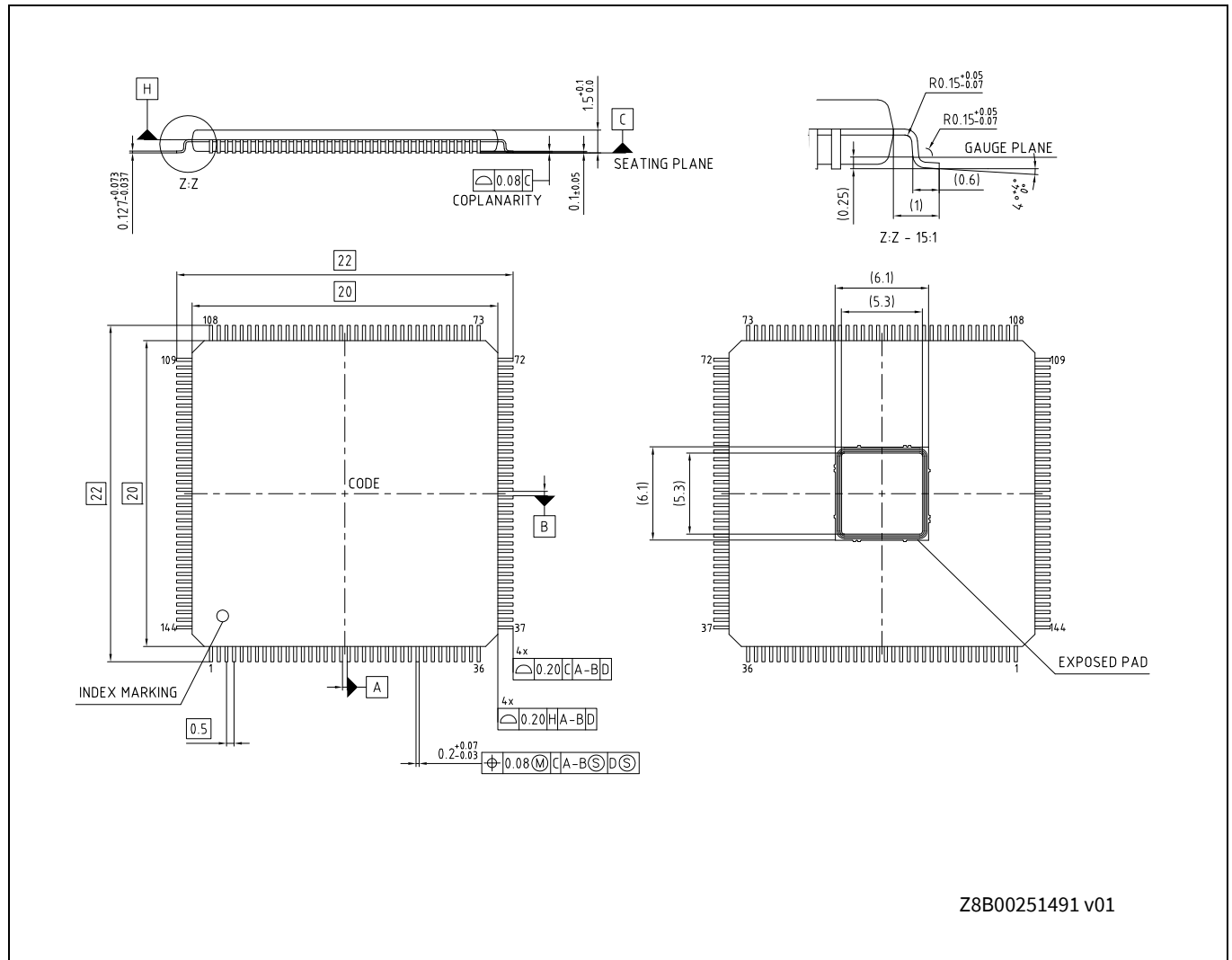
Figure 60 144-lead TEQFP (20.0 × 20.0 × 1.6 mm) LEL144 package outline, Z8B00251491
