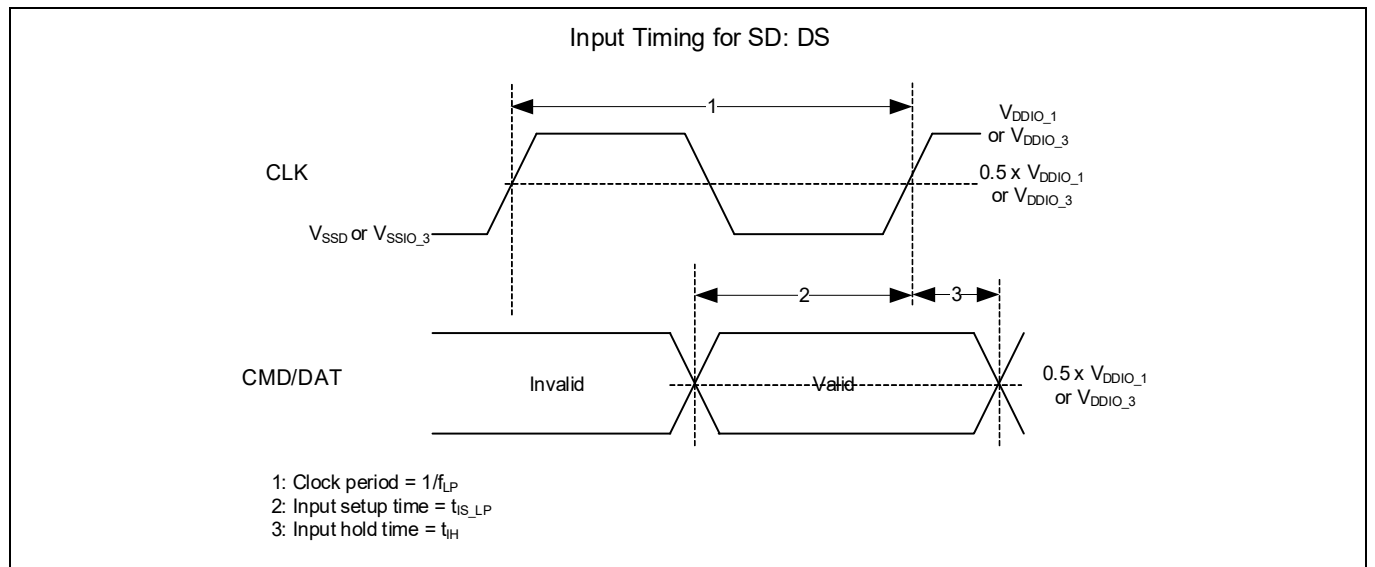
Figure 42 SD default speed input timing
