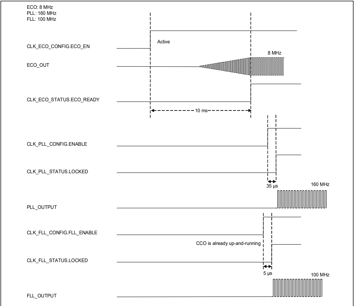
Figure 37 ECO to PLL or FLL diagram
