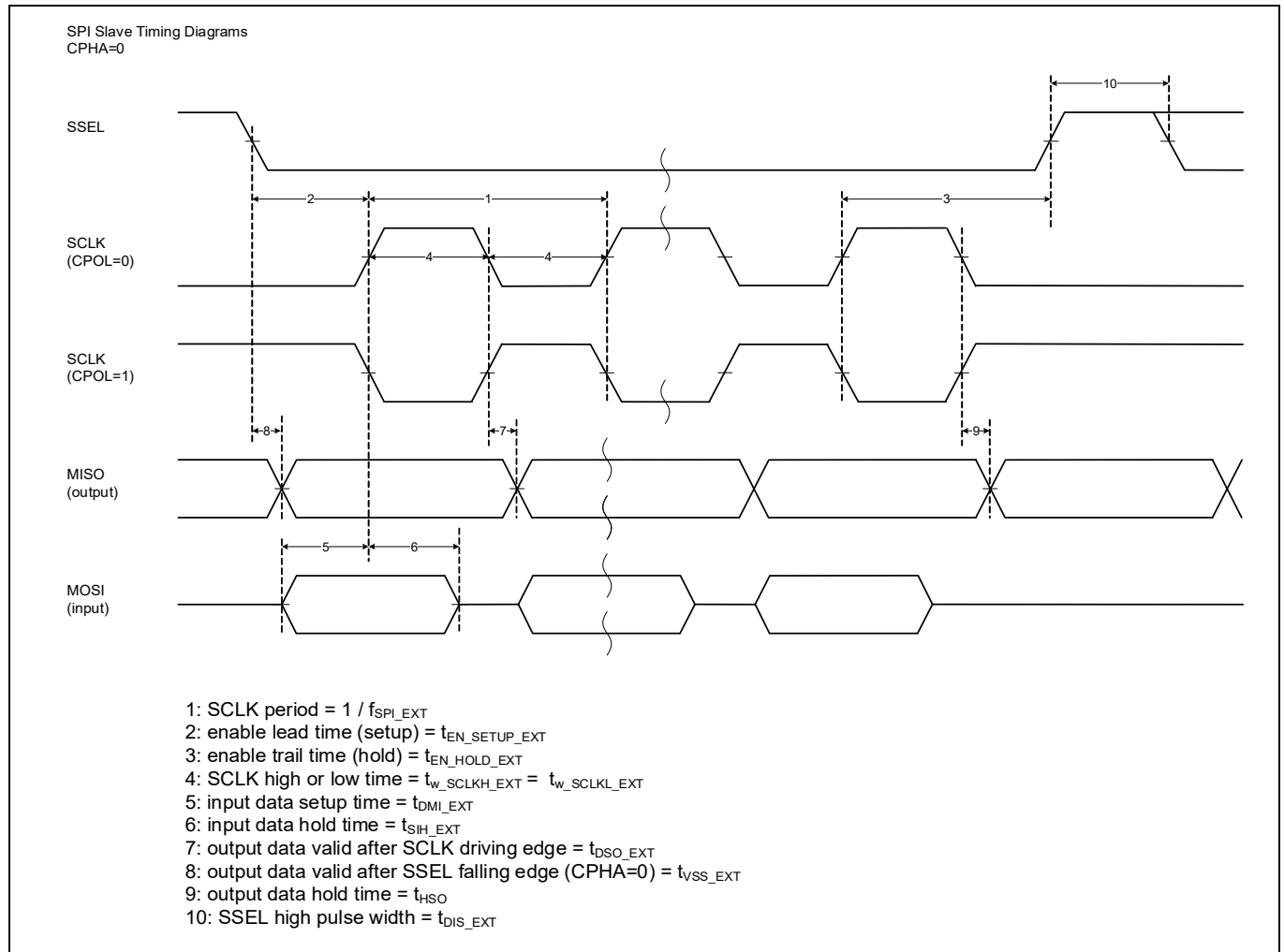
Figure 25 SPI slave timing diagrams with LOW clock phase
