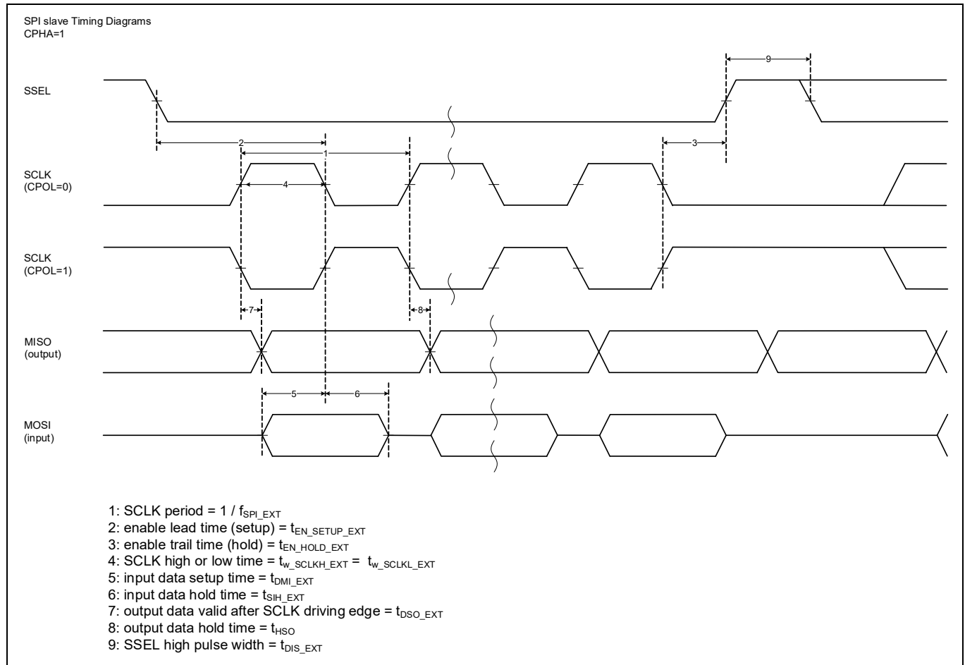
Figure 26 SPI slave timing diagrams with HIGH clock phase
