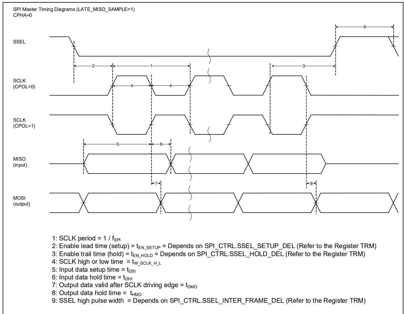
Figure 23 SPI master timing diagrams with LOW clock phase
