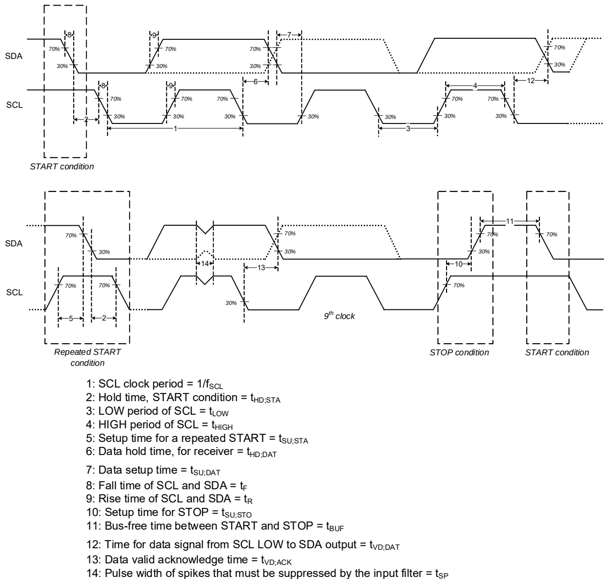
Figure 22 I 2 C timing diagrams
