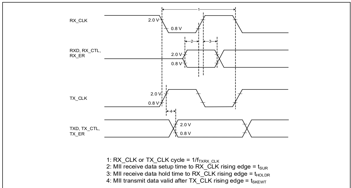
Figure 39 MII timing diagram
