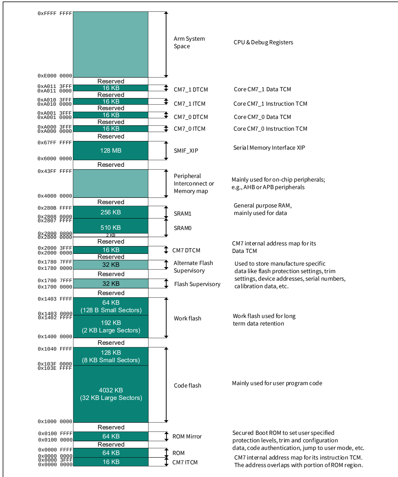
Figure 3 CYT3BB/4BB address map [21, 22]
