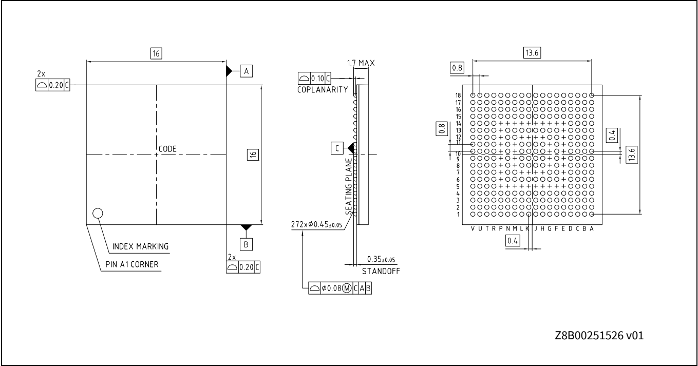
Figure 62 272-ball FBGA (16.00 × 16.00 × 1.70 mm) LBM272 package outline, Z8B00251526
