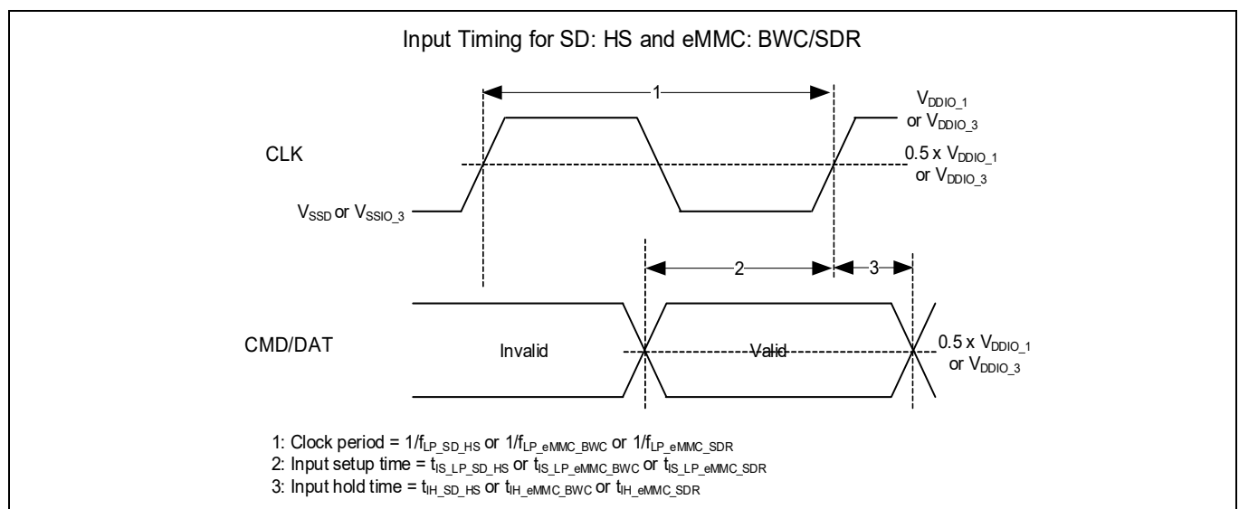
Figure 44 SD high speed and eMMC BWC/SDR input timing
