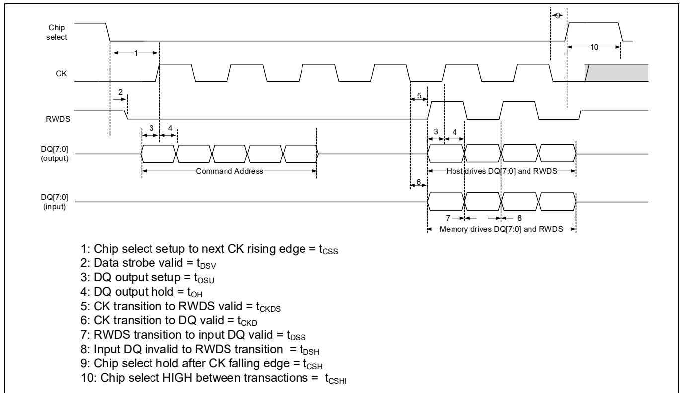
Figure 58 HYPERBUS™ timing diagram
