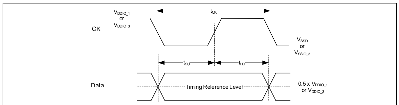
Figure 51 SDR write timing reference level
