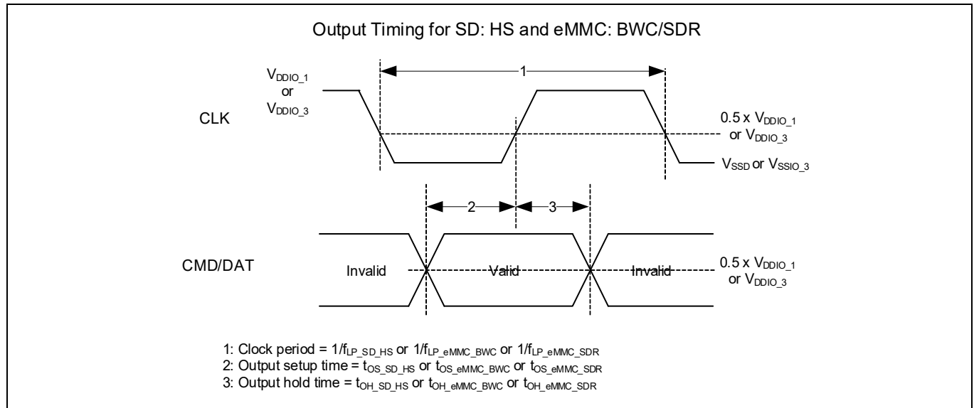
Figure 45 SD high speed and eMMC BWC/SDR output timing
