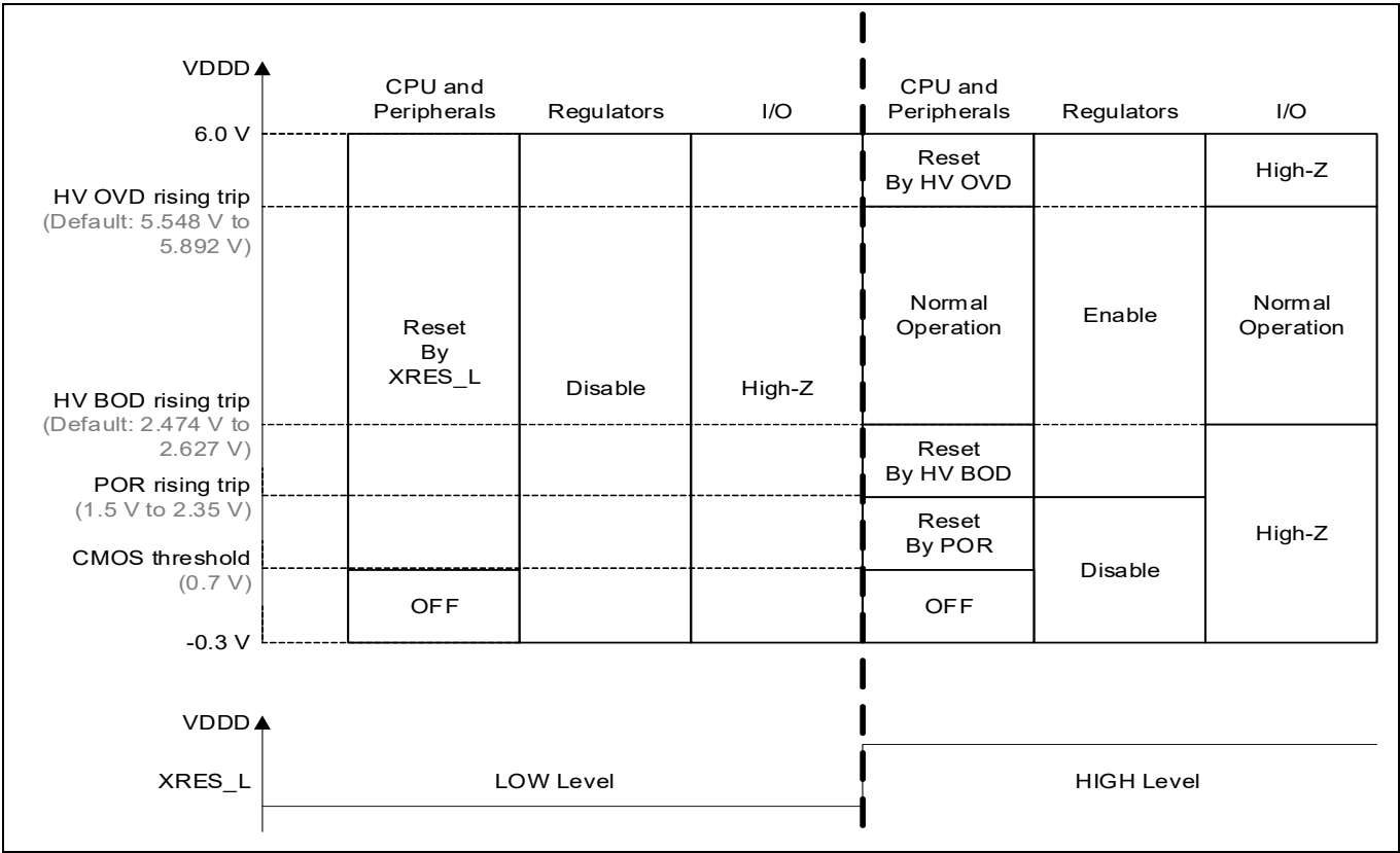
Figure 27 Device operations supply range
