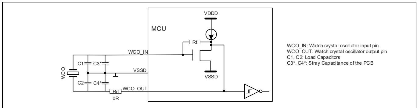
Figure 36 WCO connection scheme [75]
