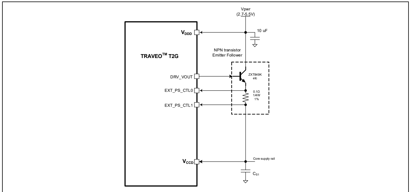
Figure 1 Sample core external regulator with NPN transistor
