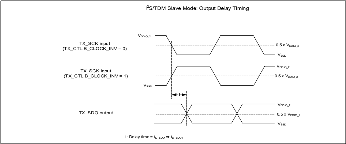
Figure 49 Slave output delay
