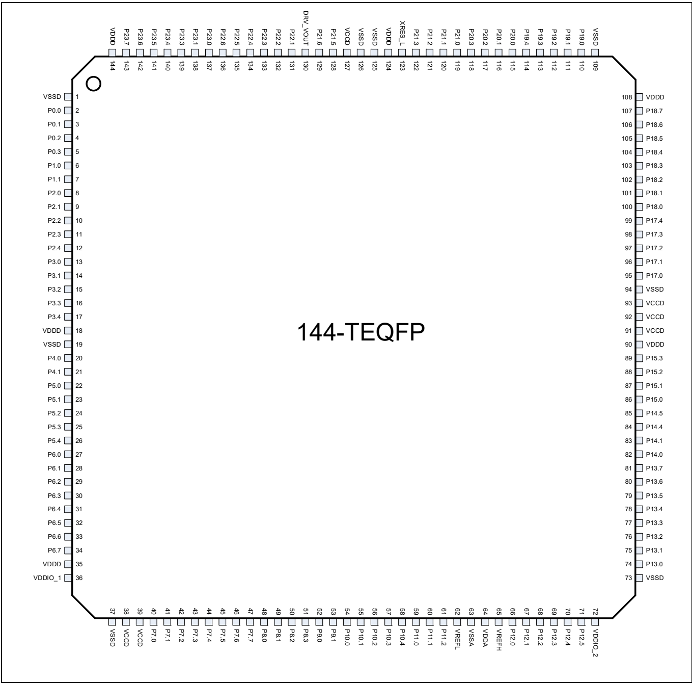
Figure 7 144-TEQFP pin assignment
