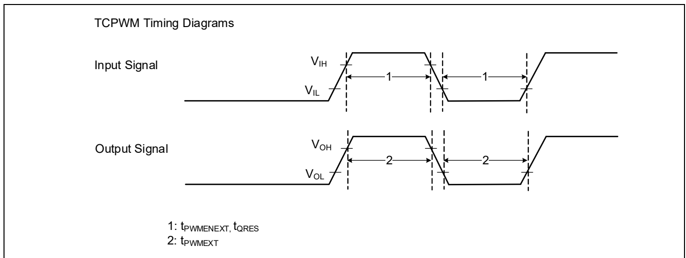
Figure 21 TCPWM timing diagrams
