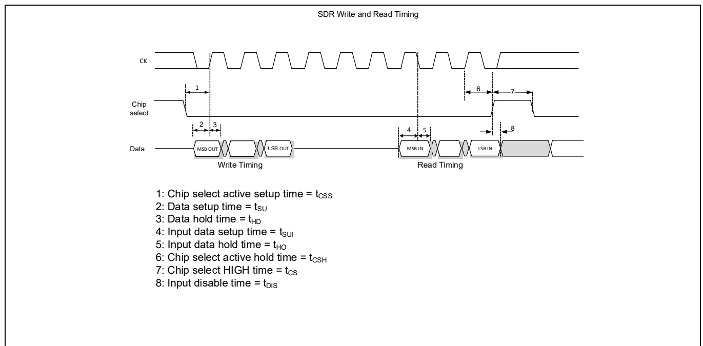
Figure 55 SDR write and read timing diagram
