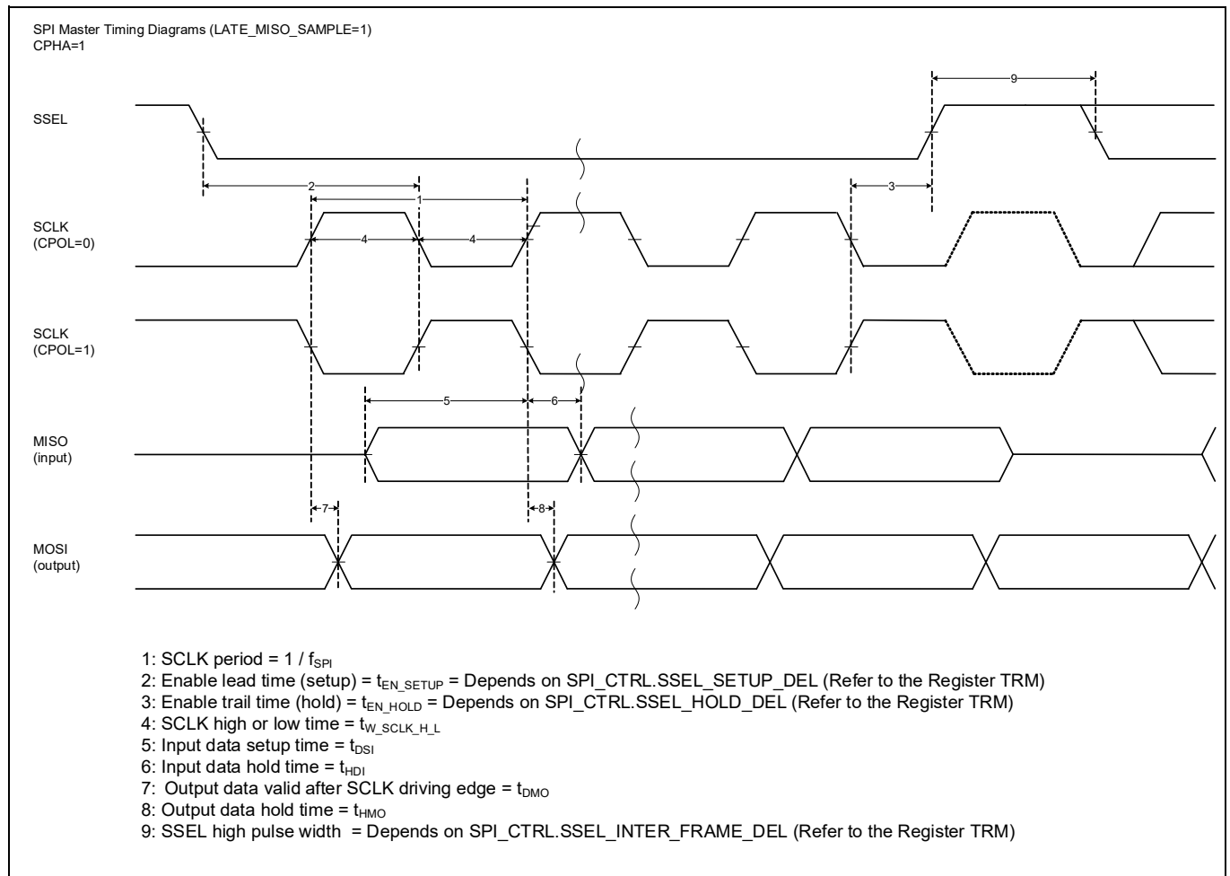
Figure 24 SPI master timing diagrams with HIGH clock phase
