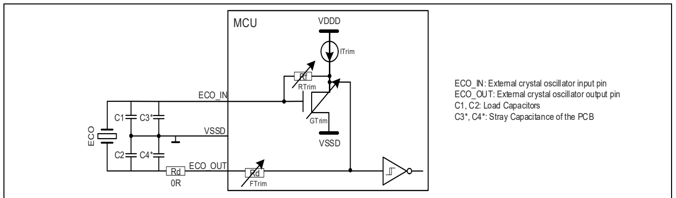
Figure 35 ECO connection scheme [73]
