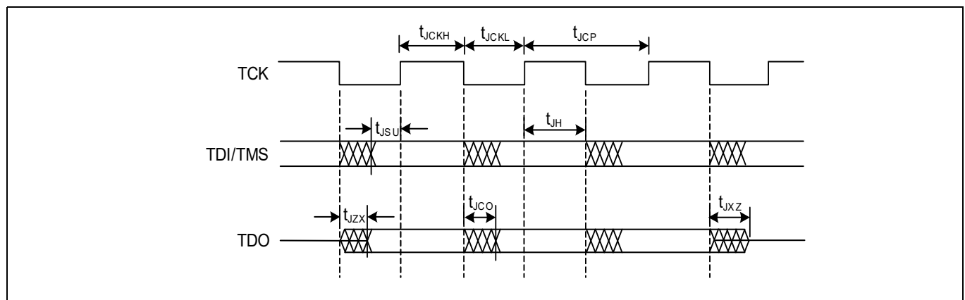
Figure 34 JTAG specifications
