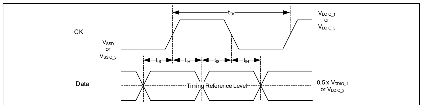
Figure 57 HYPERBUS™ timing reference level
