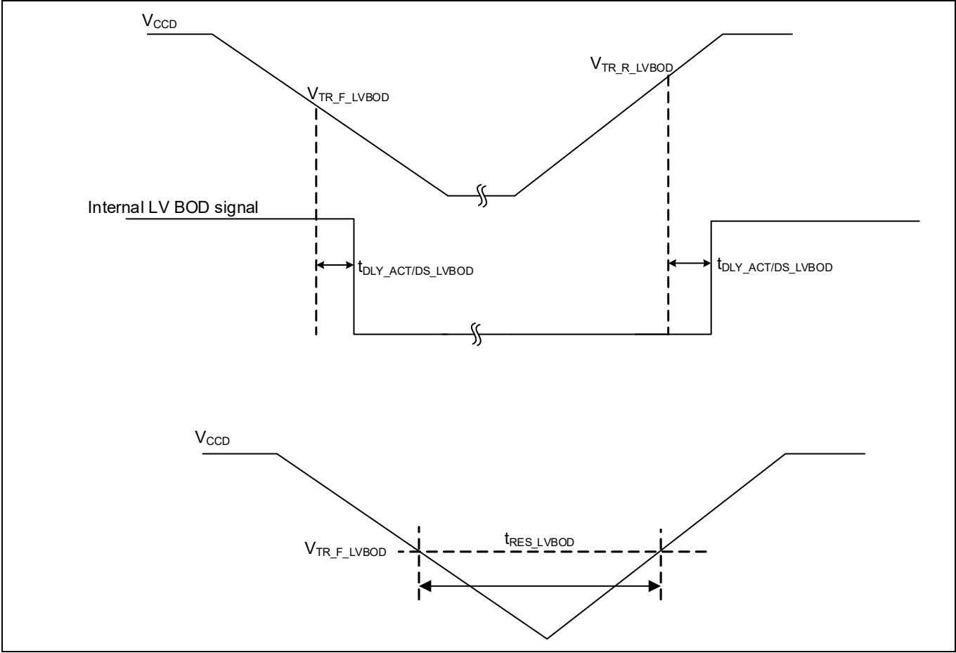
Figure 30 Low-voltage BOD specifications
