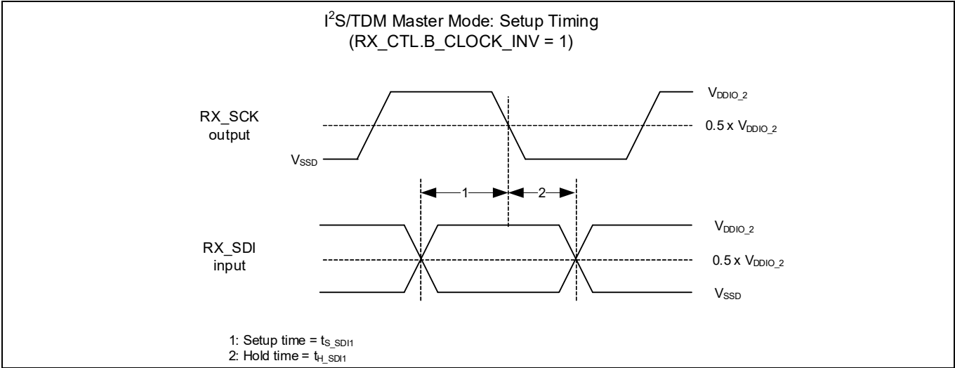
Figure 48 Master setup with clock inversion
