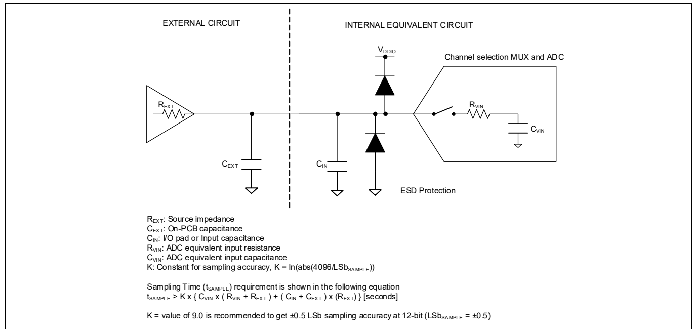
Figure 19 ADC equivalent circuit for analog input
