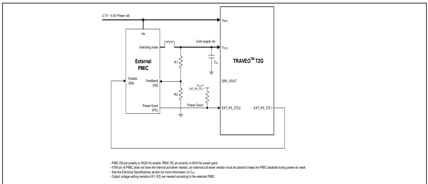
Figure 2 Sample core external regulator with PMIC/LDO
