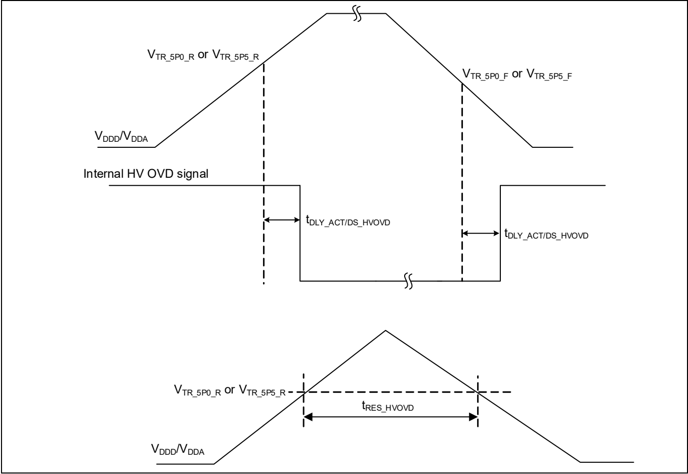
Figure 31 High-voltage OVD specifications
