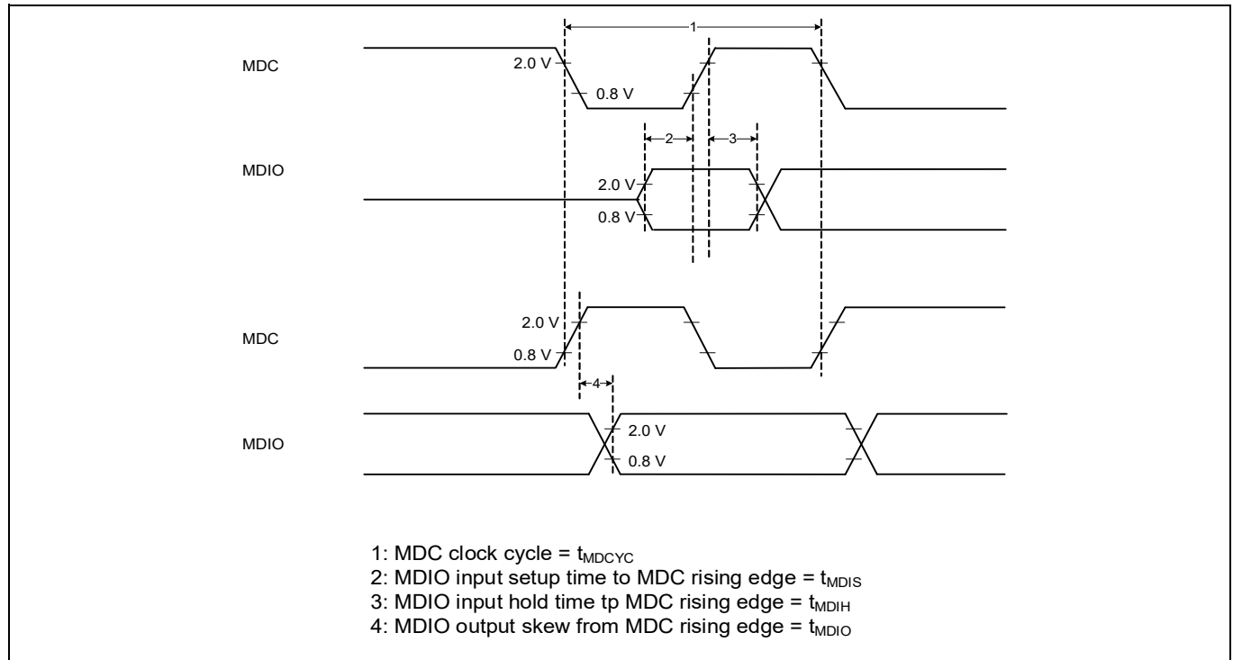
Figure 40 MDIO timing diagram
