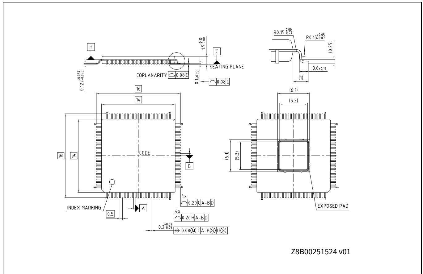
Figure 59 100-lead TEQFP (14.0 x 14.0 x 1.6 mm) LED100 package outline, Z8B00251524
