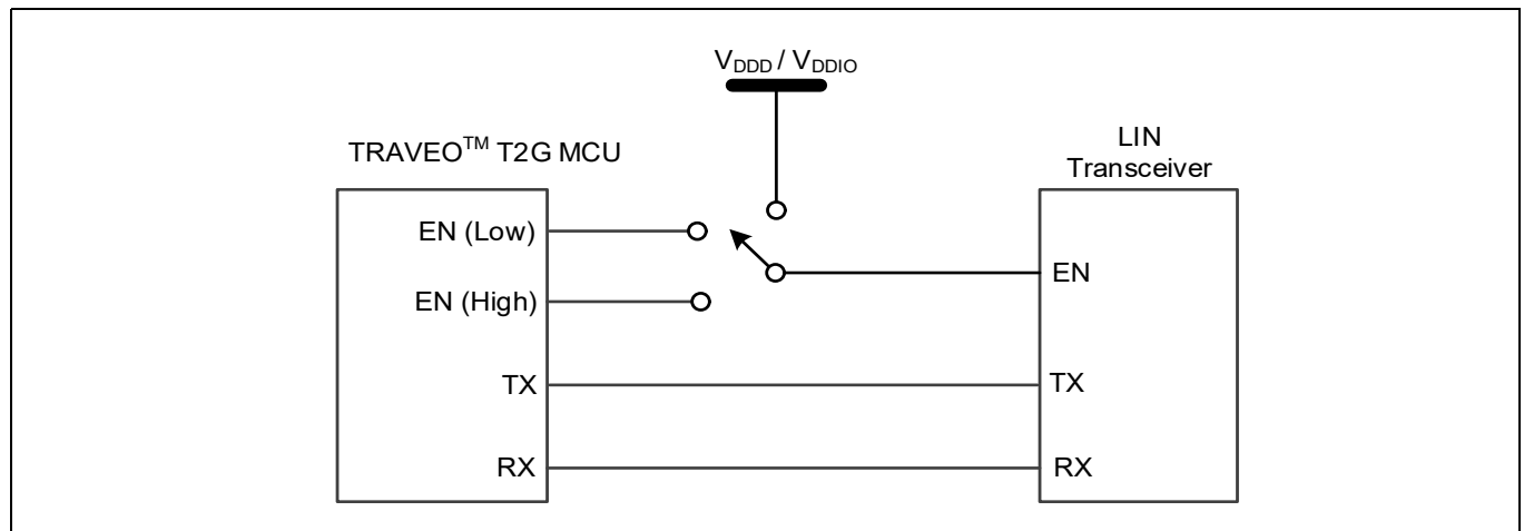
Figure 65 MCU to LIN transceiver connections
