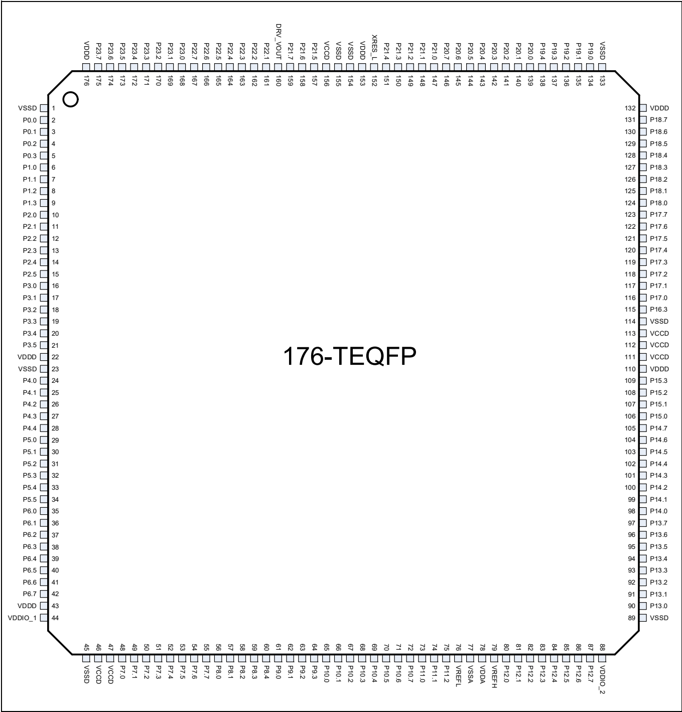
Figure 9 176-TEQFP pin assignment
