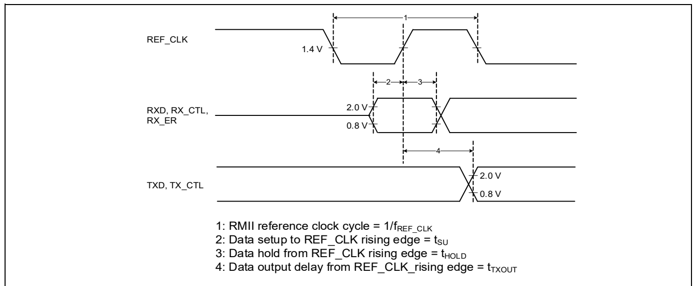
Figure 41 RMII timing diagram
