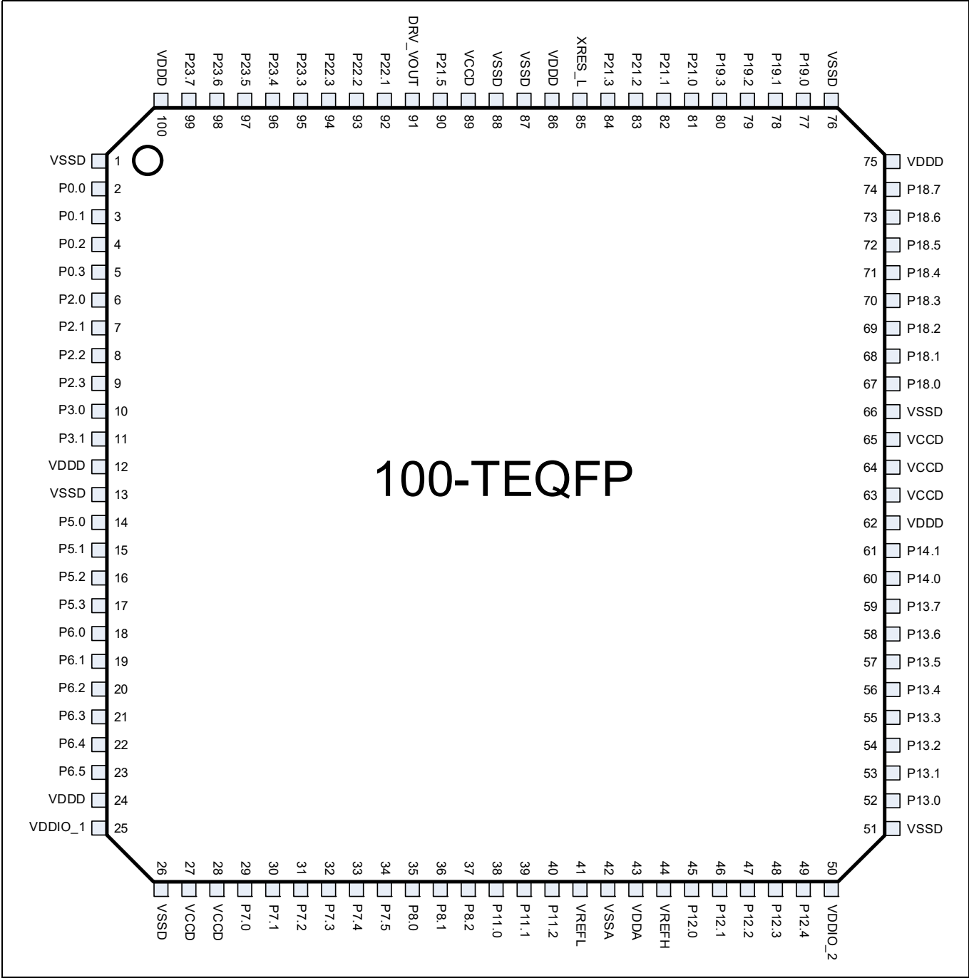
Figure 5 100-TEQFP pin assignment
