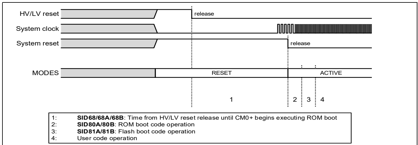
Figure 16 Reset sequence
