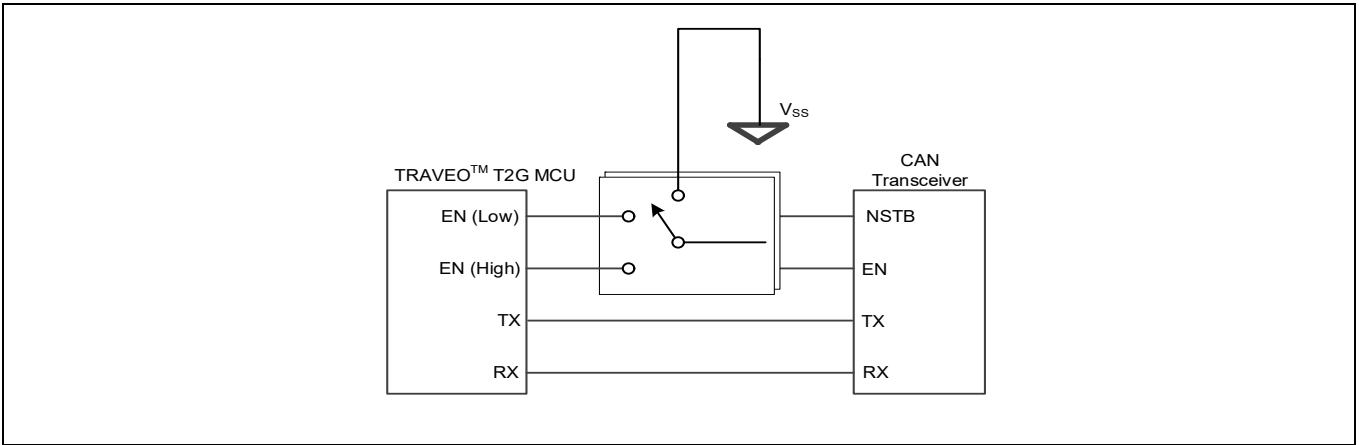
Figure 64 MCU to CAN transceiver connections
