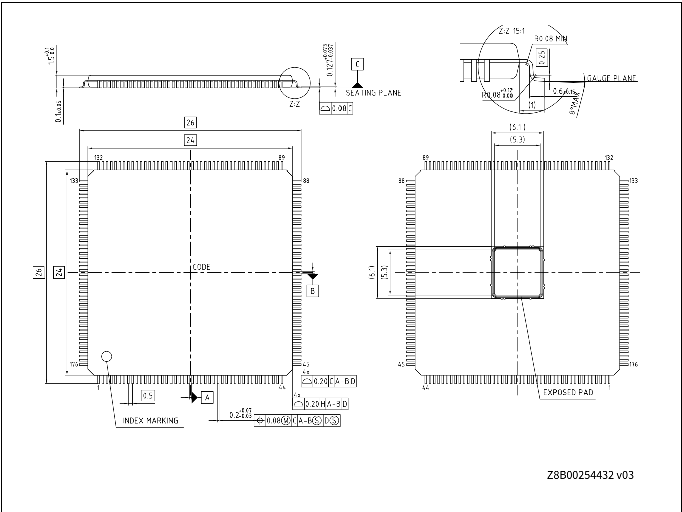
Figure 61 176-lead TEQFP (24.0 x 24.0 x 1.6 mm) LEN176 package outline, Z8B00254432
