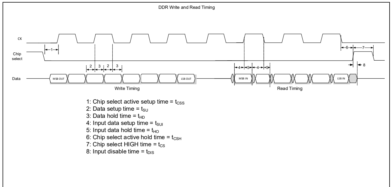
Figure 56 DDR write and read timing diagram
