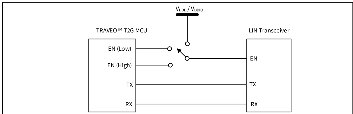
Figure 47 MCU to LIN transceiver connections
