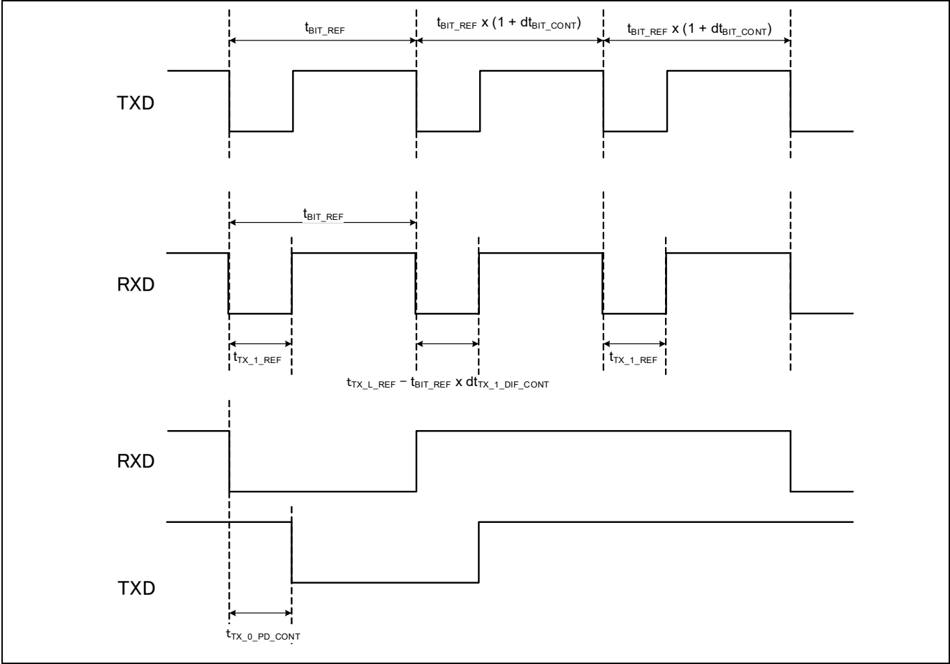
Figure 27 CXPI specifications
