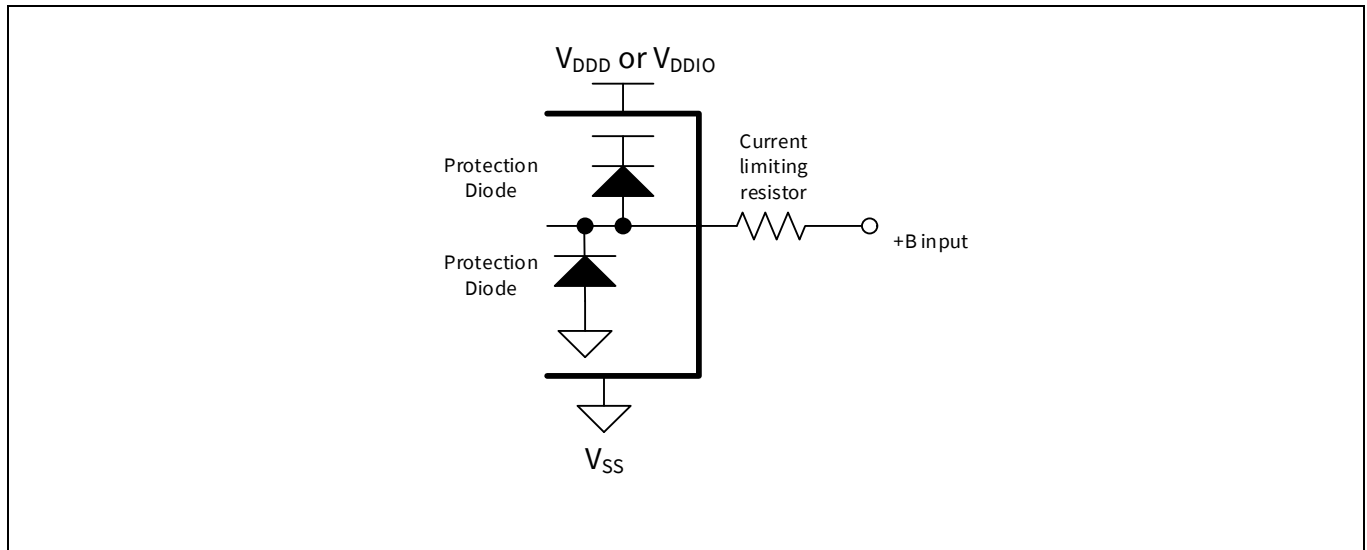
Figure 14 Example of a recommended circuit [43]
