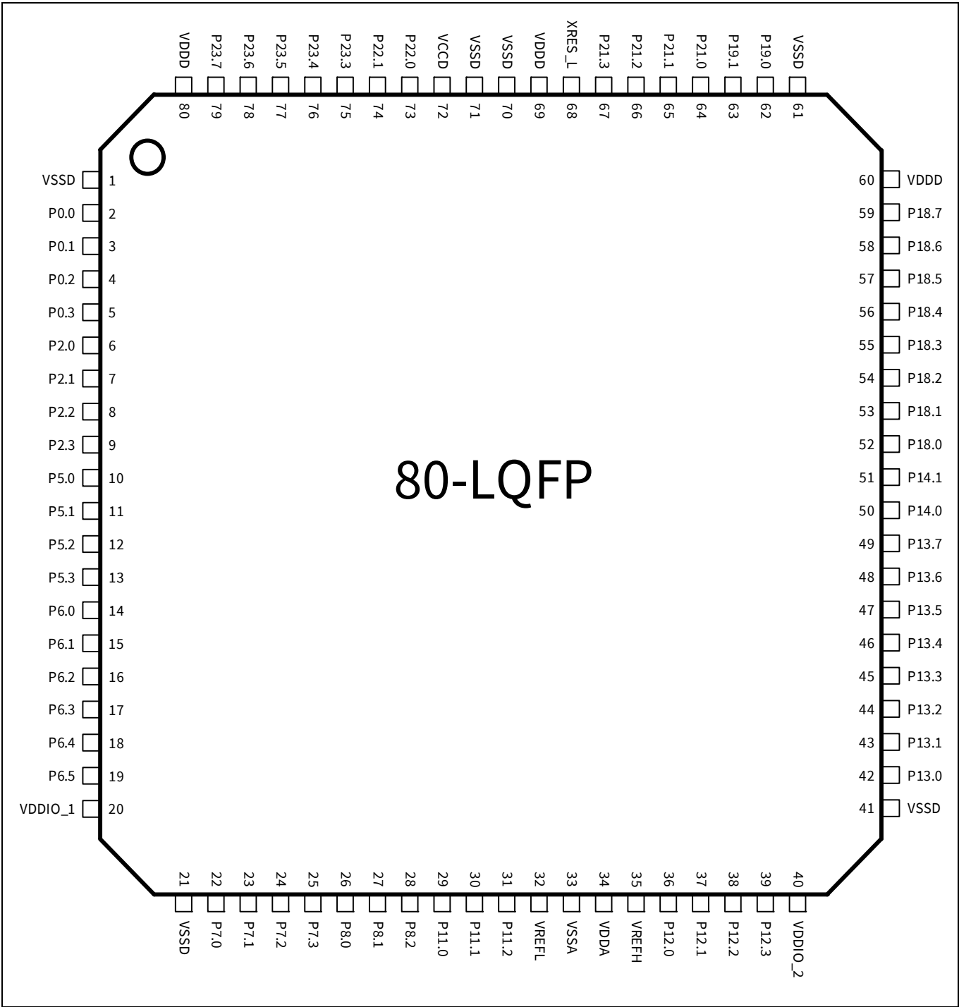
Figure 9 80-LQFP pin assignment
