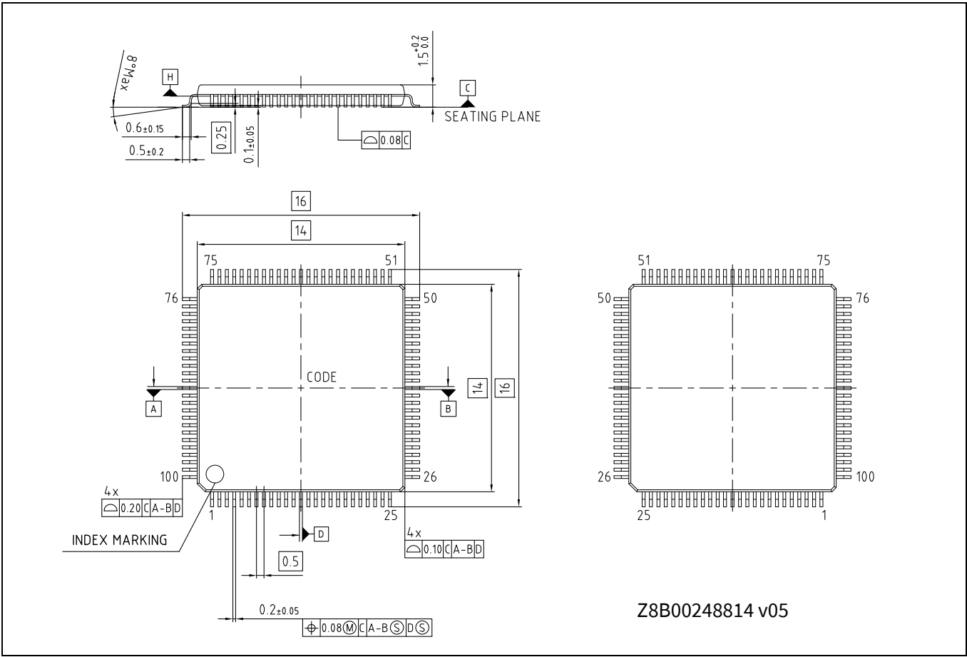
Figure 42 100-LQFP package outline (PG-LQFP-100)
