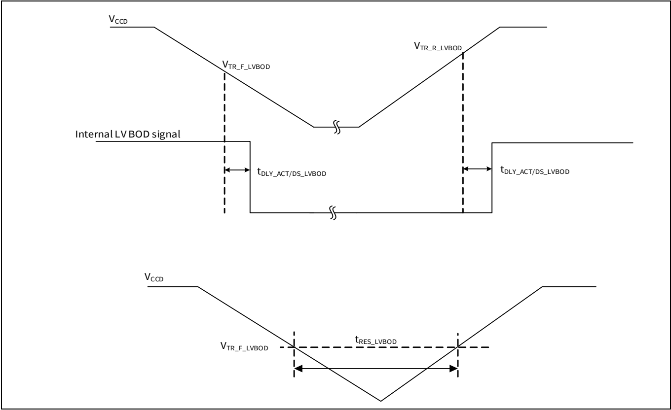
Figure 31 Low-voltage BOD specifications
