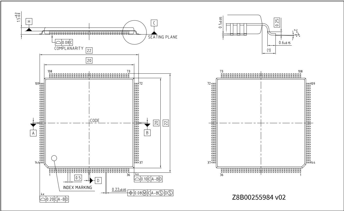
Figure 41 144-LQFP Package outline (PG-LQFP-144)
