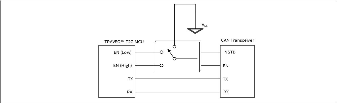
Figure 46 MCU to CAN transceiver connections
