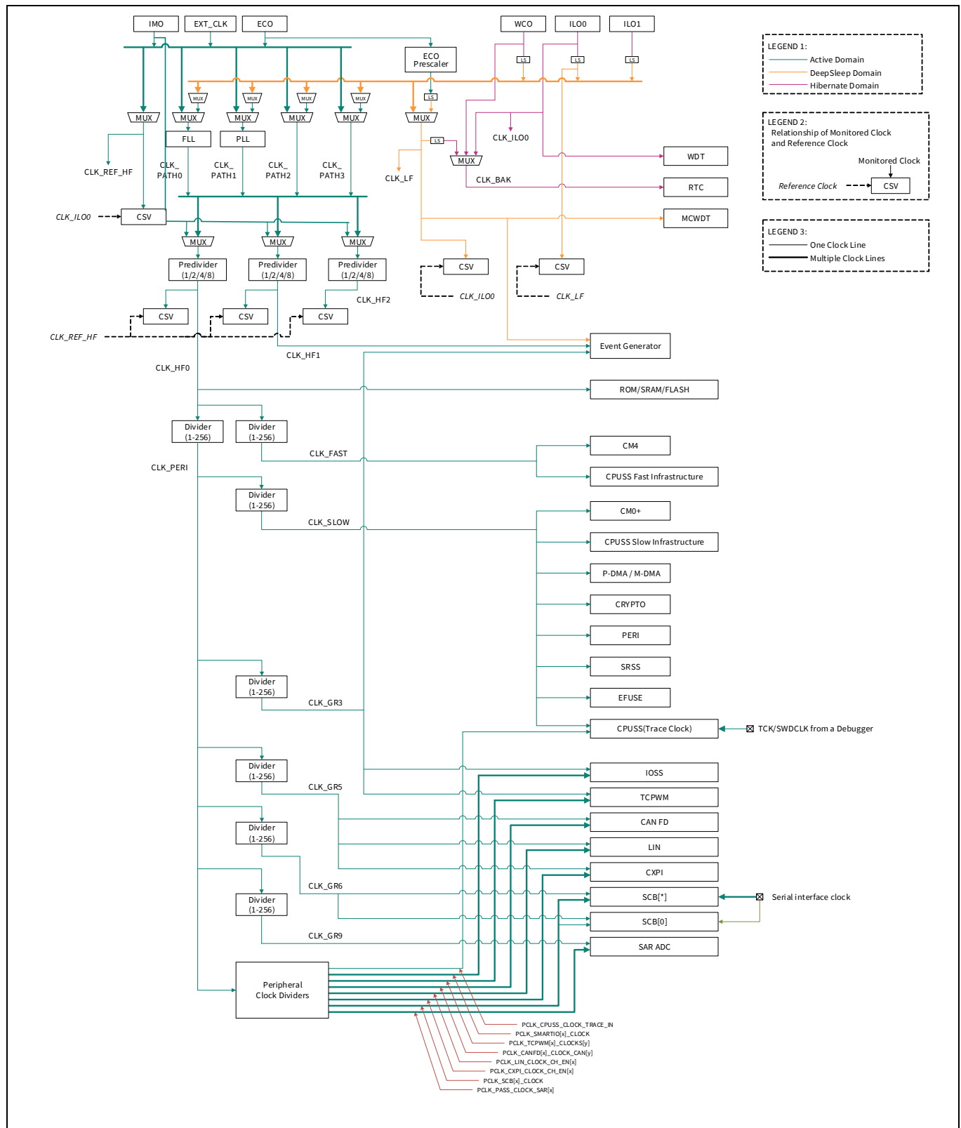
Figure 2 CYT2BL clock diagram
