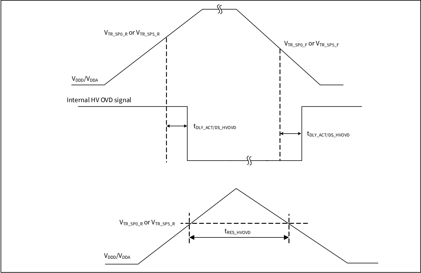
Figure 32 High-voltage OVD specifications
