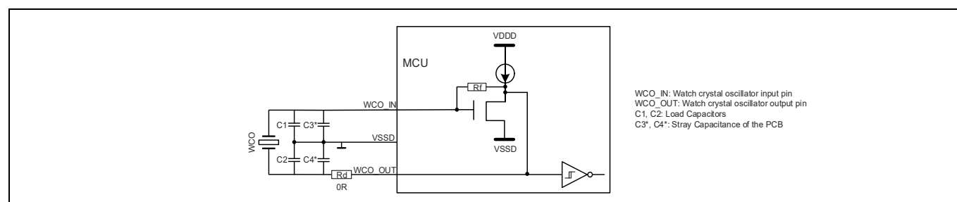
Figure 37 WCO connection scheme [63]
