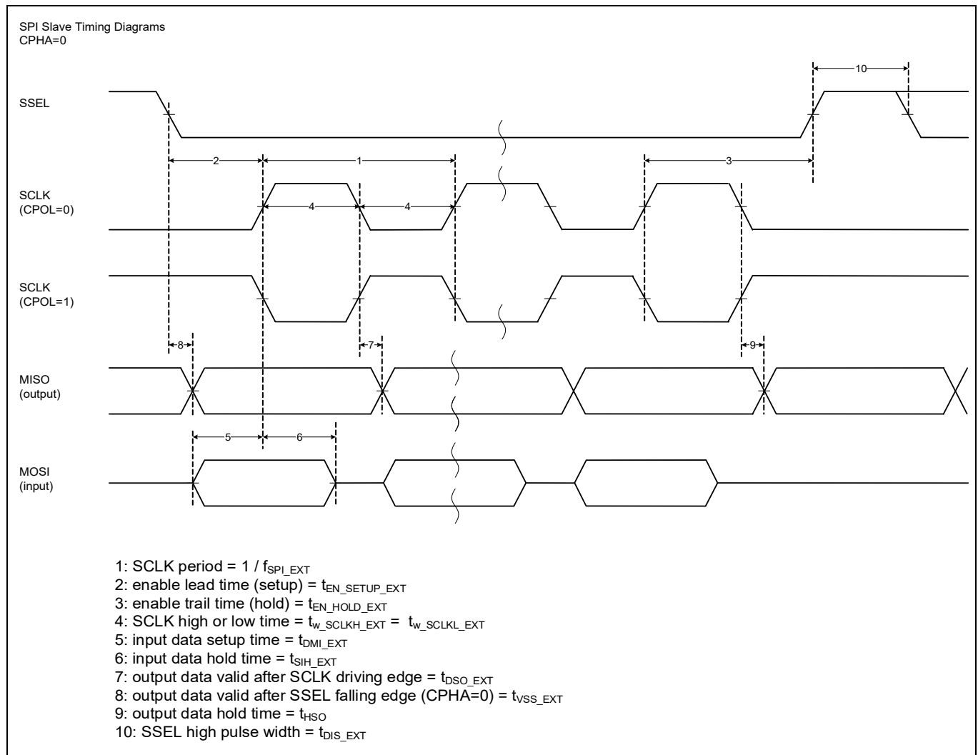
Figure 25 SPI slave timing diagrams with LOW clock phase
