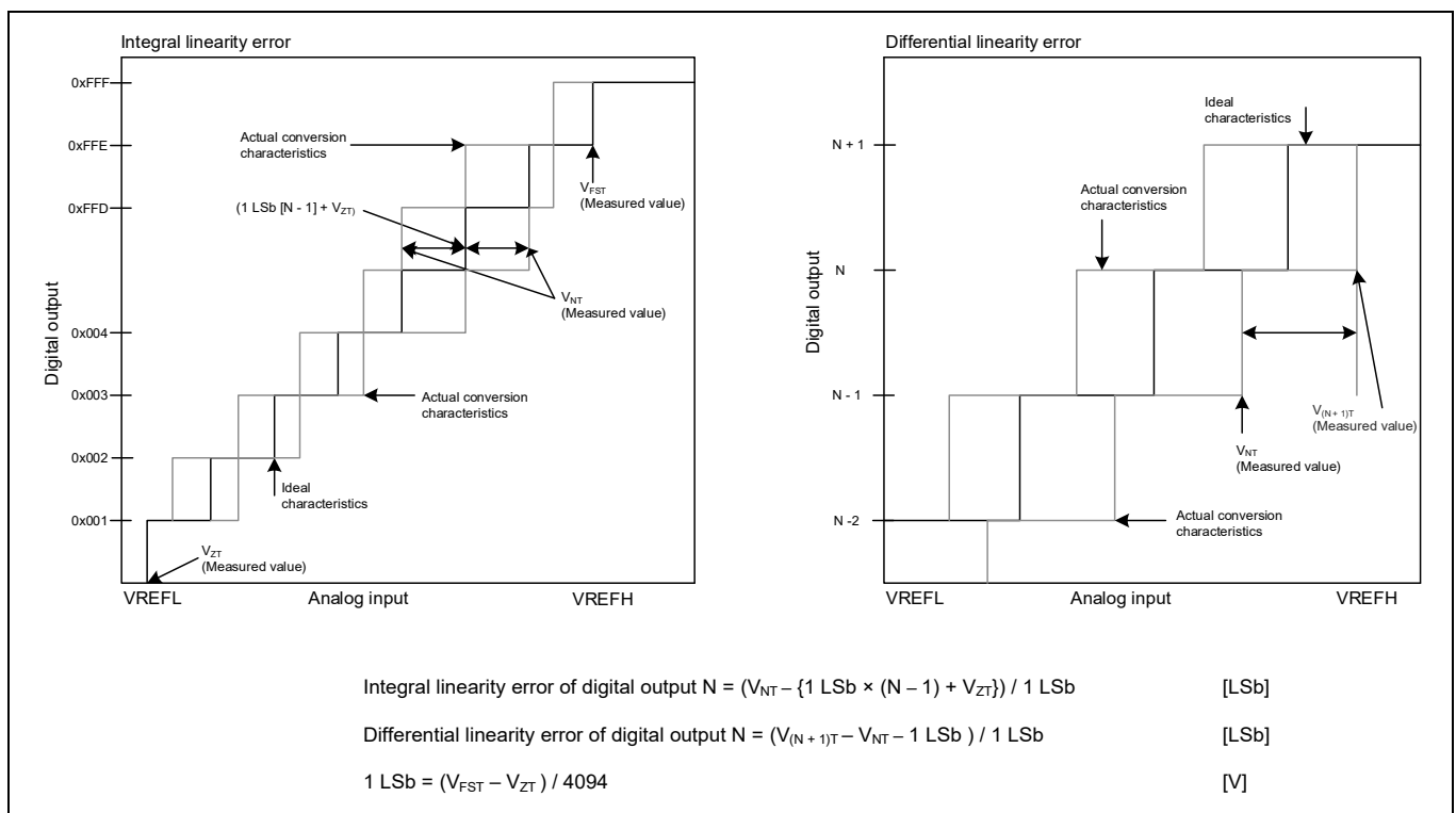
Figure 18 Integral and differential linearity errors
