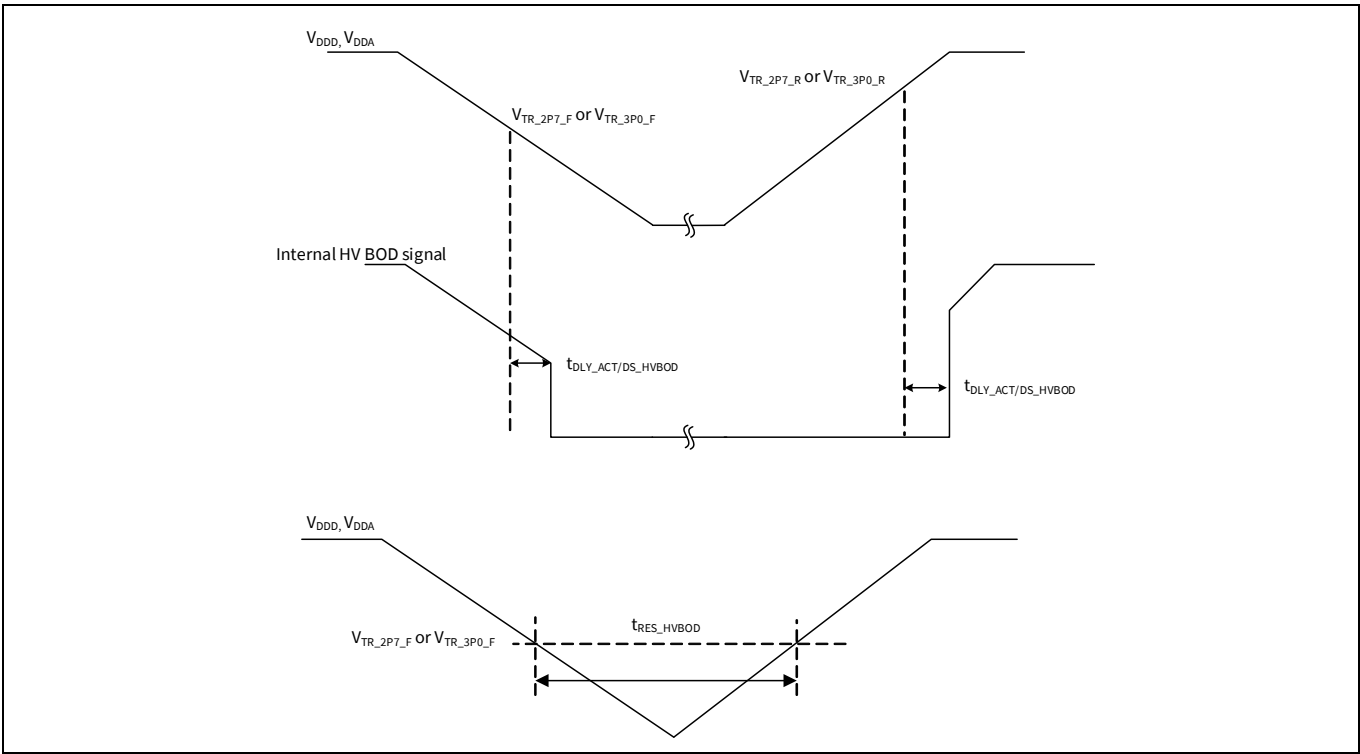
Figure 30 High-voltage BOD specifications
