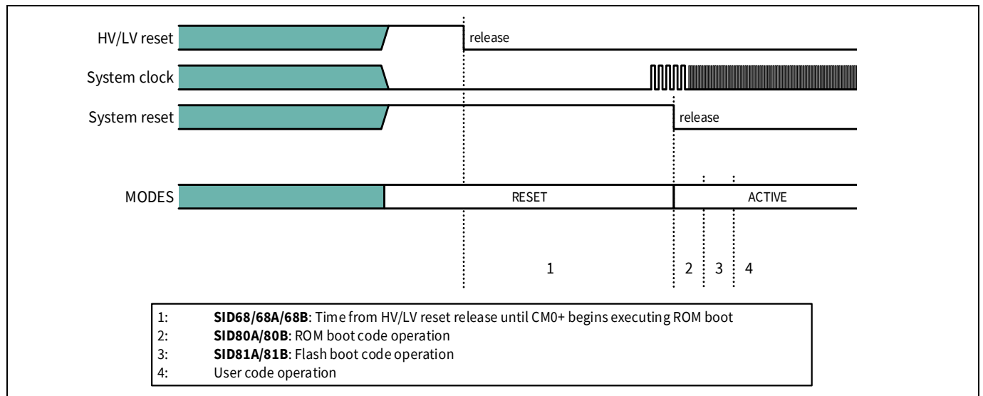
Figure 16 Reset sequence
