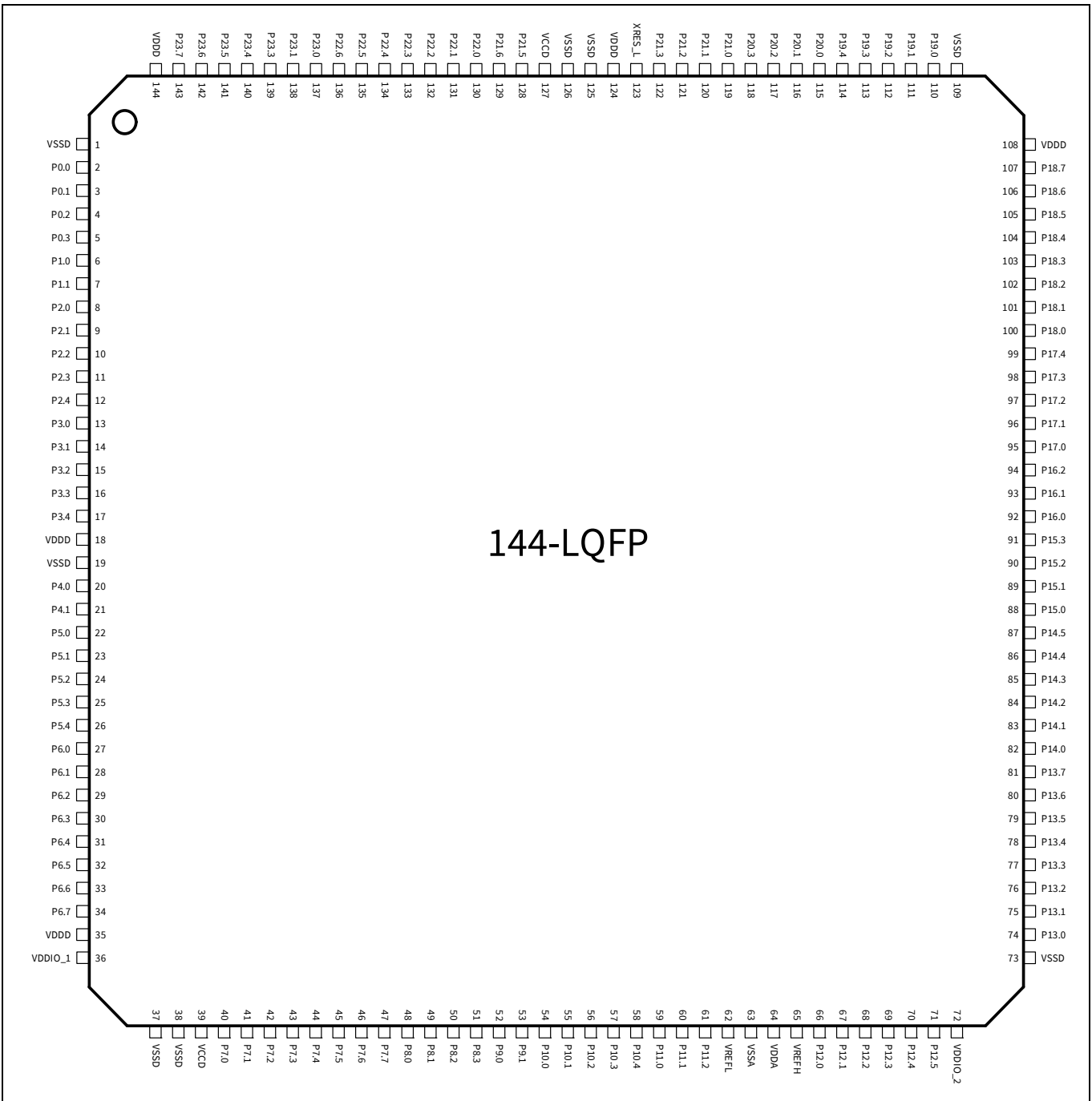
Figure 5 144-LQFP pin assignment
