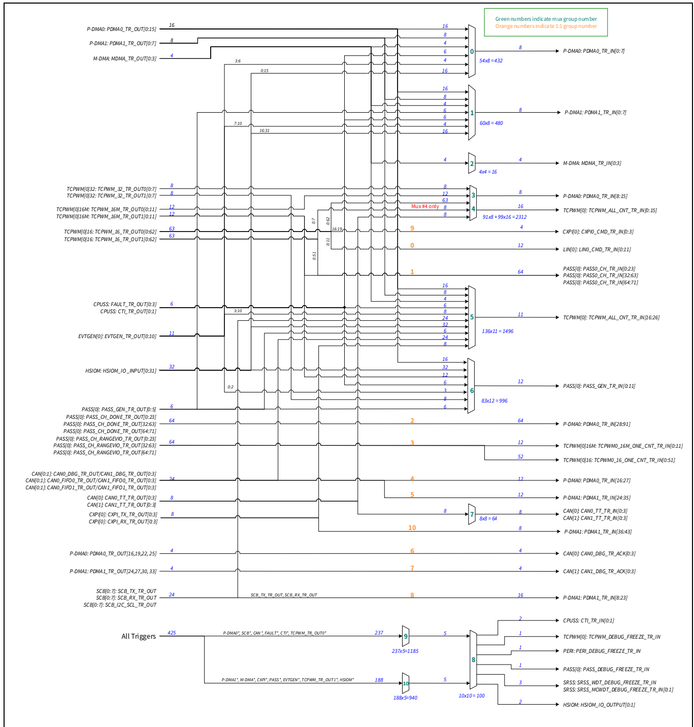
Figure 13 Trigger multiplexer [31]
