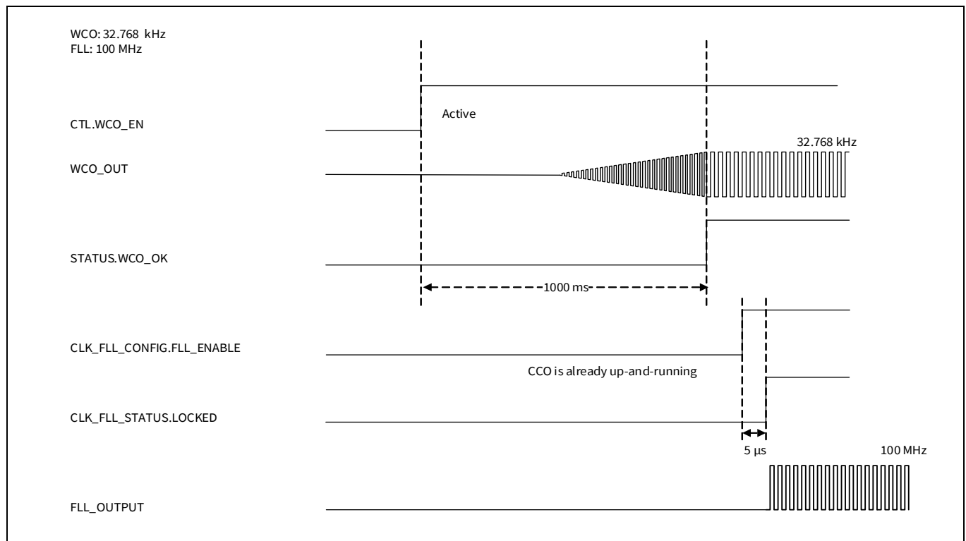
Figure 39 WCO to FLL diagram
