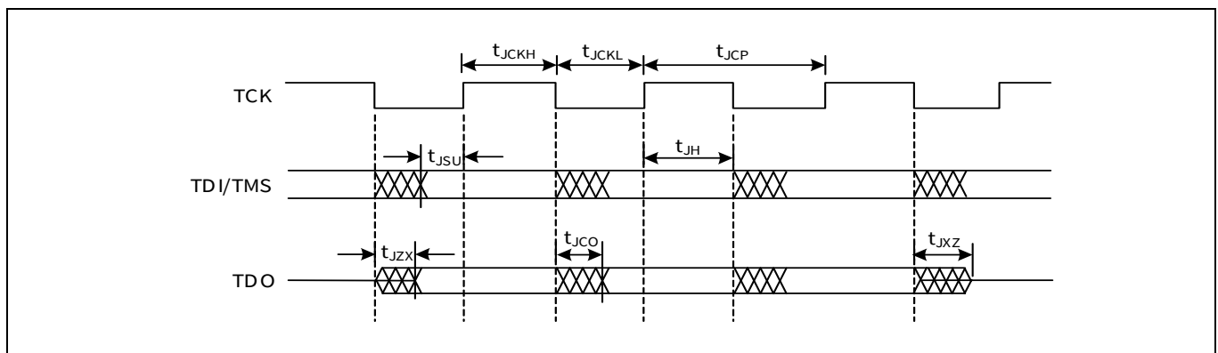
Figure 35 JTAG specifications
