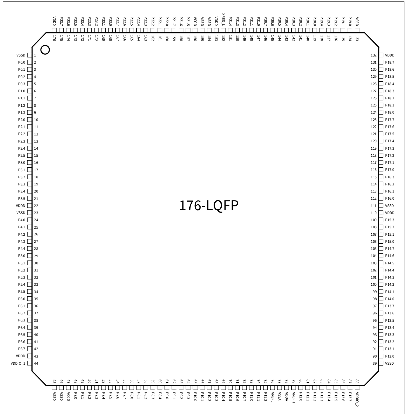
Figure 3 176-LQFP pin assignment
