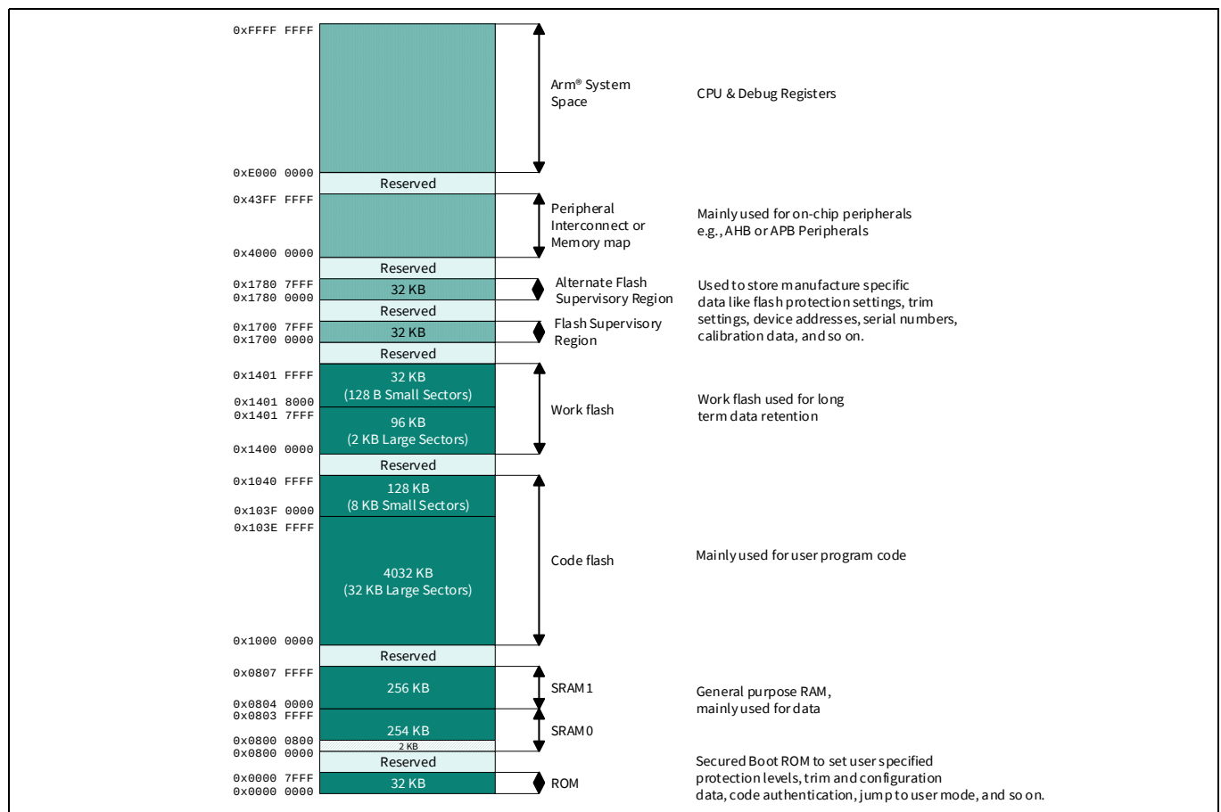
Figure 1 CYT2BL address map [14, 15]
