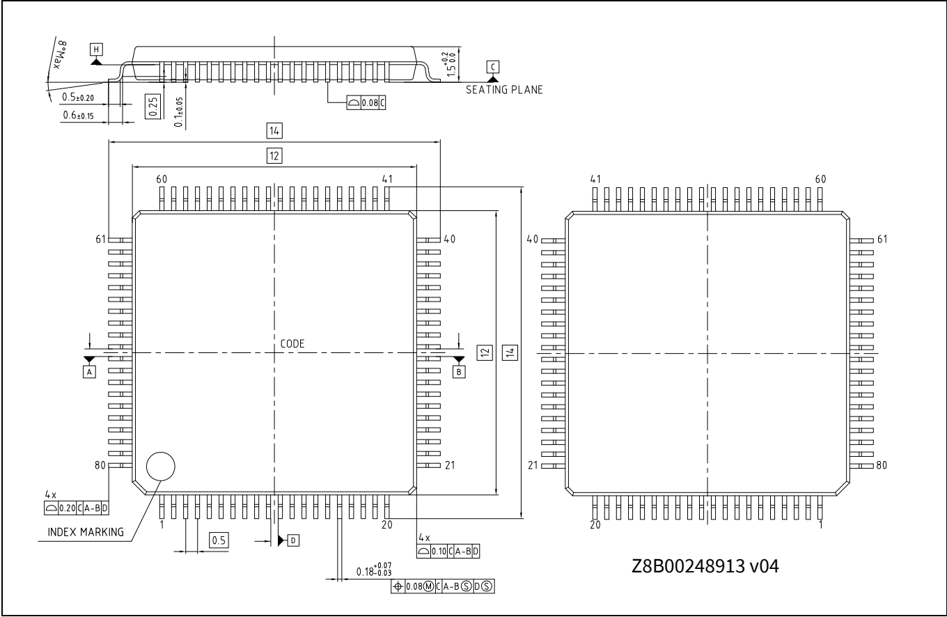
Figure 43 80-LQFP package outline (PG-LQFP-80)
