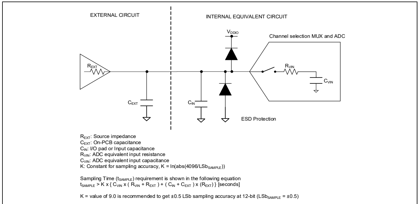
Figure 19 ADC equivalent circuit for analog input
