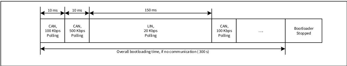
Figure 45 Bootloading sequence
