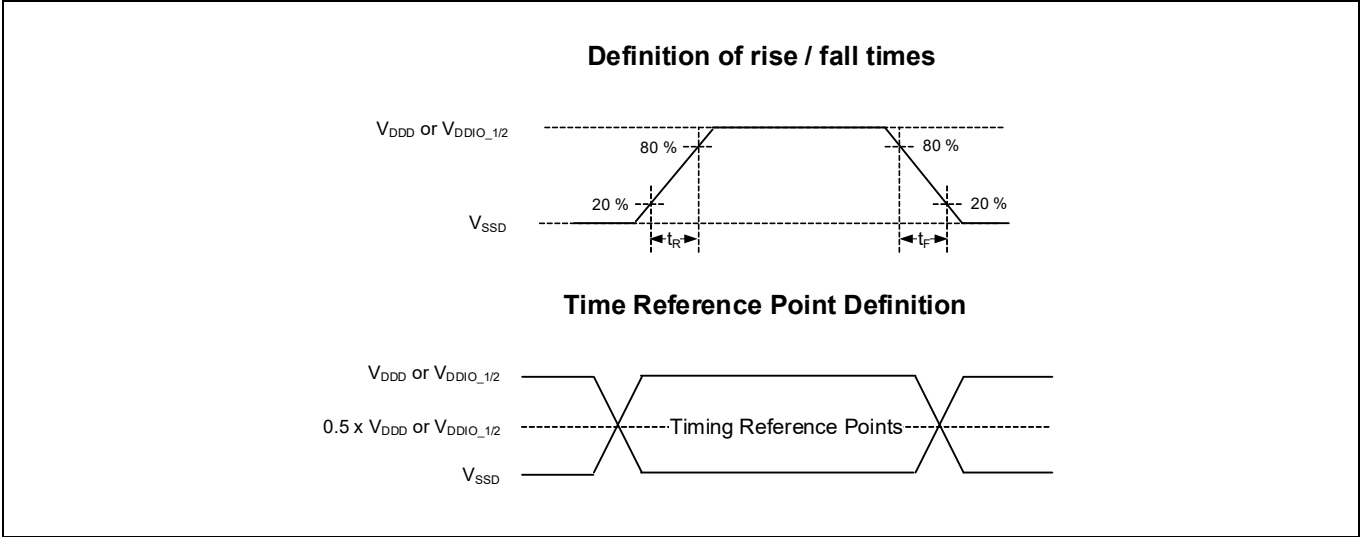
Figure 20 AC timings specifications
