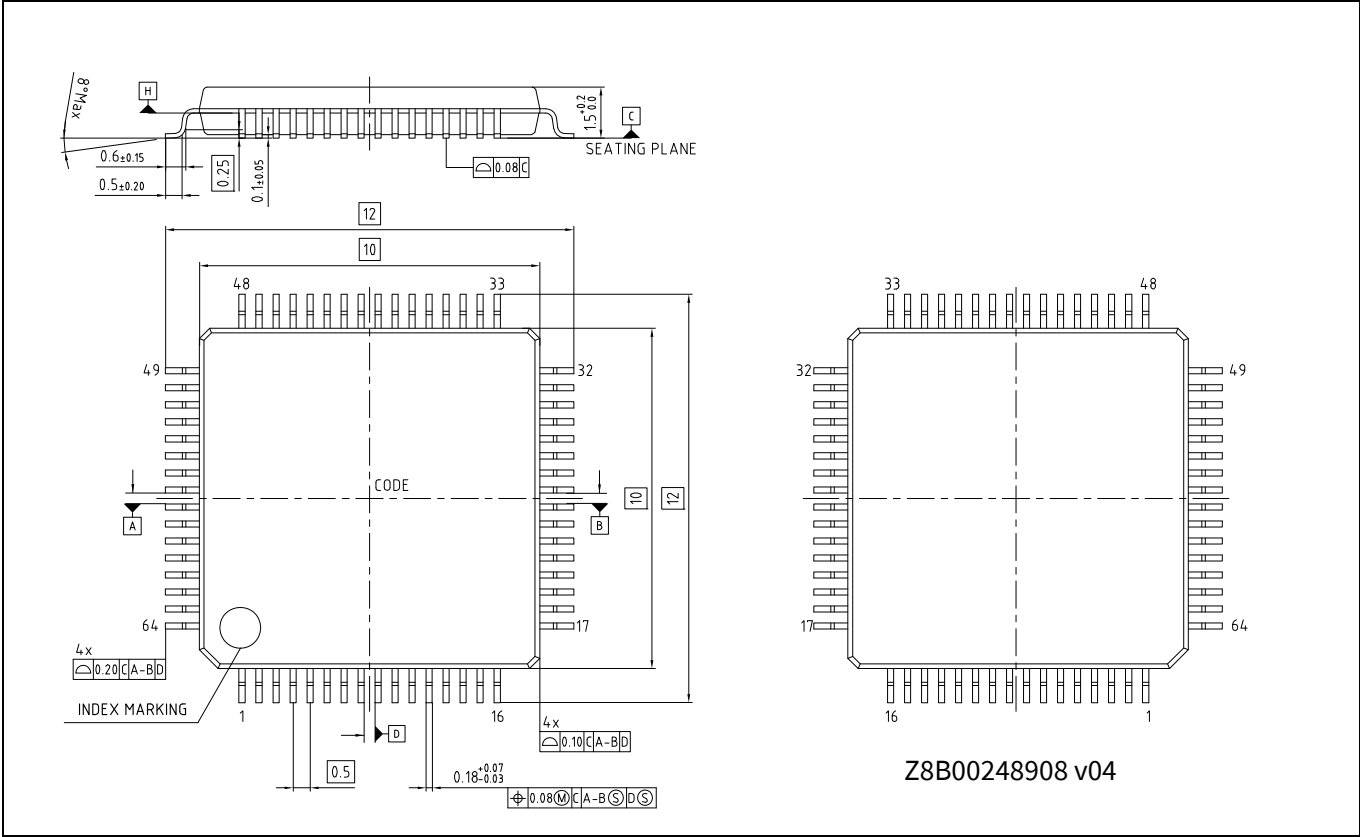
Figure 44 64-LQFP package outline (PG-LQFP-64)
