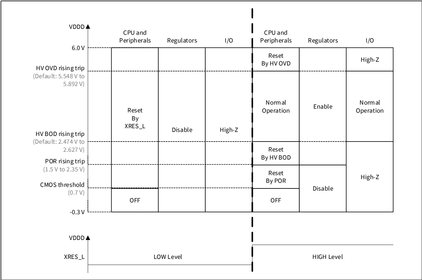
Figure 28 Device operations supply range
