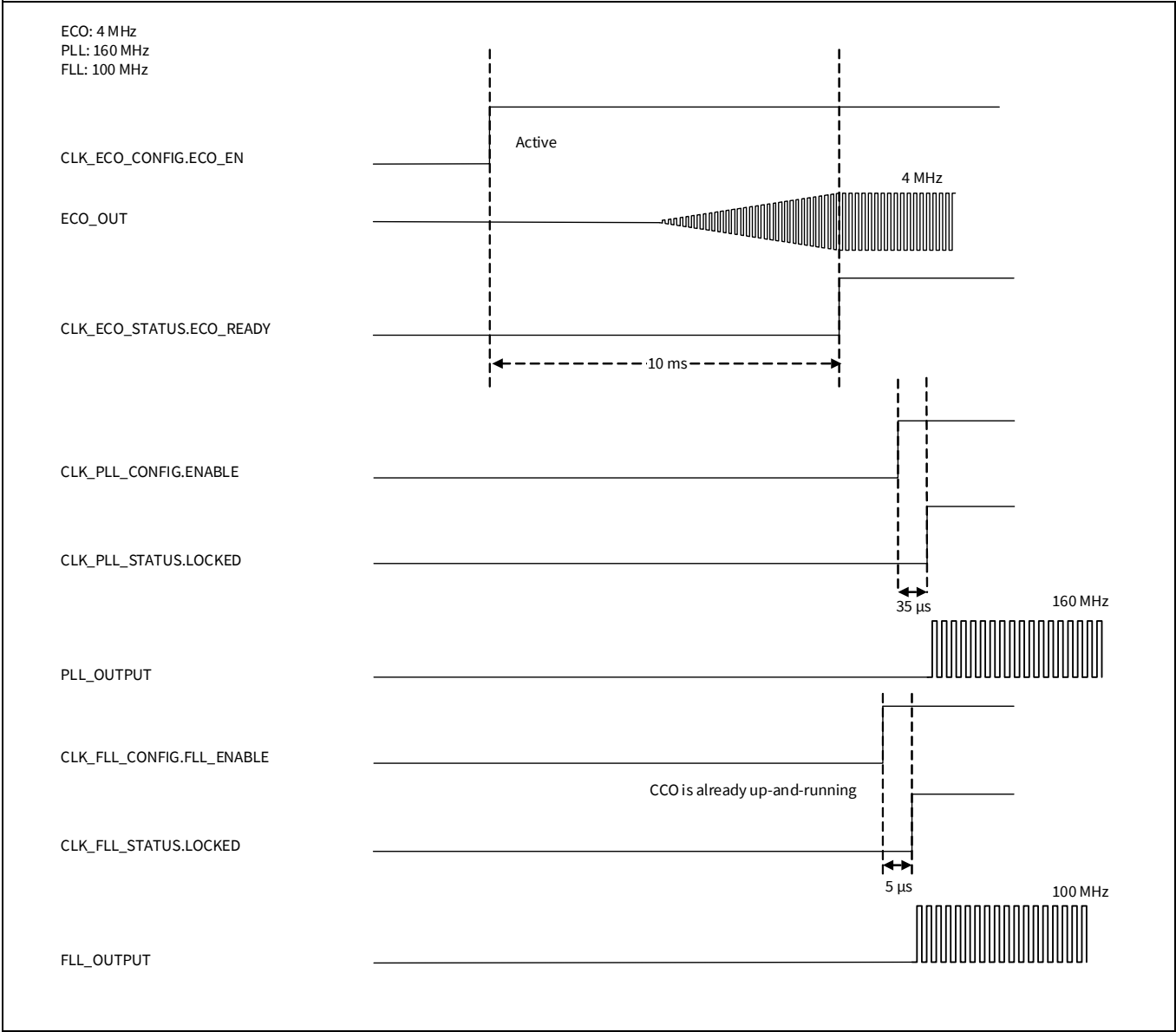
Figure 38 ECO to PLL or FLL diagram
