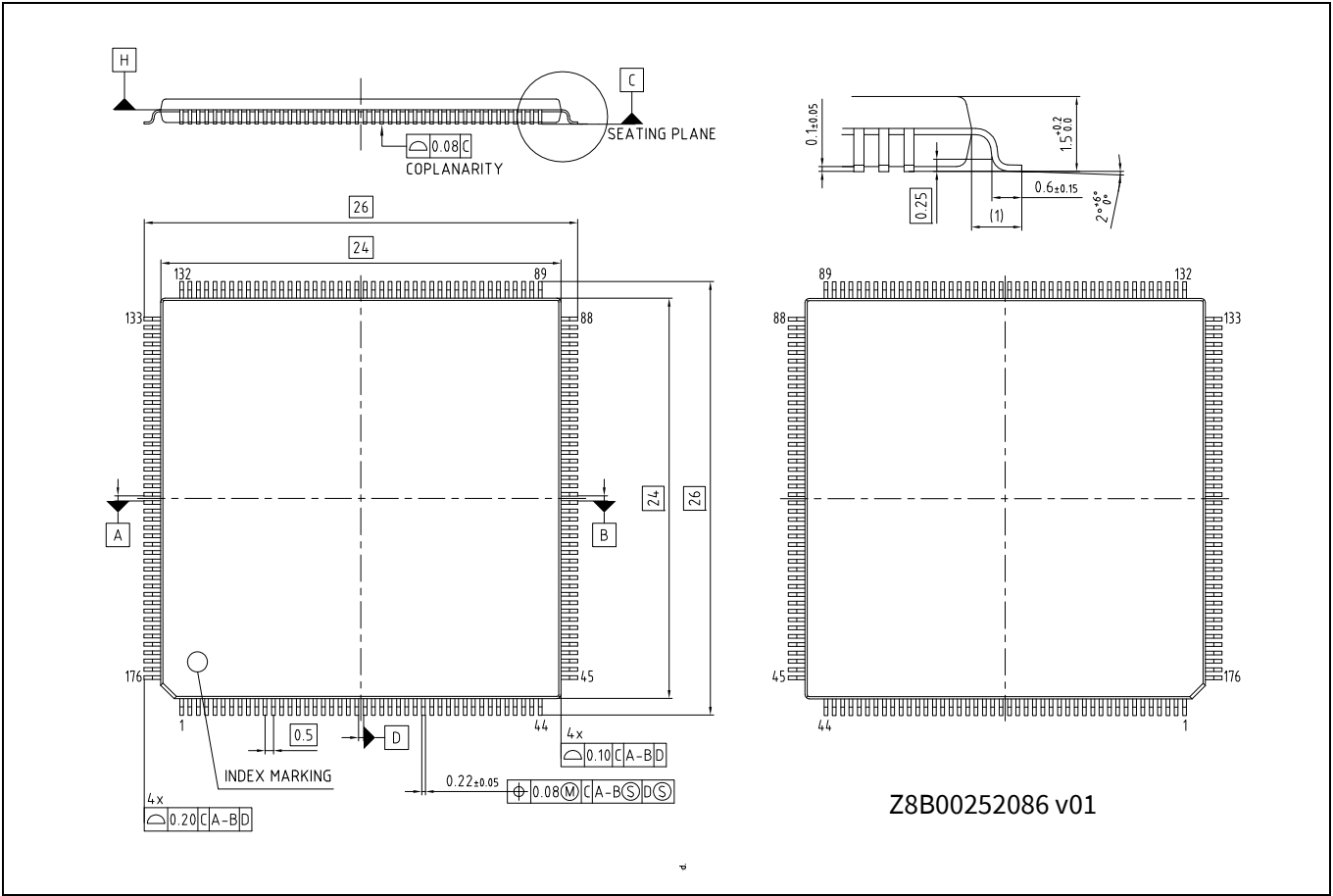
Figure 40 176-LQFP Package outline (PG-LQFP-176)
