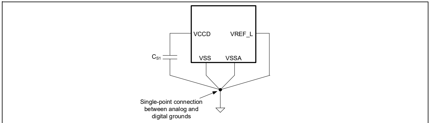
Figure 15 Smoothing capacitor
