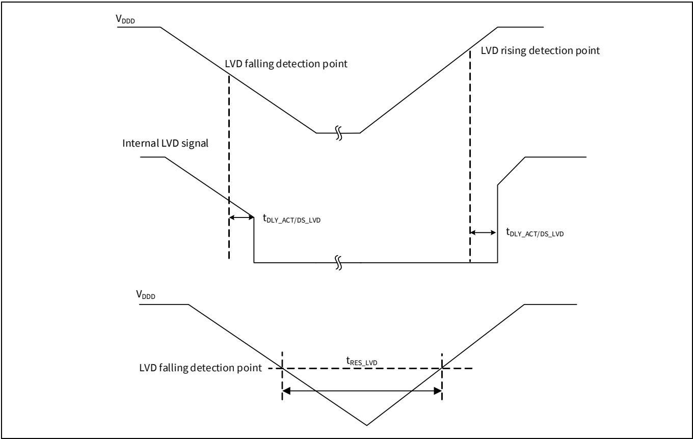
Figure 34 LVD specifications
