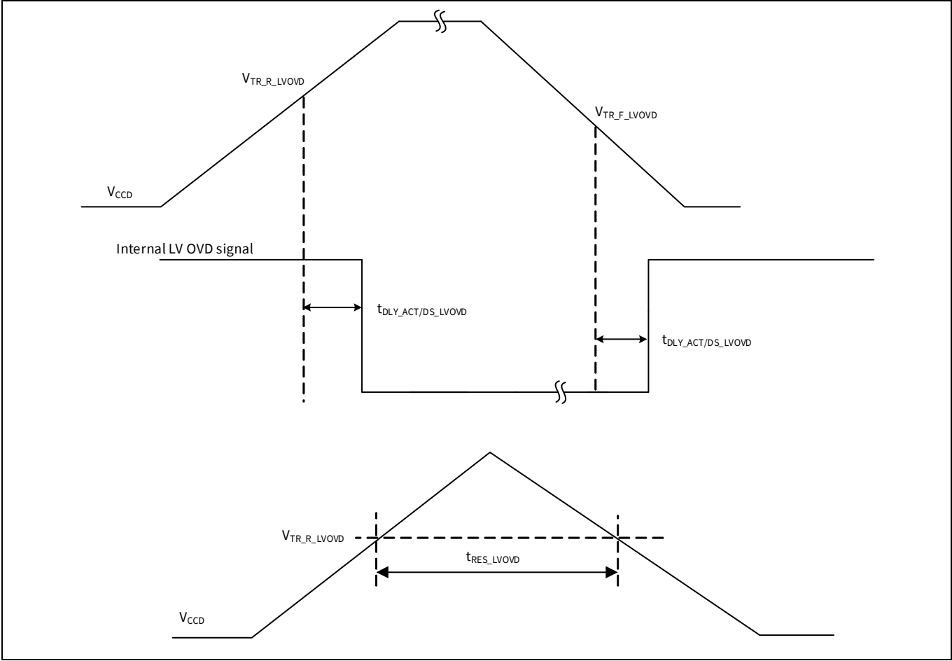
Figure 33 Low-voltage OVD specifications
