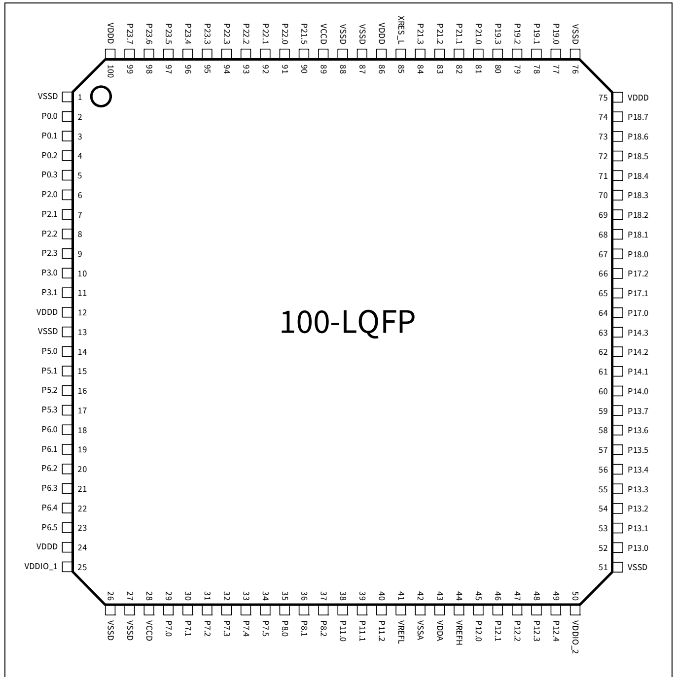
Figure 7 100-LQFP pin assignment
