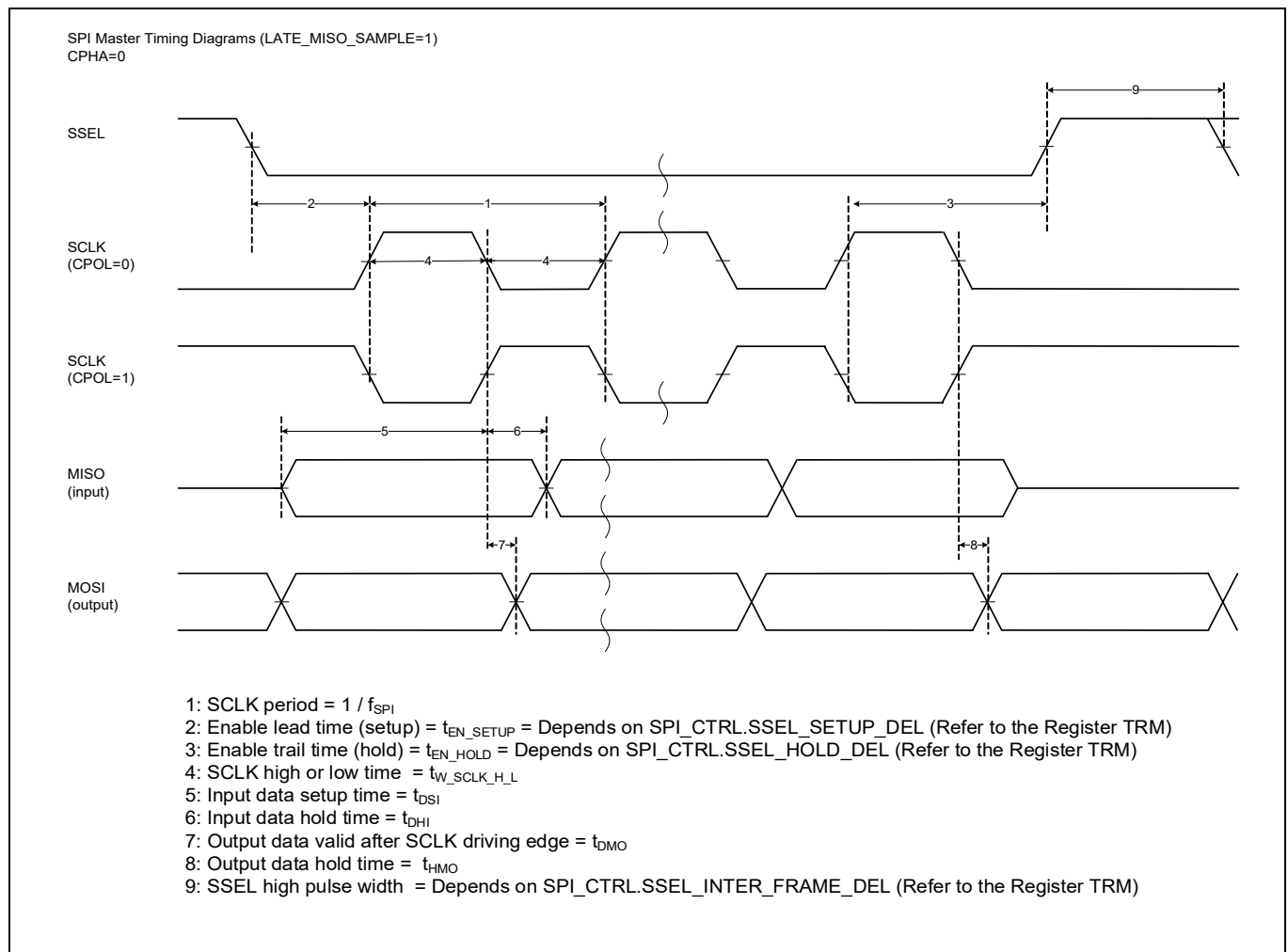
Figure 23 SPI master timing diagrams with LOW clock phase
