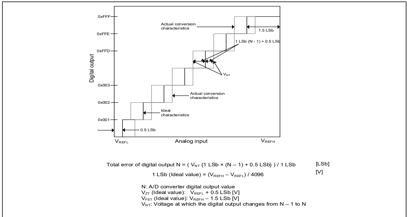
Figure 17 ADC characteristics and error definitions
