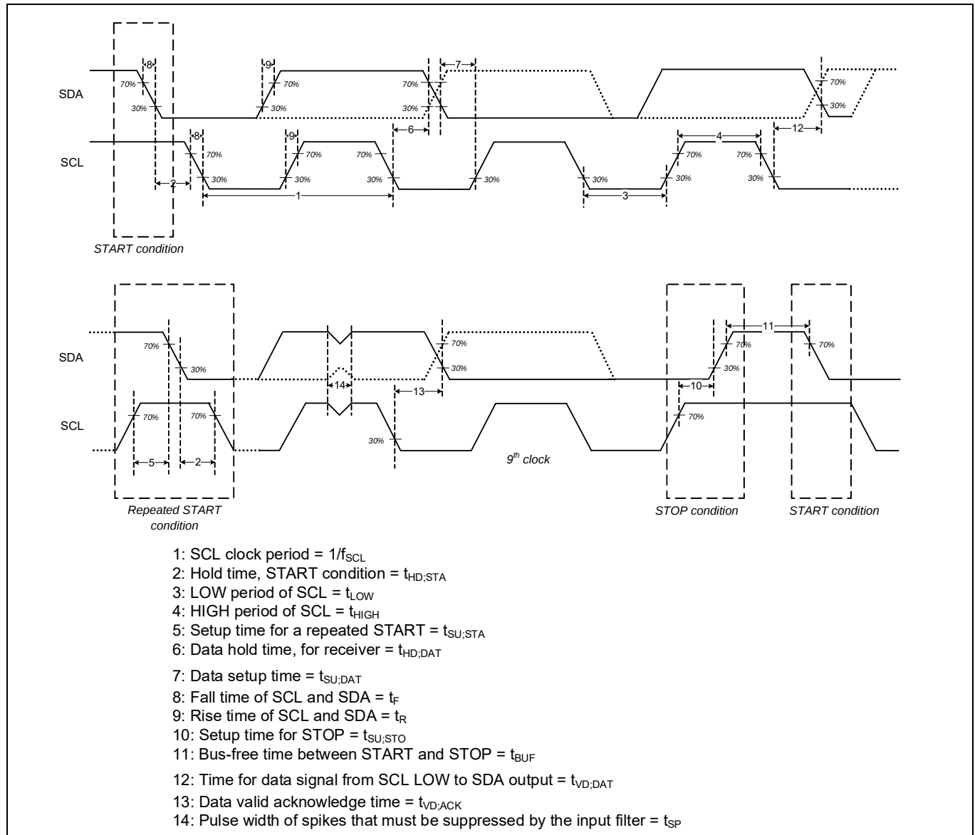
Figure 22 I 2 C timing diagrams
