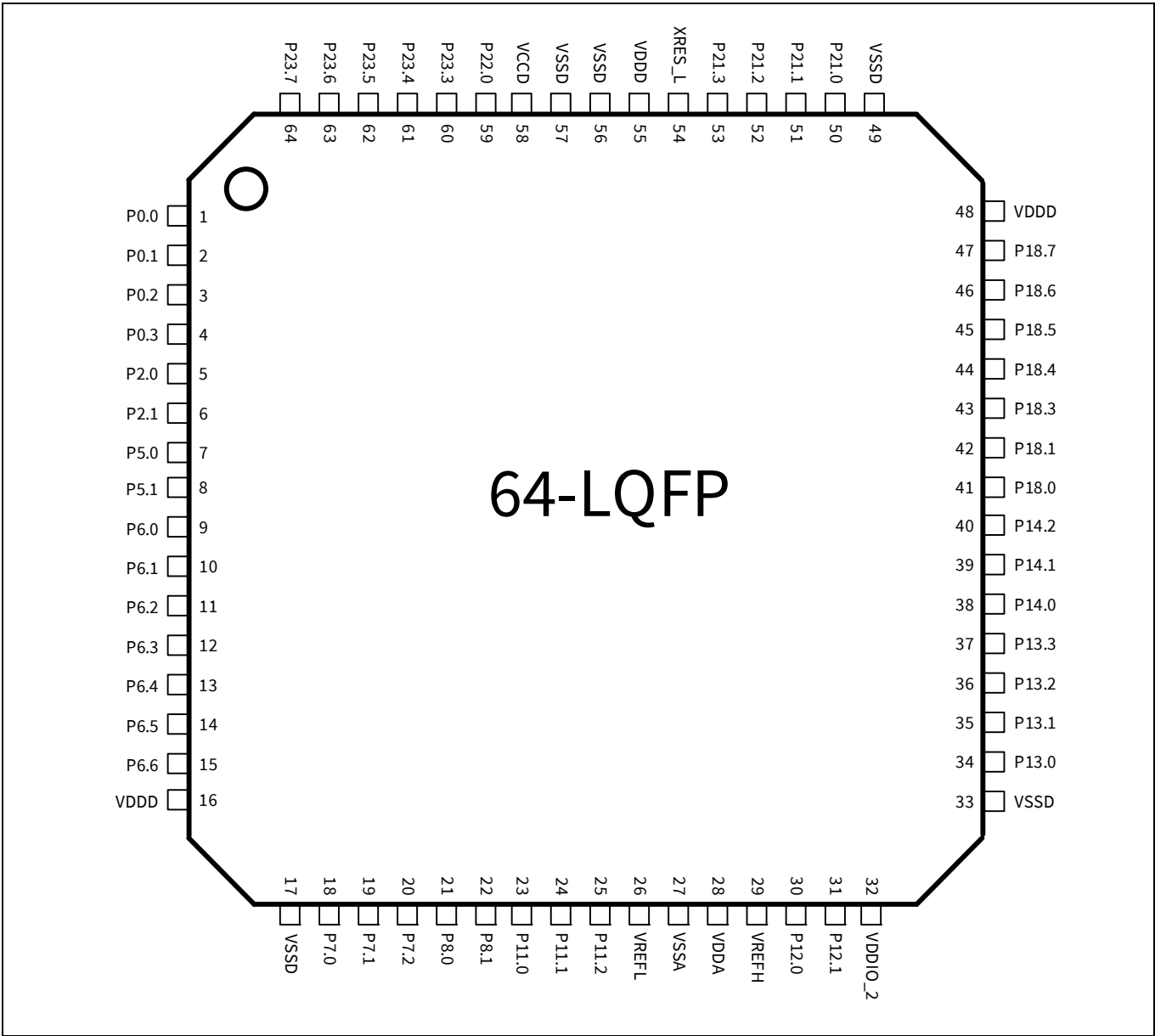
Figure 11 64-LQFP pin assignment
