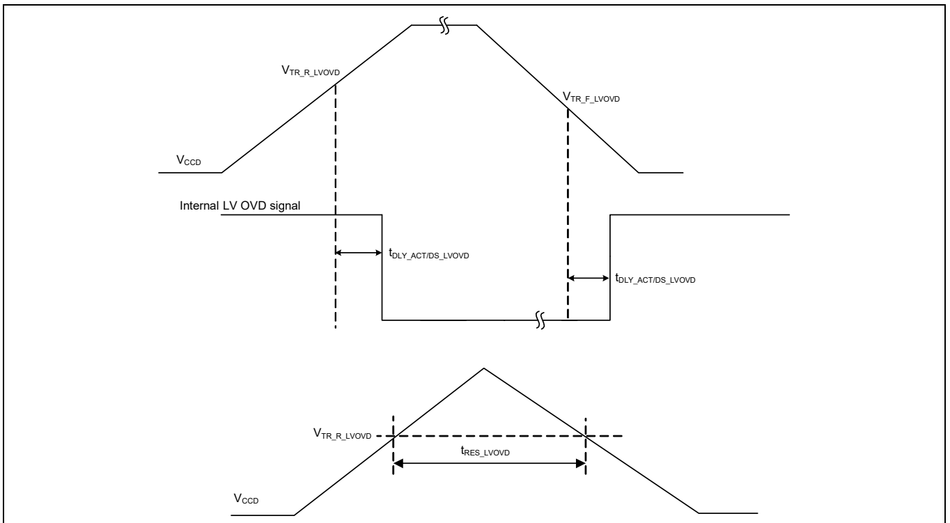
Figure 33 Low-voltage OVD specifications
