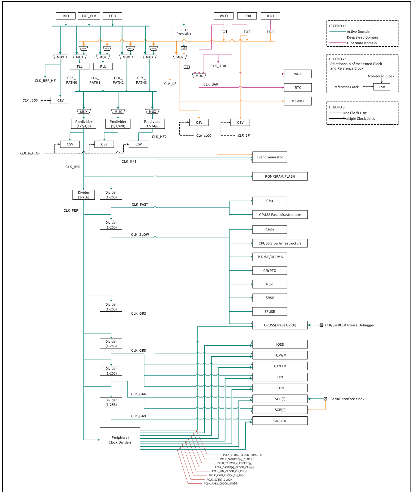
Figure 2 CYT2B9 clock diagram
