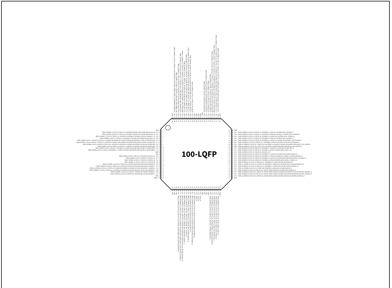
Figure 8 100-LQFP pin assignment with alternate functions
