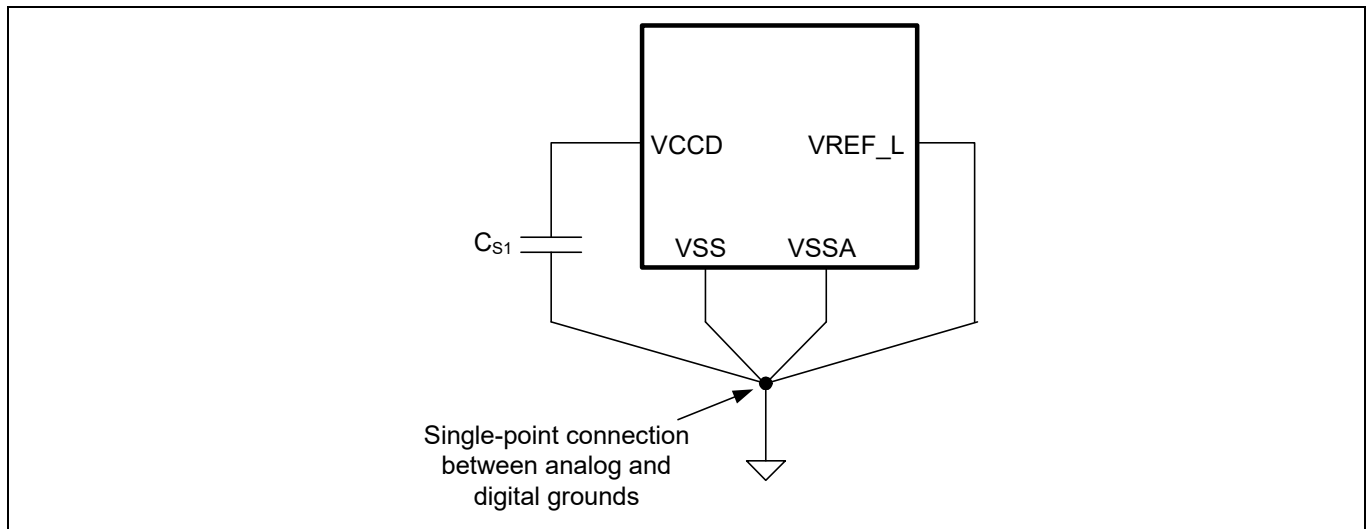
Figure 15 Smoothing capacitor
