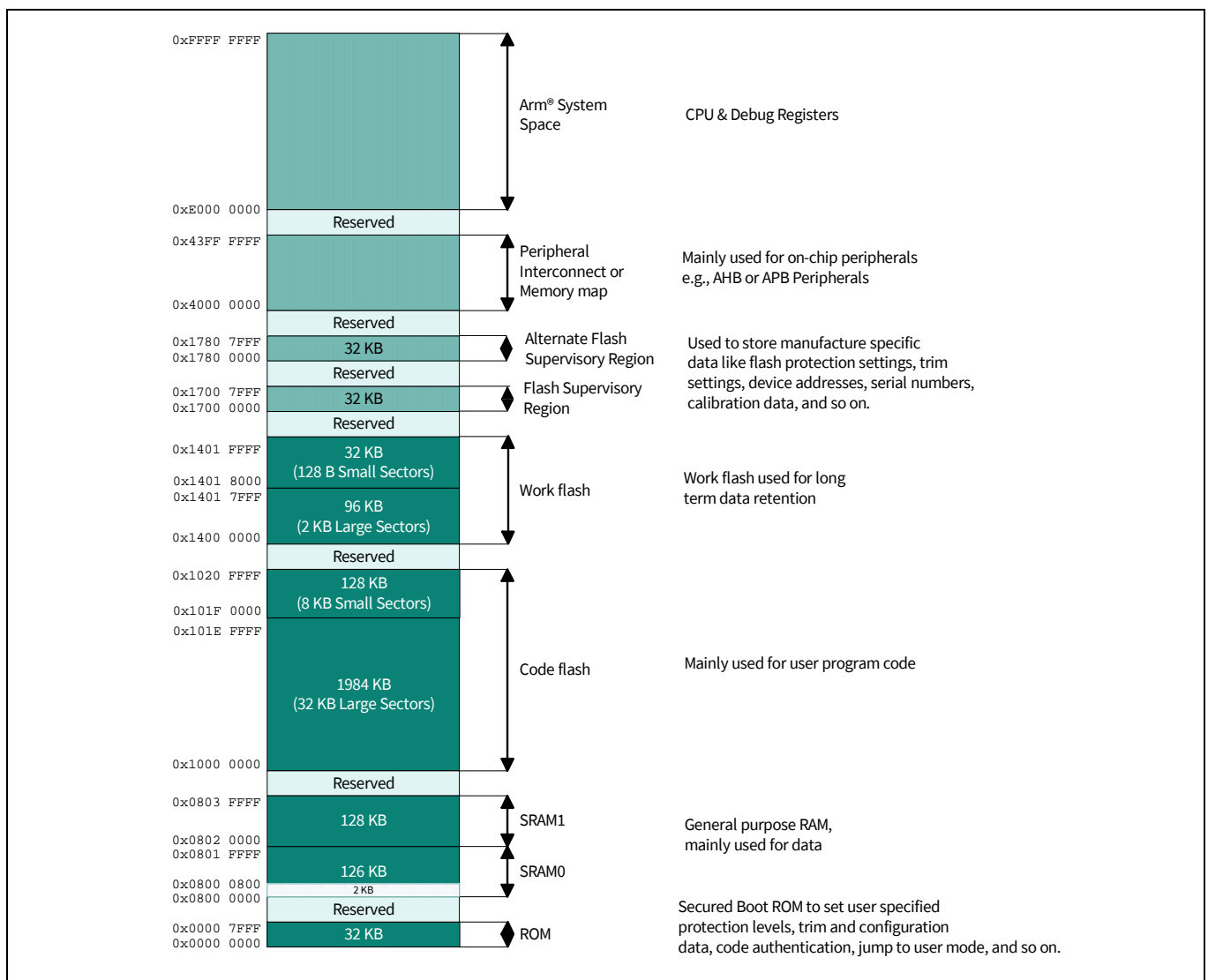
Figure 1 CYT2B9 address map [14, 15]
