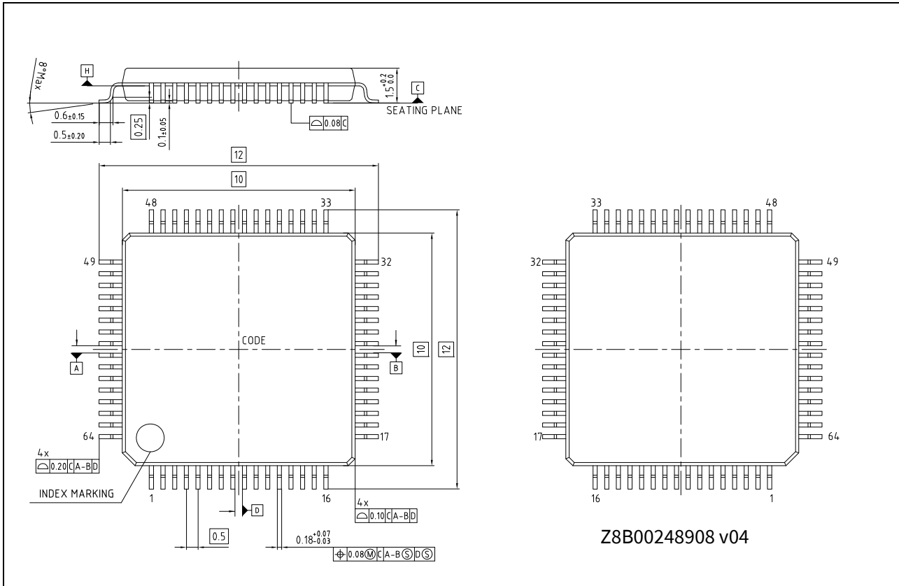
Figure 44 64-LQFP package outline (PG-LQFP-64)
