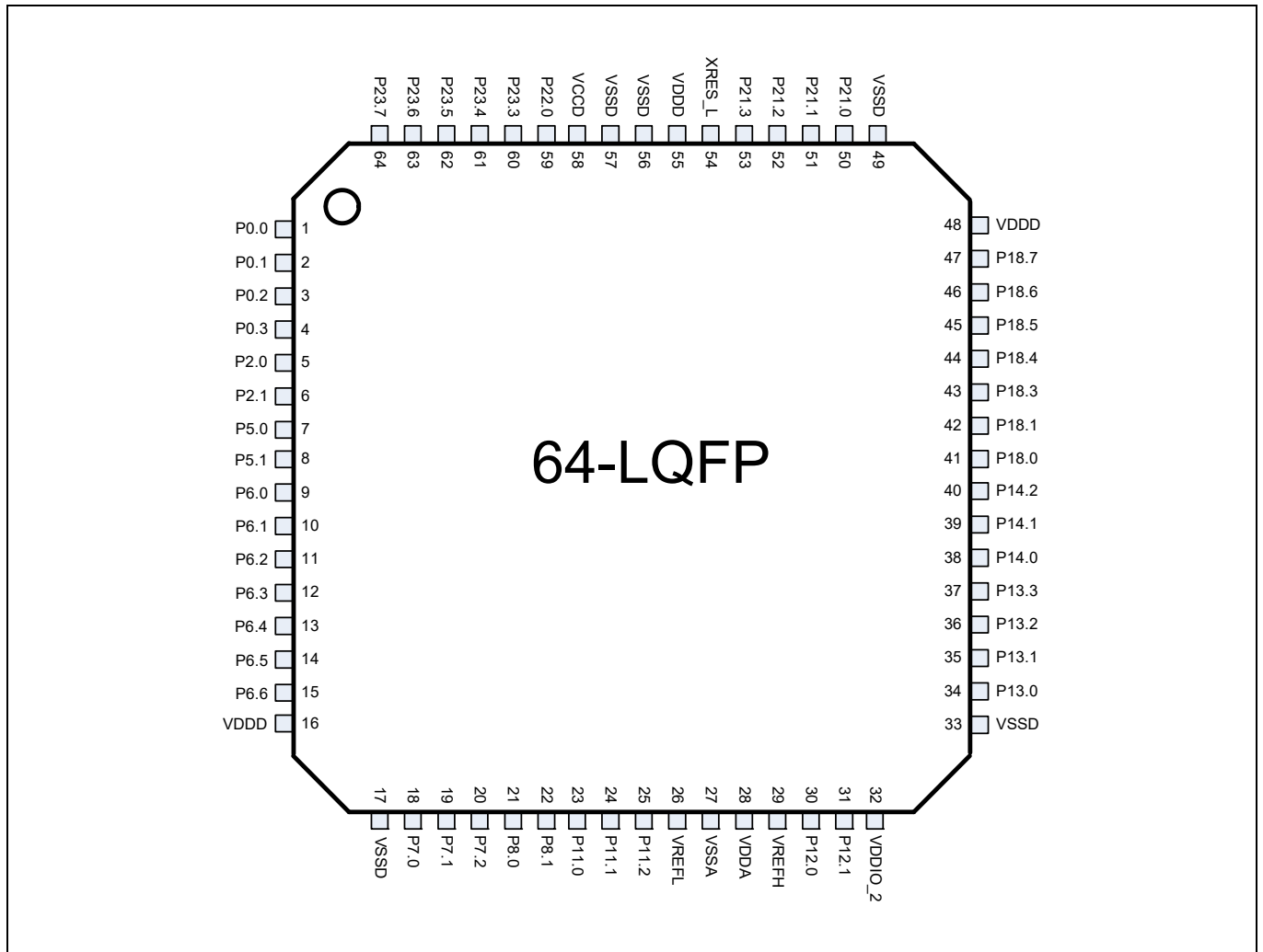
Figure 11 64-LQFP pin assignment
