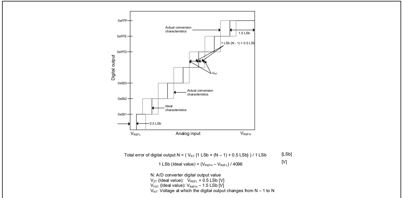
Figure 17 ADC characteristics and error definitions
