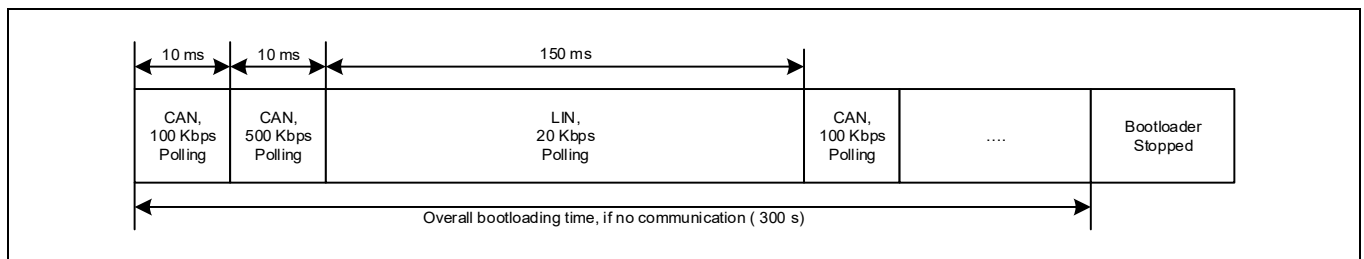
Figure 45 Bootloading sequence
