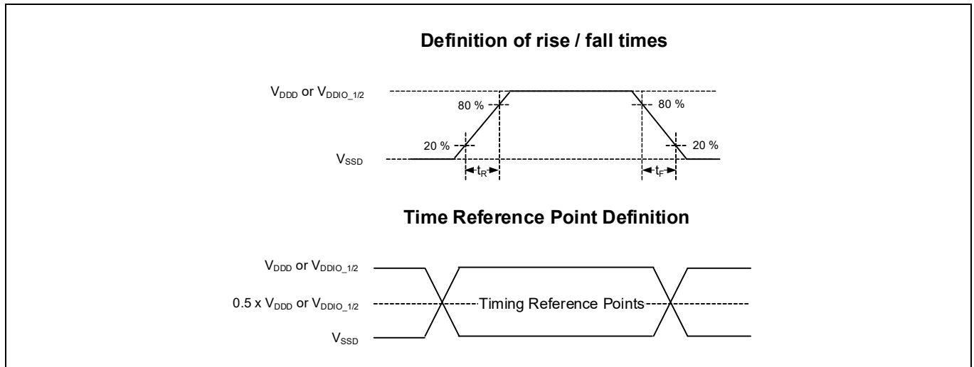
Figure 20 AC timings specifications
