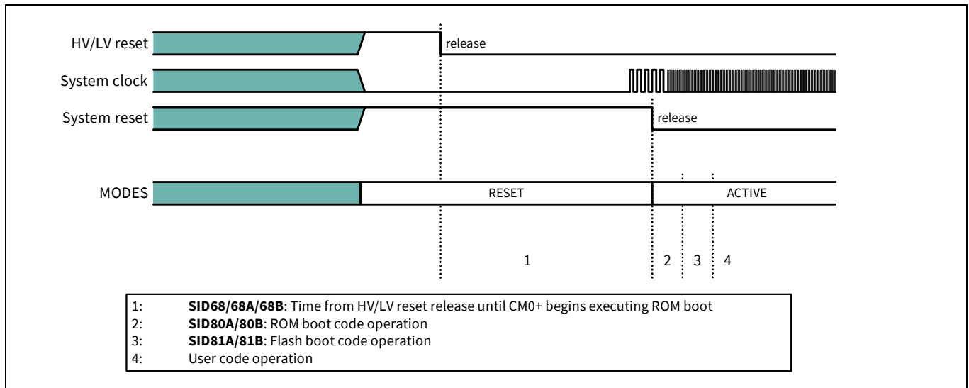
Figure 16 Reset sequence
