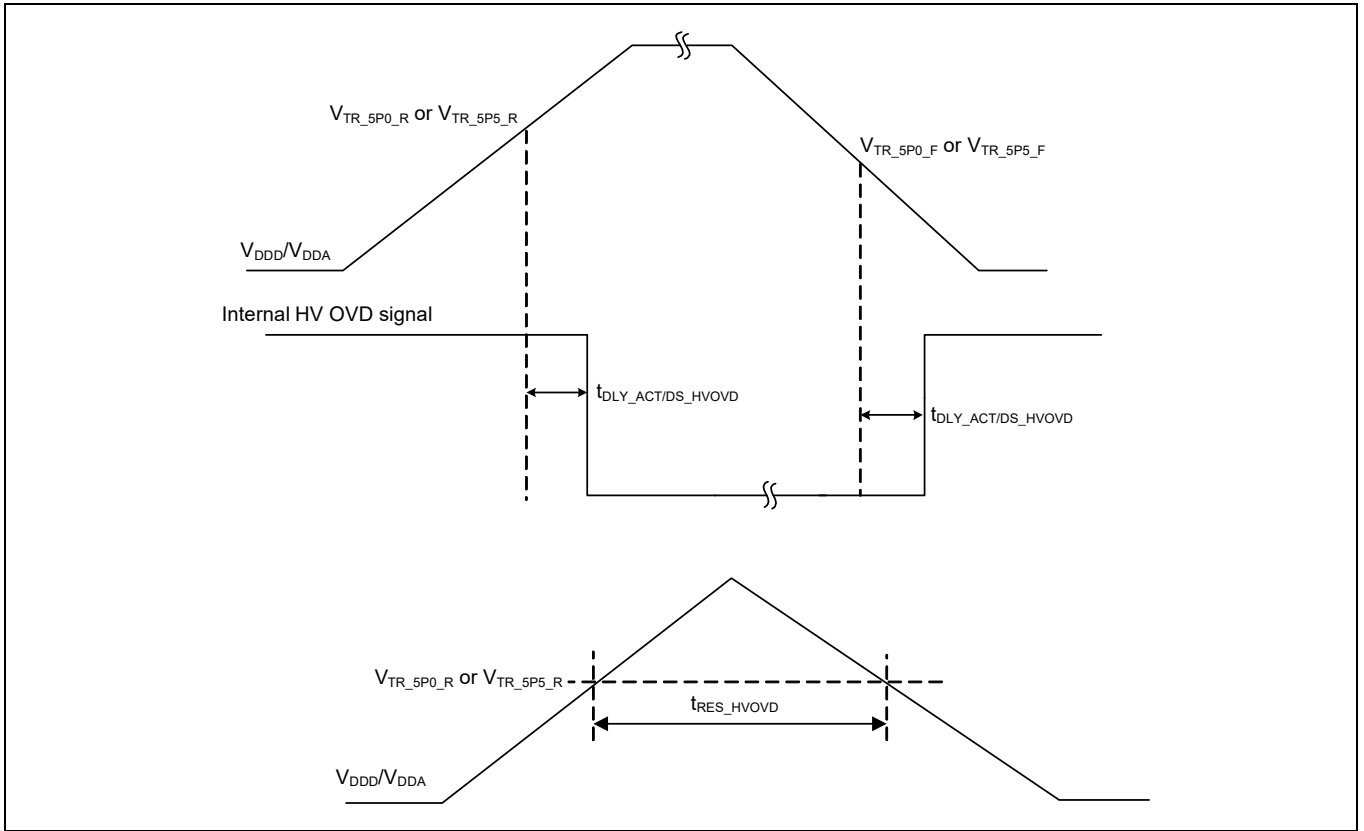
Figure 32 High-voltage OVD specifications
