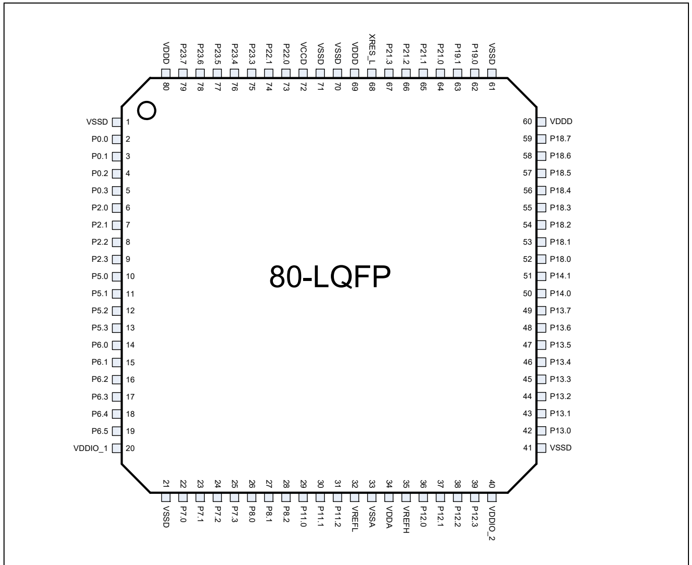
Figure 9 80-LQFP pin assignment
