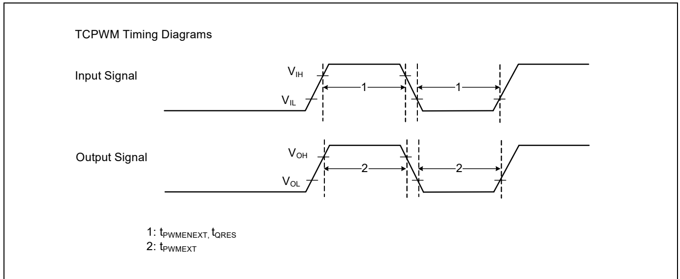
Figure 21 TCPWM timing diagrams
