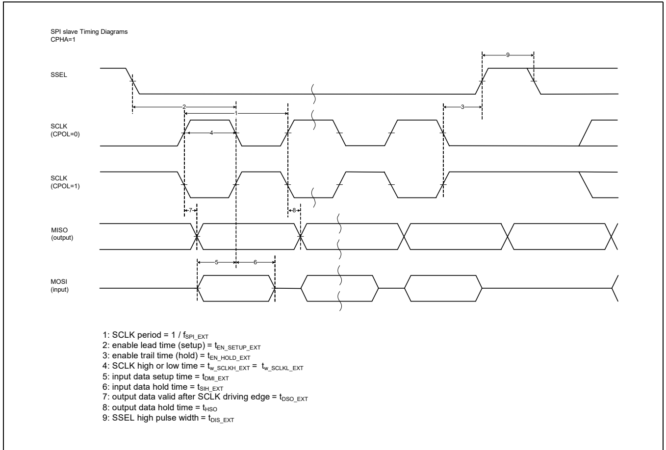
Figure 26 SPI slave timing diagrams with HIGH clock phase
