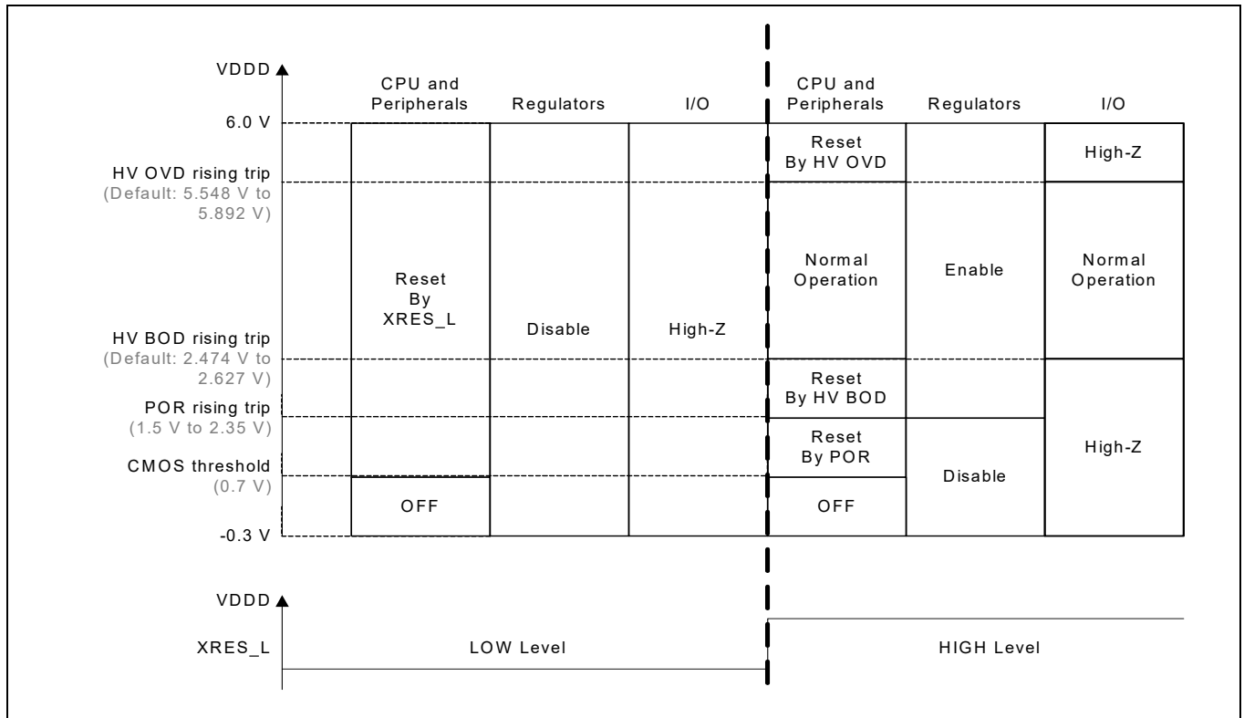
Figure 28 Device operations supply range, and relationship to XRES_L levels
