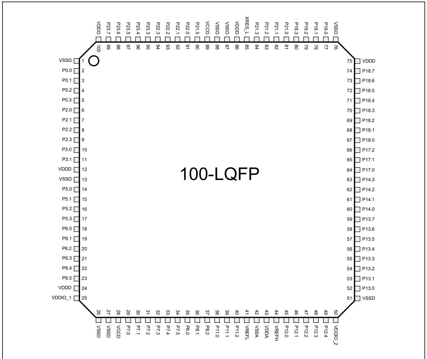
Figure 7 100-LQFP pin assignment
