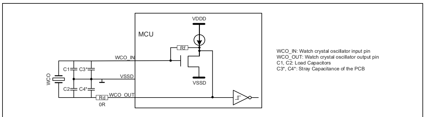
Figure 37 WCO connection scheme [62]
