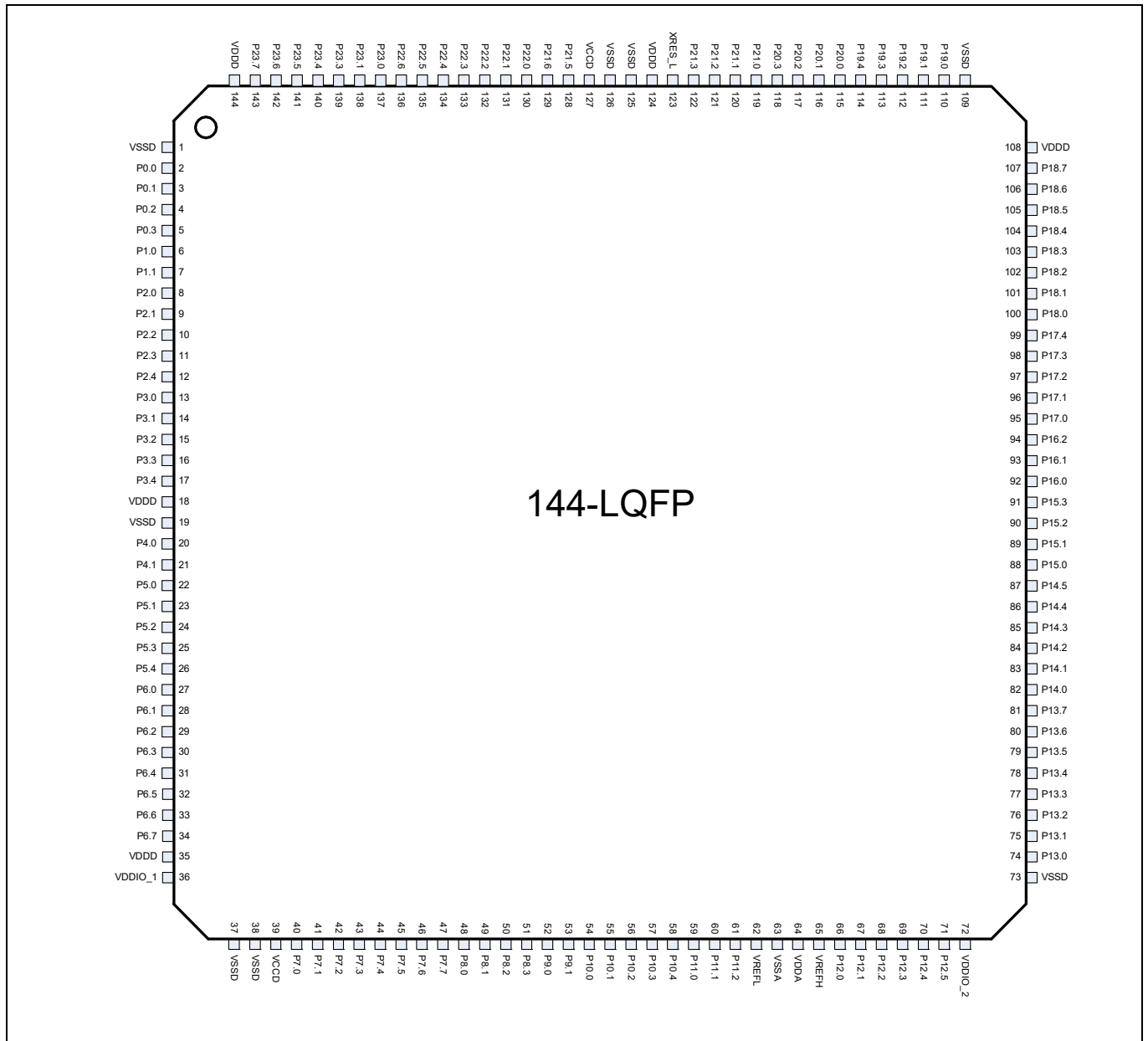
Figure 5 144-LQFP pin assignment
