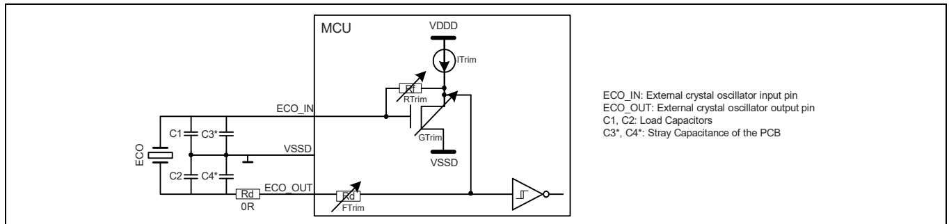
Figure 36 ECO connection scheme [60]
