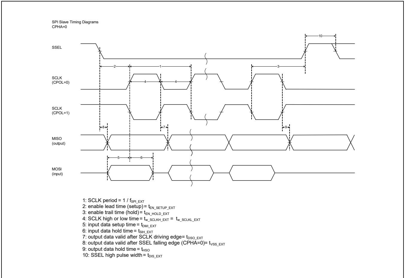
Figure 25 SPI slave timing diagrams with LOW clock phase
