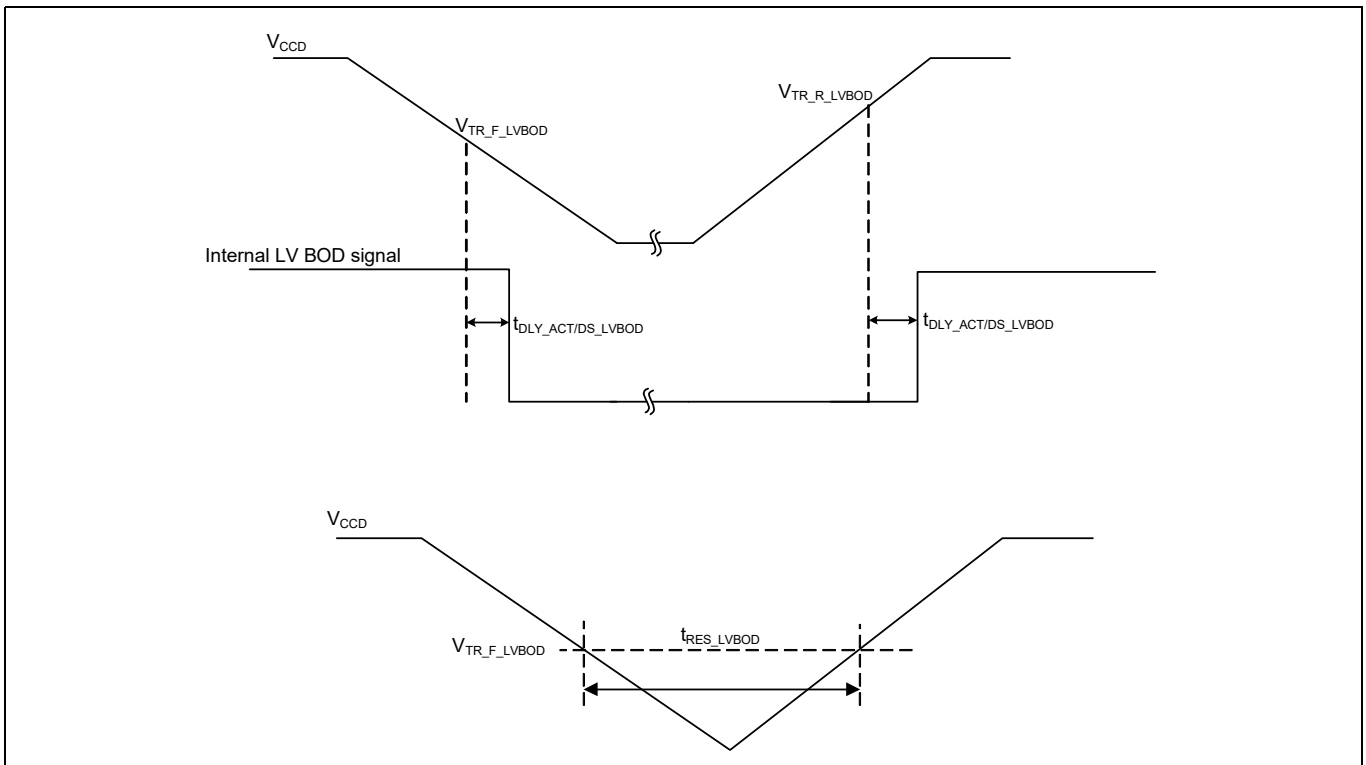
Figure 31 Low-Voltage BOD specifications
