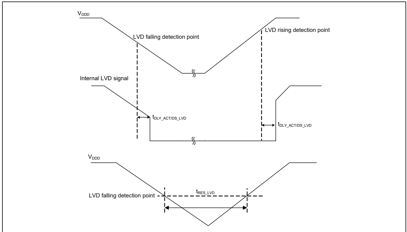
Figure 34 LVD specifications
