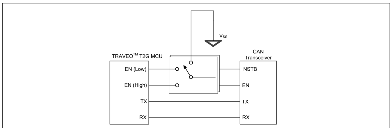
Figure 46 MCU to CAN transceiver connections
