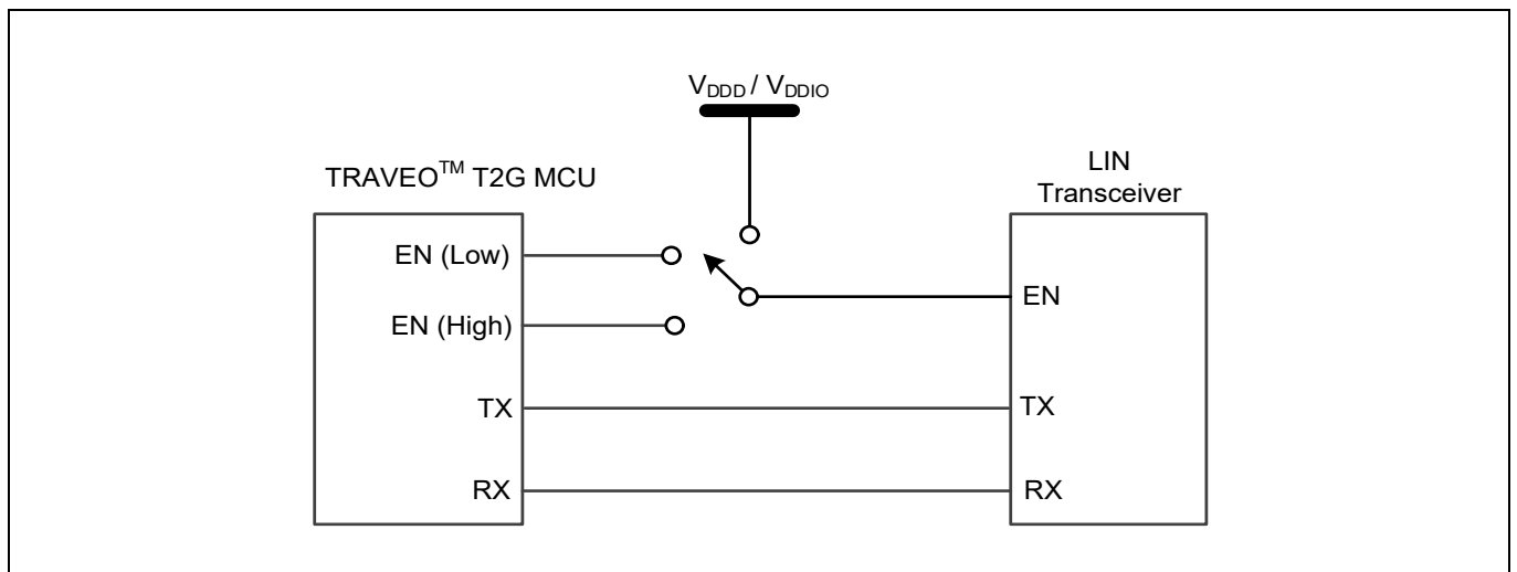
Figure 47 MCU to LIN transceiver connections
