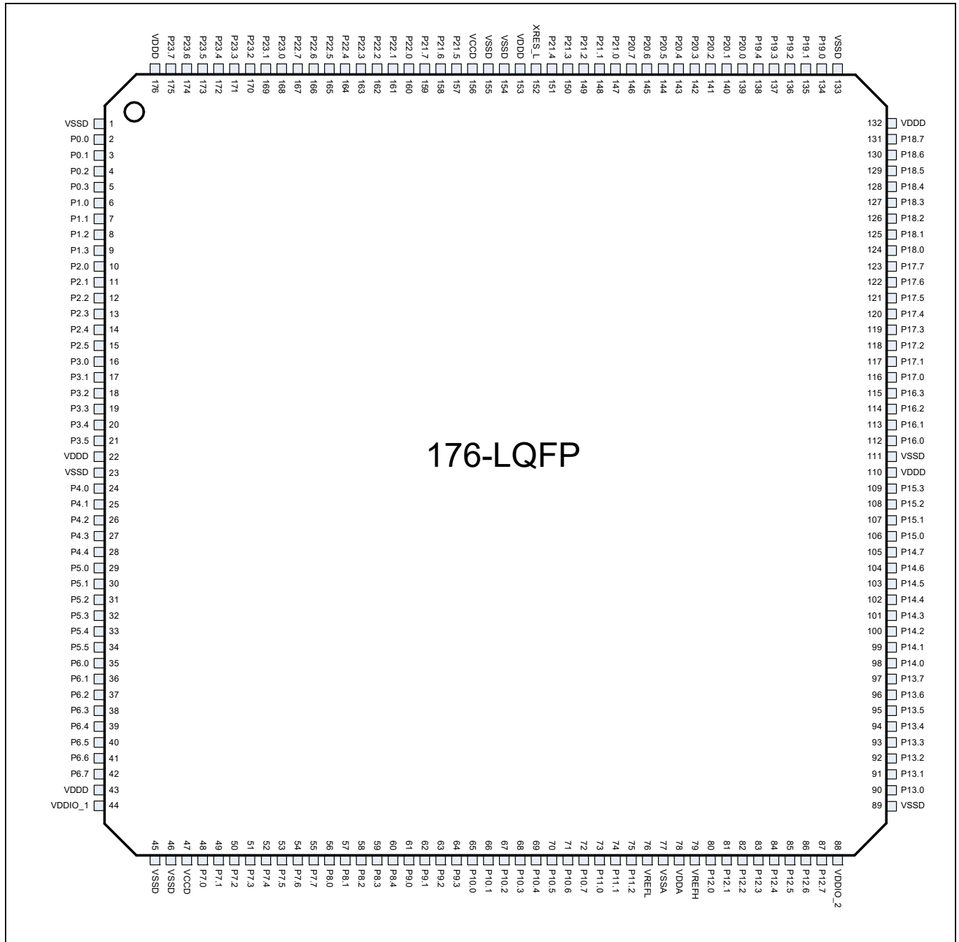
Figure 3 176-LQFP pin assignment
