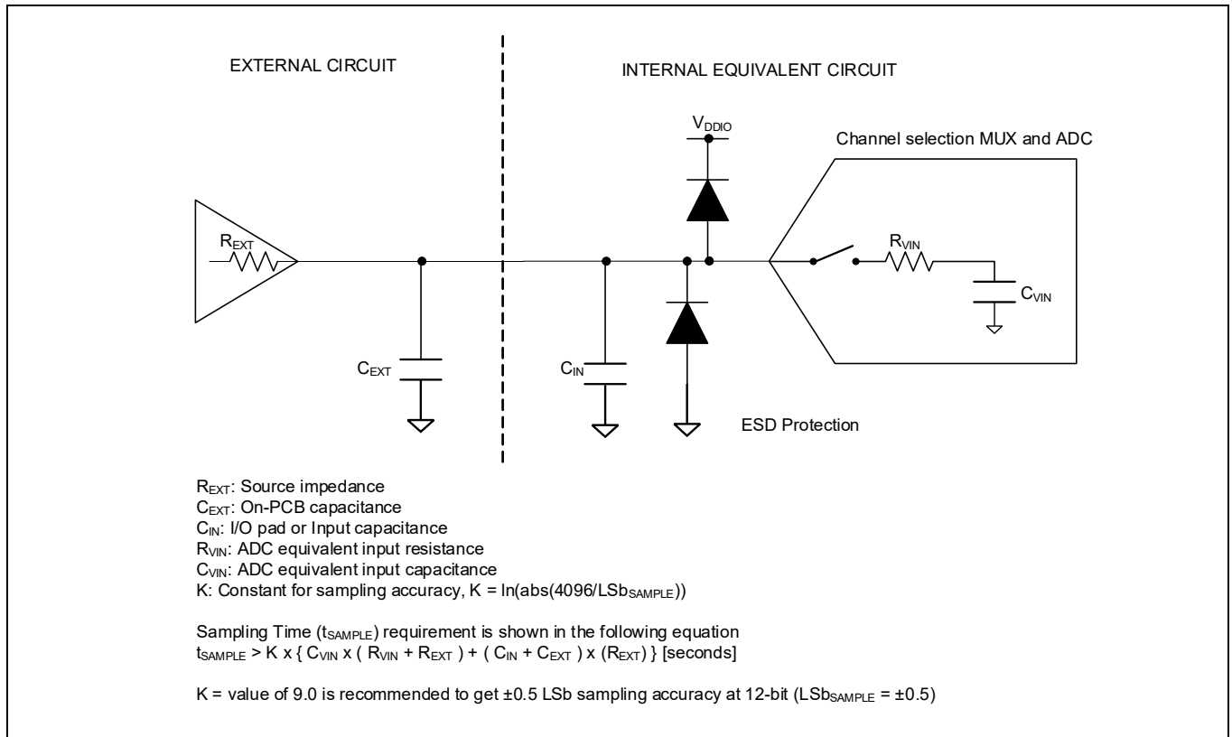
Figure 19 ADC equivalent circuit for analog input
