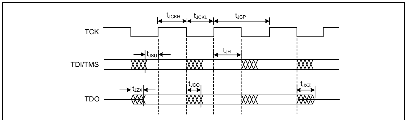
Figure 35 JTAG specifications
