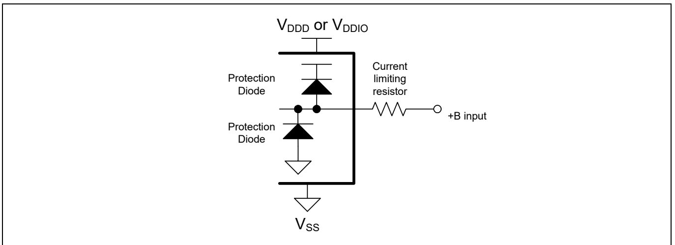
Figure 14 Example of a recommended circuit [44]
