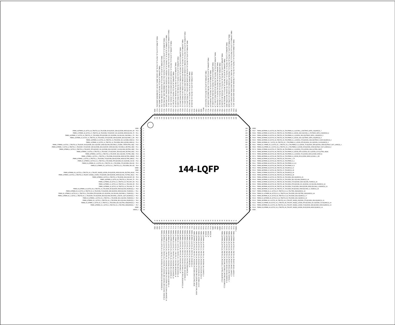
Figure 7 144-LQFP pin assignment with alternate functions
