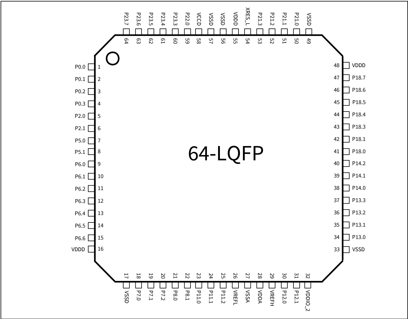
Figure 7 64-LQFP pin assignment
