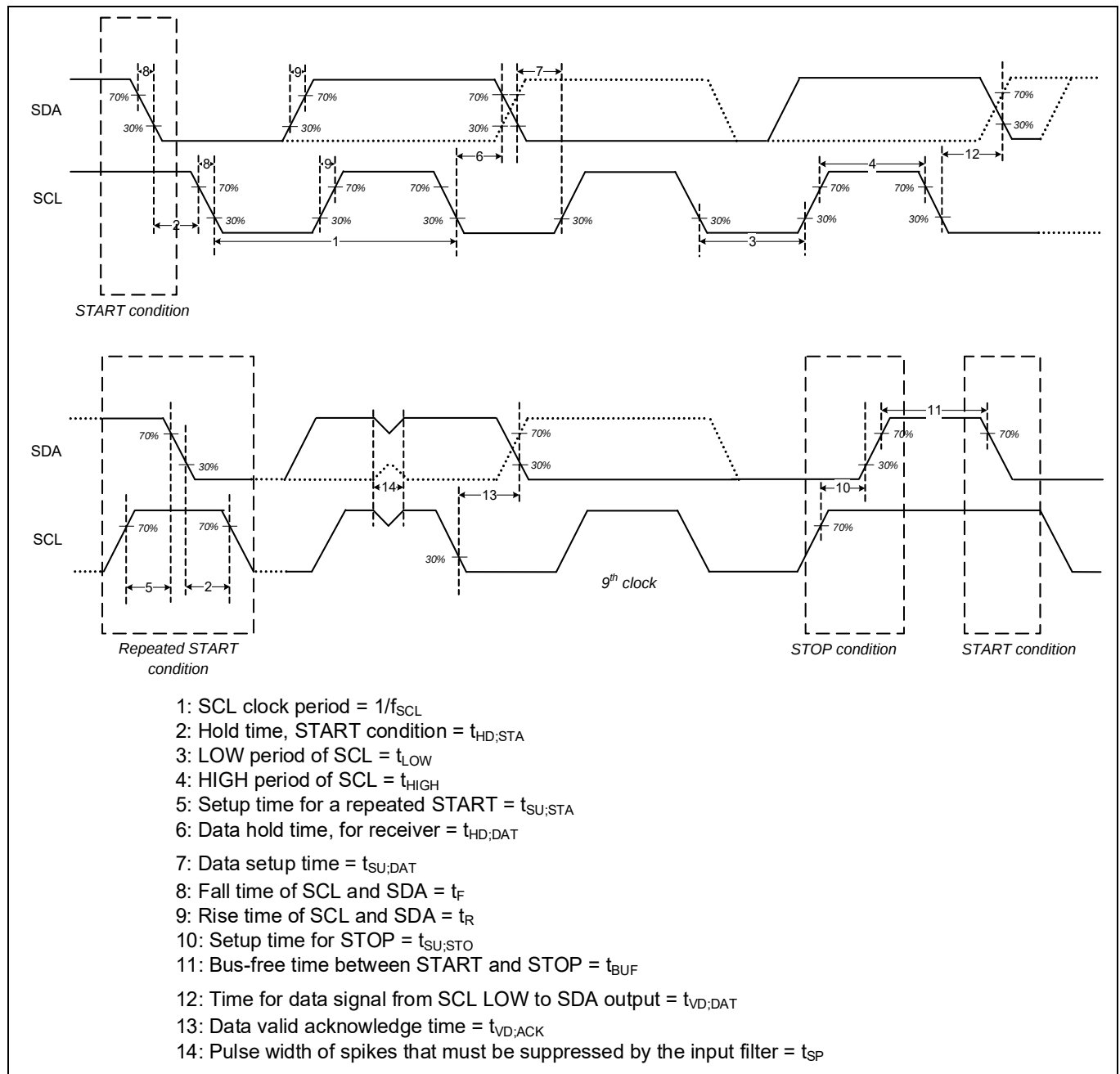
Figure 18 I 2 C timing diagrams
