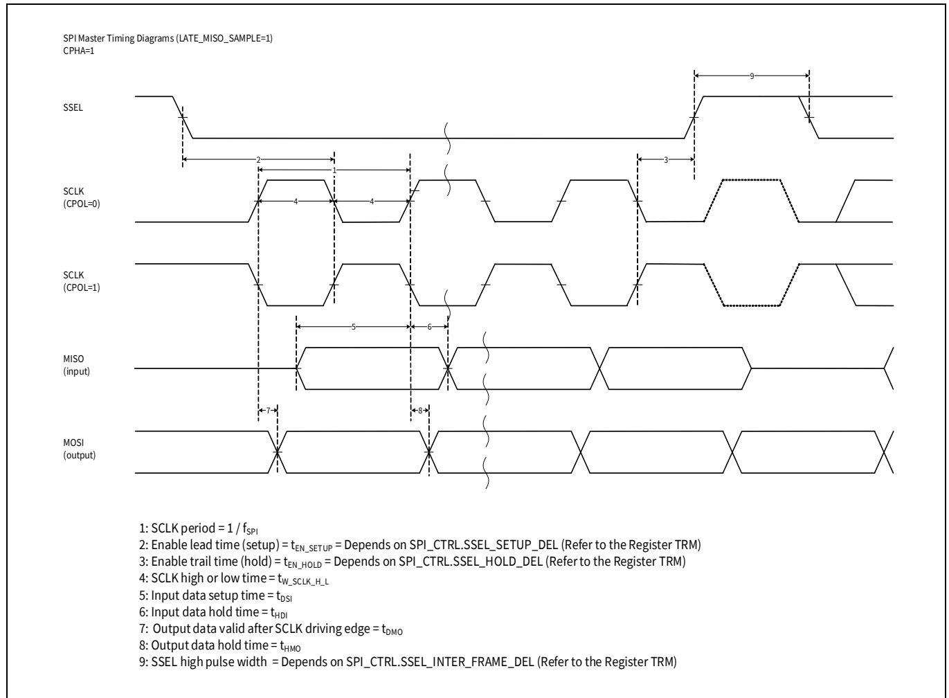
Figure 20 SPI master timing diagrams with HIGH clock phase
