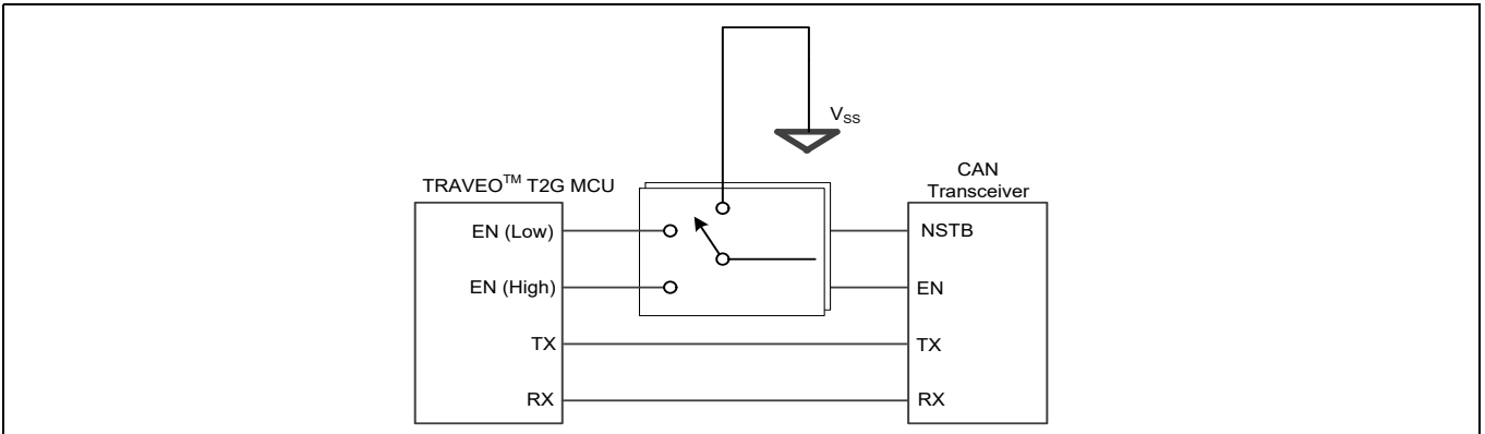
Figure 39 MCU to CAN transceiver connections
