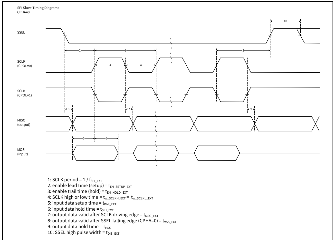
Figure 21 SPI slave timing diagrams with LOW clock phase
