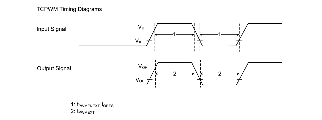
Figure 17 TCPWM timing diagrams
