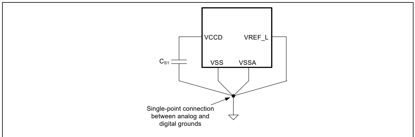
Figure 11 Smoothing capacitor
