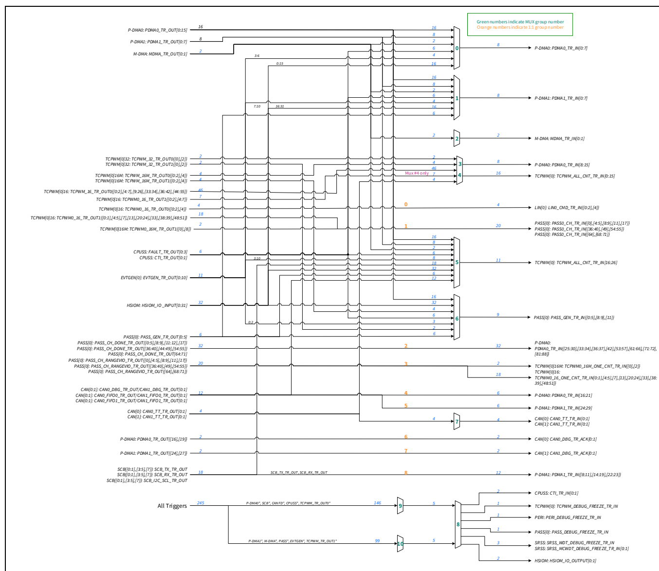
Figure 9 Trigger multiplexer [30]
