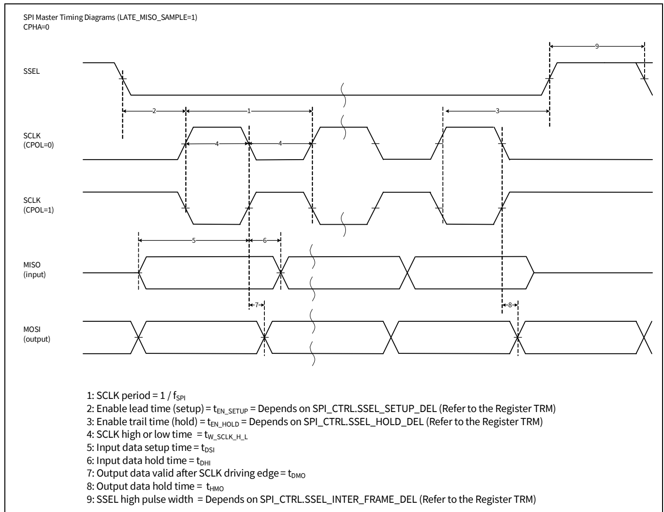
Figure 19 SPI master timing diagrams with LOW clock phase
