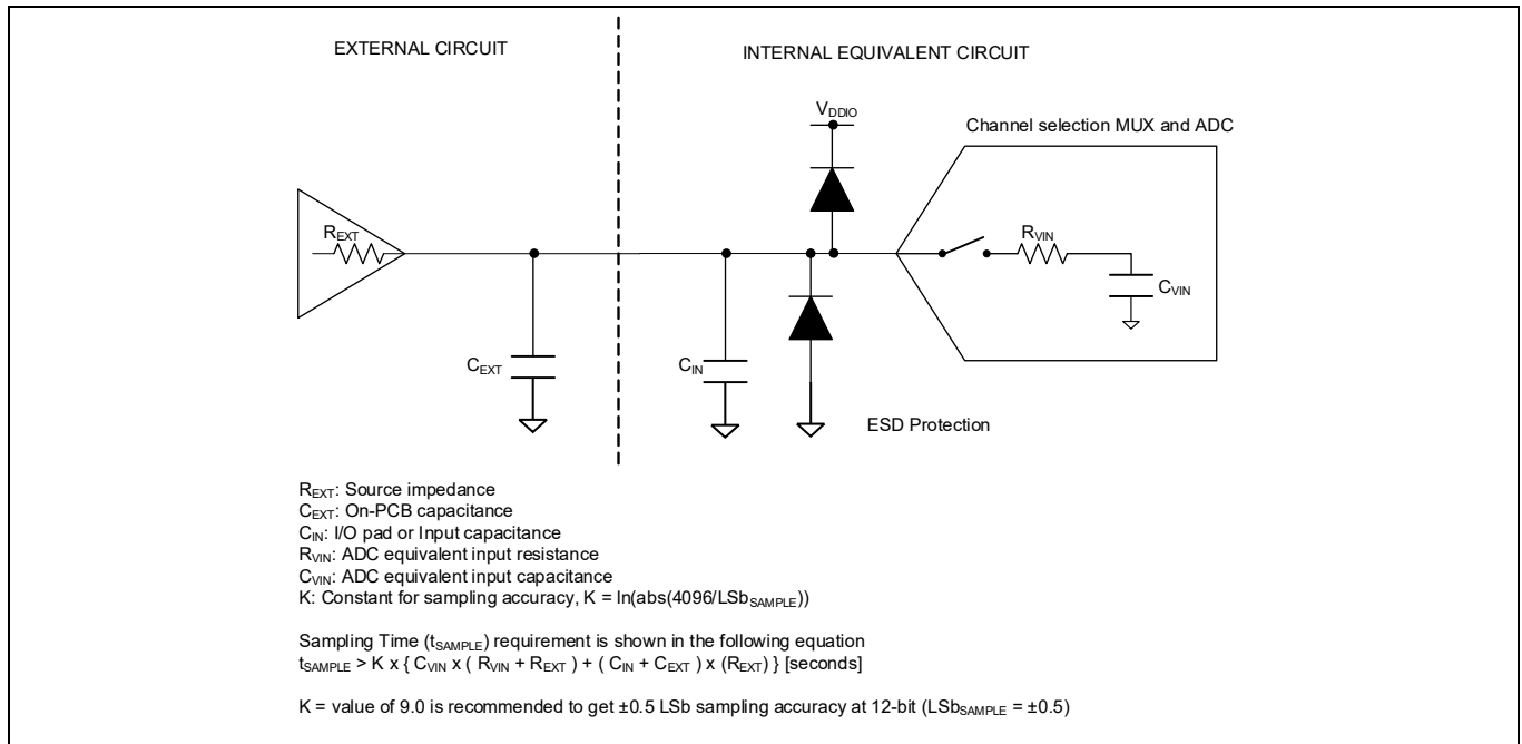
Figure 15 ADC equivalent circuit for analog input
