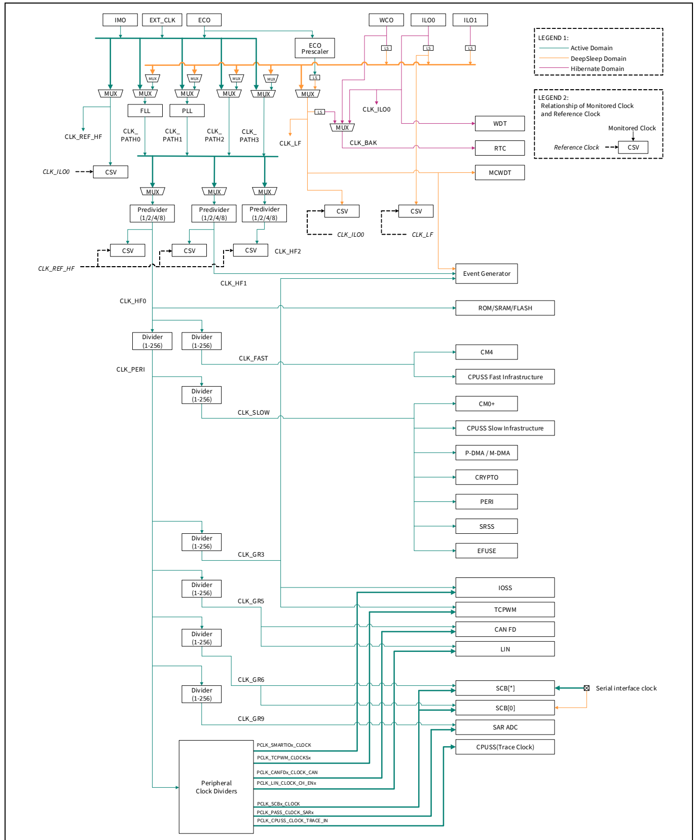
Figure 2 CYT2B6 clock diagram
