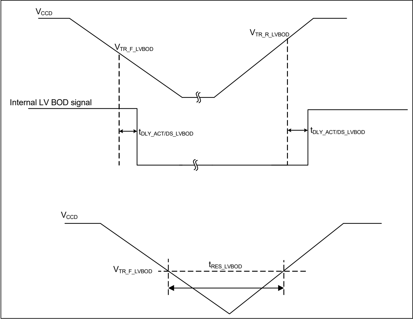
Figure 26 Low-voltage BOD specifications
