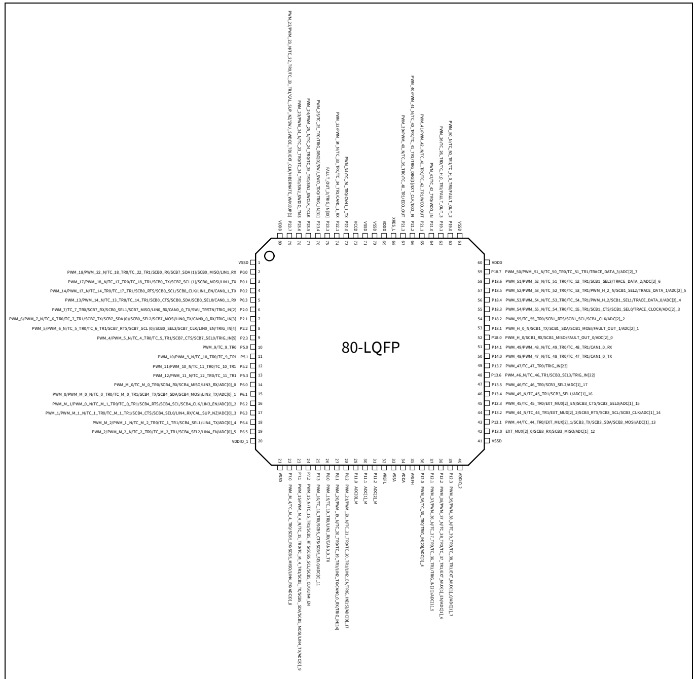
Figure 6 80-LQFP pin assignment with alternate functions
