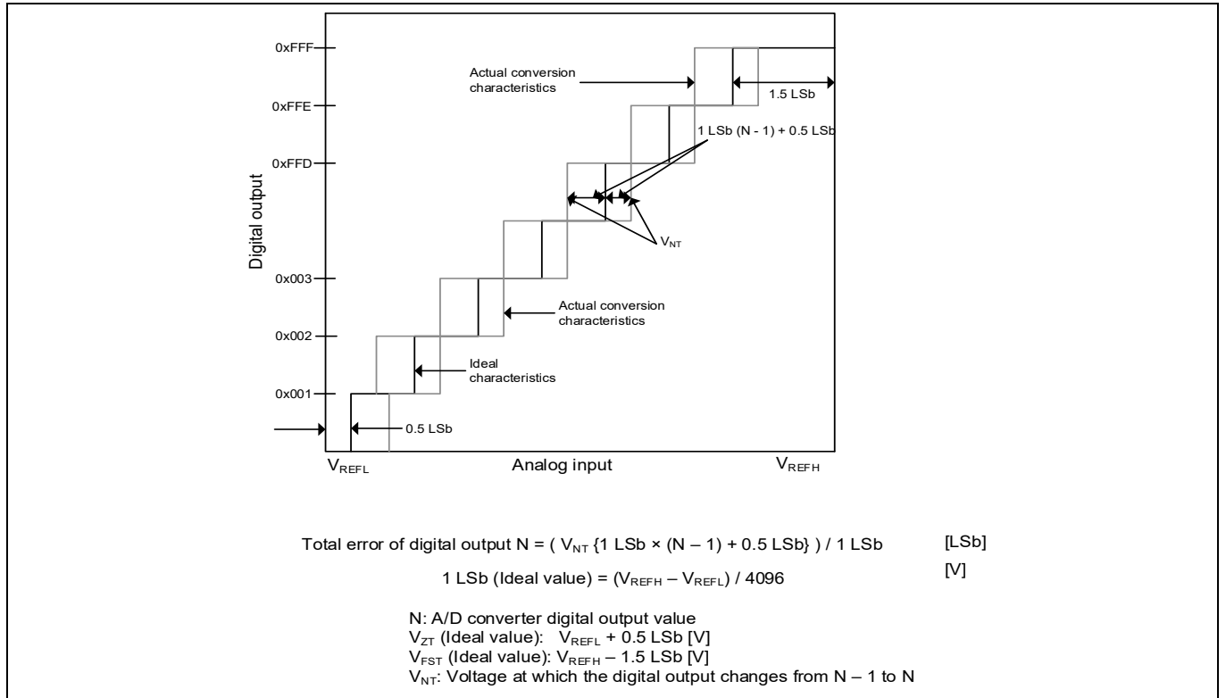
Figure 13 ADC characteristics and error definitions
