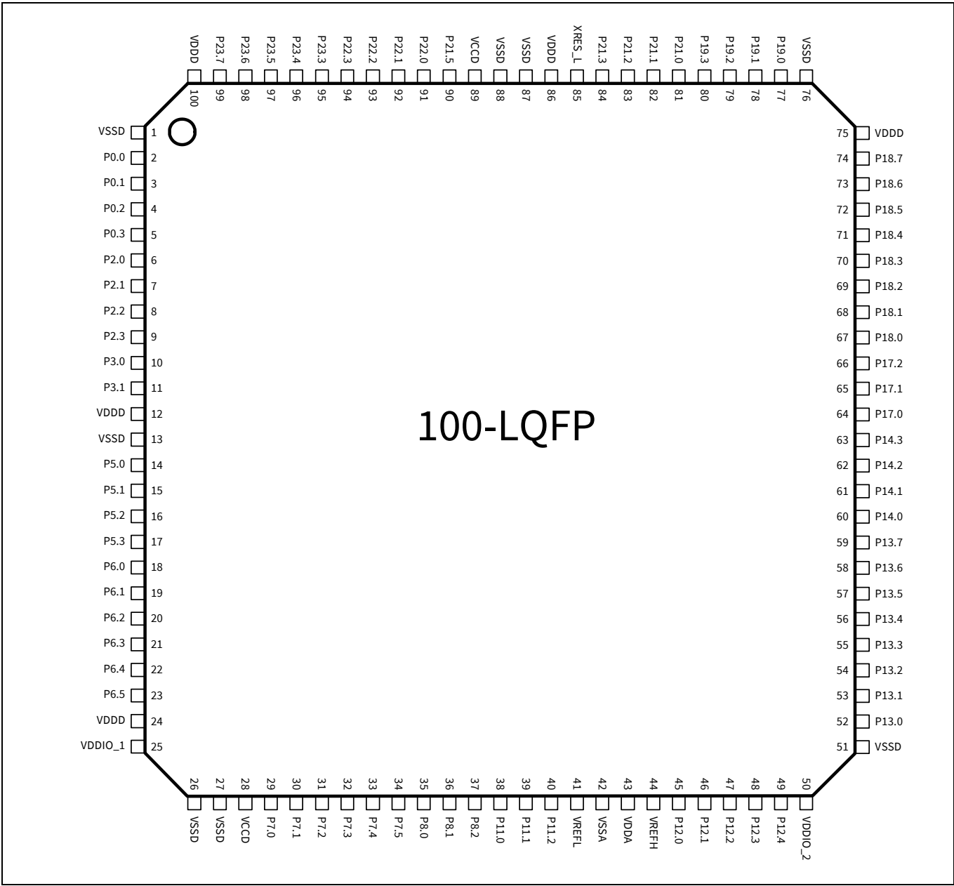
Figure 3 100-LQFP pin assignment
