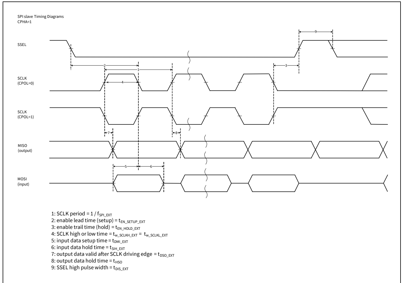
Figure 22 SPI slave timing diagrams with HIGH clock phase
