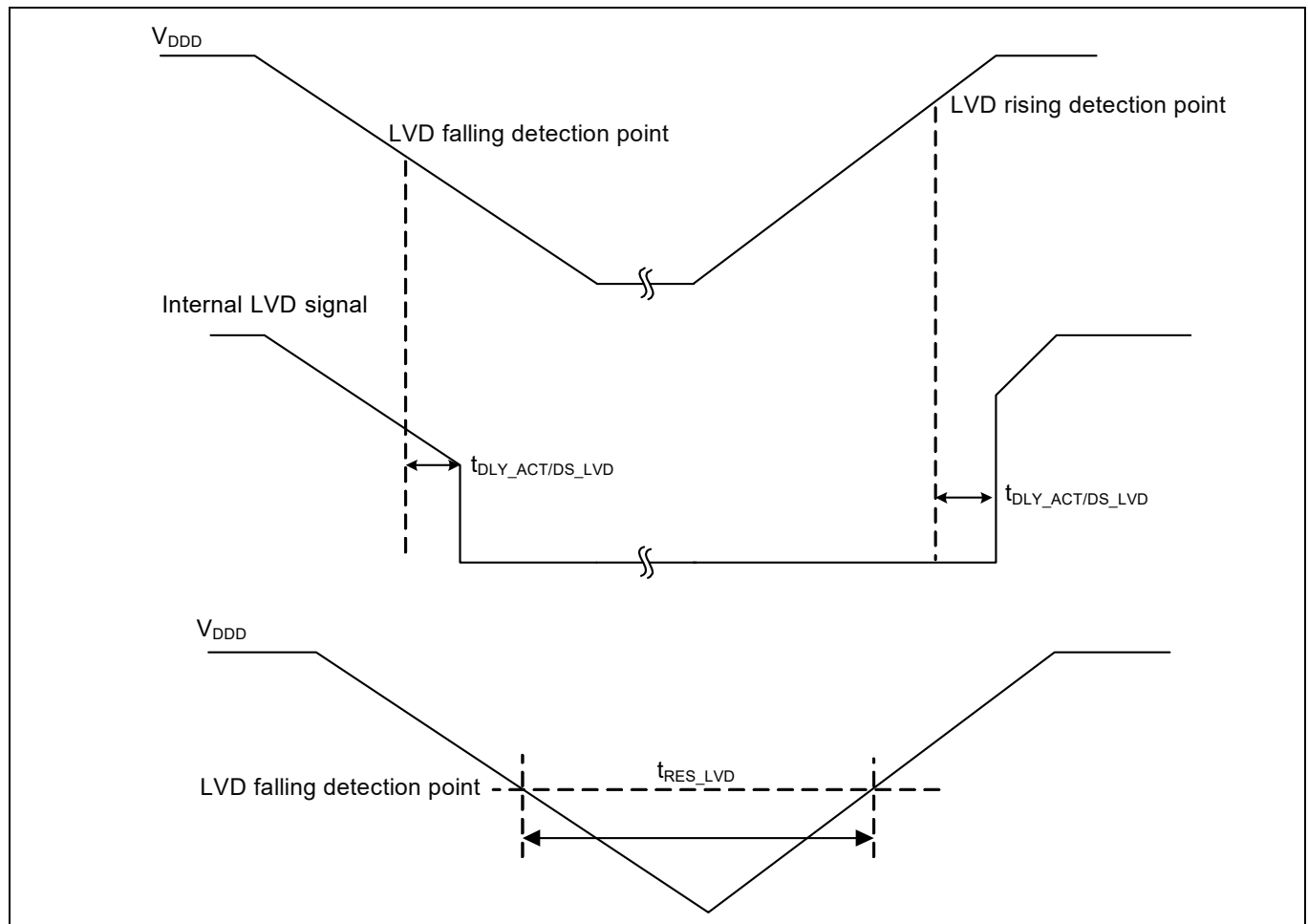
Figure 29 LVD specifications
