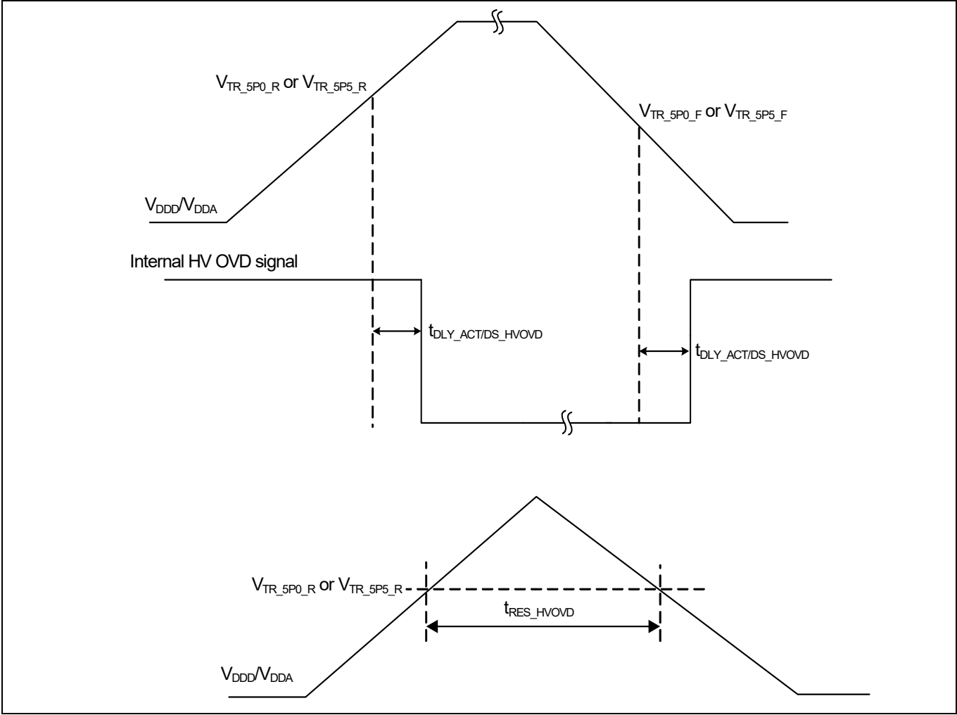
Figure 27 High-voltage OVD specifications
