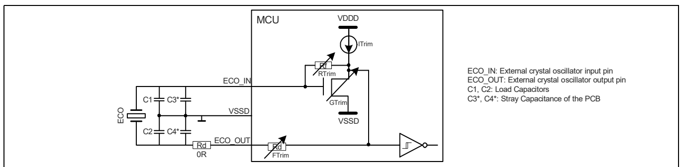
Figure 31 ECO connection scheme [58]
