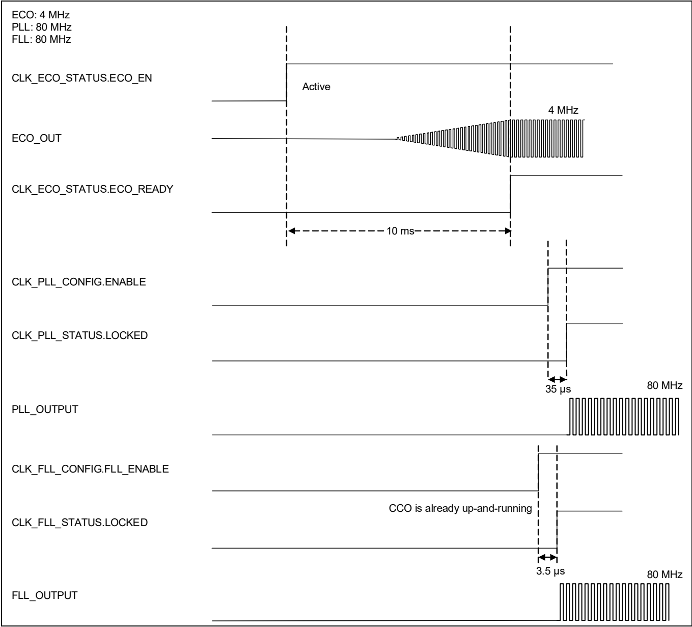
Figure 33 ECO to PLL or FLL diagram
