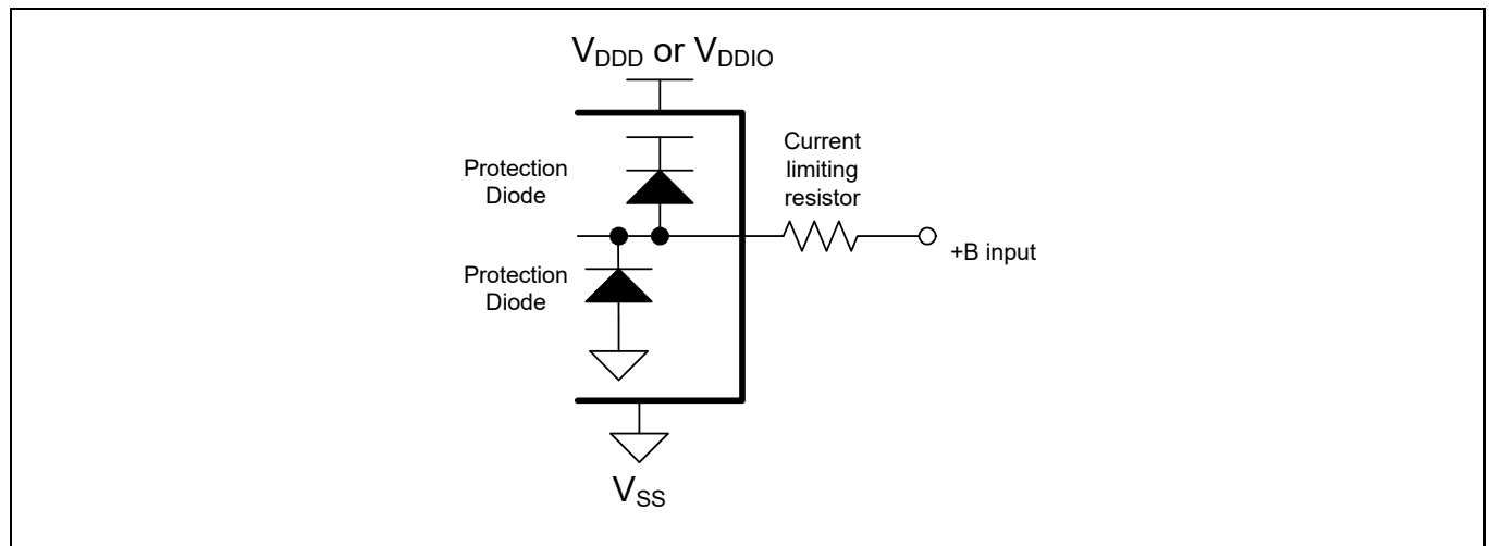
Figure 10 Example of a recommended circuit [43]
