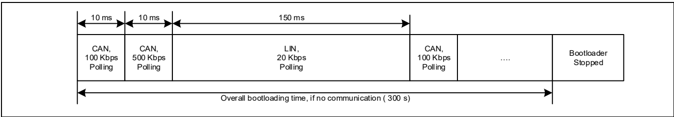
Figure 38 Bootloading sequence
