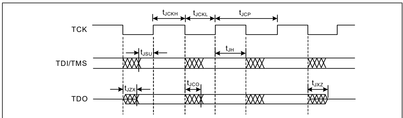
Figure 30 JTAG timing diagram
