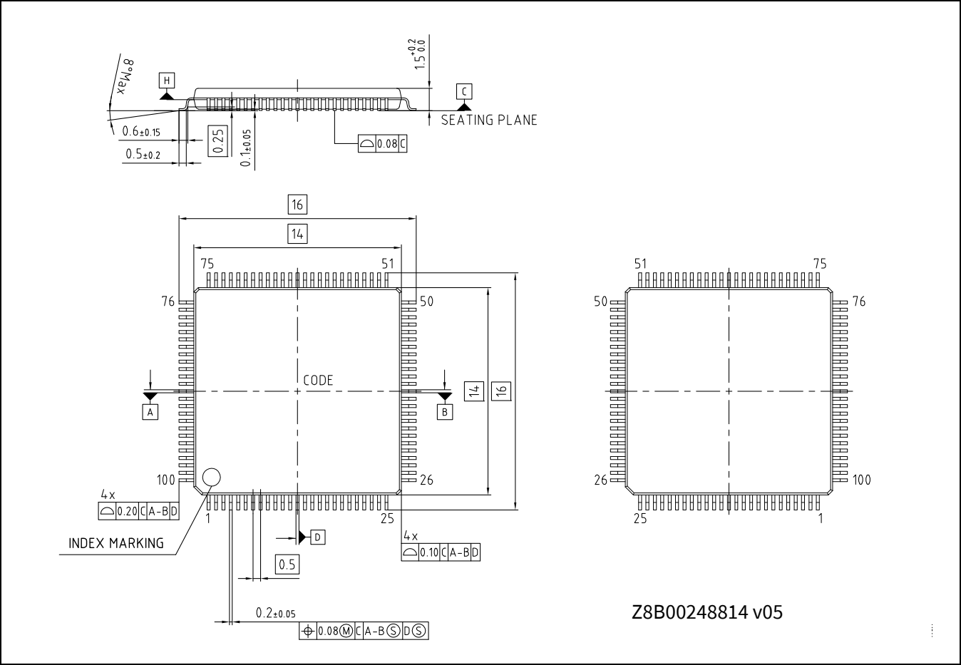
Figure 35 100-LQFP package outline (PG-LQFP-100)
