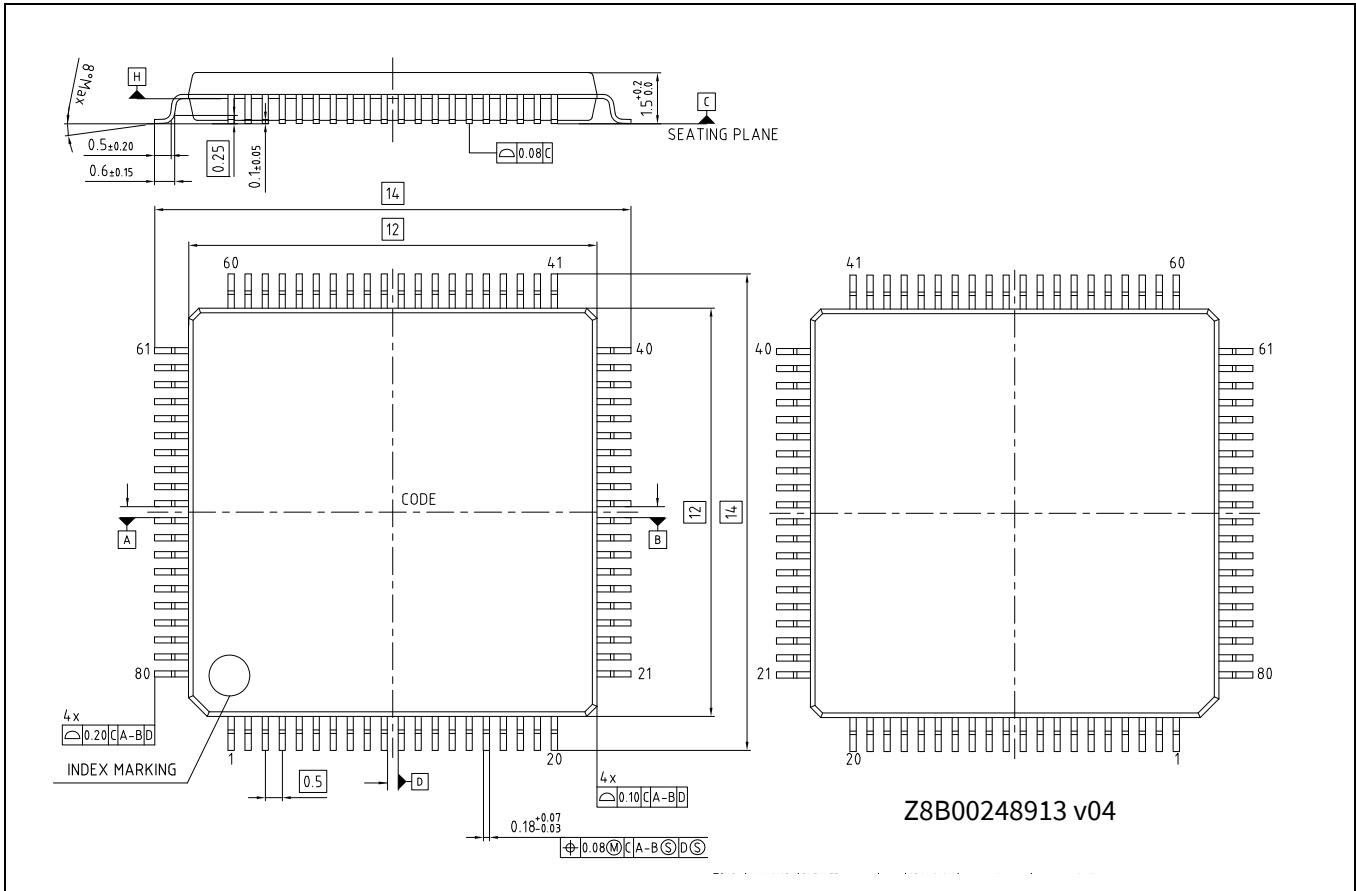
Figure 36 80-LQFP package outline (PG-LQFP-80)
