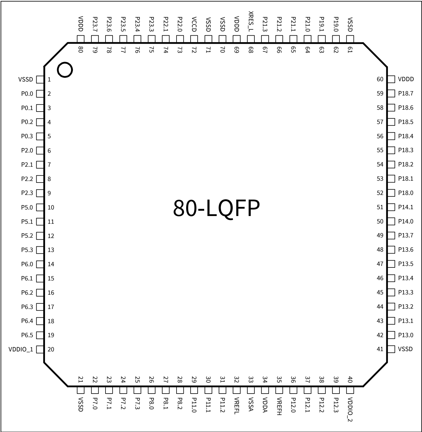
Figure 5 80-LQFP pin assignment
