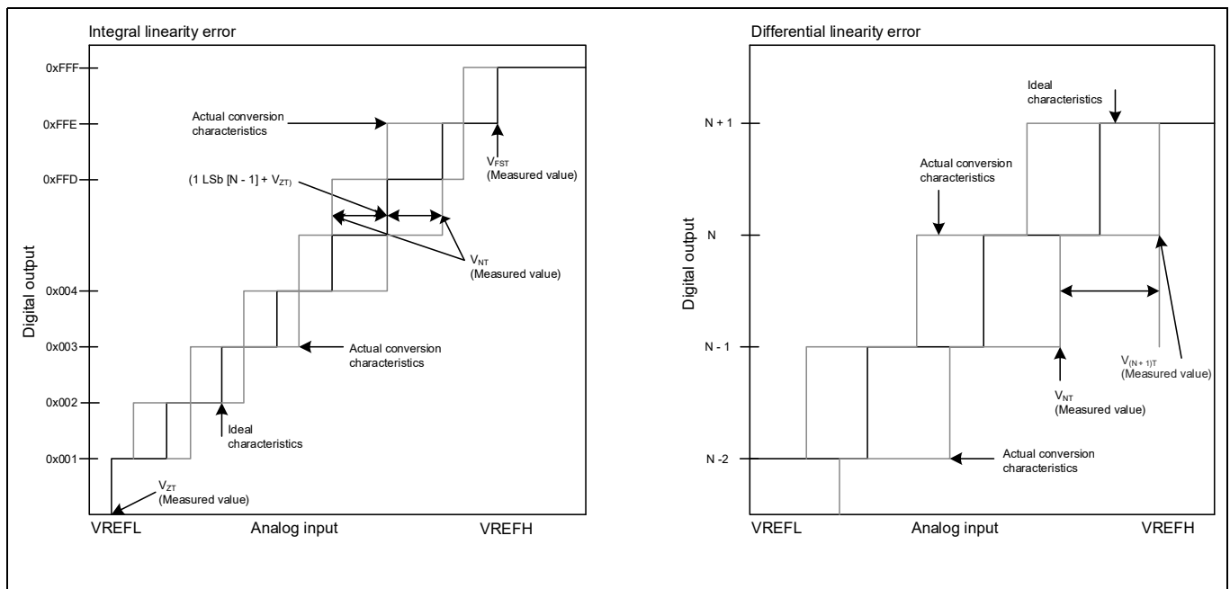
Figure 14 Integral and differential linearity errors
