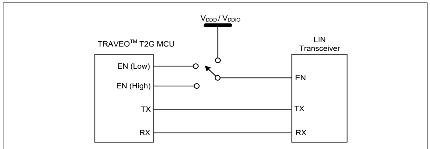
Figure 40 MCU to LIN transceiver connections
