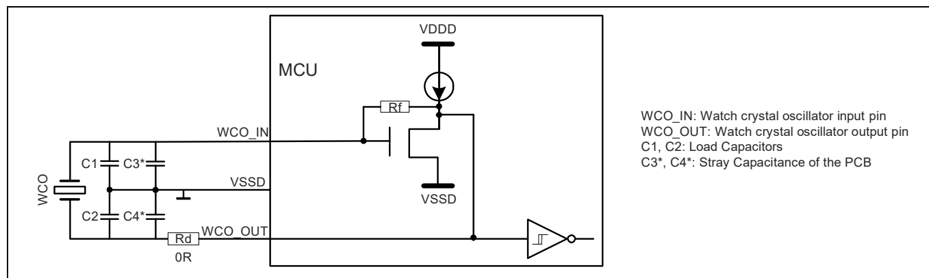
Figure 32 WCO connection scheme [60]
