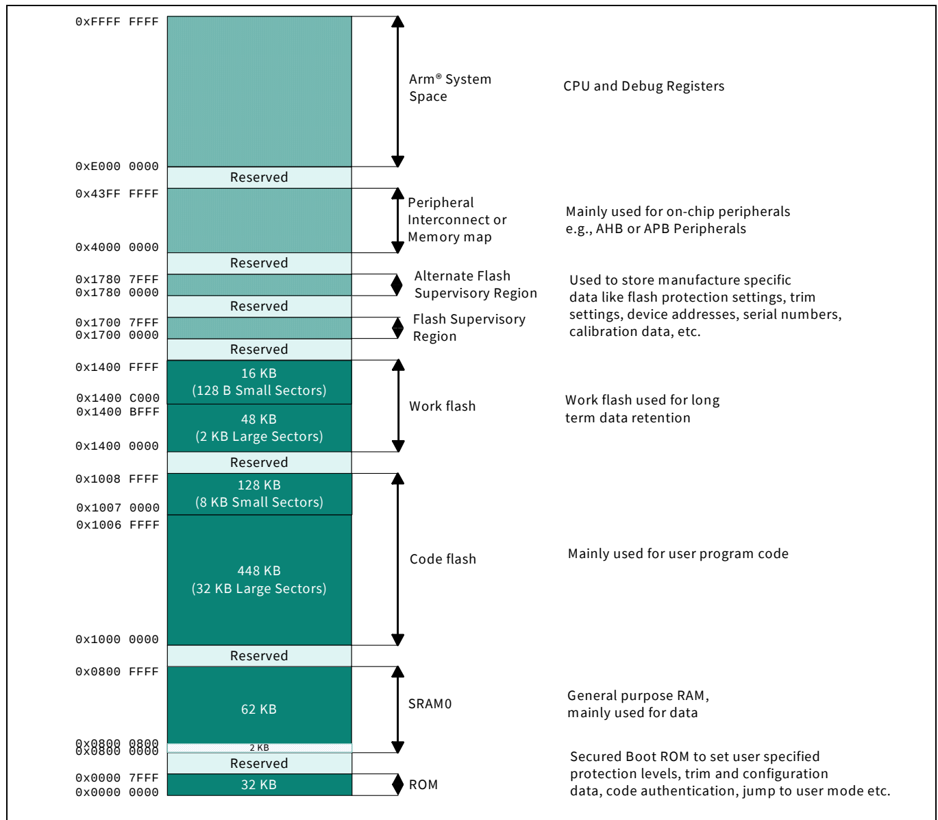
Figure 1 CYT2B6 address map [14, 15]
