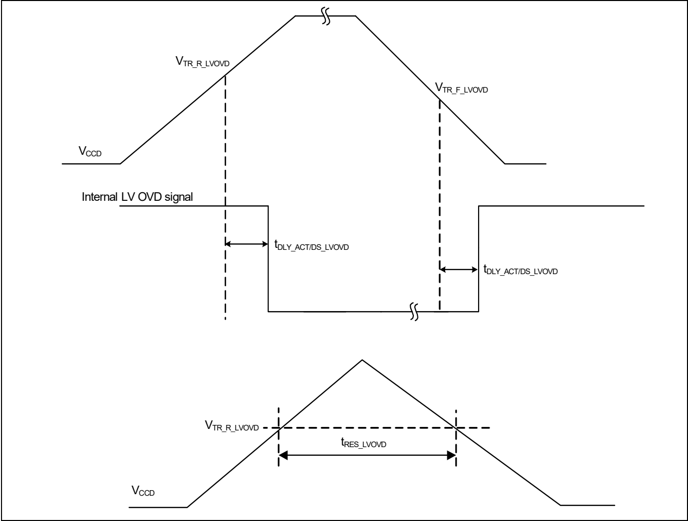
Figure 28 Low-voltage OVD specifications
