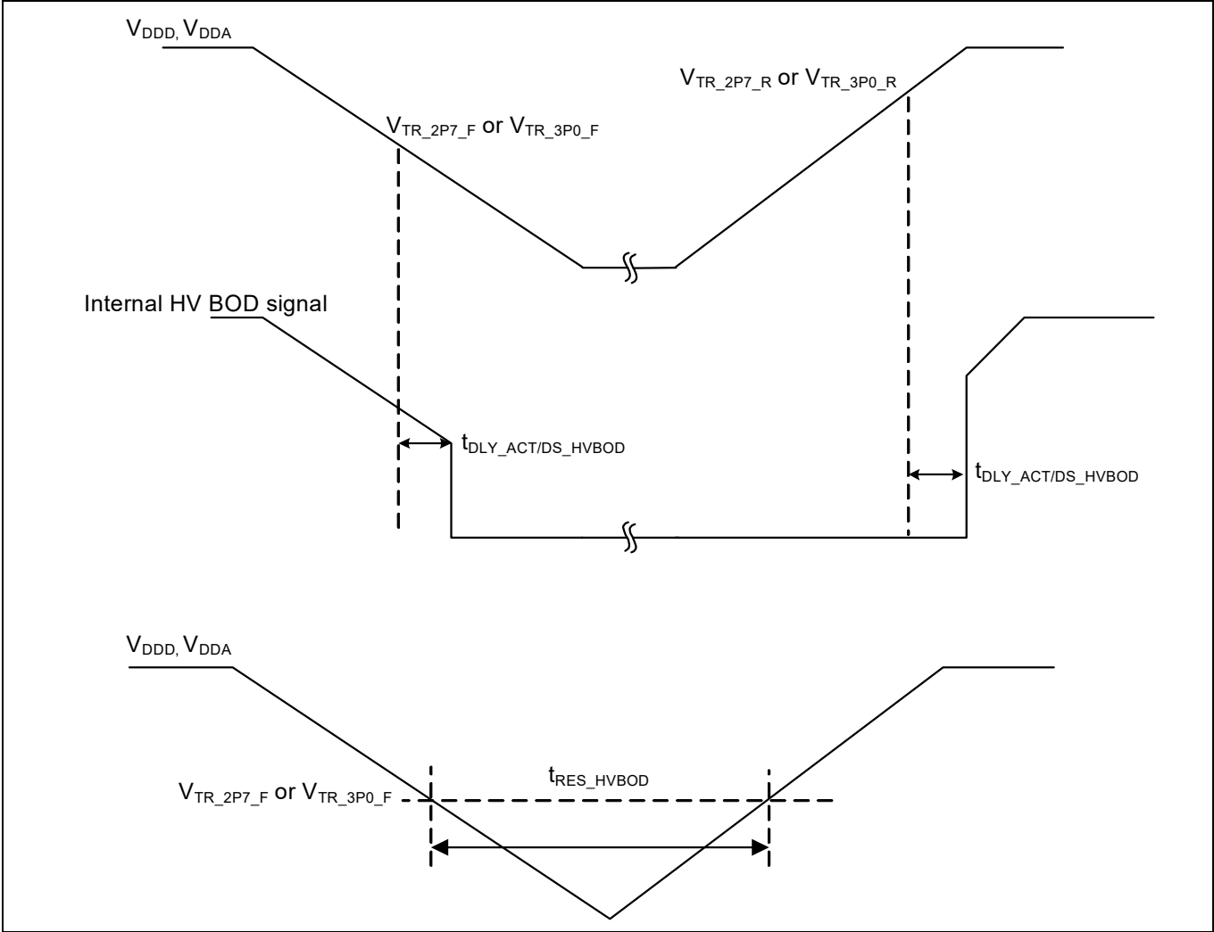
Figure 25 High-voltage BOD specifications
