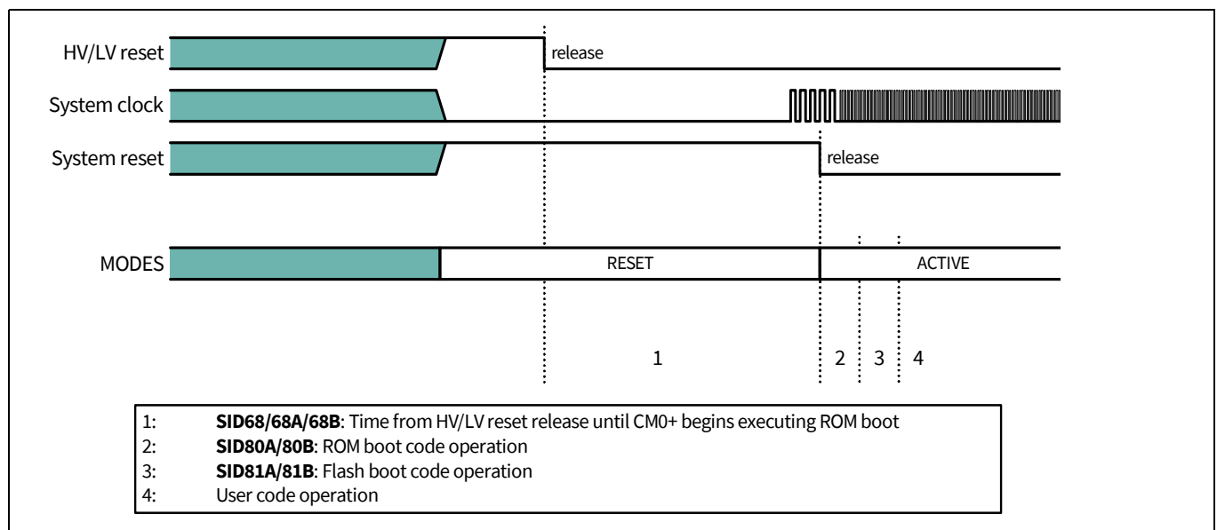
Figure 12 Reset sequence
