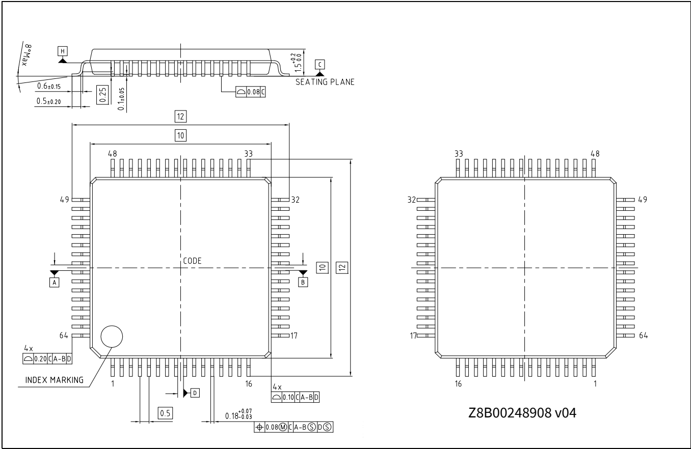
Figure 37 64-LQFP package outline (PG-LQFP-64)
