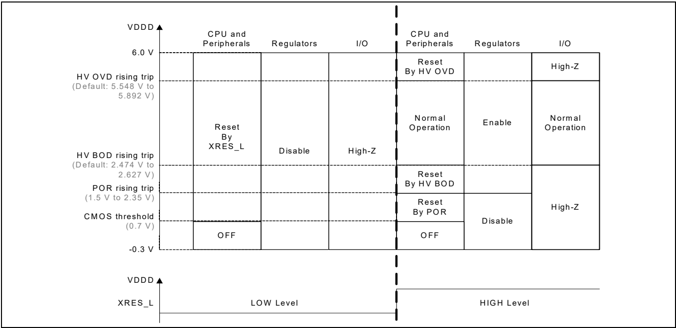
Figure 23 Device operations supply range
