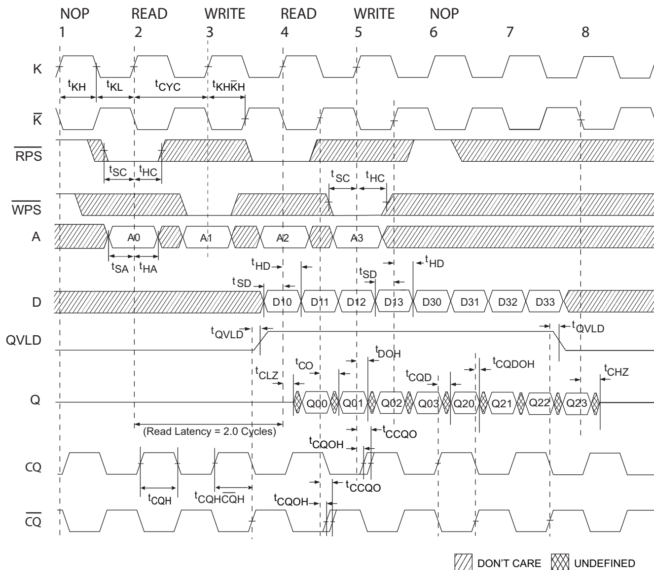
Figure 6. Waveform for 2.0 Cycle Read Latency [41, 42, 43]
