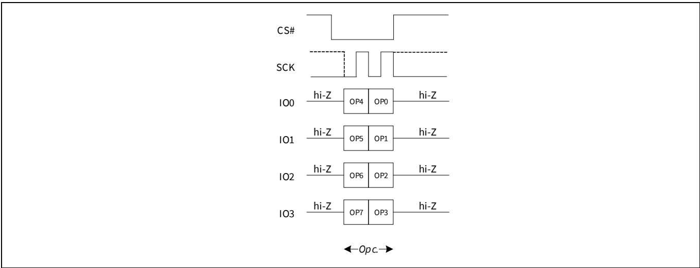
Figure 66 Chip Scrub (CSCRB 8Eh) QPI command sequence
