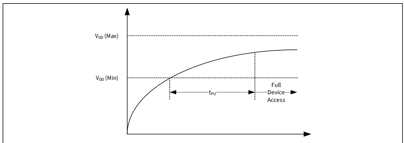
Figure 81 Power-up
