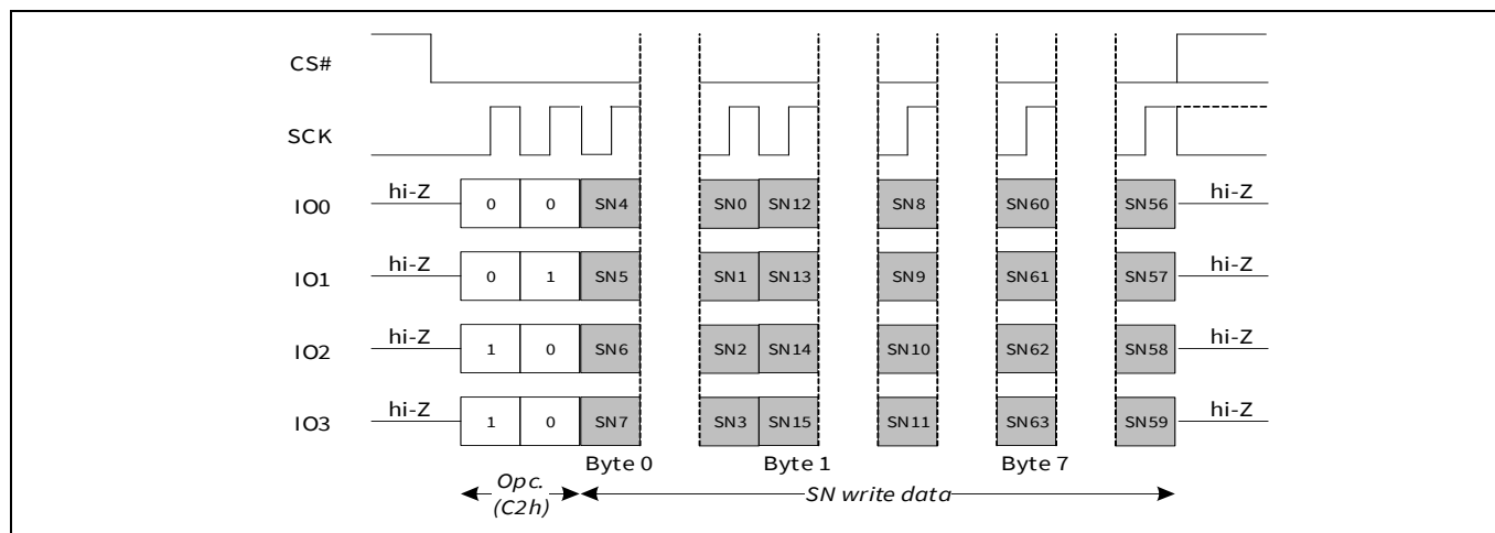
Figure 20 WRSN in QPI mode
