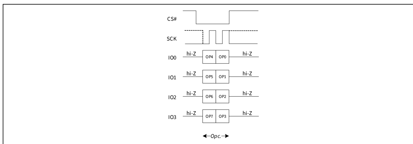
Figure 72 Chip Erase command sequence QPI mode
