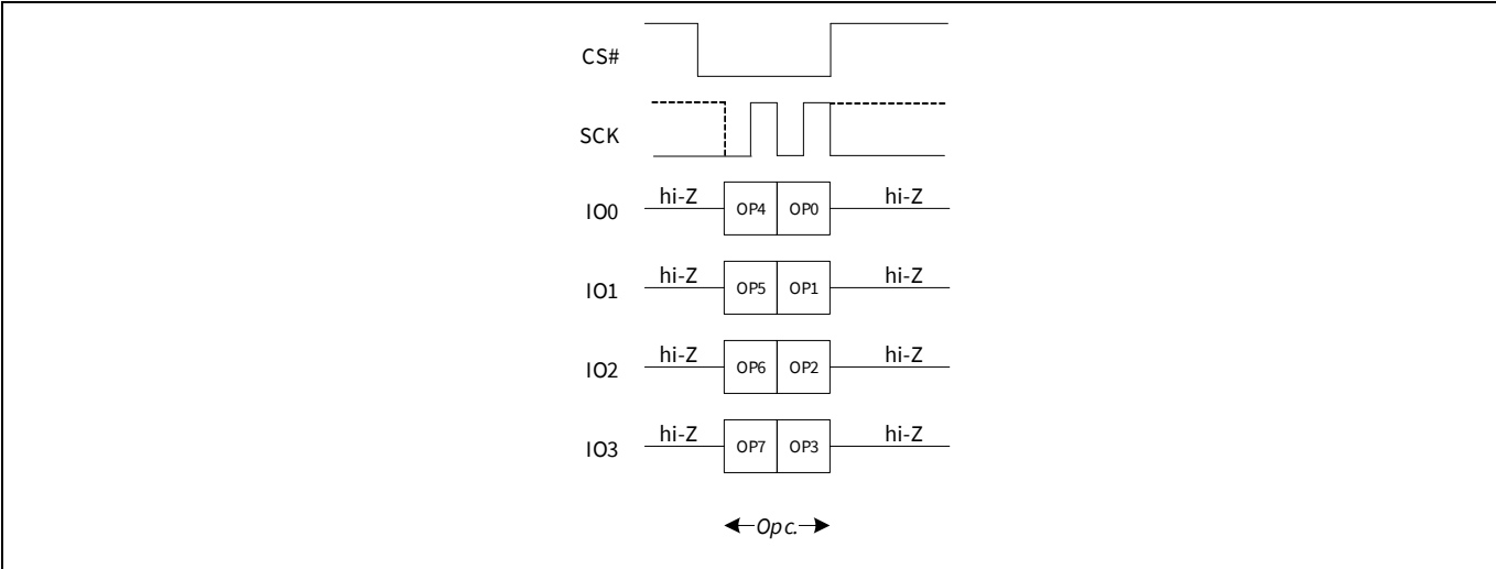
Figure 78 Software Reset/Mode Bit command sequence – QPI mode
