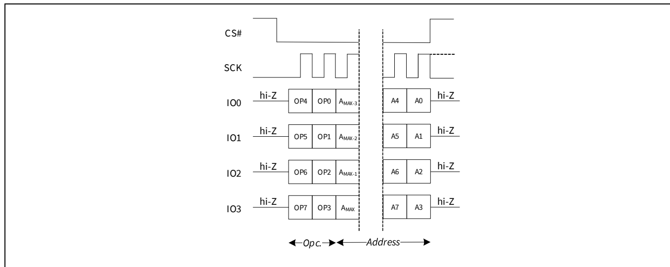
Figure 64 Page Scrub (PSCRB CEh or 4PSCRB CFh) QPI Mode command sequence [13]
