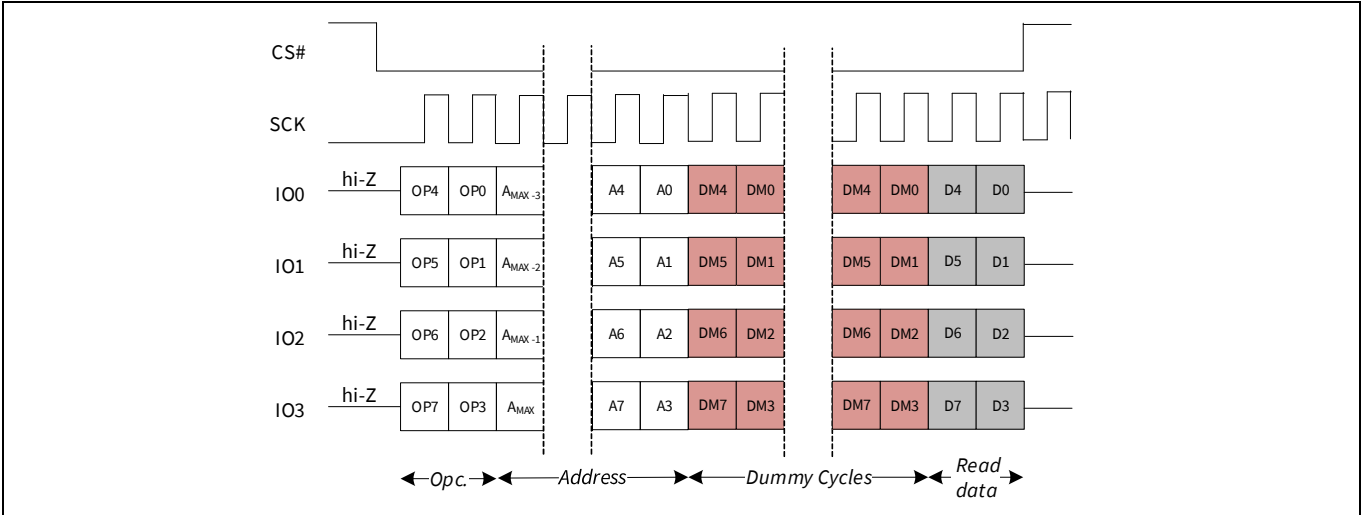
Figure 44 Read Any Register, QPI mode, command sequence [4]
