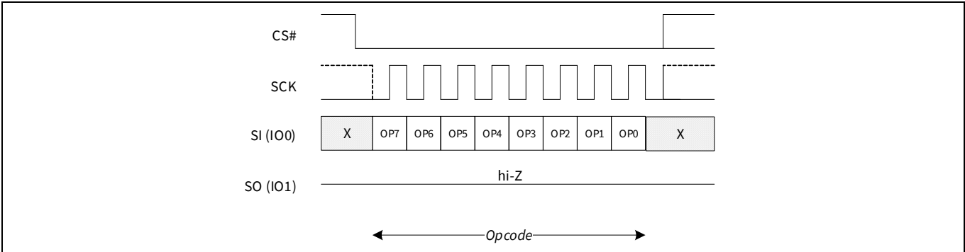
Figure 73 Erase Suspend command sequence
