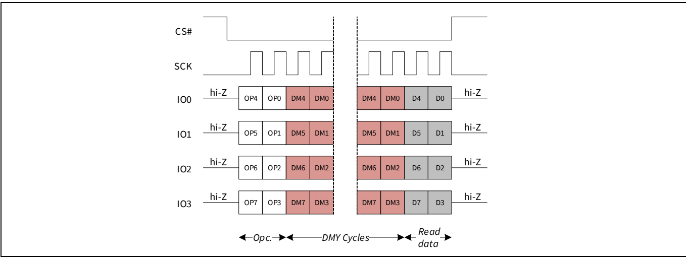
Figure 28 Read Status Register 2 (RDSR2) QPI Mode command
