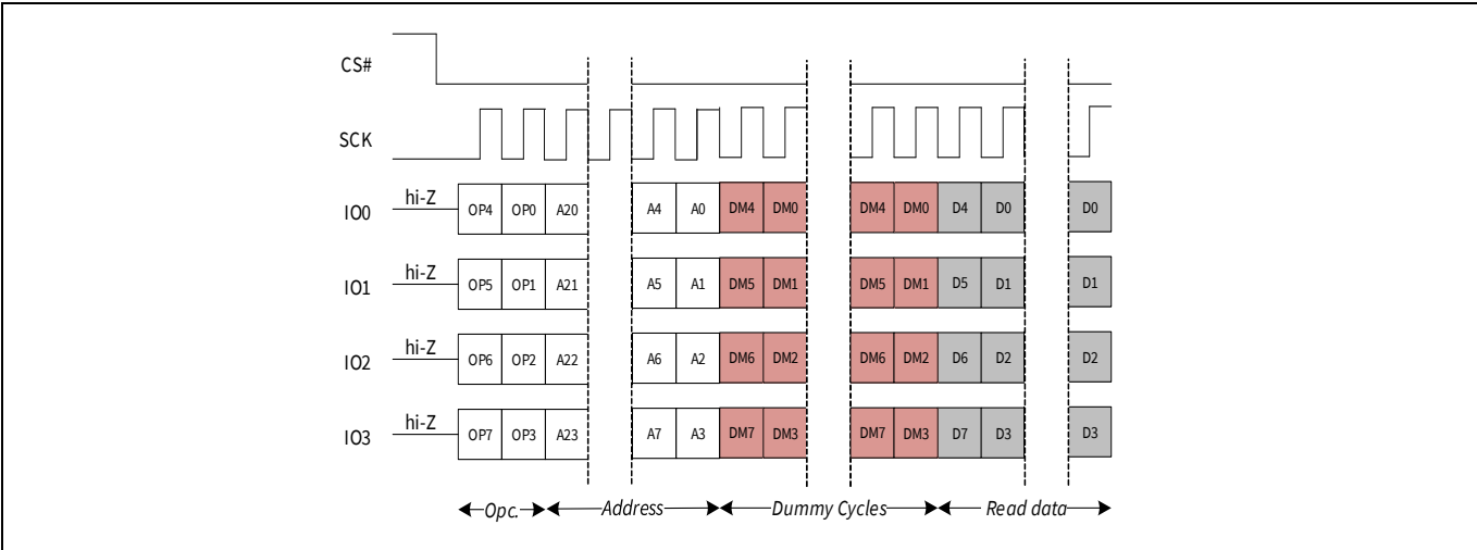
Figure 22 RSFDP QPI Mode command sequence
