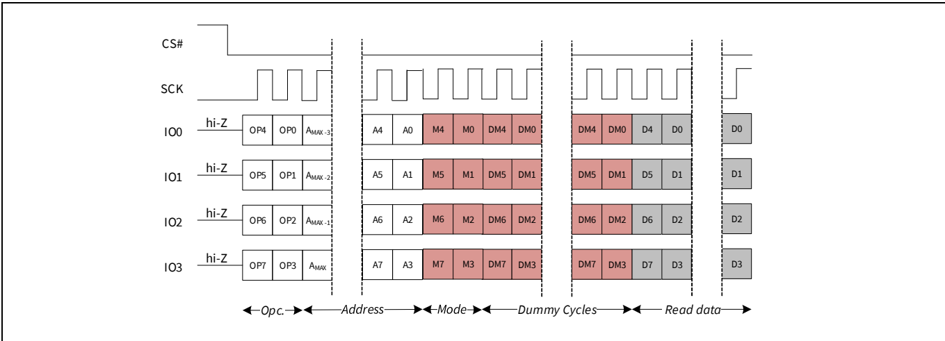
Figure 58 Quad I/O Read Initial Access command sequence QPI mode [8]
