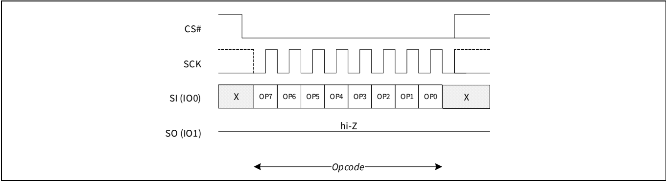
Figure 37 Clear Status Register (CLSR) command sequence
