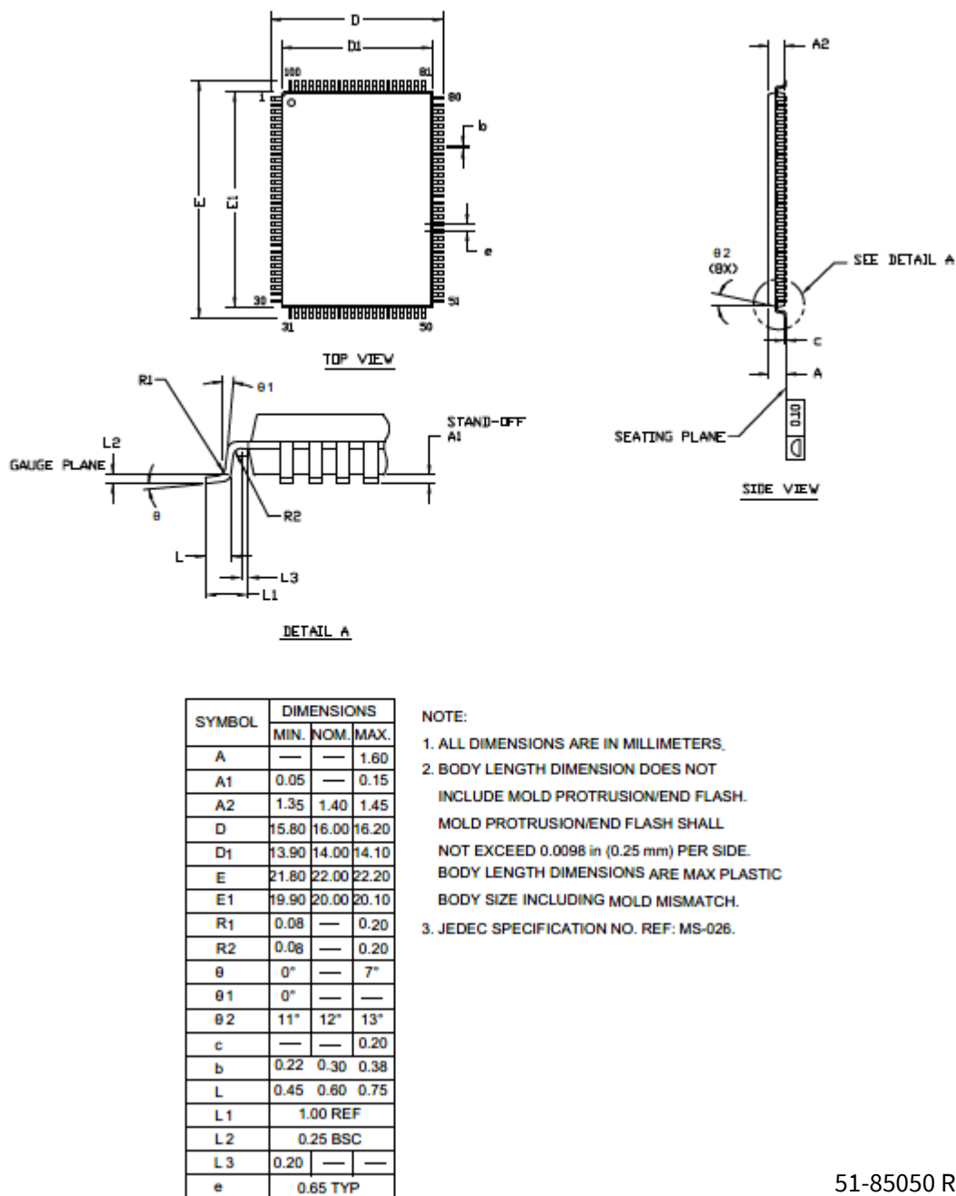
Figure 96 100-lead TQFP (14.0 × 20.0 × 1.4 mm) A100RA, (PG-TQFP-100)
