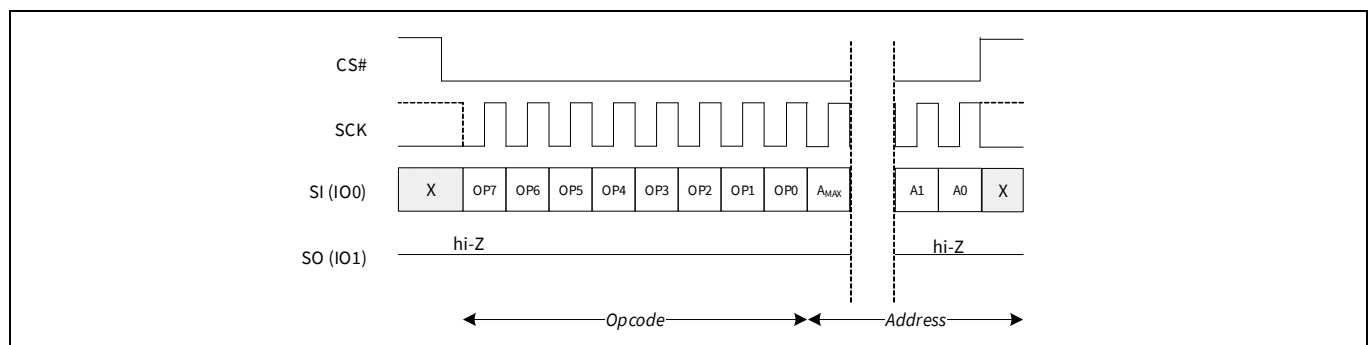
Figure 69 Block Erase (BE D8h or 4BE DCh) command sequence [16]
