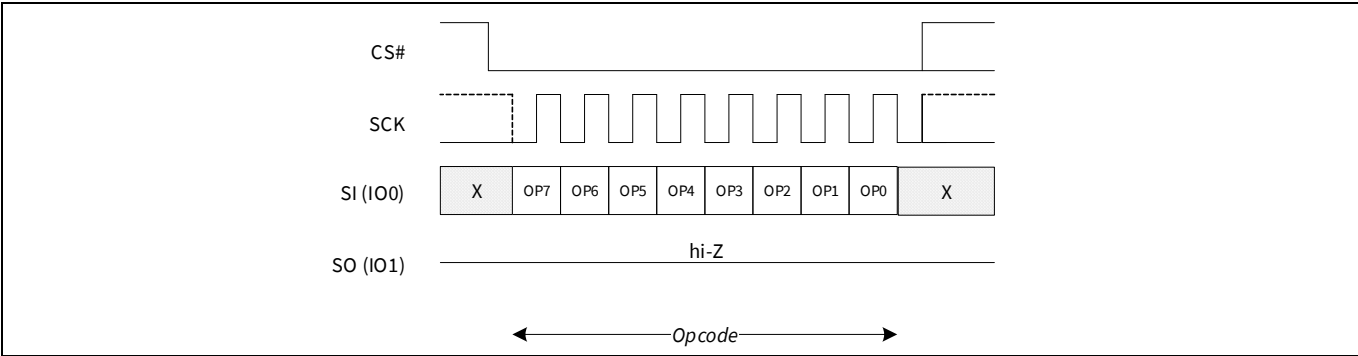
Figure 47 Enter QPI mode (QPIEN 38h) command sequence
