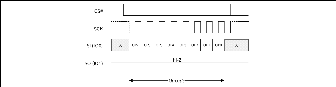
Figure 65 Chip Scrub (CSCRB 8Eh) command sequence
