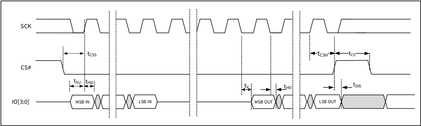
Figure 93 Quad/QPI timing
