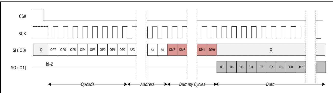
Figure 21 RSFDP command sequence
