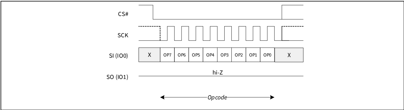
Figure 33 Write Enable (WREN) command sequence
