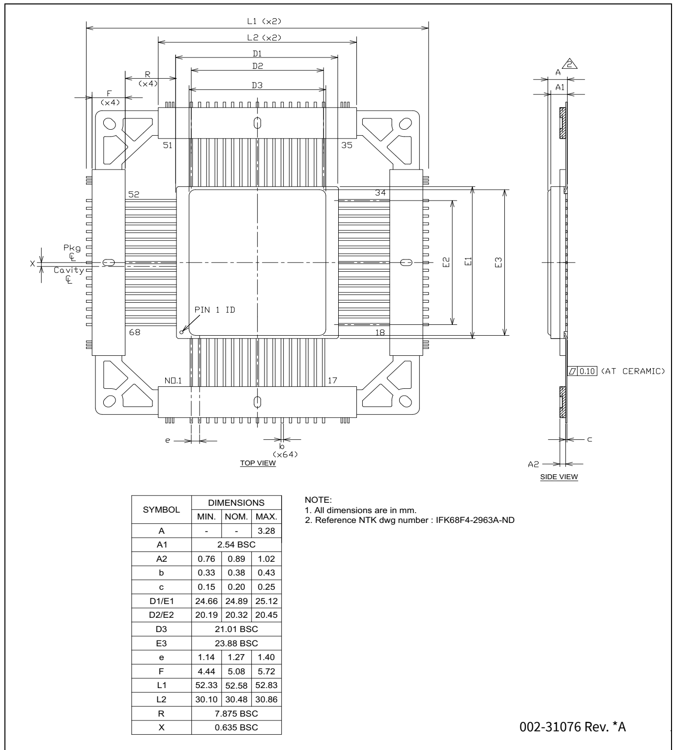
Figure 95 68-lead ceramic quad flatpack (24.89 × 24.89 × 3.28 mm) UZ68A, (CG-FP-68)
