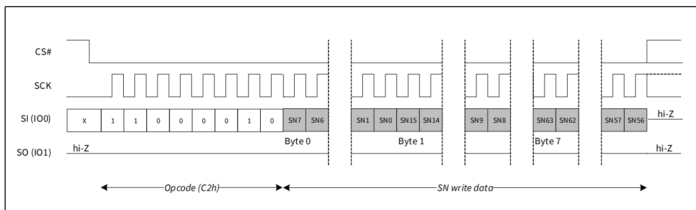
Figure 19 WRSN in SPI mode
