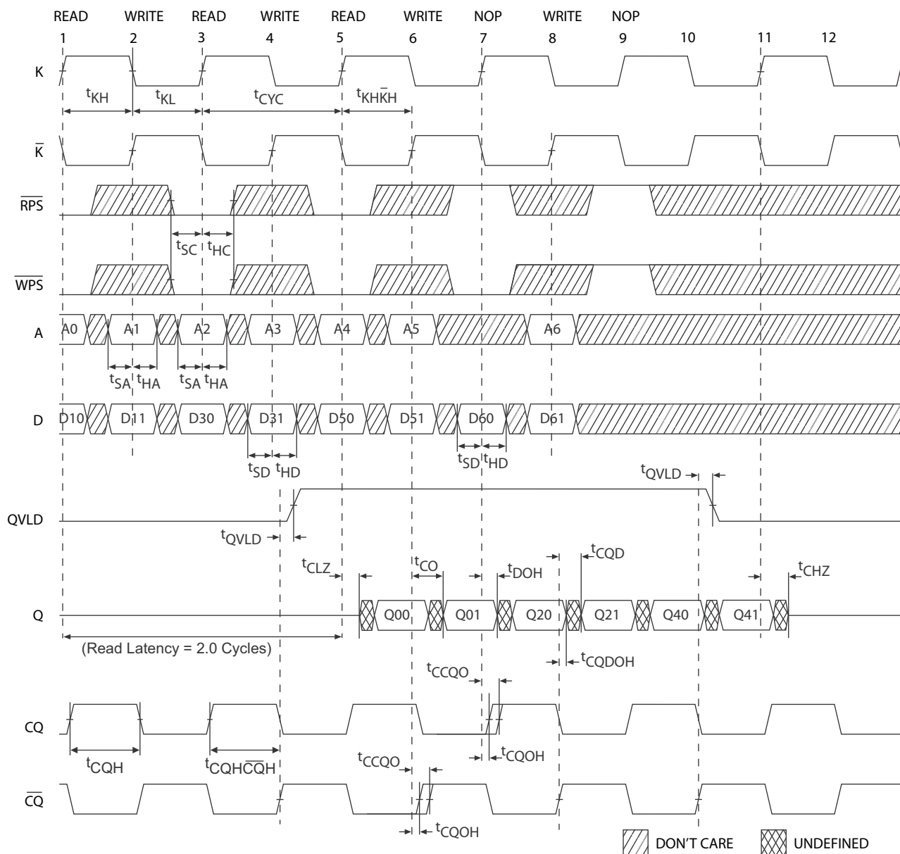
Figure 6. Read/Write/Deselect Sequence [36, 37, 38]
