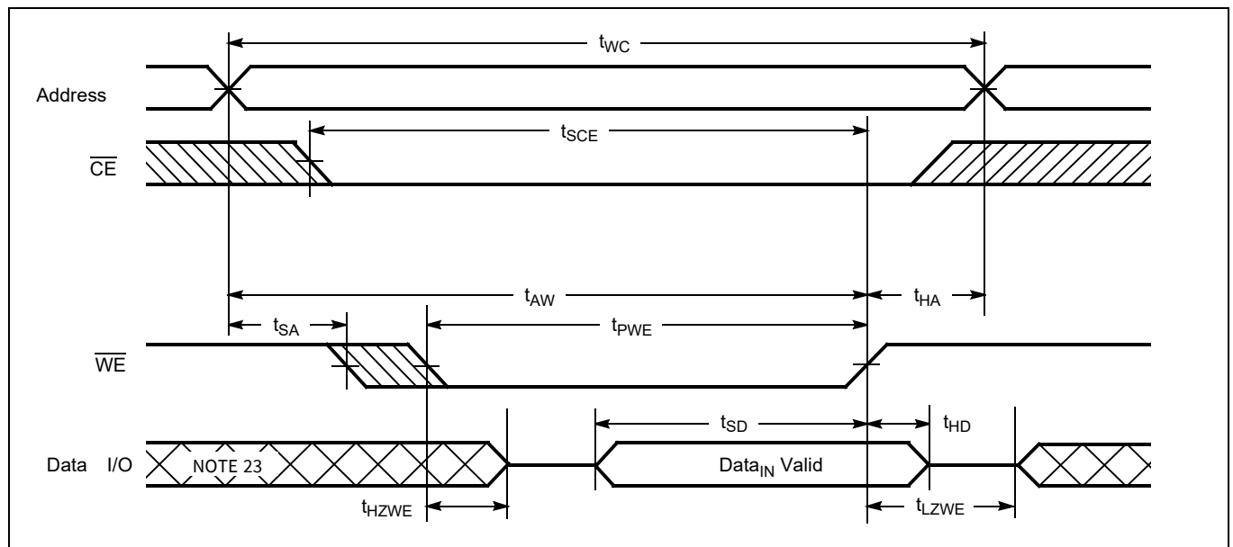
Figure 8 Write cycle No. 3 ( \overline{WE} Controlled, \overline{OE} LOW)
