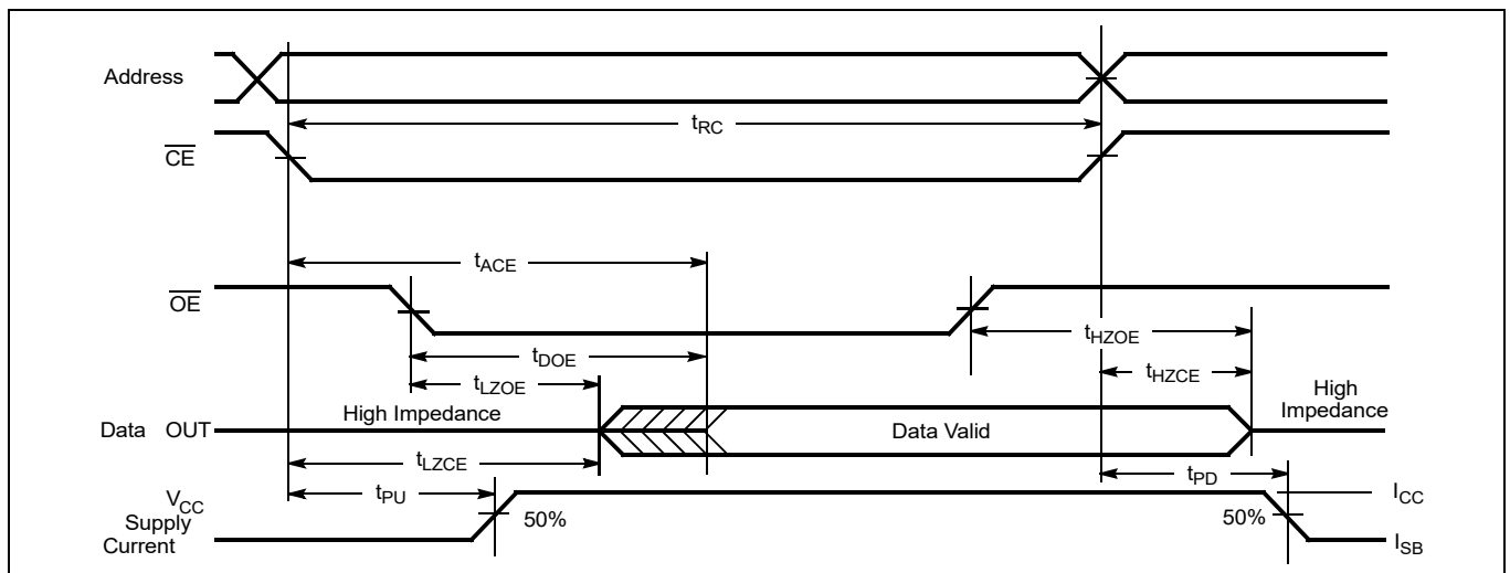
Figure 5 Read cycle No. 2 ( \overline{OE} Controlled, \overline{WE} HIGH) [18, 19]
