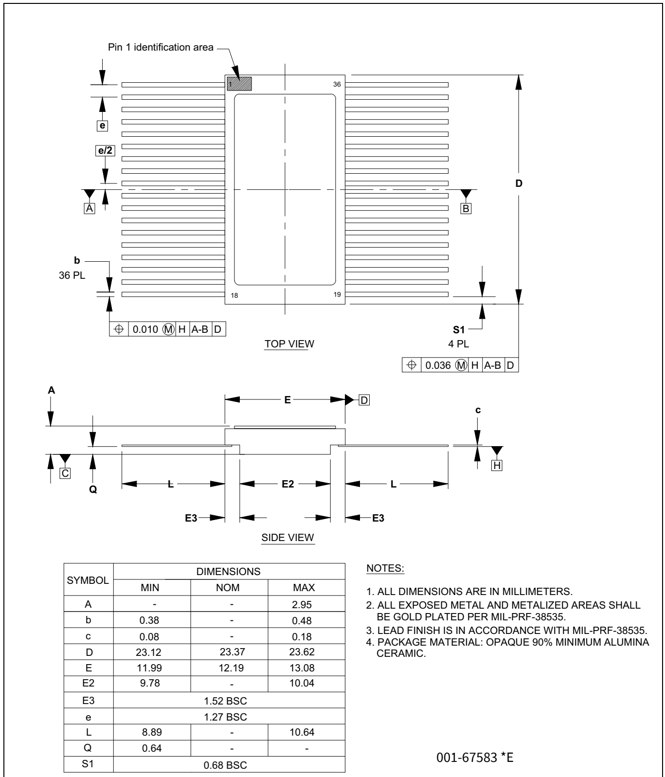
Figure 9 36-lead ceramic flat pack (23.37 × 12.19 × 2.95 mm) F36/FZ36 package outline (CG-FP-36), 001-67583
