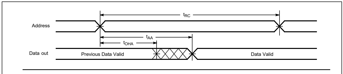
Figure 4 Read cycle No. 1 [16, 17]
