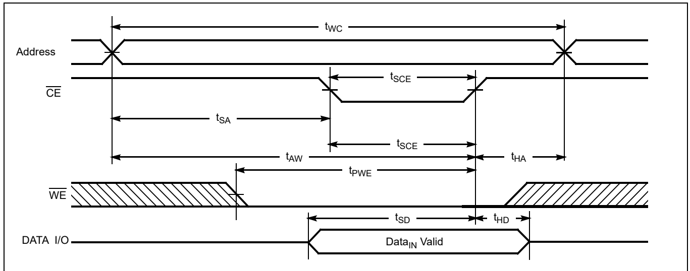
Figure 6 Write cycle No. 1 ( \overline{\text{CE}} Controlled) [20, 21]
