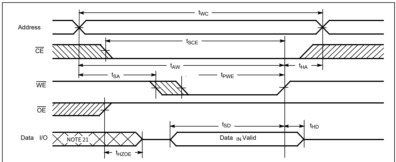
Figure 7 Write cycle No. 2 ( \overline{\text{WE}} Controlled, \overline{\text{OE}} HIGH) [20, 21, 22]
