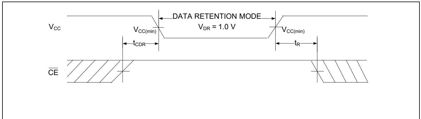
Figure 3 Data retention waveform
