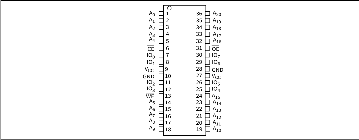
Figure 1 36-pin ceramic flat package pinout (top view) [3]
