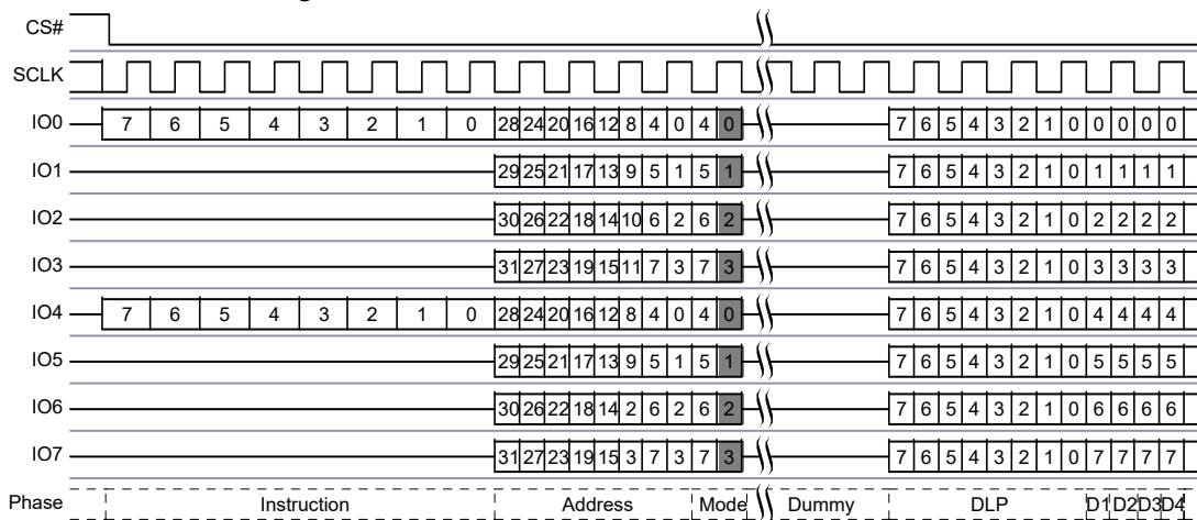
Figure 13. SPI DDR Quad I/O Read Command [9, 10]
