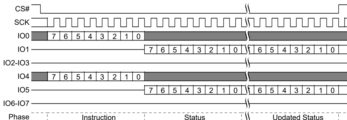
Figure 26. SPI Read Status Register-1 (RDSR1) Command Sequence
