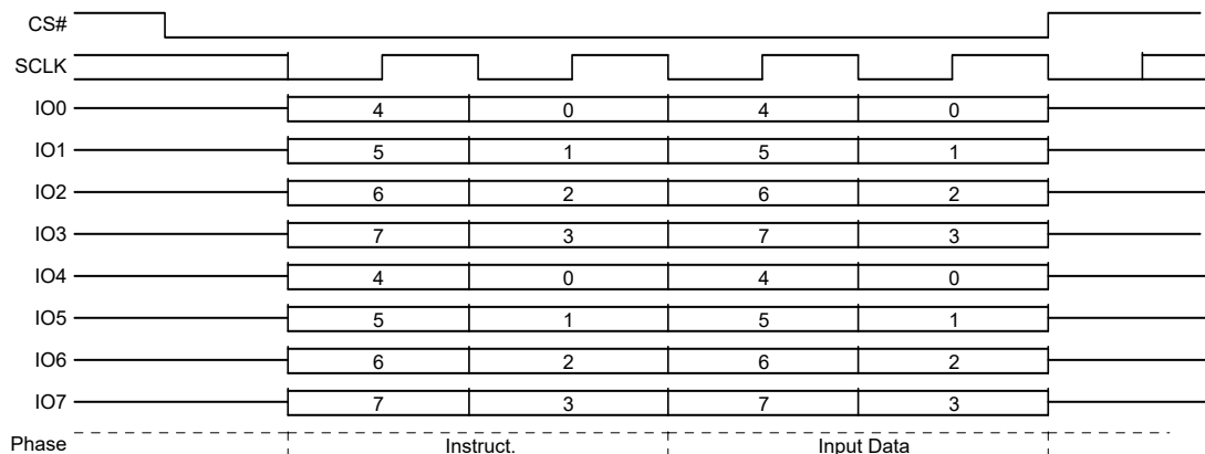
Figure 41. SPI Program DLRNV (PDLRNV) Command Sequence – QPI Mode
