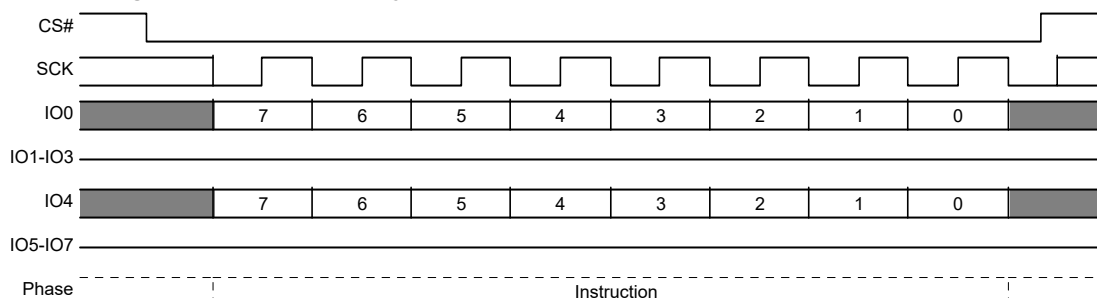
Figure 46. SPI Enter 4 Byte Address Mode (4BEN B7h) Command Sequence
