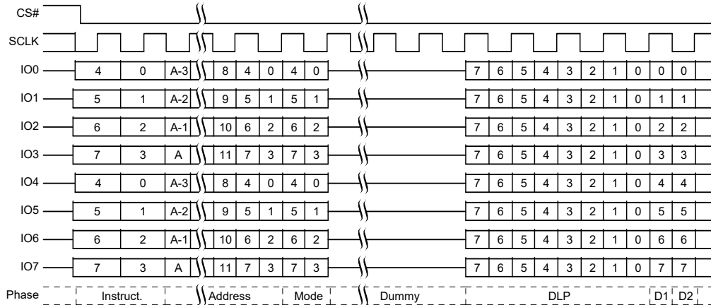
Figure 63. SPI DDR Quad I/O Read Initial Access QPI Mode [37, 39]
