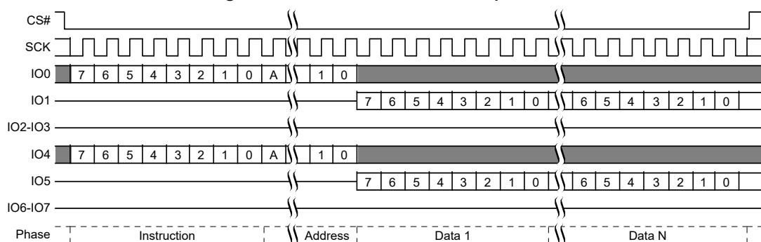
Figure 56. SPI Read Command Sequence [32]
