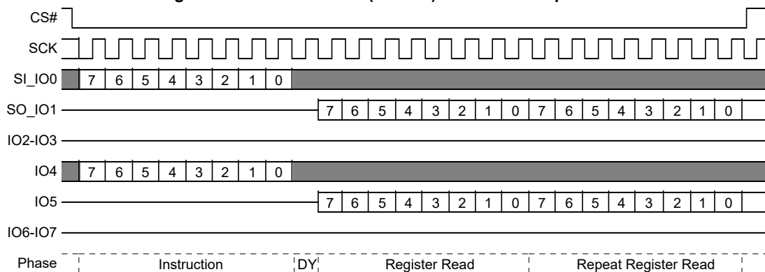
Figure 44. SPI DLP Read (DLPRD) Command Sequence
