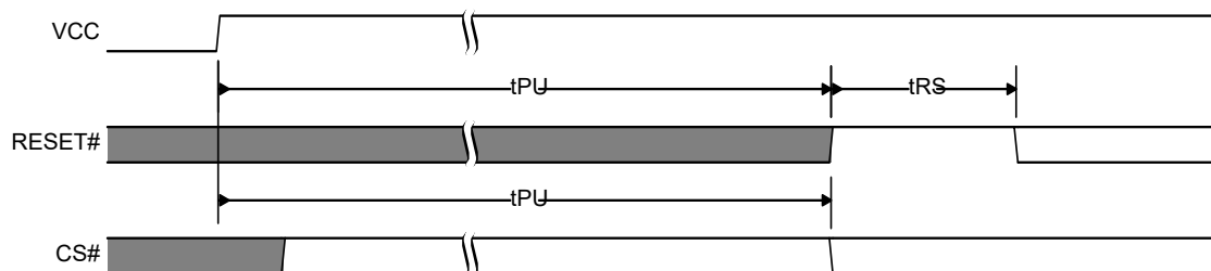
Figure 124. POR Followed by Hardware Reset
