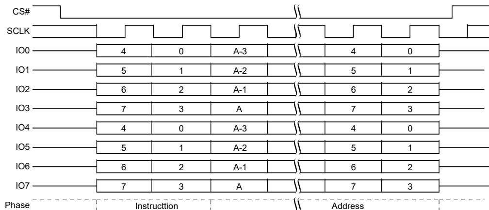
Figure 88. IBUL Command Sequence QPI Mode [53, 54]
