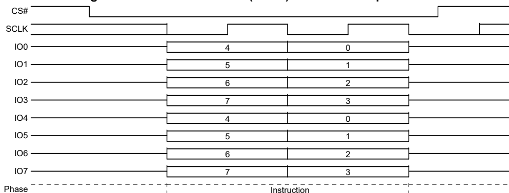
Figure 35. SPI Write Disable (WRDI) Command Sequence QPI Mode
