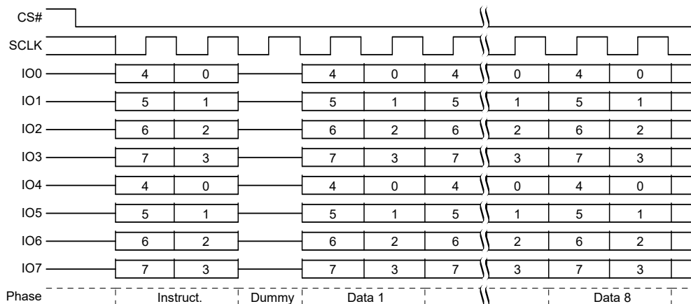
Figure 104. SPI Password Read (PASSRD) Command Sequence – QPI Mode
