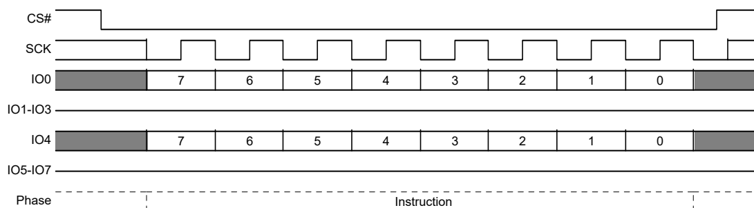
Figure 89. SPI Global IBL Lock (GBL) Command Sequence
