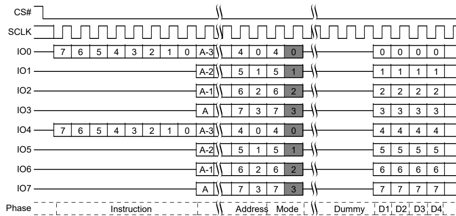
Figure 59. SPI, Quad I/O Read Initial Access Command Sequence [35]
