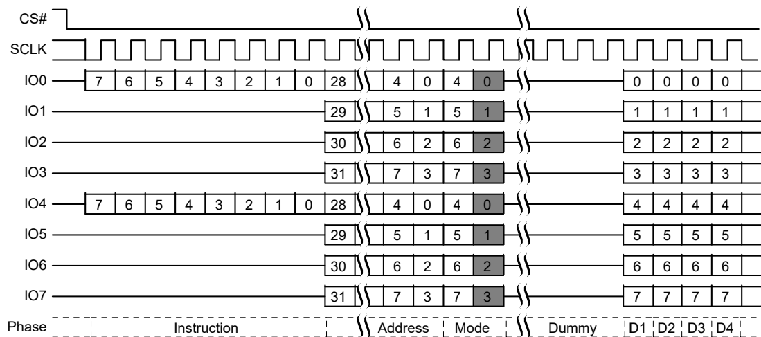
Figure 11. SPI, Quad I/O Command [7, 8]
