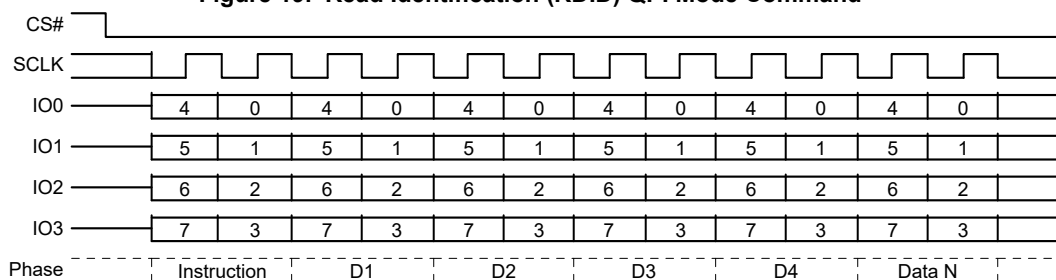
Figure 19. Read Identification (RDID) QPI Mode Command
