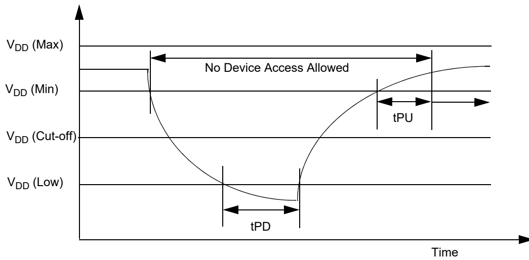
Figure 118. Power-down and Voltage Drop
