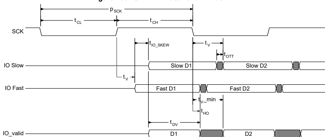
Figure 130. SPI DDR Data Valid Window
