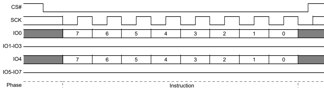
Figure 101. SPI Protection Register Lock (PRL) Command Sequence
