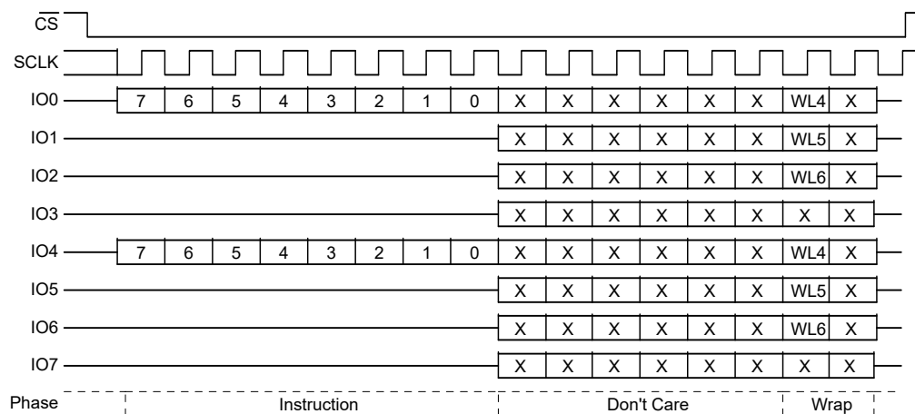
Figure 52. SPI Set Burst Length Command Sequence Quad I/O Mode
