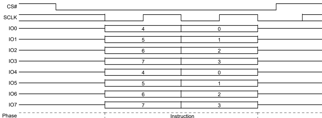
Figure 75. Chip Erase Command Sequence QPI Mode
