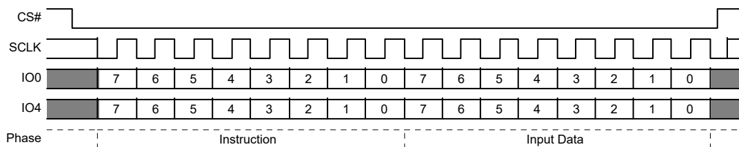
Figure 7. SPI Single Bit Wide Input Command [6]
