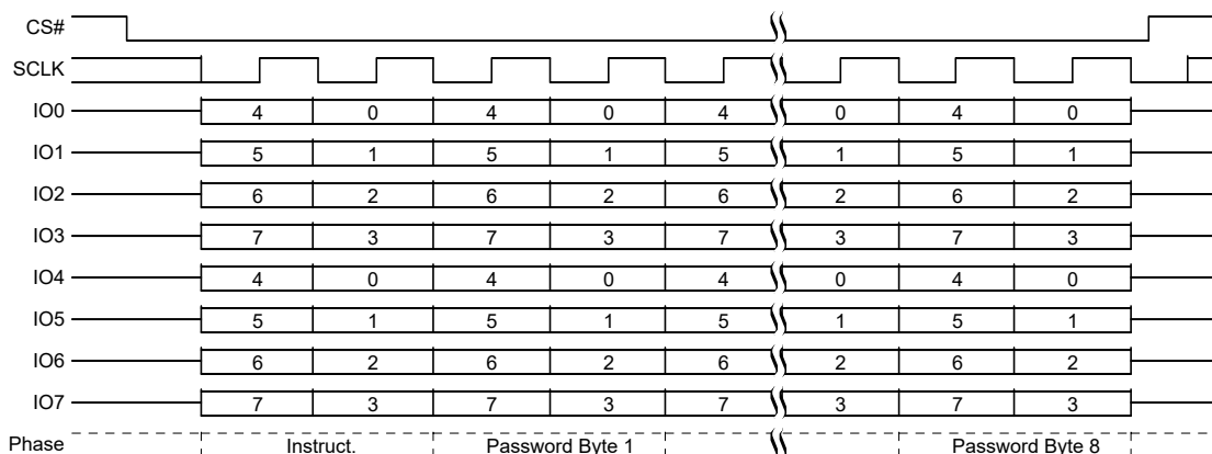
Figure 108. Password Unlock (PASSU) Command Sequence QPI Mode
