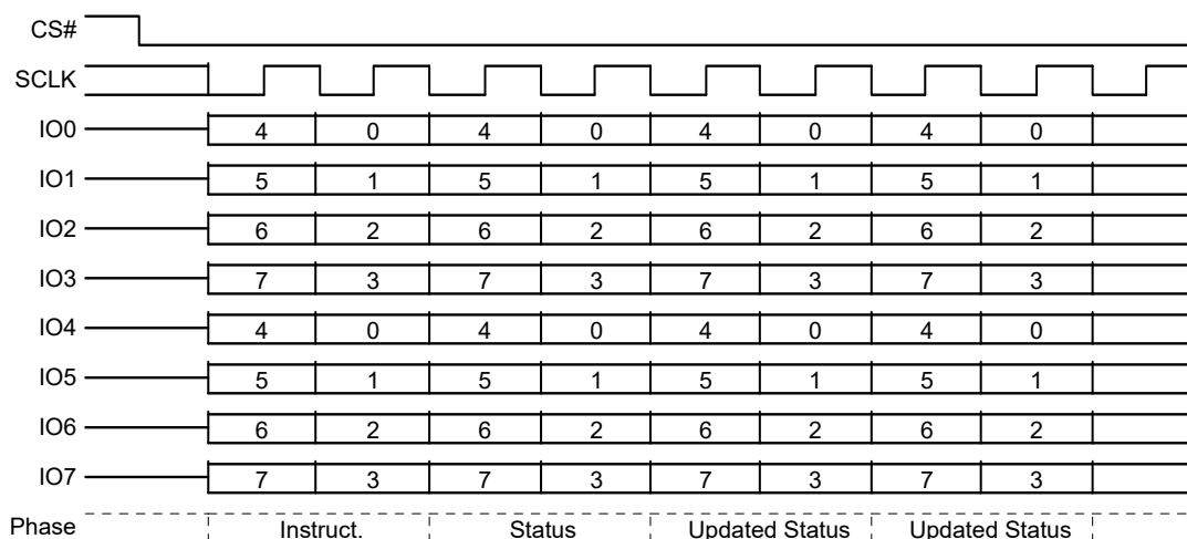
Figure 27. SPI Read Status Register-1 (RDSR1) QPI Mode Command
