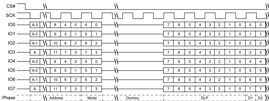
Figure 64. SPI Continuous DDR Quad I/O Read Subsequent Access [37, 39, 40]
