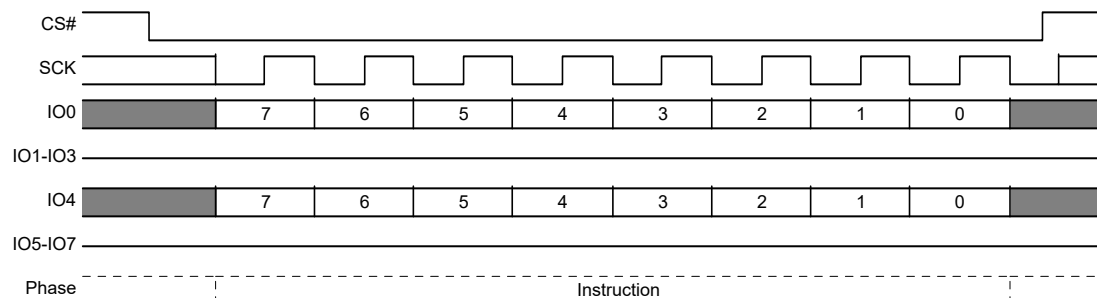
Figure 48. SPI Exit 4 Byte Address Mode (4BEX E9h) Command Sequence
