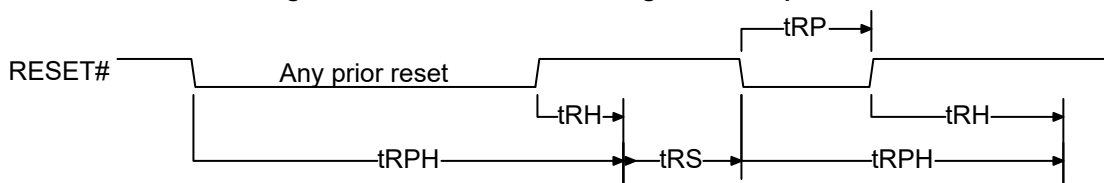
Figure 125. Hardware Reset using RESET# Input
