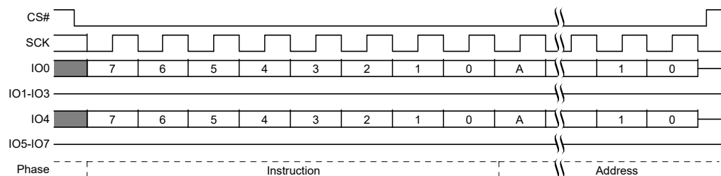
Figure 68. Sector Erase (SE 20h or 4SE 21h) Command Sequence [44]
