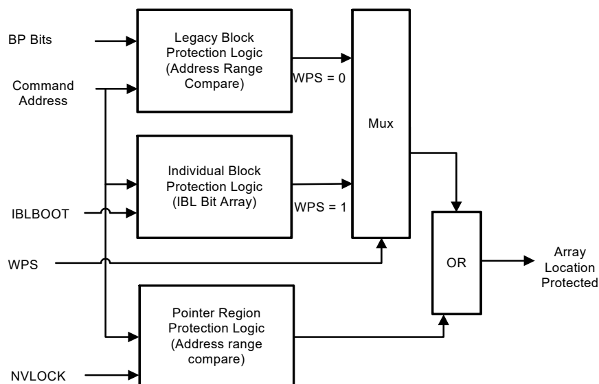
Figure 15. WPS Selection of LBP or IBL and PRP Array Protection
