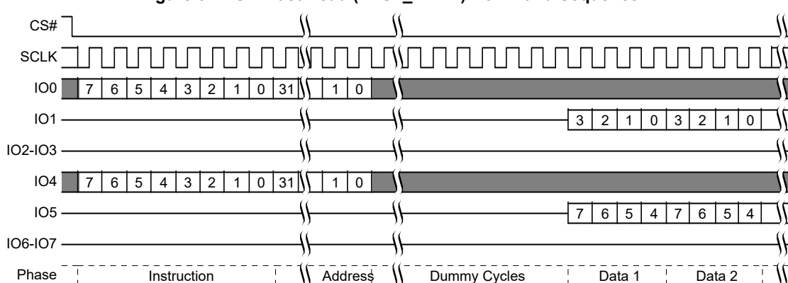
Figure 57. SPI Fast Read (FAST_READ) Command Sequence [33]
