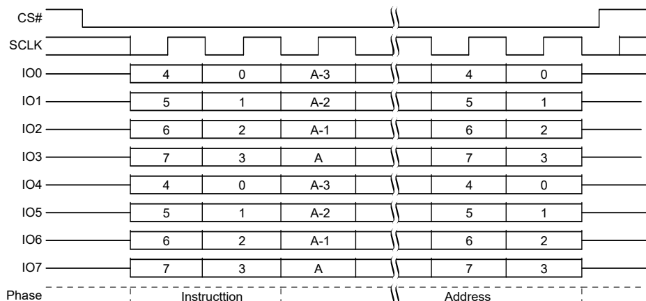
Figure 71. Half Block Erase (HBE 52h or 4HBE 53h) QPI Mode Command Sequence [45]
