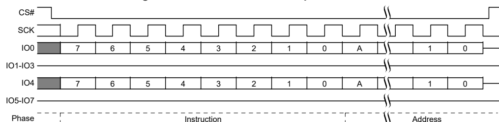
Figure 87. IBUL Command Sequence [53, 54]
