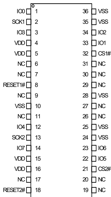
Figure 1. 36-Lead Ceramic Flatpack (36FP), Top View [1]
