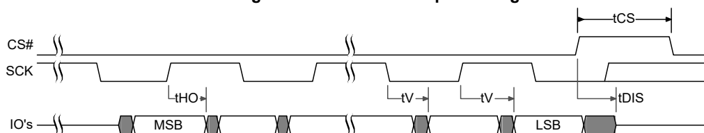
Figure 129. SPI DDR Output Timing
