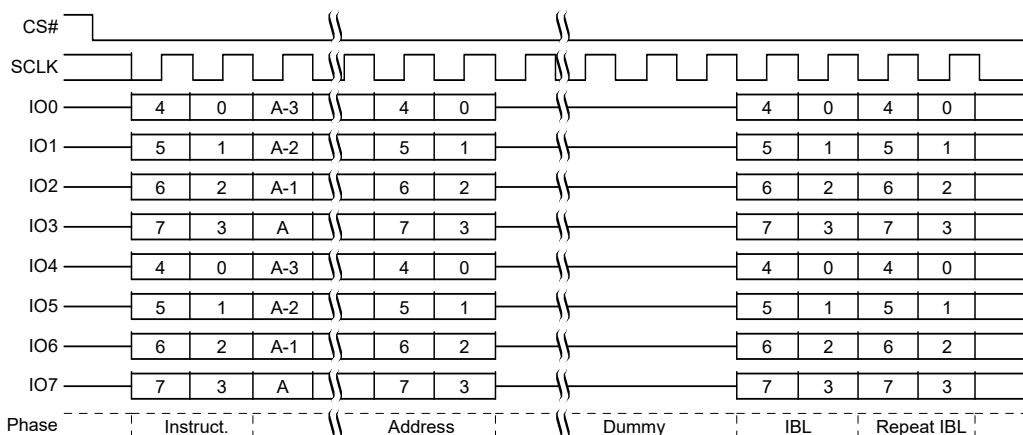
Figure 84. IBLRD Command Sequence QPI [49, 50]
