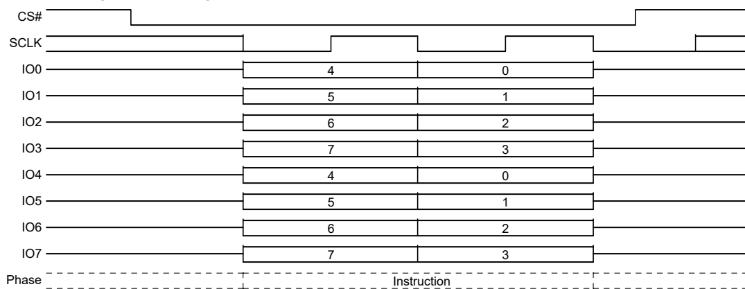
Figure 77. Program or Erase Suspend Command Sequence QPI Mode
