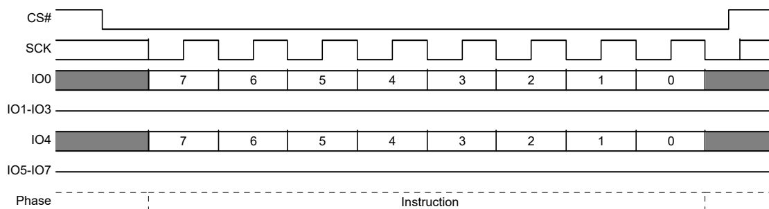
Figure 109. SPI Software Mode Bit Reset Command Sequence
