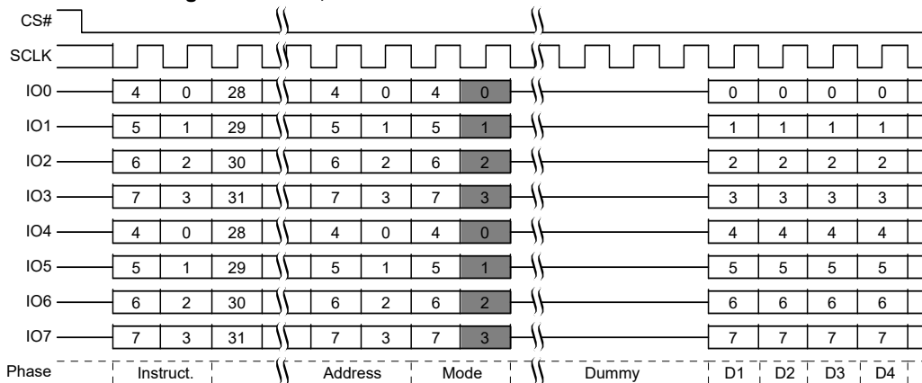
Figure 12. SPI, Quad I/O Read Command in QPI Mode [7, 8]
