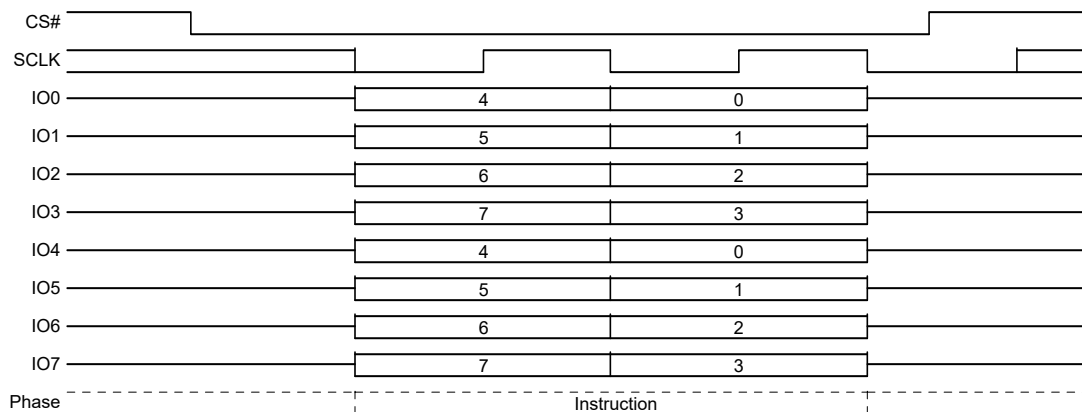
Figure 90. SPI Global IBL Lock (GBL) Command Sequence QPI Mode
