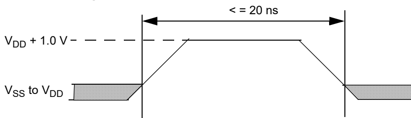
Figure 116. Maximum Positive Overshoot Waveform
