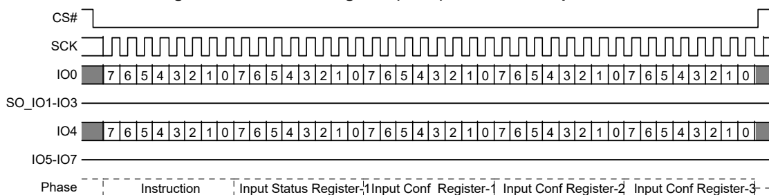
Figure 30. SPI Write Register (WRR) Command Sequence
