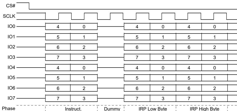
Figure 96. SPI IRPRD Command Sequence – QPI Mode
