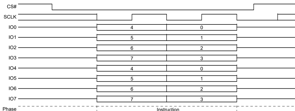
Figure 33. SPI Write Enable (WREN) Command Sequence QPI Mode
