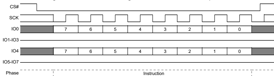
Figure 79. SPI Erase or Program Resume command Sequence
