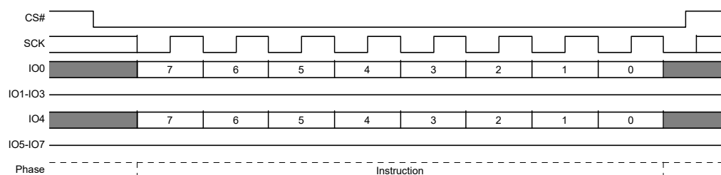
Figure 74. SPI Chip Erase Command Sequence
