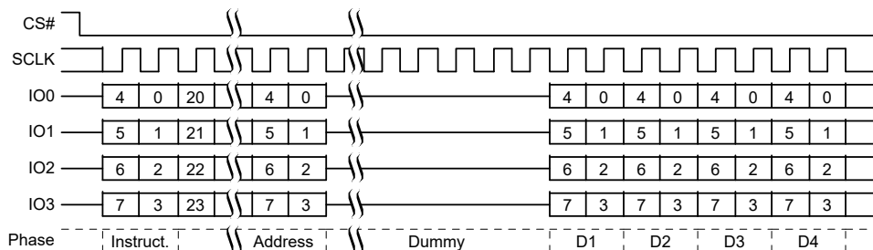
Figure 23. RSFDP QPI Mode Command Sequence
