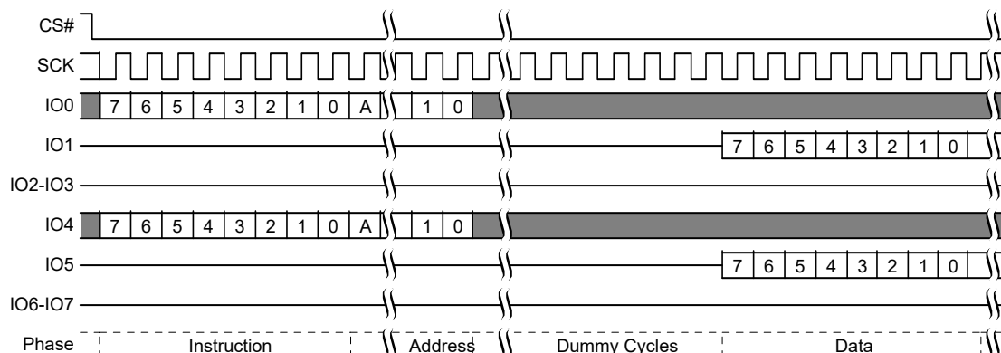
Figure 50. SPI Read Any Register Read Command Sequence [31]
