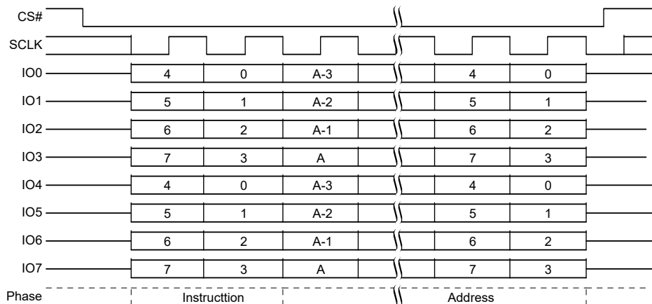
Figure 86. IBL Command Sequence QPI Mode [51, 52]
