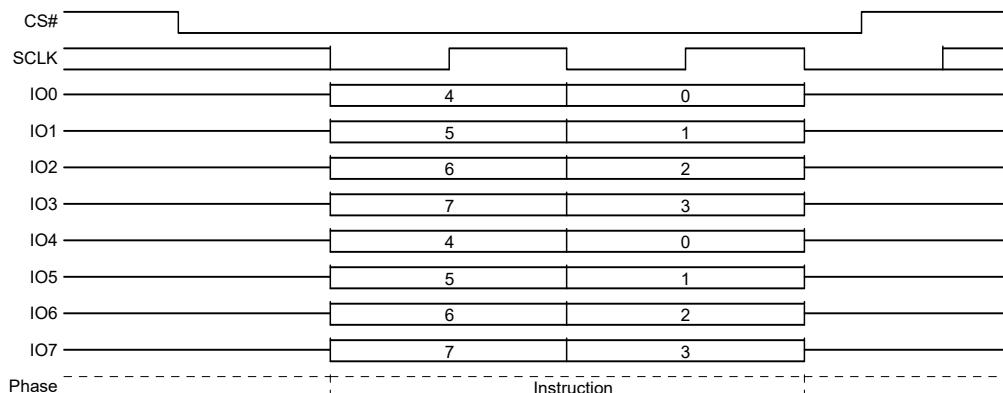
Figure 102. SPI Protection Register Lock (PRL) Command Sequence – QPI Mode
