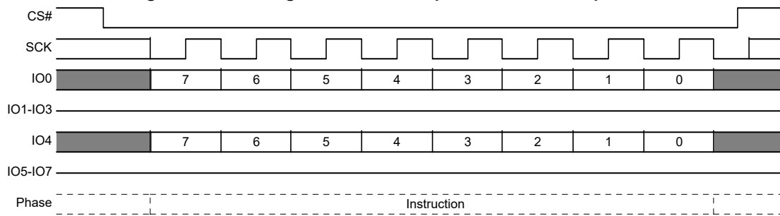
Figure 76. SPI Program or Erase Suspend Command Sequence
