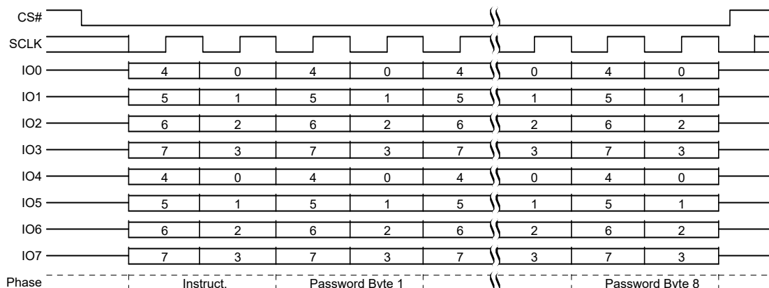
Figure 106. Password Program (PASSP) Command Sequence QPI Mode
