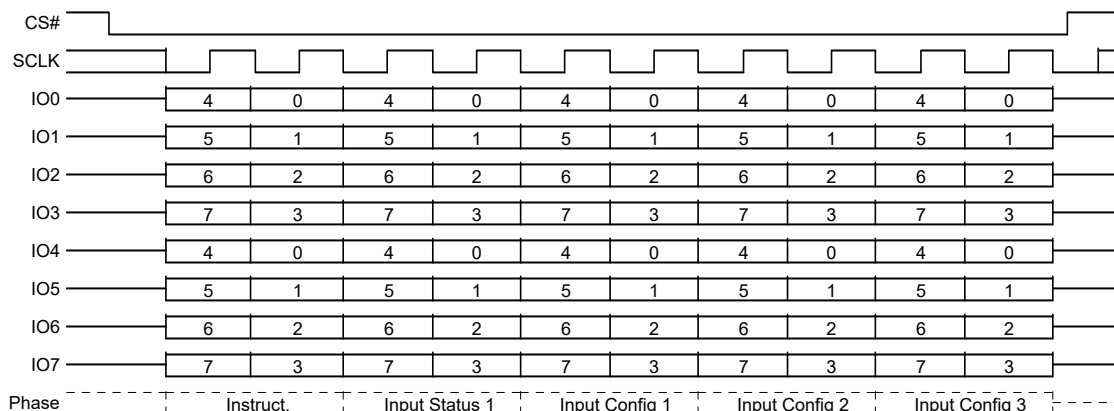
Figure 31. SPI Write Registers (WRR) Command Sequence QPI Mode
