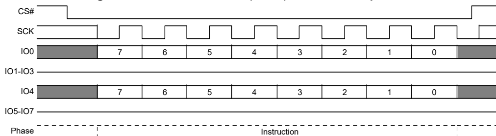
Figure 34. SPI Write Disable (WRDI) Command Sequence
