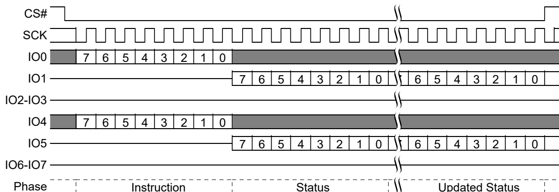
Figure 28. SPI Read Status Register-2 (RDSR2) Command
