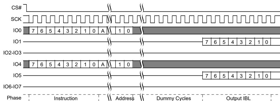
Figure 83. IBLRD Command Sequence [49, 50]
