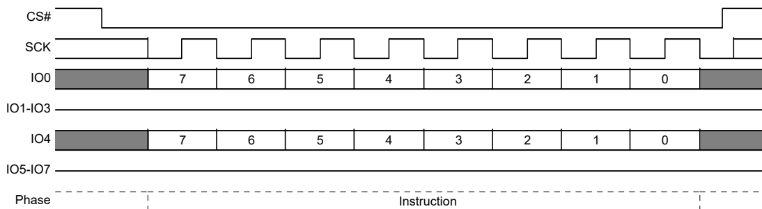
Figure 32. SPI Write Enable (WREN) Command Sequence
