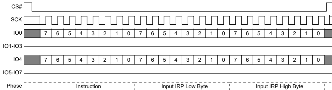
Figure 97. IRP Program (IRPP) Command
