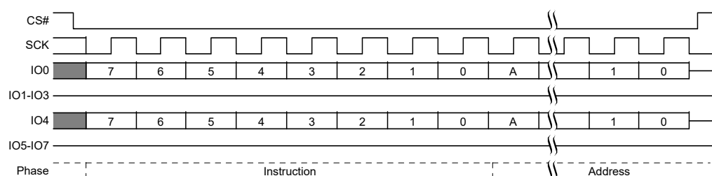
Figure 72. Block Erase (BE D8h or 4BE DCh) Command Sequence [46]
