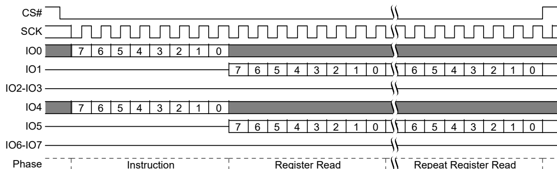
Figure 29. SPI Read Configuration Register (RDCR1) (RDCR2) (RDCR3) Command Sequence
