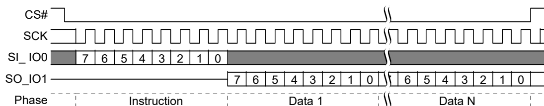
Figure 18. Read Identification (RDID) Command Sequence
