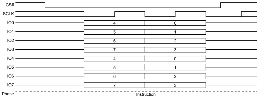
Figure 49. SPI Exit 4 Byte Address QPI Mode
