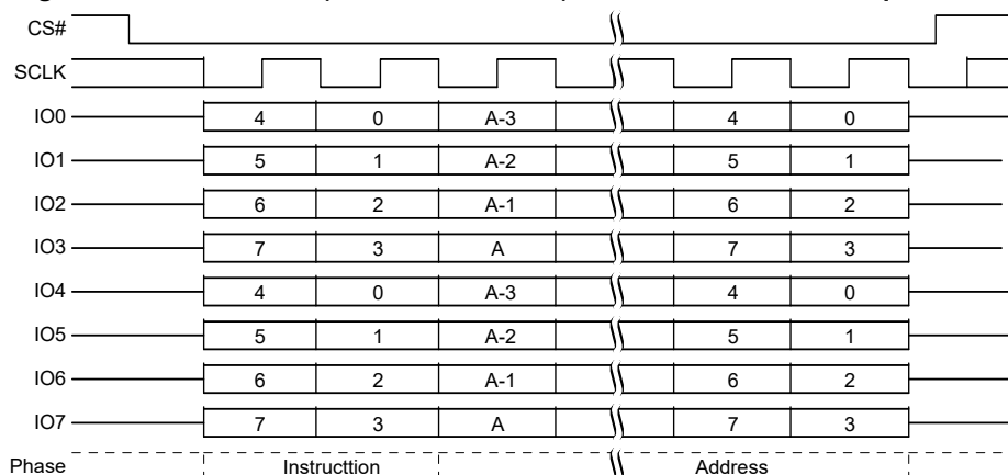
Figure 69. Sector Erase (SE 20h or 4SE 21h) QPI Mode Command Sequence [44]
