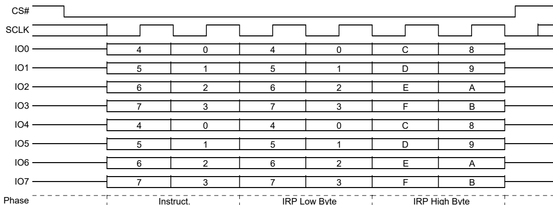
Figure 98. IRP Program (IRPP) Command QPI
