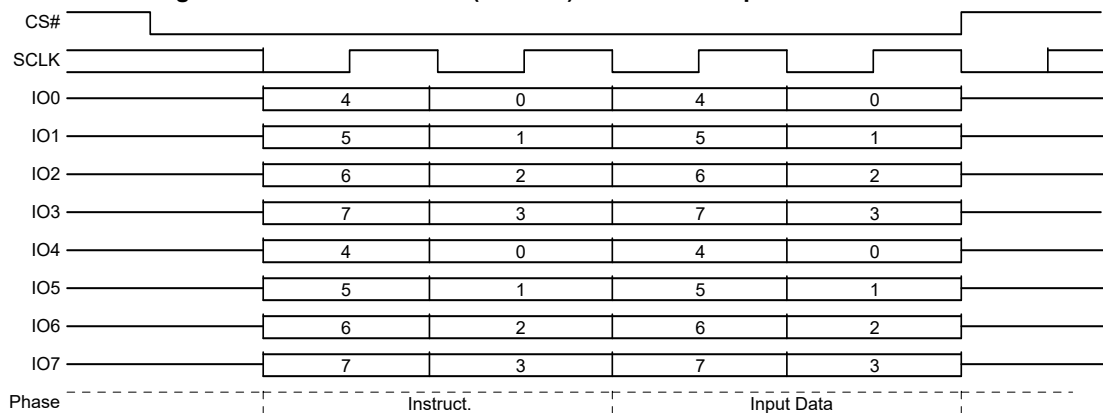
Figure 43. SPI Write DLRV (WDLRV) Command Sequence – QPI Mode
