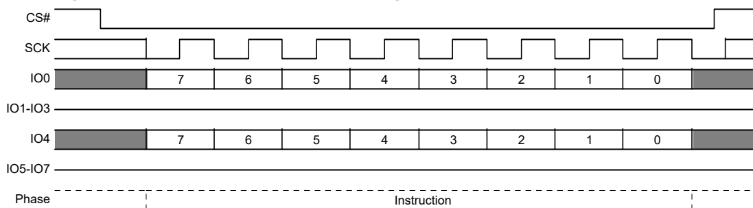
Figure 36. SPI Write Enable for Volatile Registers (WRENV) Command Sequence
