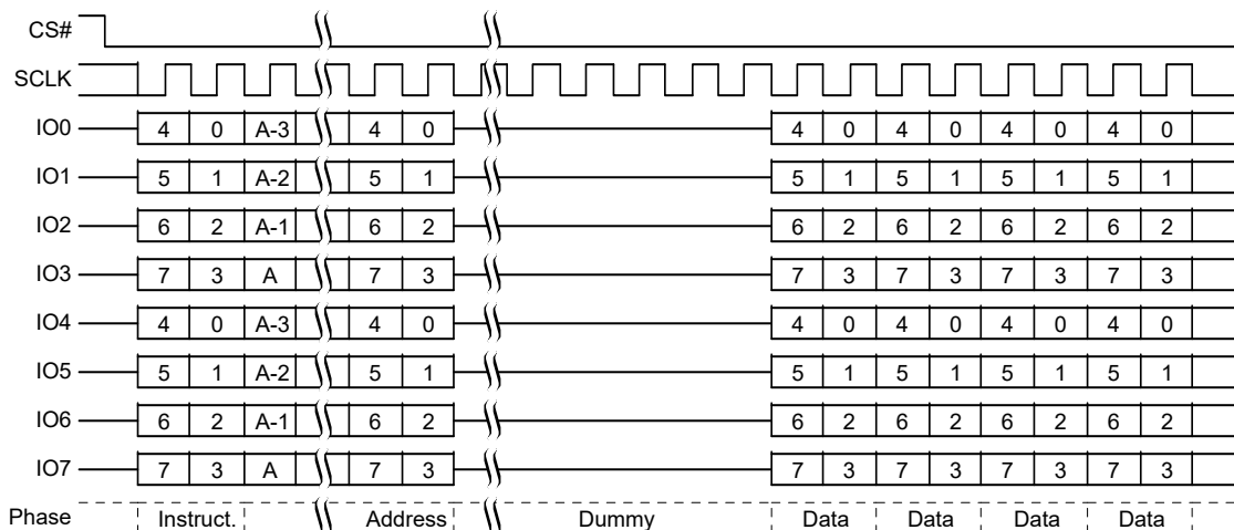
Figure 51. SPI Read Any Register, QPI Mode, Command Sequence [31]
