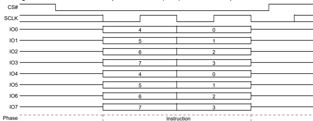
Figure 114. SPI Release Deep Power Down (RES) Command Sequence – QPI Mode
