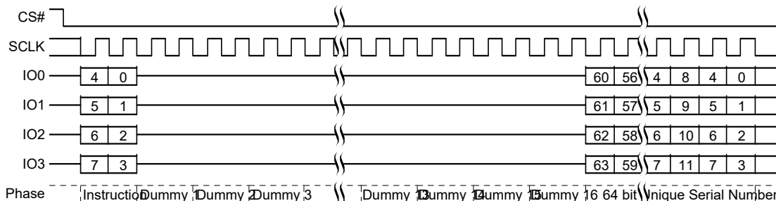
Figure 25. Read Unique ID (RUID) QPI Mode Command
