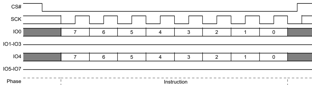
Figure 113. SPI Release from Deep Power Down (RES) Command Sequence
