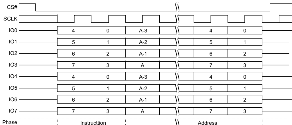
Figure 94. SPRP Command Sequence QPI Mode [57, 58]
