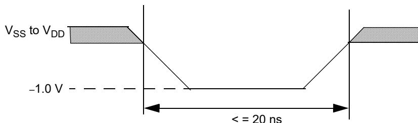
Figure 115. Maximum Negative Overshoot Waveform
