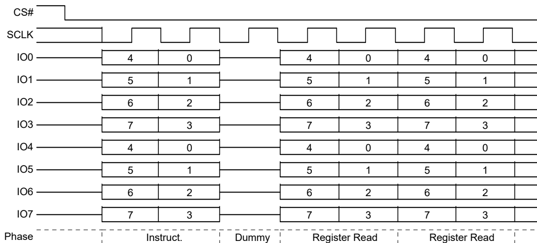
Figure 45. SPI DLP Read (DLPRD) Command Sequence – QPI Mode
