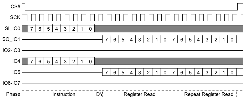
Figure 95. SPI IRPRD Command Sequence
