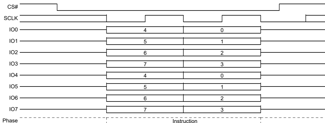
Figure 110. SPI Software / Mode Bit Reset Command Sequence – QPI Mode
