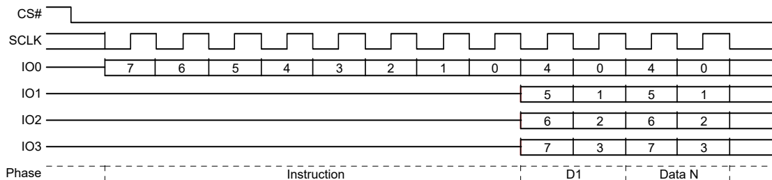
Figure 21. Read Quad Identification (RDQID) Command Sequence Quad Mode
