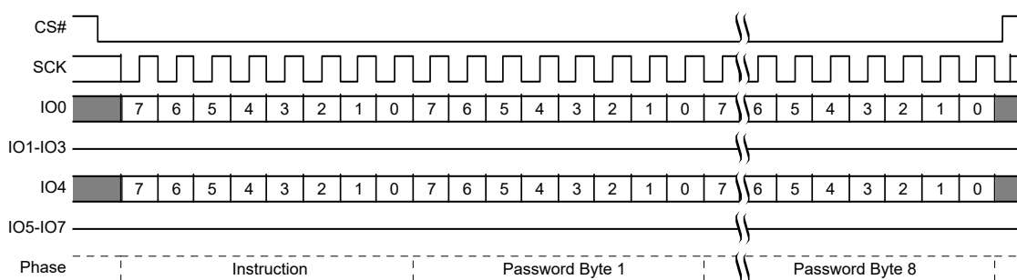
Figure 105. Password Program (PASSP) Command Sequence
