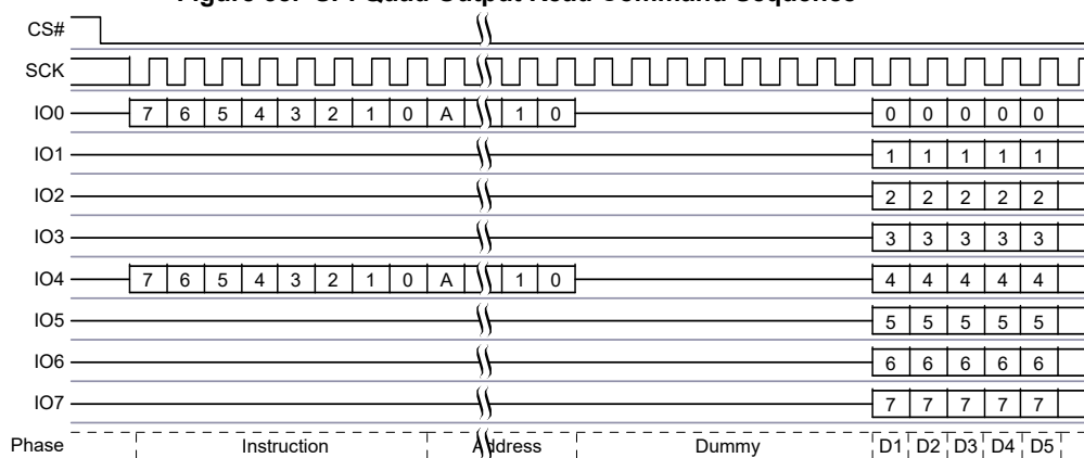
Figure 58. SPI Quad Output Read Command Sequence [34]
