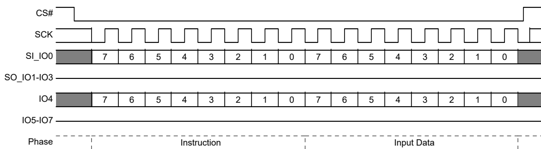
Figure 40. SPI Program DLRNV (PDLRNV) Command Sequence
