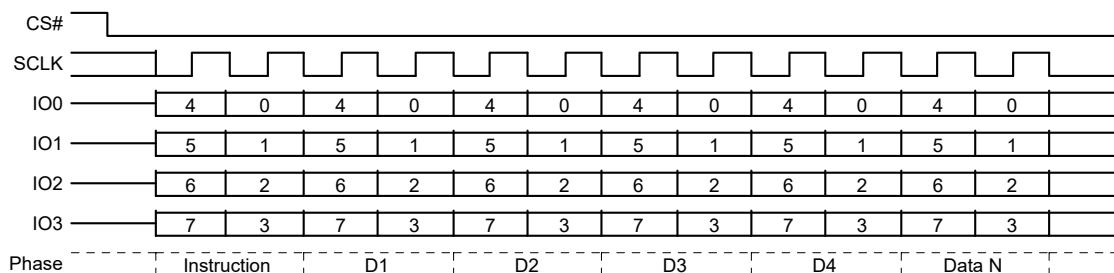
Figure 20. Read Quad Identification (RDQID) Command Sequence QPI Mode
