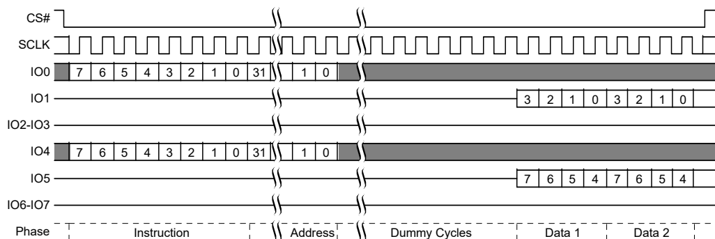
Figure 9. SPI Single Bit Wide I/O Command with Latency [6]
