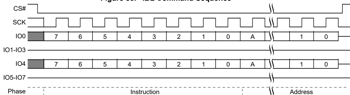
Figure 85. IBL Command Sequence [51, 52]
