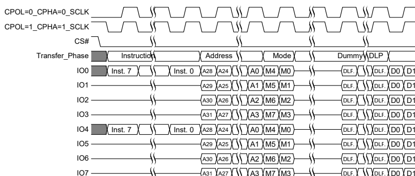
Figure 5. SPI DDR Modes Supported
