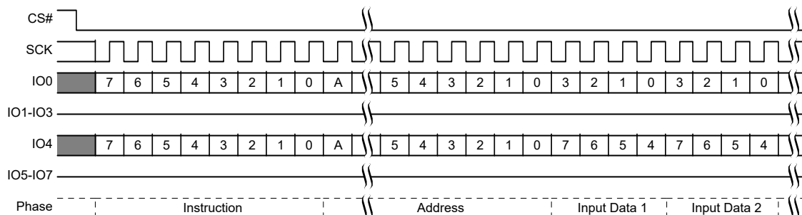
Figure 65. SPI Page Program (PP 02h or 4PP 12h) Command Sequence [41]
