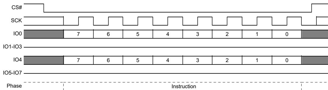
Figure 111. SPI Deep Power Down (DPD) Command Sequence
