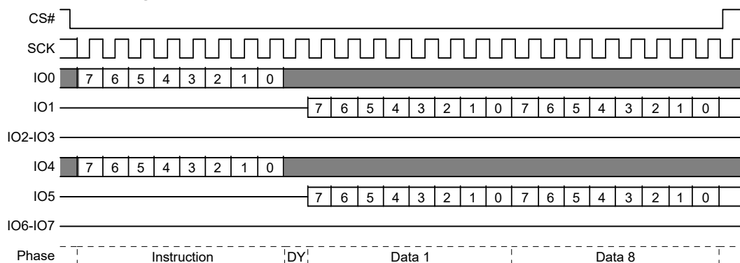
Figure 103. SPI Password Read (PASSRD) Command Sequence
