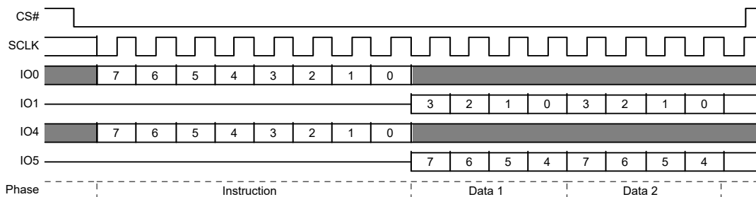
Figure 8. SPI Single Bit Wide Output Command without Latency [6]
