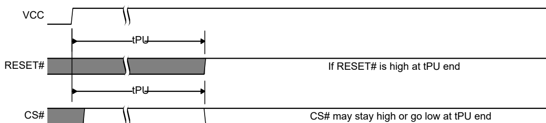
Figure 123. Reset high at the end of POR
