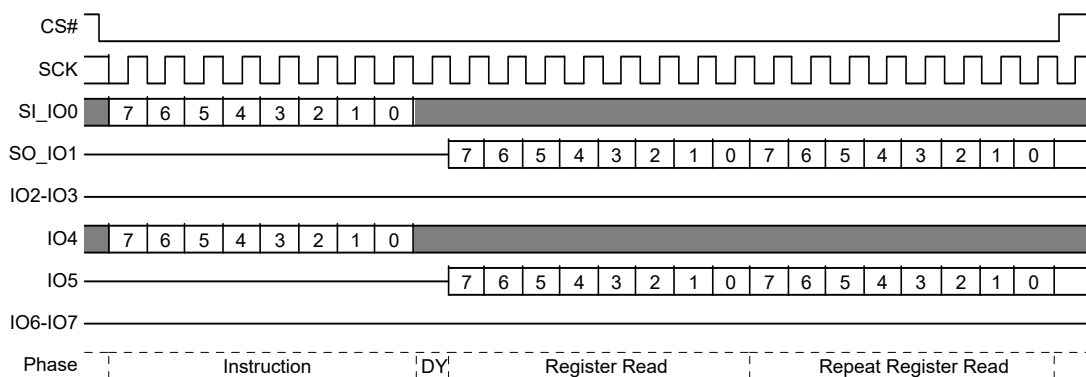
Figure 99. SPI Protection Register Read (PRRD) Command Sequence
