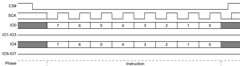
Figure 6. SPI Stand Alone Instruction Command [6]
