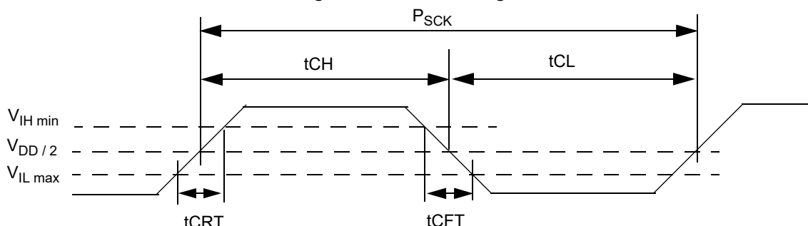
Figure 126. Clock Timing
