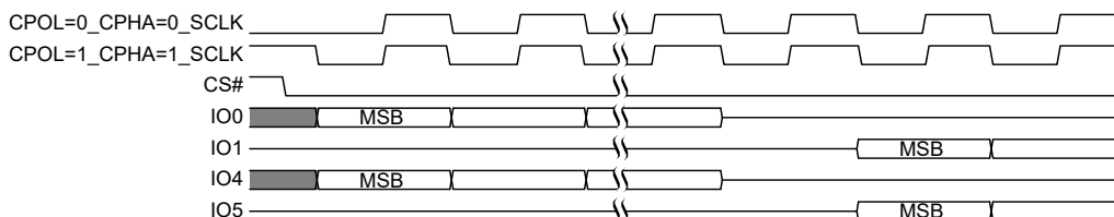
Figure 4. SPI SDR Modes Supported
