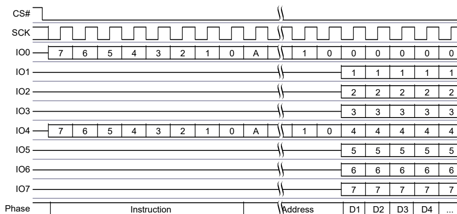
Figure 67. SPI, Quad Page Program Command Sequence [43]
