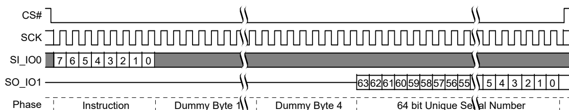
Figure 24. Read Unique ID (RUID) Command Sequence
