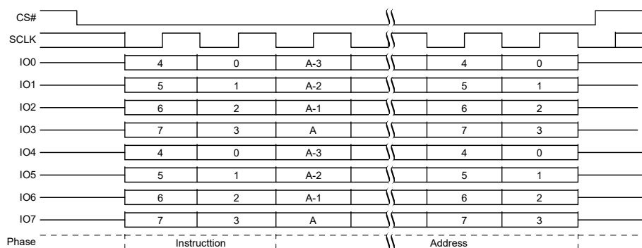
Figure 73. Block Erase (BE D8h or 4BE DCh) QPI Mode Command Sequence [46]
