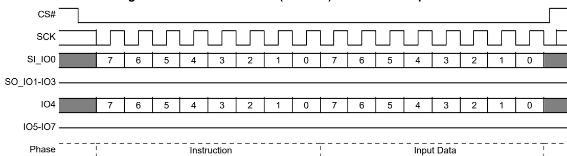
Figure 42. SPI Write DLRV (WDLRV) Command Sequence
