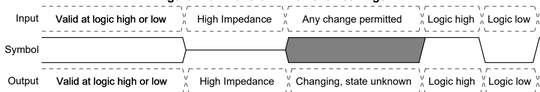
Figure 119. Waveform Element Meanings
