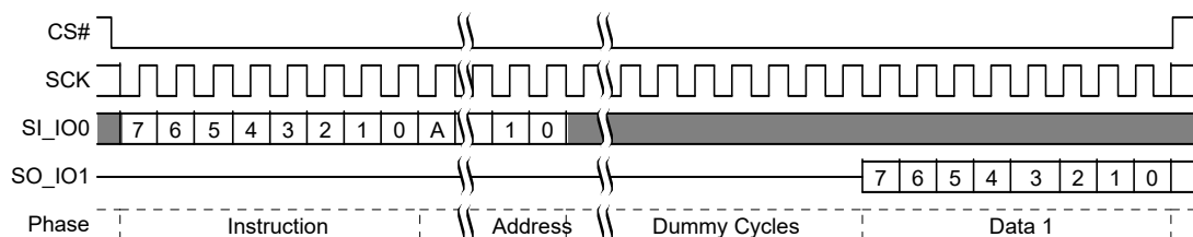
Figure 22. RSFDP Command Sequence [30]
