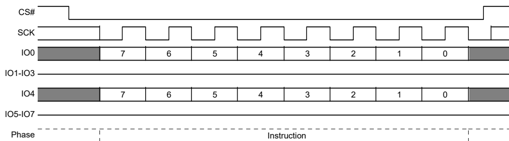
Figure 54. SPI Enter QPI Mode (QPIEN 38h) Command Sequence
