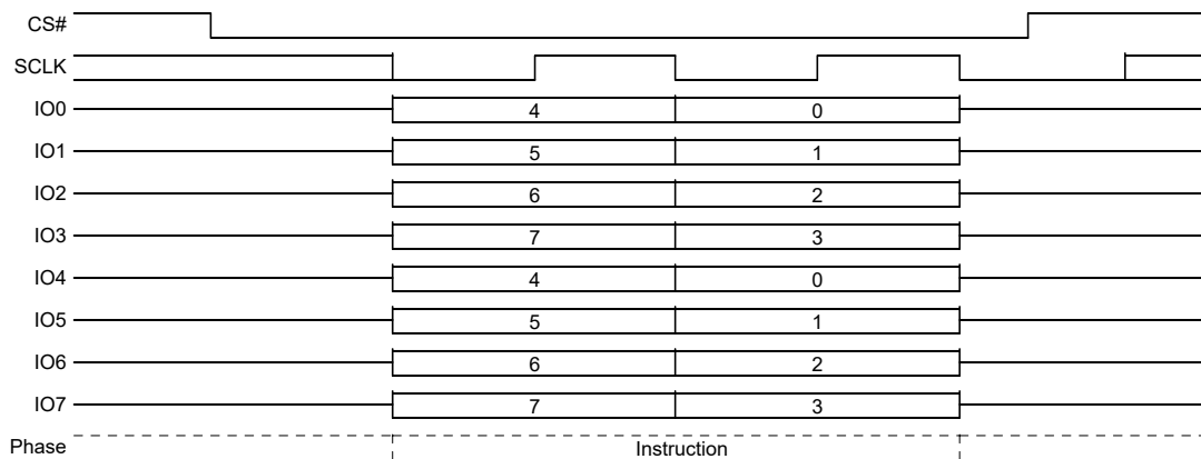
Figure 37. SPI Write Enable for Volatile Registers (WRENV) Command Sequence QPI Mode
