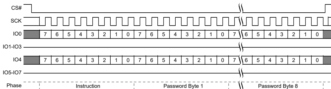
Figure 107. Password Unlock (PASSU) Command Sequence
