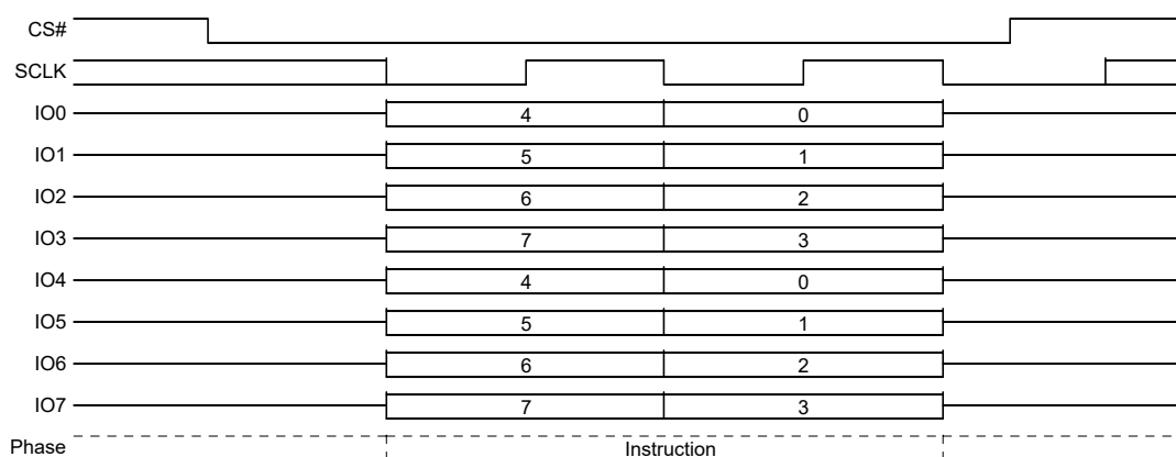
Figure 80. Erase or Program Resume command Sequence QPI Mode
