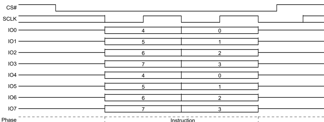
Figure 47. Enter 4 Byte Address QPI Mode
