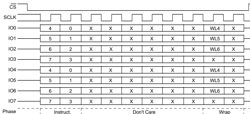
Figure 53. SPI Set Burst Length Command Sequence QPI Mode
