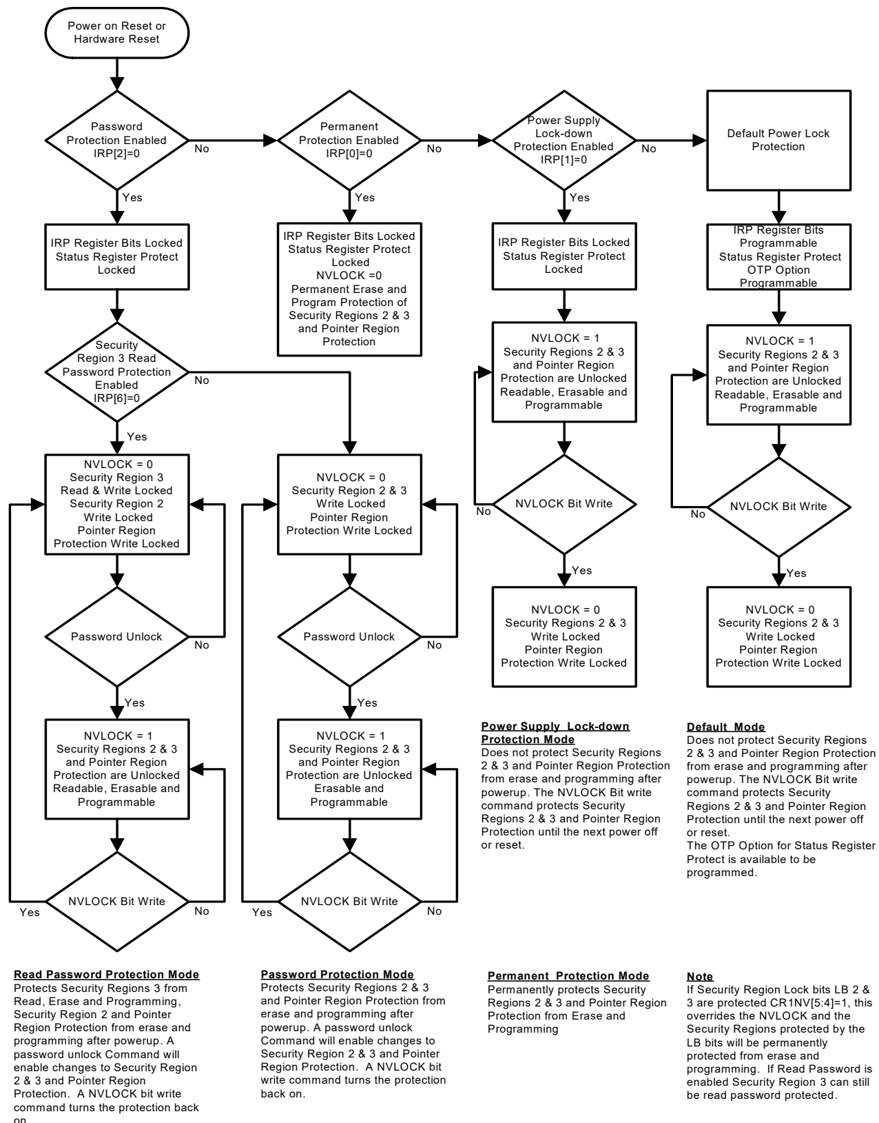
Figure 17. Permanent, Password and Power Supply Lock-down Protection Overview
