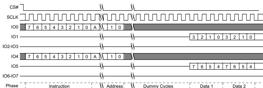
Figure 81. SPI Security Regions Read Command Sequence [48]
