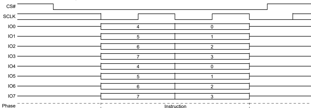
Figure 55. SPI Exit QPI (QPIEX F5h) Command Sequence
