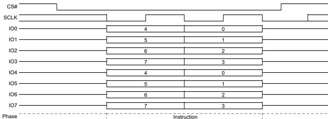
Figure 39. SPI Clear Status Register (CLSR) QPI Mode
