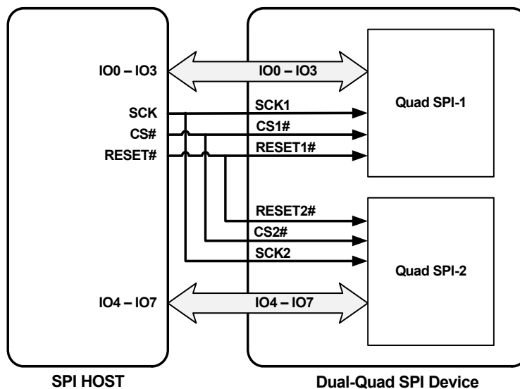
Figure 3. SPI Host and SPI Device with Dual CS#, SCK and RESET# [4, 5]
