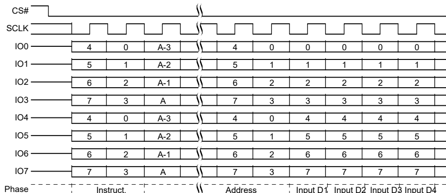
Figure 66. SPI Page Program (PP 02h or 4PP 12h) QPI Mode Command Sequence [42]
