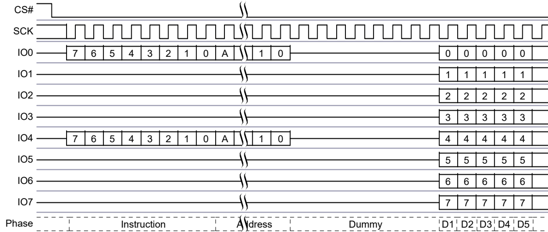
Figure 10. SPI, Quad Output Read Command
