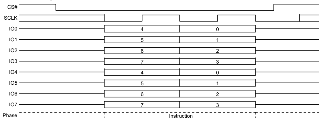
Figure 92. SPI Global IBL Unlock (GBUL) Command Sequence QPI Mode
