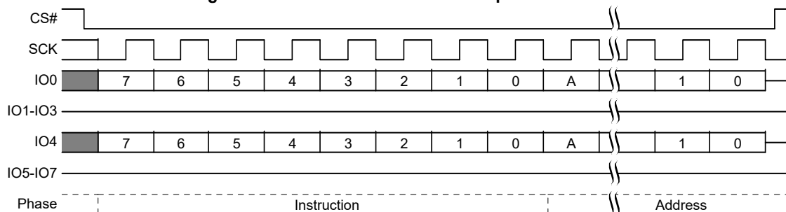
Figure 93. SPRP SPRP Command Sequence [55, 56]
