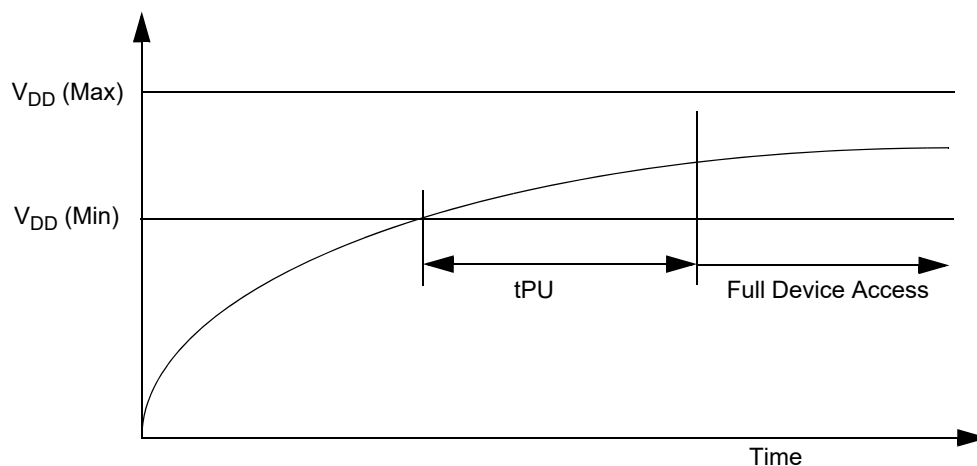
Figure 117. Power-up
