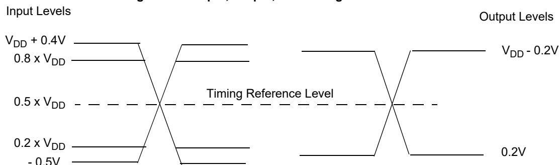
Figure 121. Input, Output, and Timing Reference Levels
