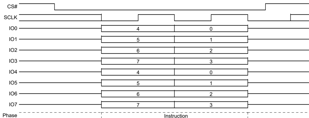
Figure 112. SPI Deep Power Down (DPD) Command Sequence – QPI Mode
