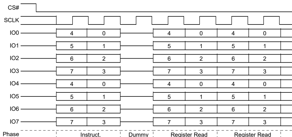
Figure 100. SPI Protection Register Read (PRRD) Command Sequence – QPI Mode
