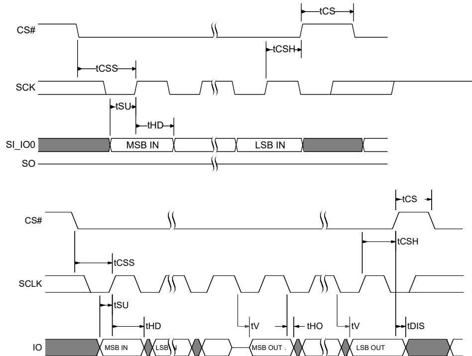
Figure 127. SDR MIO Timing
