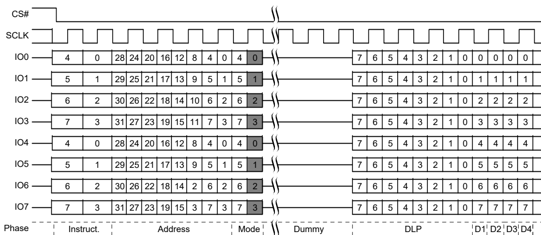
Figure 14. SPI DDR Quad I/O Read Command QPI Mode [9, 10]
