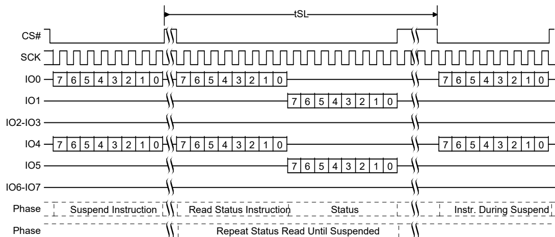
Figure 78. Program or Erase Suspend Command with Continuing Instruction Commands Sequence
