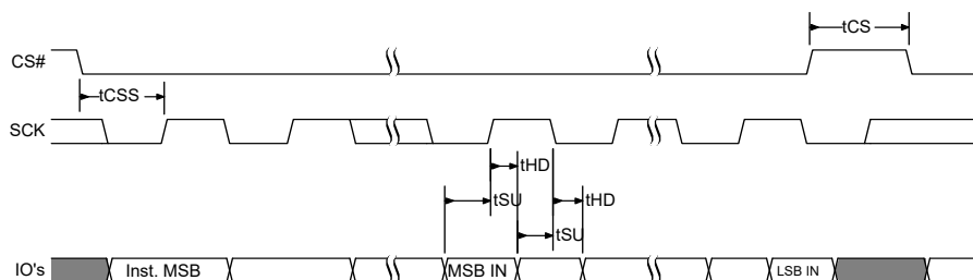
Figure 128. SPI DDR Input Timing
