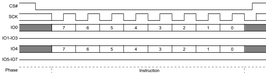
Figure 38. SPI Clear Status Register (CLSR) Command Sequence
