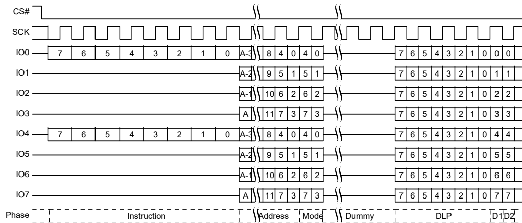
Figure 62. SPI DDR Quad I/O Read Initial Access [37, 38]
