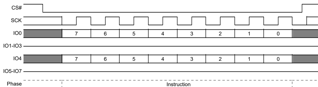
Figure 91. SPI Global IBL Unlock (GBUL) Command Sequence
