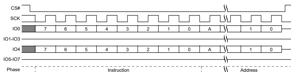
Figure 70. Half Block Erase (HBE 52h or 4HBE 53h) Command Sequence [45]
