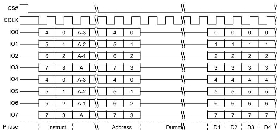
Figure 82. SPI Security Regions Read Command Sequence QPI Mode [48]
