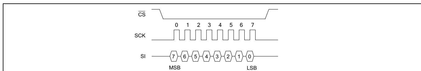
Figure 4 SPI mode 0
