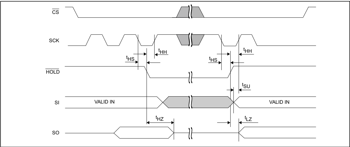
Figure 17 HOLD timing
