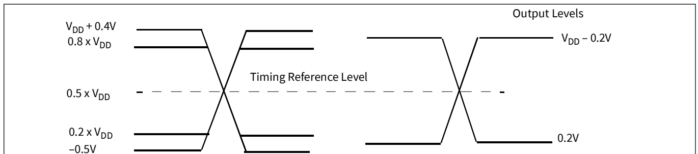
Figure 86 Input, output, and timing reference levels [26]
