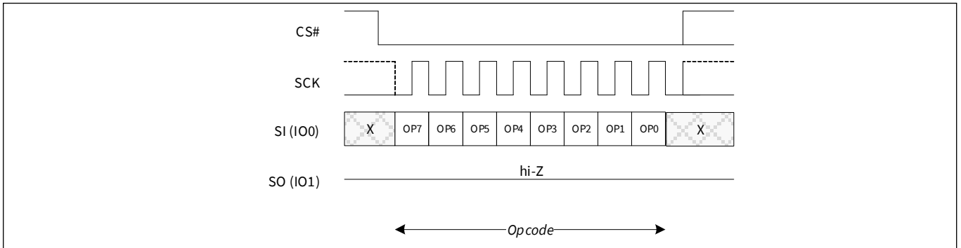
Figure 66 Chip Scrub (CSCR8 8Eh) command sequence
