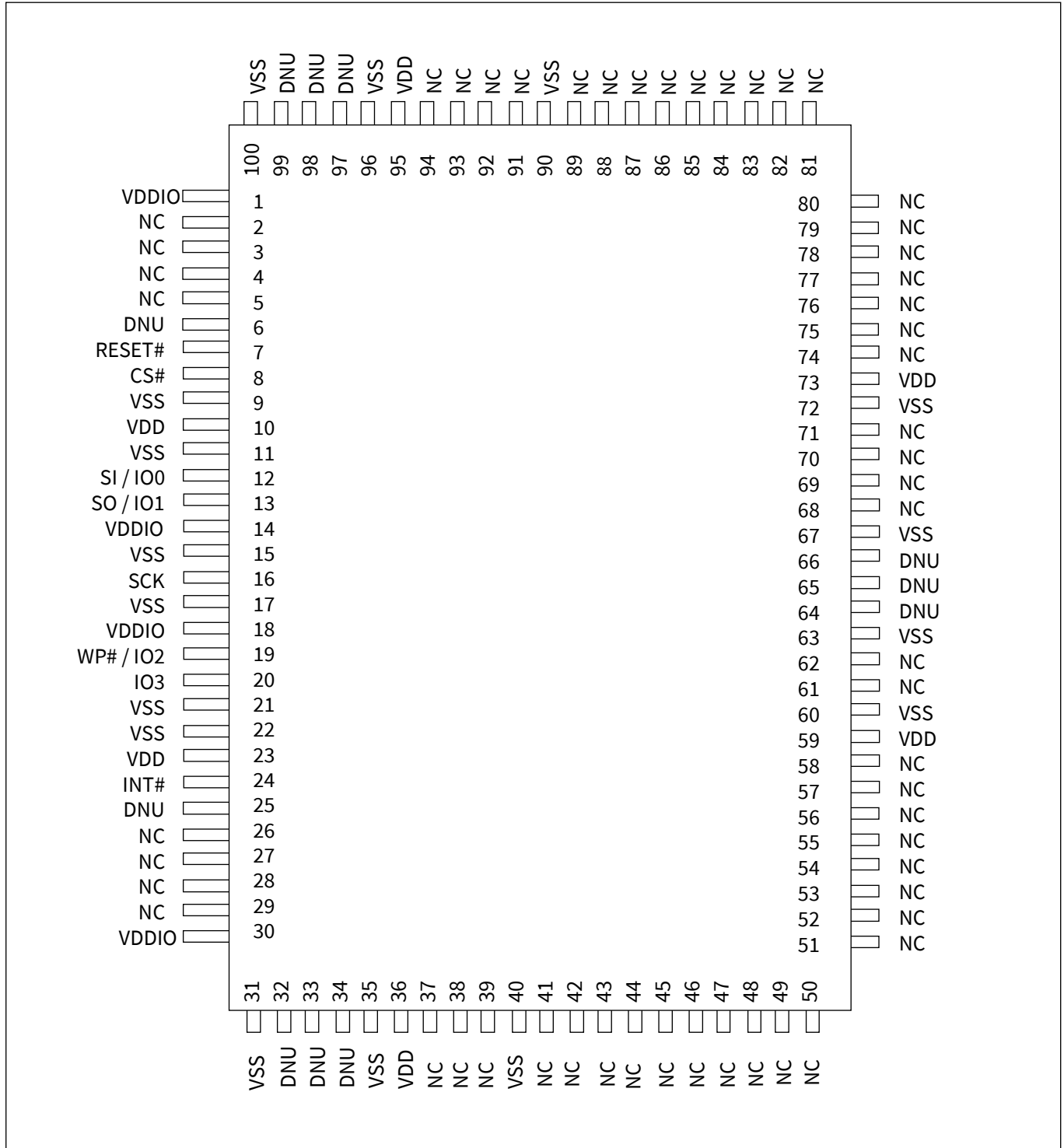
Figure 1 100-lead thin quad flatpack (100TQFP), top view
