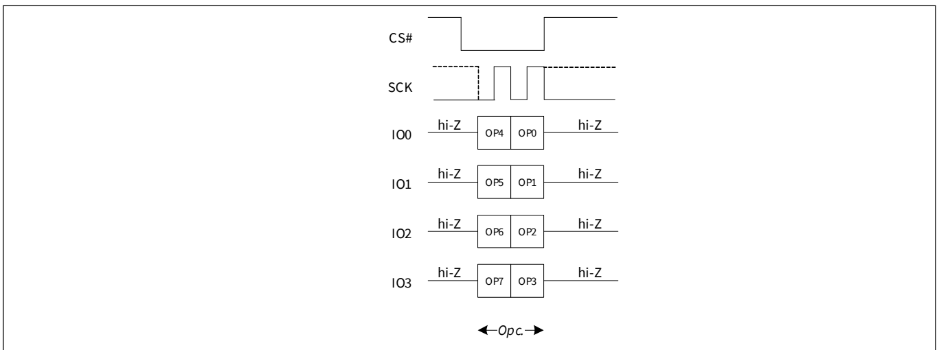
Figure 67 Chip Scrub (CSCR8 8Eh) QPI command sequence
