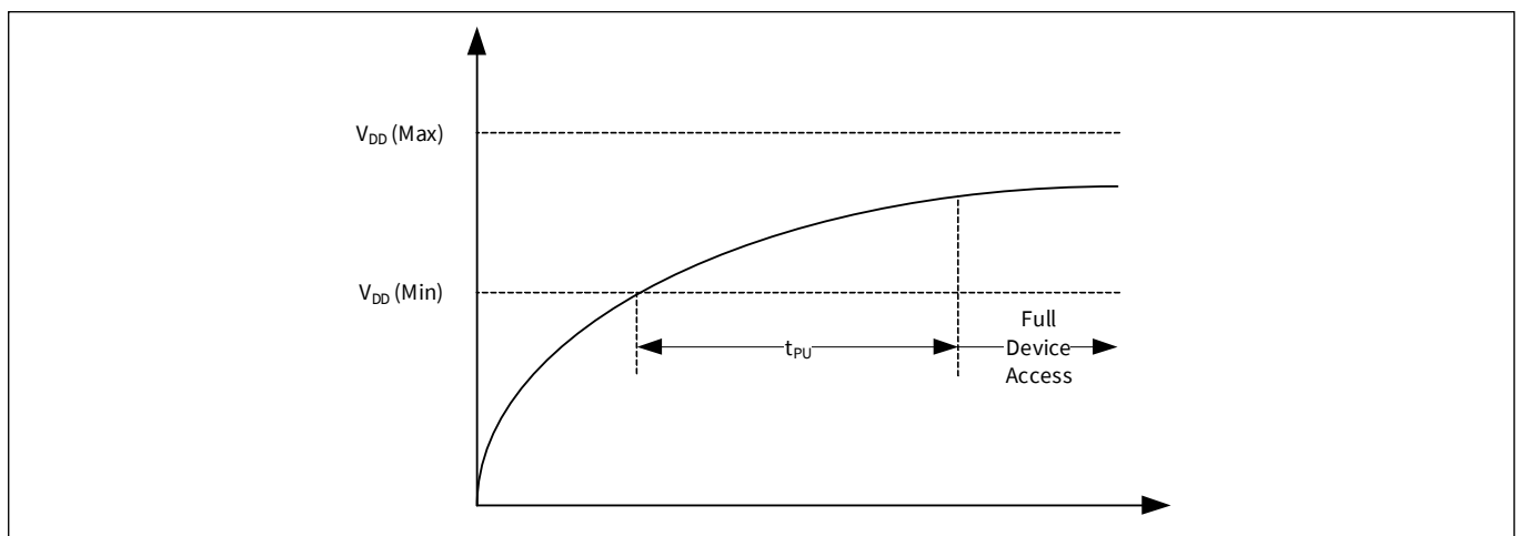
Figure 82 Power-up
