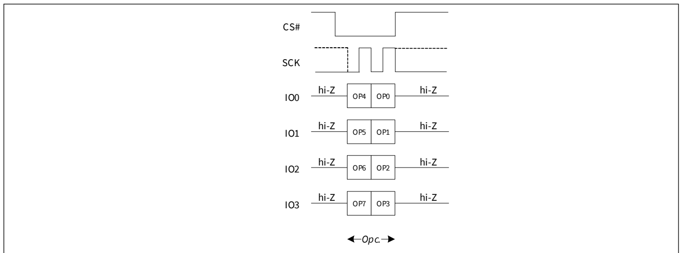
Figure 39 Clear Status Register (CLSR) QPI mode
