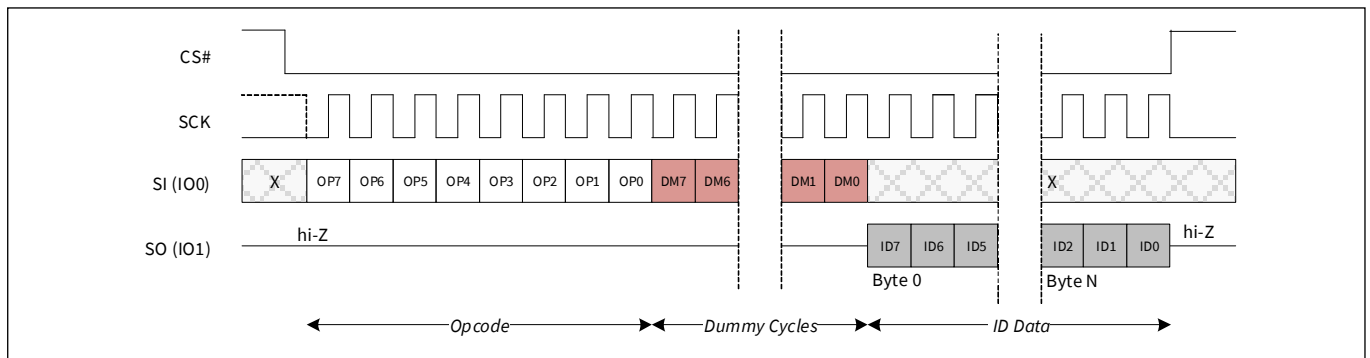
Figure 14 Read Identification (RDID) command sequence
