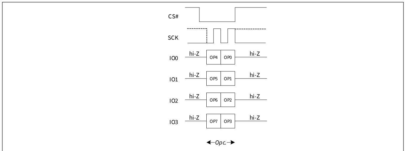
Figure 75 Erase Suspend command sequence QPI mode
