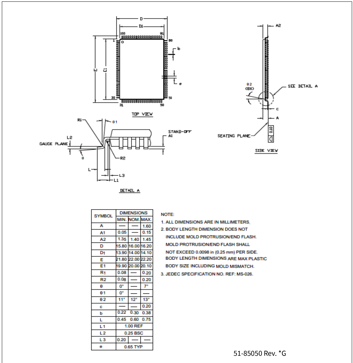
Figure 96 100-lead TQFP (14.0 × 20.0 × 1.4 mm) A100RA, (PG-TQFP-100)
