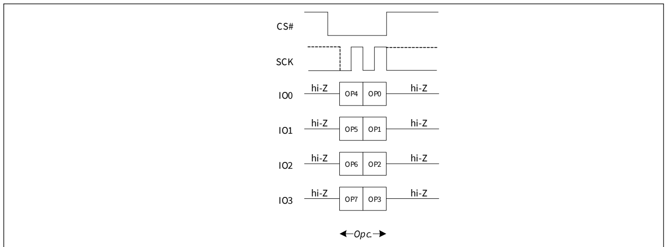
Figure 41 Enter 4-byte address QPI mode
