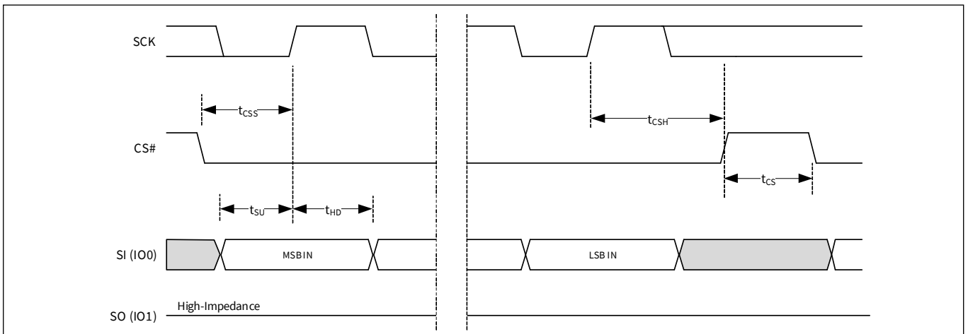
Figure 92 SPI single bit input timing
