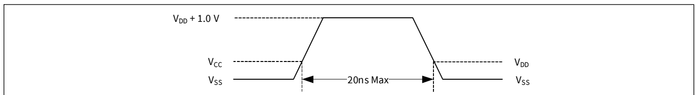
Figure 81 Maximum positive overshoot waveform
