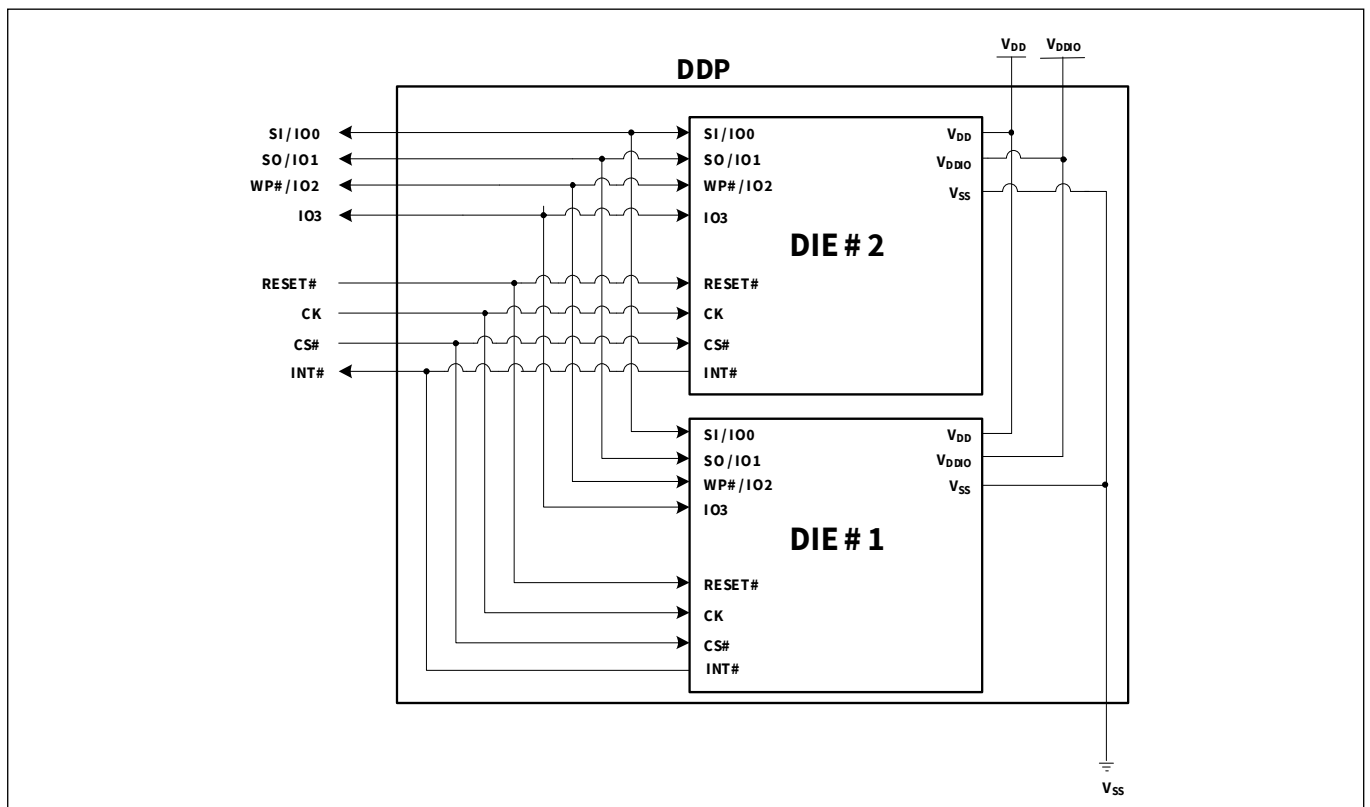
Figure 3 DDP diagram
