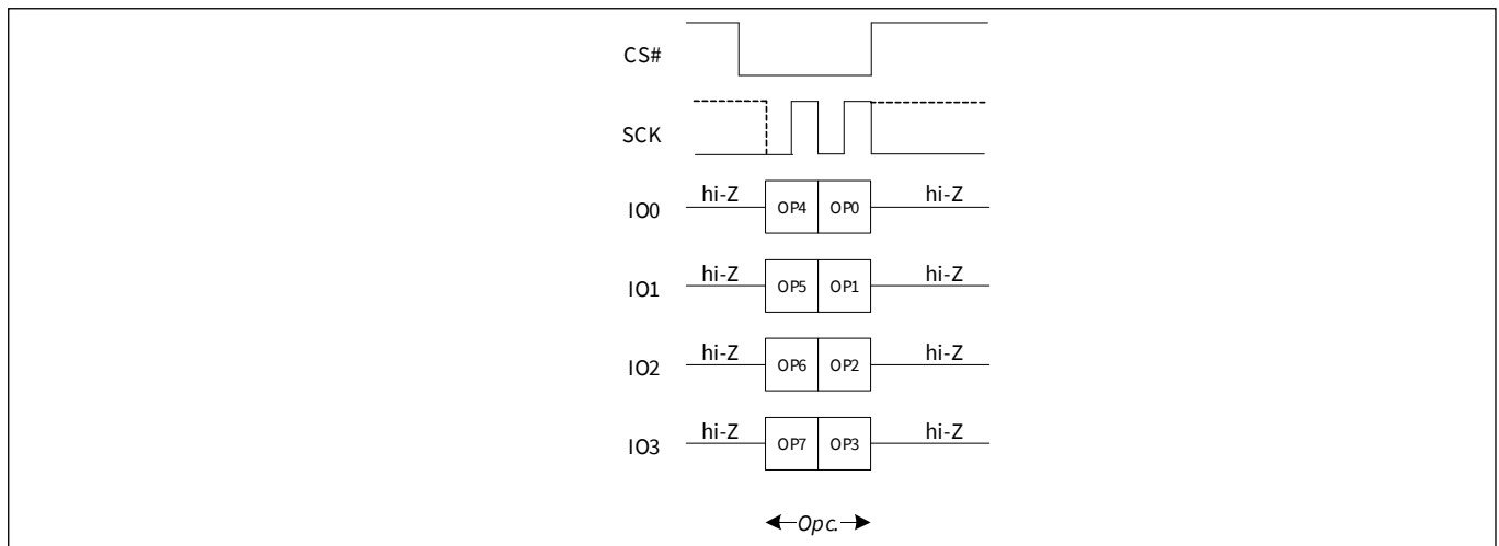
Figure 79 Software Reset/Mode Bit command sequence - QPI mode
