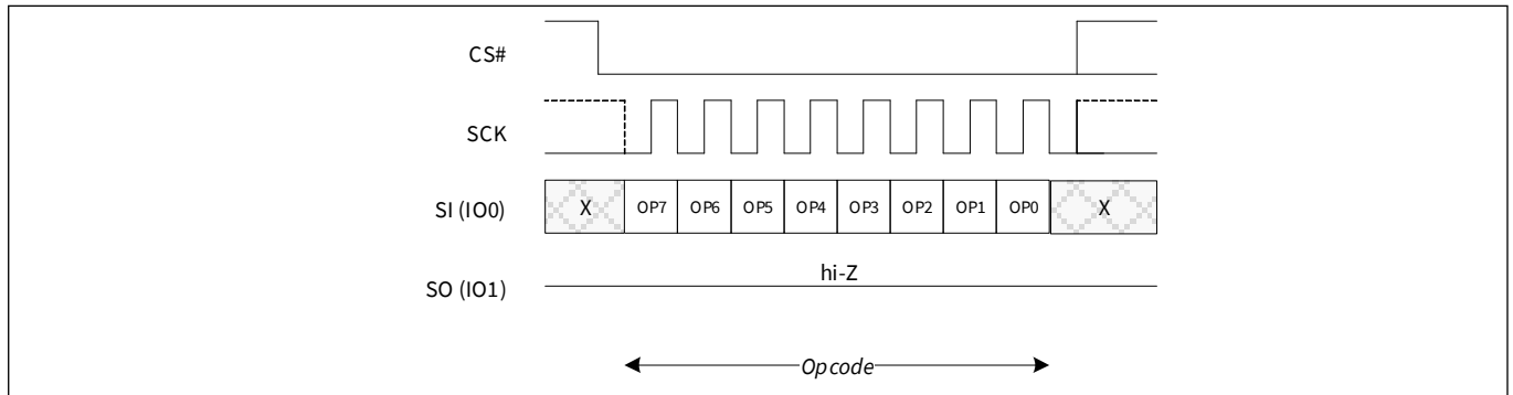
Figure 34 Write Enable (WREN) command sequence
