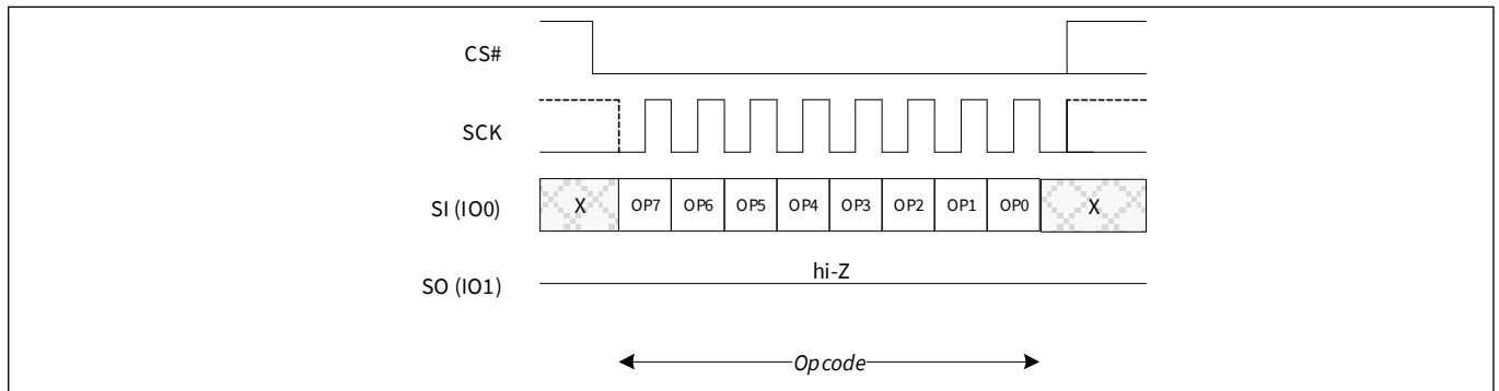
Figure 48 Enter QPI mode (QPIEN 38h) command sequence
