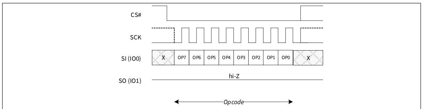
Figure 72 Chip Erase command sequence
