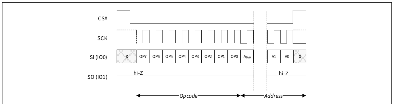
Figure 68 Sector Erase (SE 20h or 4SE 21h) command sequence [13]
