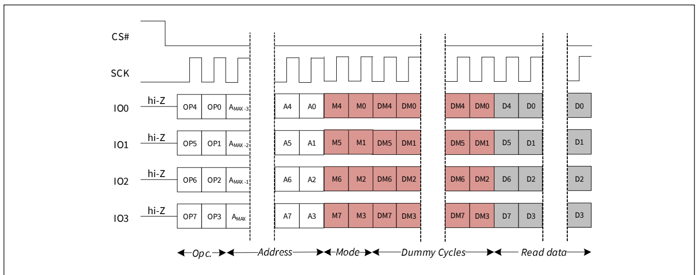
Figure 59 Quad I/O Read Initial Access command sequence QPI mode [7]
