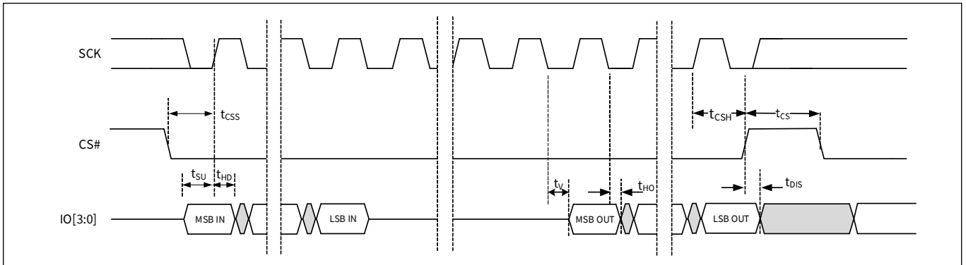
Figure 94 Quad/QPI timing
