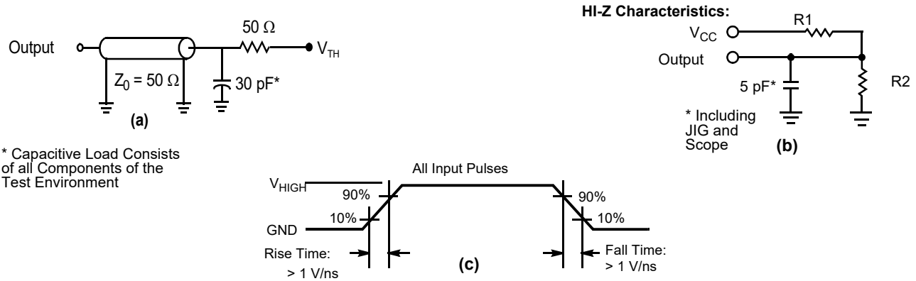
Figure 5. AC Test Loads and Waveforms [15]
