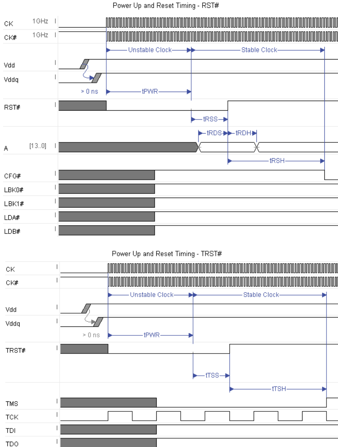
Figure 16. Reset Timings
