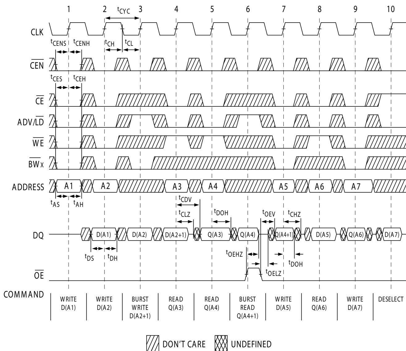
Figure 5. Read/Write Timing [24, 25, 26]
