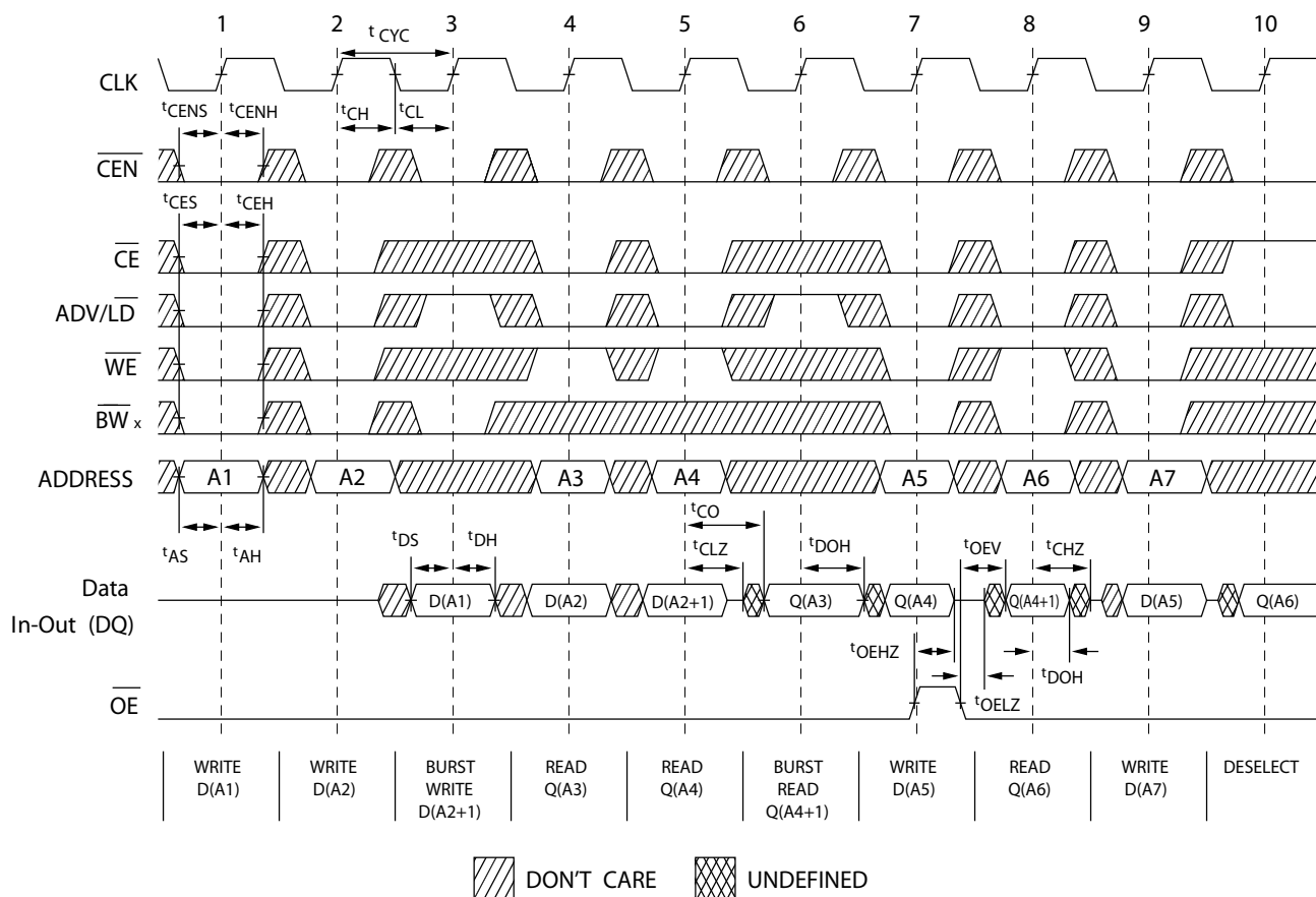
Figure 5. Read/Write Timing [25, 26, 27]
