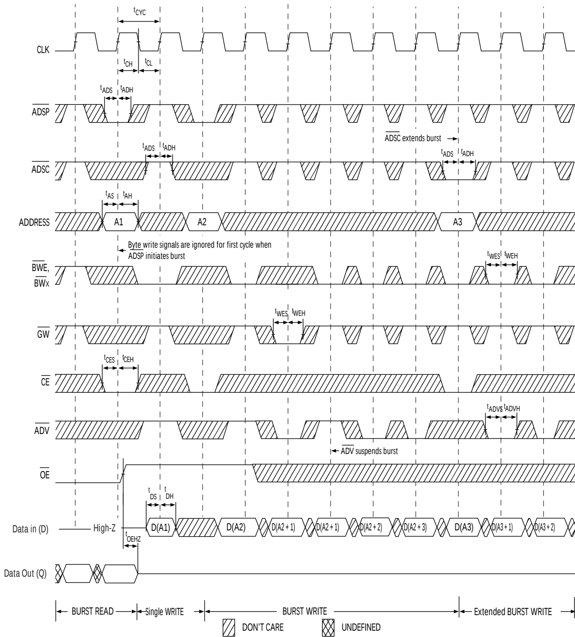
Figure 4. Write Cycle Timing [17, 18]
