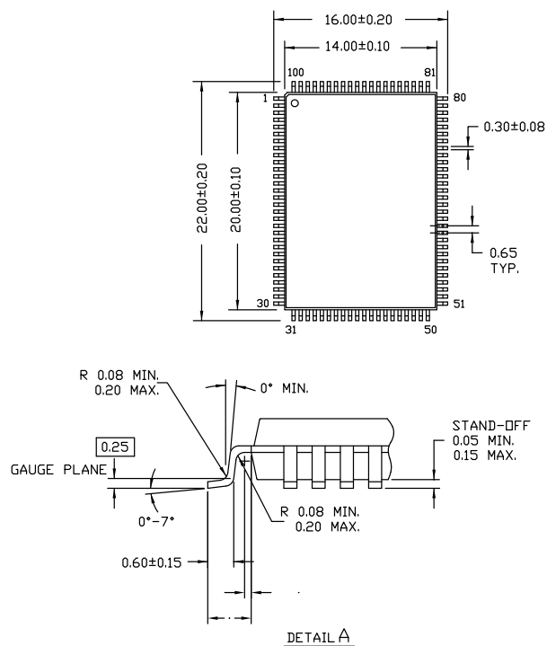
图 7. 100-TQFP (14 × 20 × 1.4 mm) A100RA 封装外形, 51-85050
