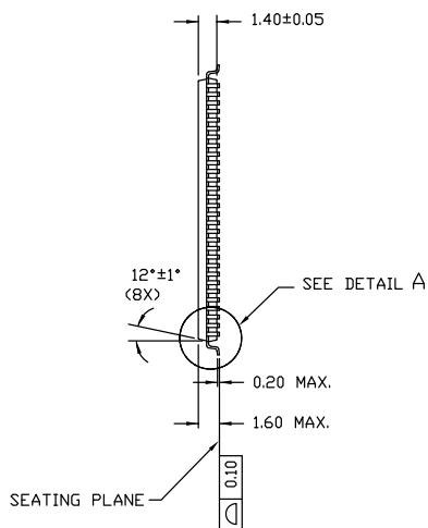
图 7. 100-TQFP (14 × 20 × 1.4 mm) A100RA 封装外形, 51-85050
