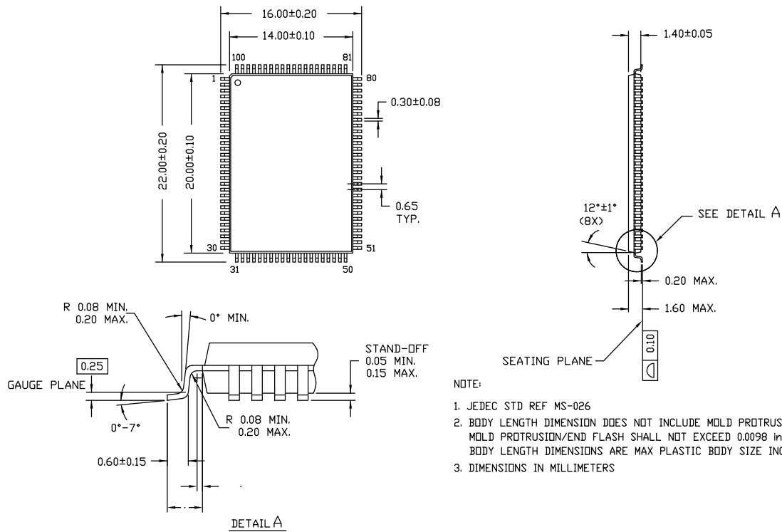
图 8. 100-TQFP (14 × 20 × 1.4 mm) A100RA 封装外形, 51-85050
