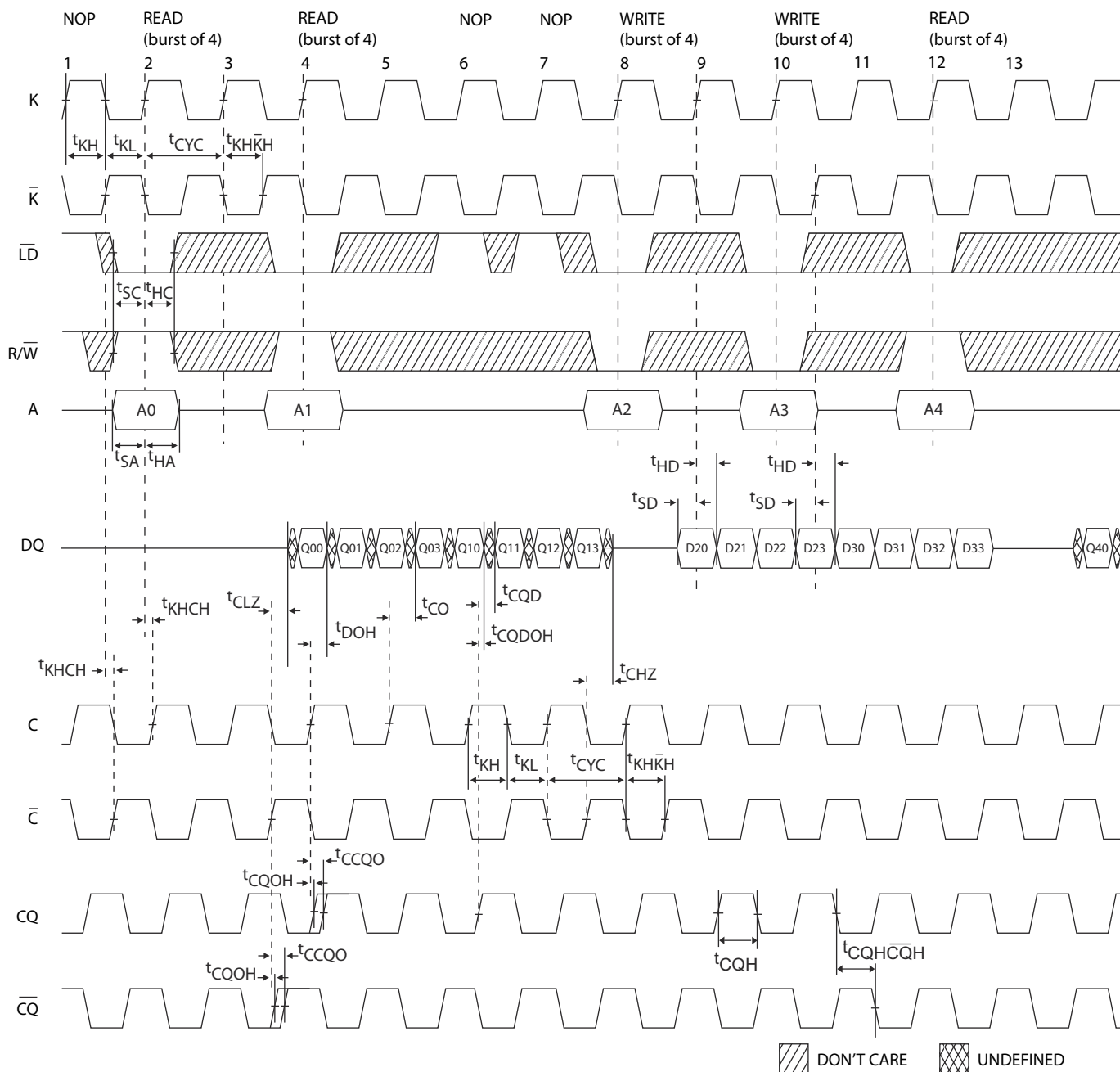
Figure 6. Read/Write/Deselect Sequence [37, 38, 39]
