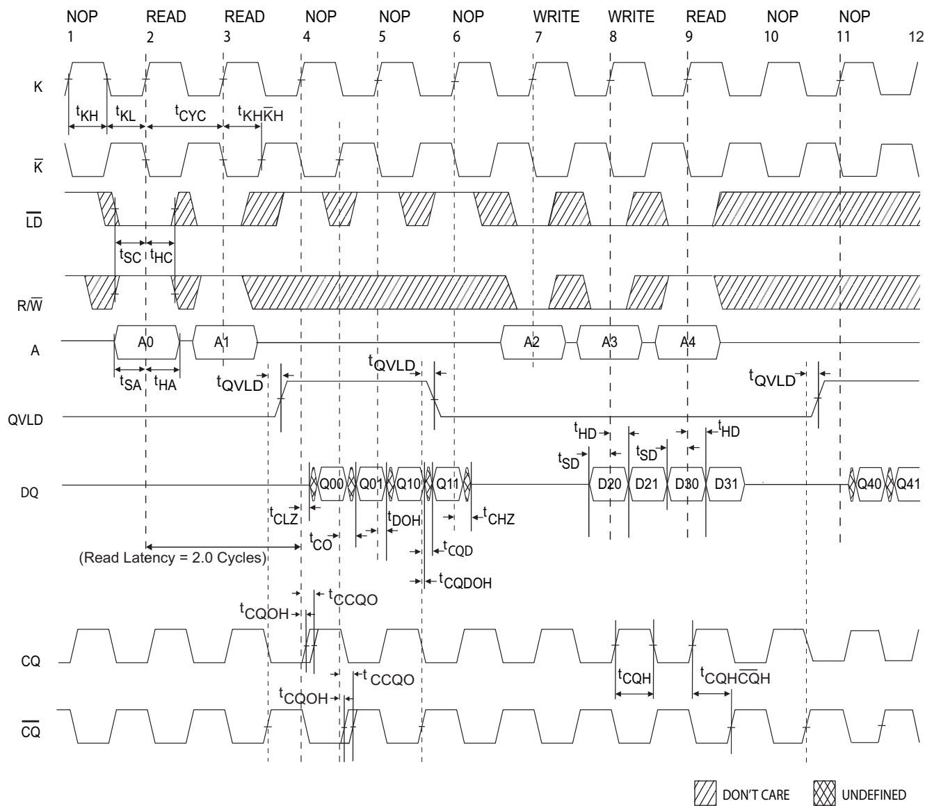
Figure 6. Waveform for 2.0 Cycle Read Latency [35, 36, 37, 38]
