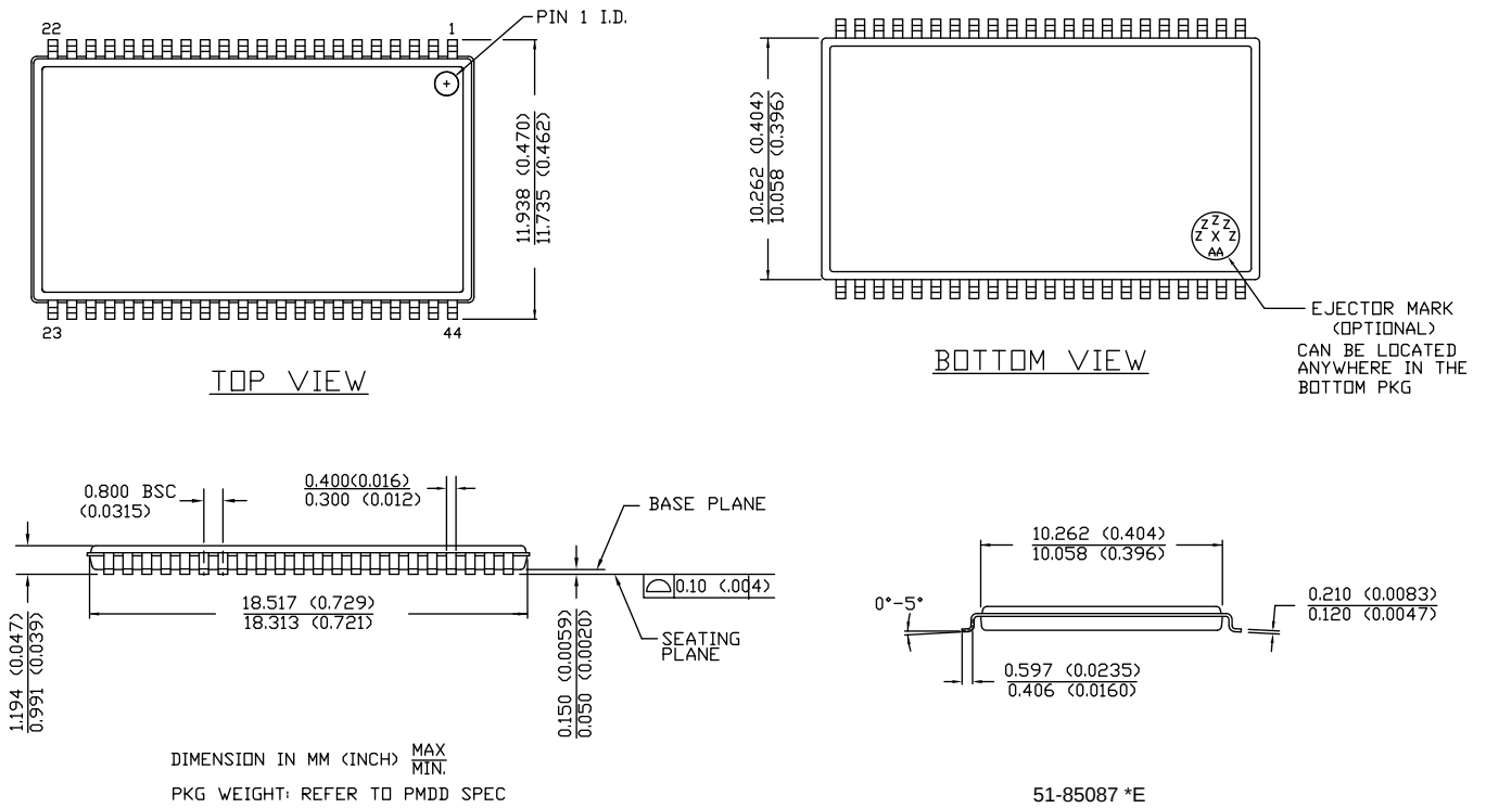
图 10. 44-TSOP Z44-II 封装外形 — 51-85087
