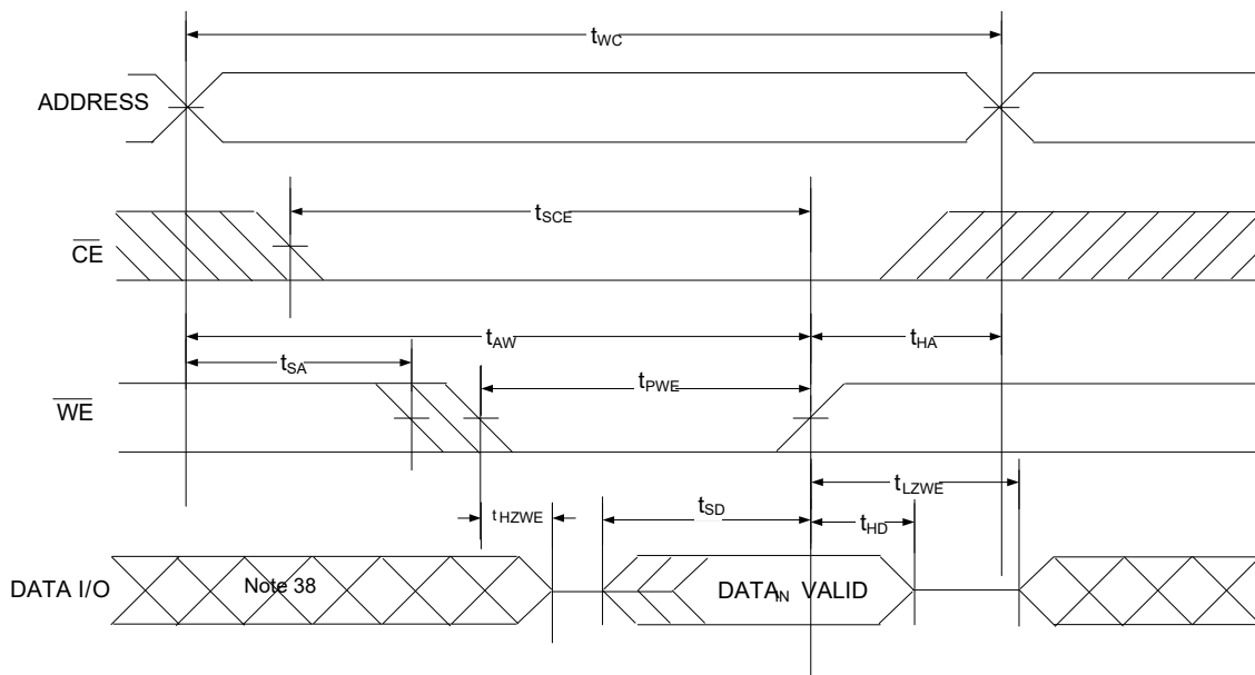
Figure 10. Write Cycle No. 3 ( \overline{CE} Controlled) [34, 35, 36]
