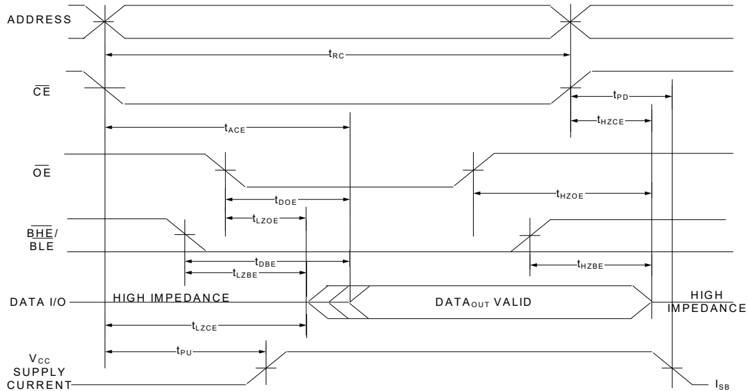
Figure 10. Read Cycle No. 2 ( \overline{\text{OE}} Controlled) [37, 38, 39, 41]
