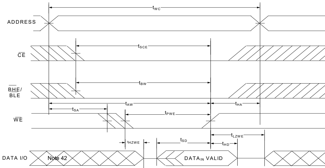
Figure 11. Write Cycle No. 1 ( \overline{\text{WE}} Controlled, \overline{\text{OE}} LOW) [38, 40, 41, 42]
