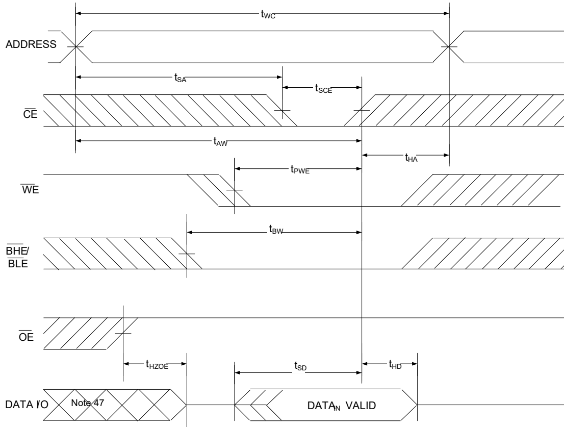
Figure 12. Write Cycle No. 2 ( \overline{\text{CE}} Controlled) [44, 45, 46]
