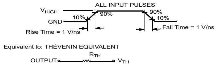
Figure 6. AC Test Loads and Waveforms
