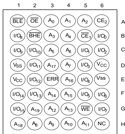
Figure 4. 48-ball VFBGA Pinout (Dual Chip Enable with ERR) – CY62167GE30 [8, 9]
