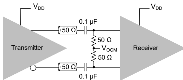
Figure 8. LVDS Termination for 1.8 V [14]
