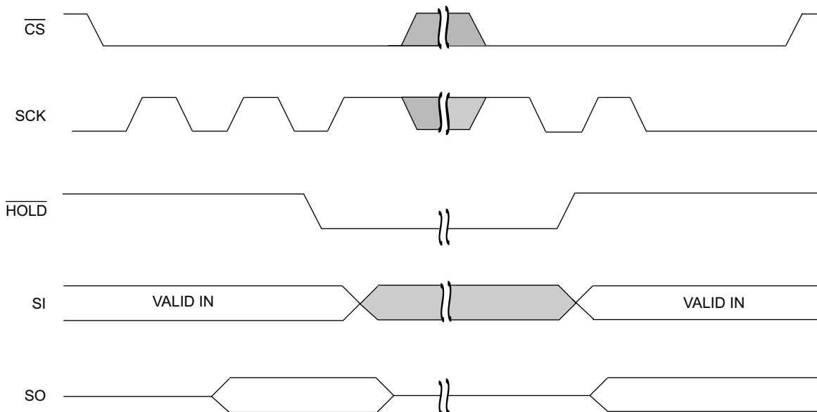
Figure 12. \overline{\text{HOLD}} Operation [2]
