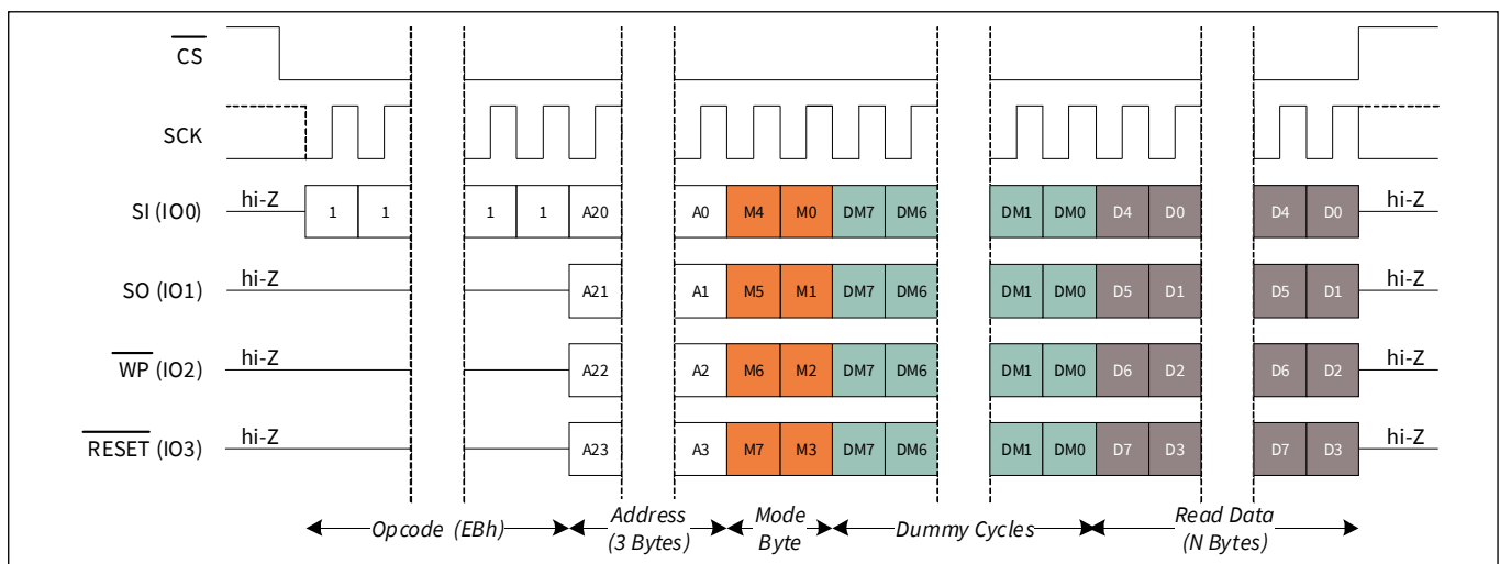
Figure 64 Quad I/O Read (QIOR) in Extended SPI mode
