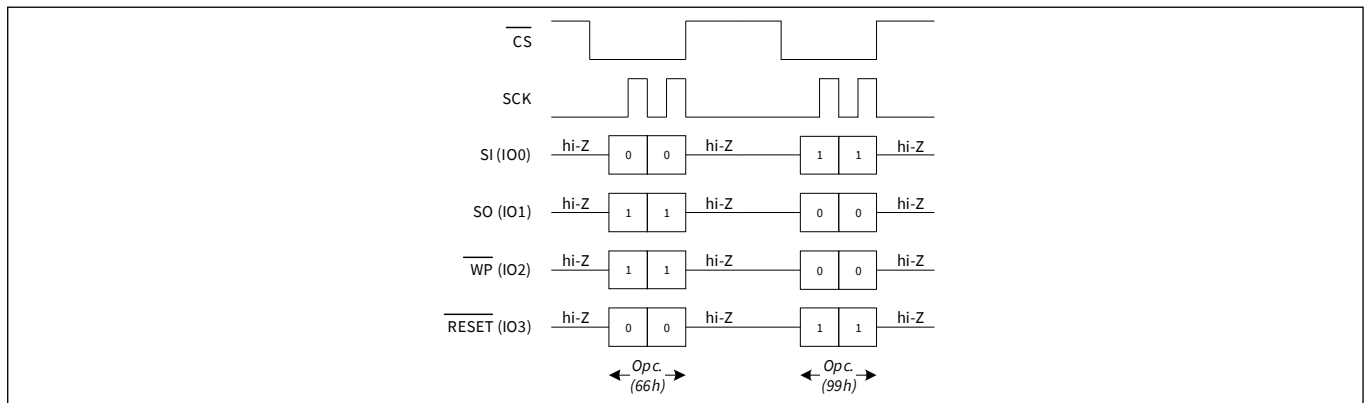
Figure 109 Software Reset timing in QPI mode
