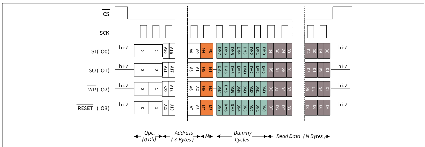
Figure 58 DDRFR in QPI mode
