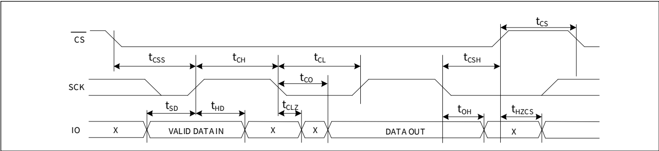
Figure 116 SPI switching timing - Multiple I/O, SDR
