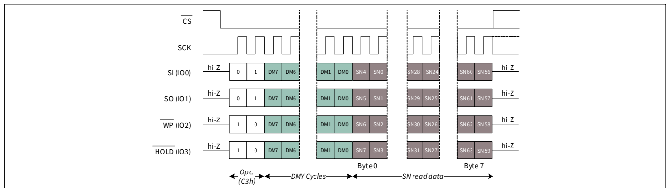
Figure 99 Read Serial Number (RDSN) in QPI mode
