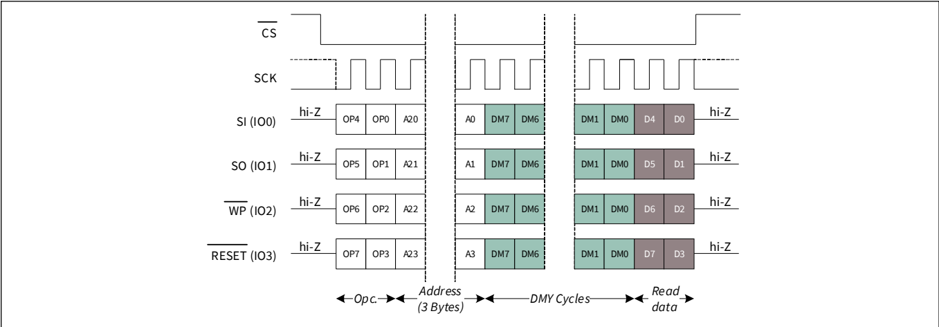
Figure 38 Read Any Register (RDAR) in QPI mode
