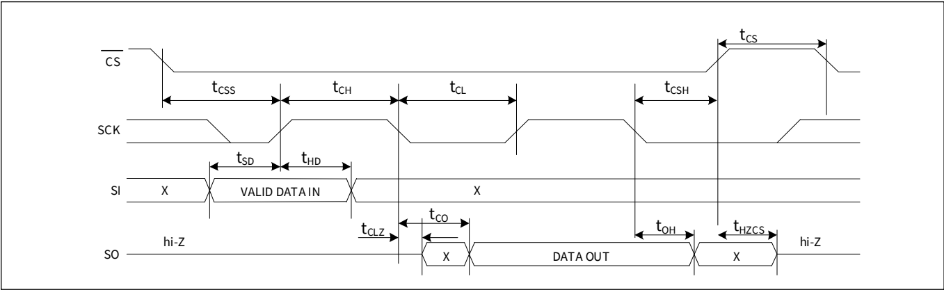
Figure 115 SPI switching timing - Single IO, SDR
