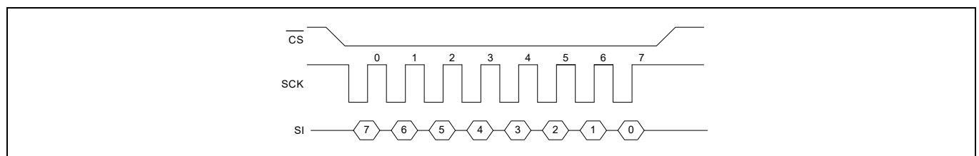
Figure 5 SPI Mode 3
