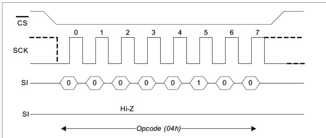
Figure 7 WRDI bus configuration
