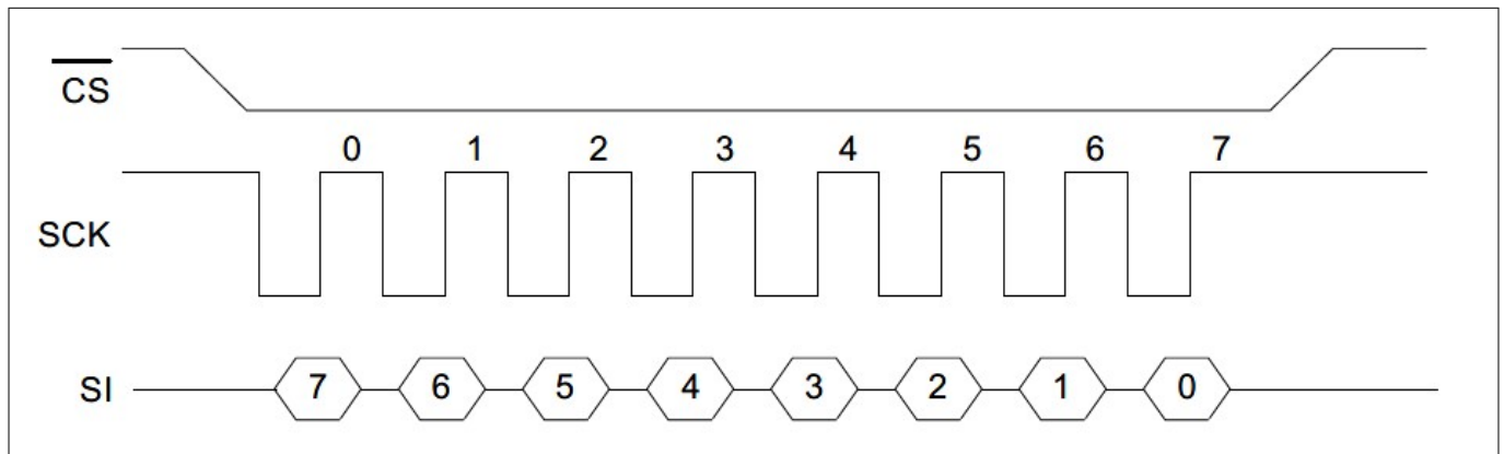
Figure 5 SPI mode 3
