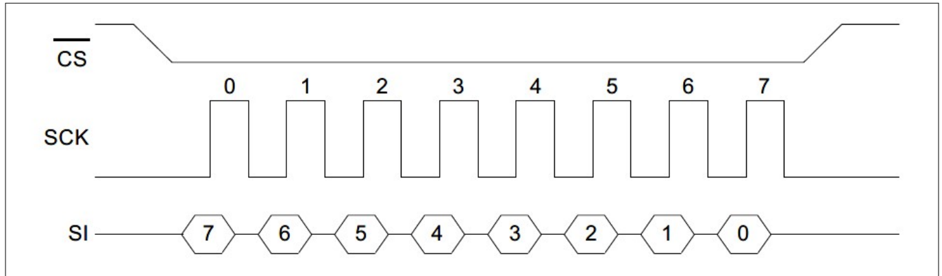
Figure 4 SPI mode 0
