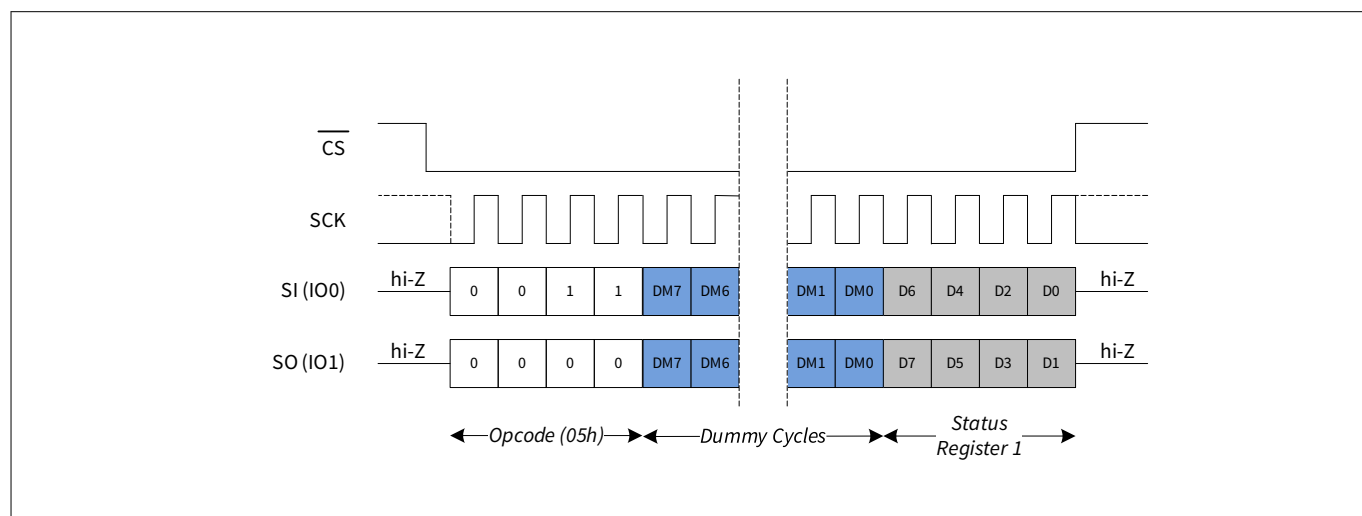
Figure 18 Read SR1 (RDSR1) in DPI mode
