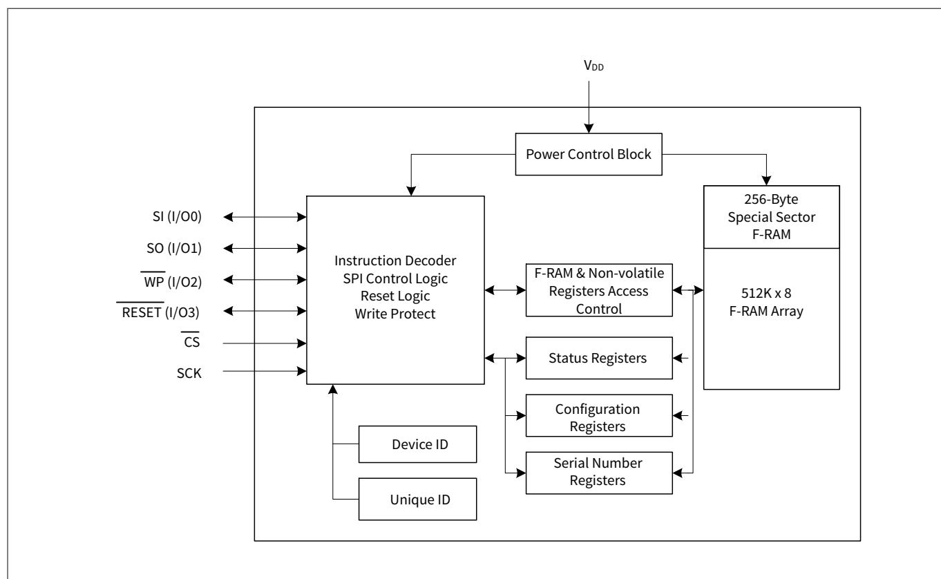
Figure 1 Block diagram
