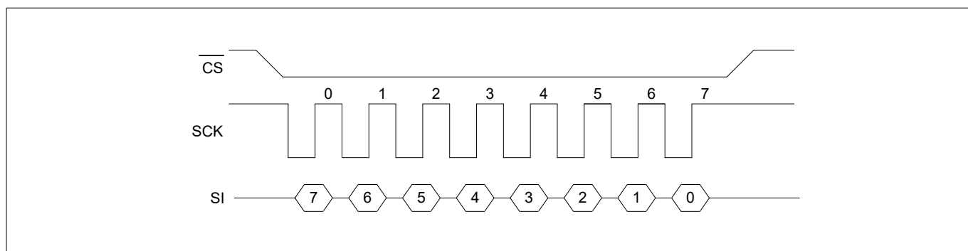
Figure 7 SPI mode 3
