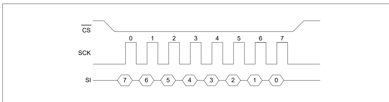
Figure 6 SPI mode 0
