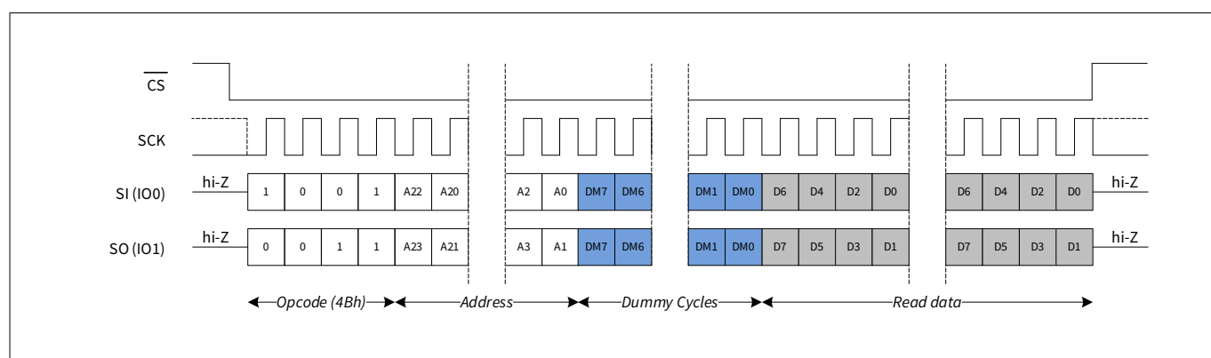
Figure 72 Special sector read (SSRD) in DPI mode
