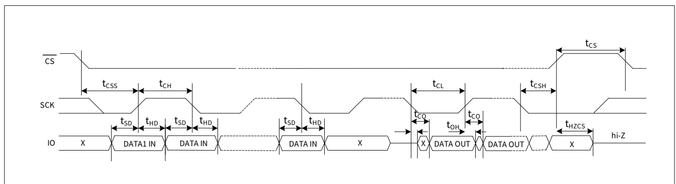
Figure 120 SPI switching timing - multiple I/O, DDR 2)
