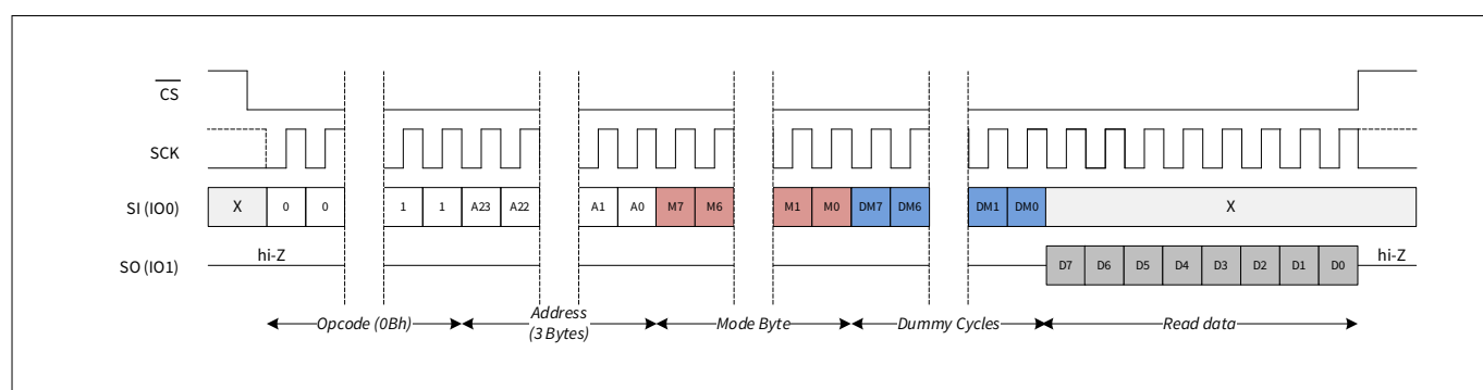
Figure 57 FAST_READ in SPI mode
