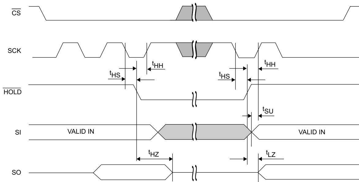
Figure 17. \overline{\text{HOLD}} Timing
