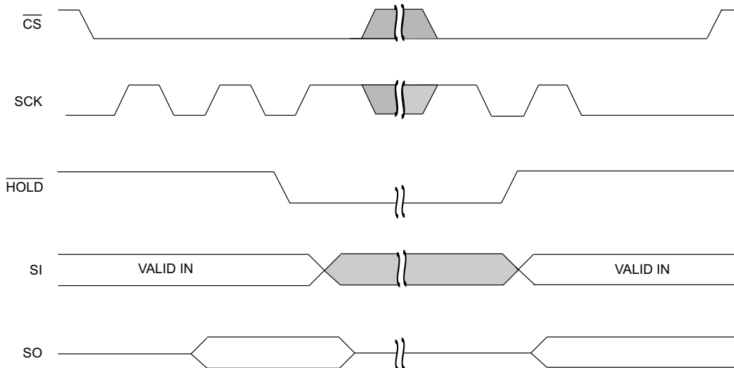
Figure 12. HOLD Operation [2]
