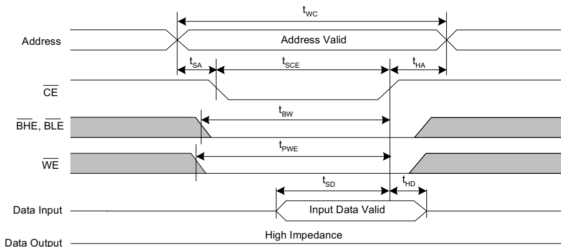
Figure 7. SRAM Write Cycle #2 ( \overline{\text{CE}} Controlled) [25, 26, 27, 28]
