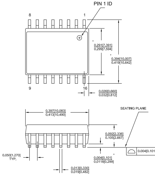
Figure 39. 16-pin SOIC (0.413 × 0.299 × 0.0932 Inches) Package Outline, 51-85022
