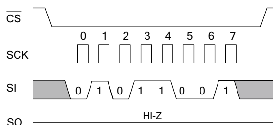
Figure 18. AutoStore Enable Operation
