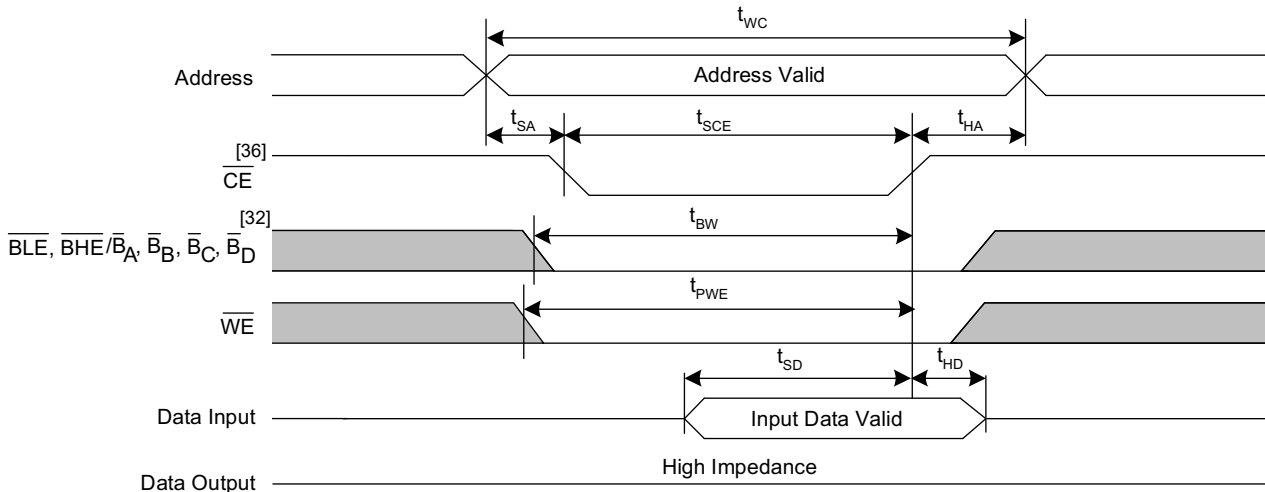
Figure 14. SRAM Write Cycle 2: \overline{\text{CE}} Controlled [33, 35, 37]
