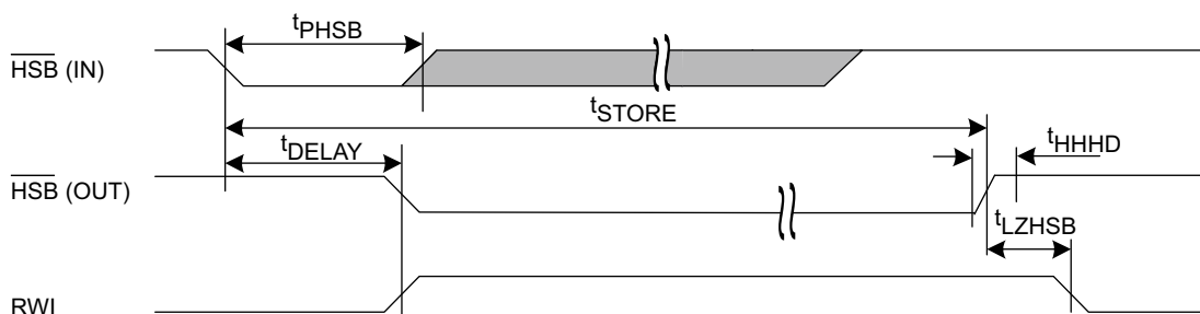
Figure 21. Hardware STORE Cycle [63]
