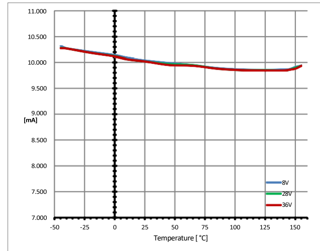
负载开路检测 ON 状态阈值 I_{L(OL)} = f(T_J)
