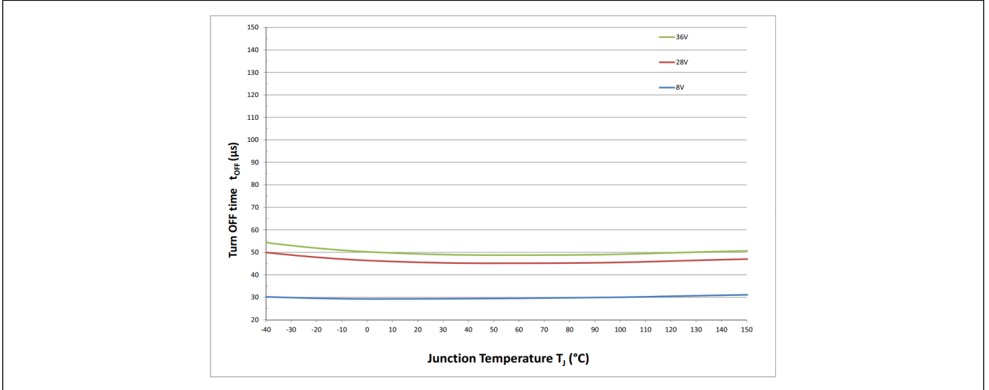
图39 关断 t_{OFF} = f(T_j; V_s) , R_L = 12\Omega
