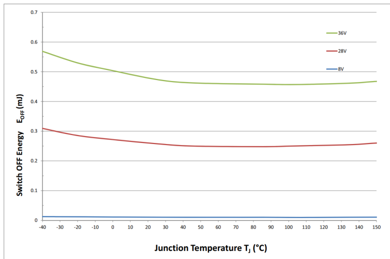
图42 关断能量 E_{OFF} = f(T_J; V_S) , R_L = 12 \Omega
