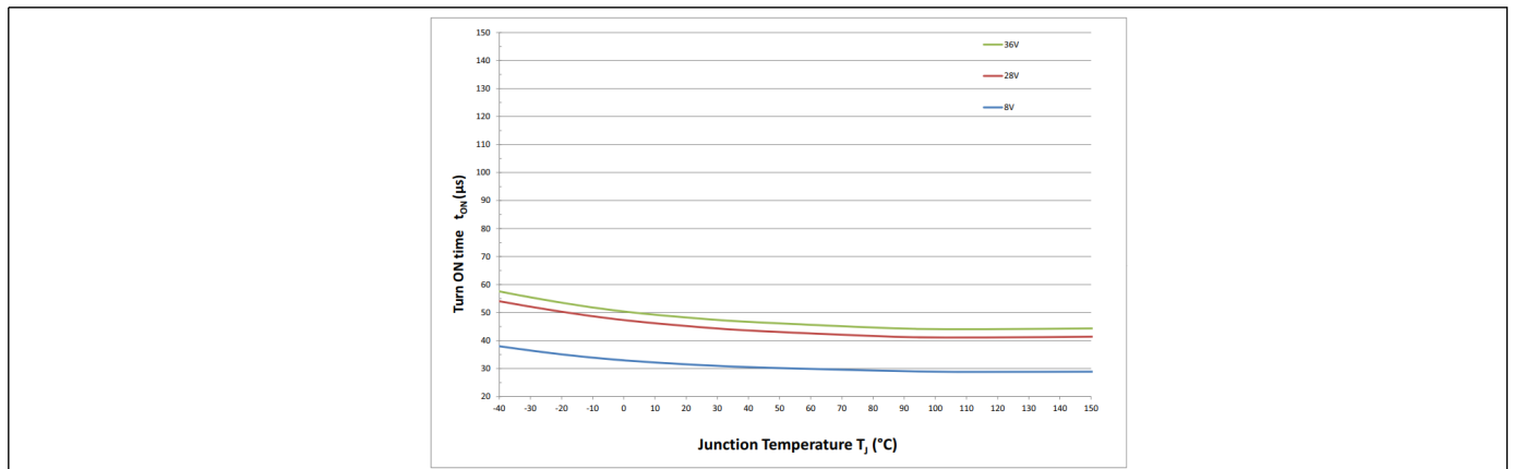
图 38 开启 t_{ON} = f(T_j; V_s), R_L = 12\Omega
