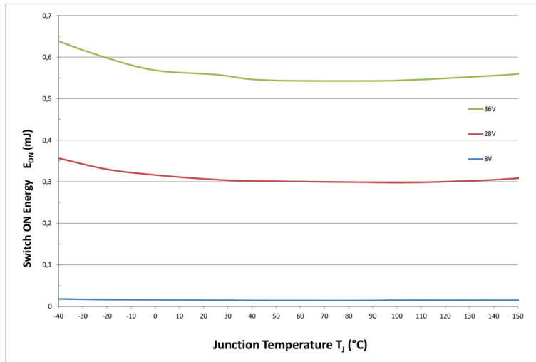
图41 开启能量 E_{ON} = f(T_J; V_S) , R_L = 12 \Omega
