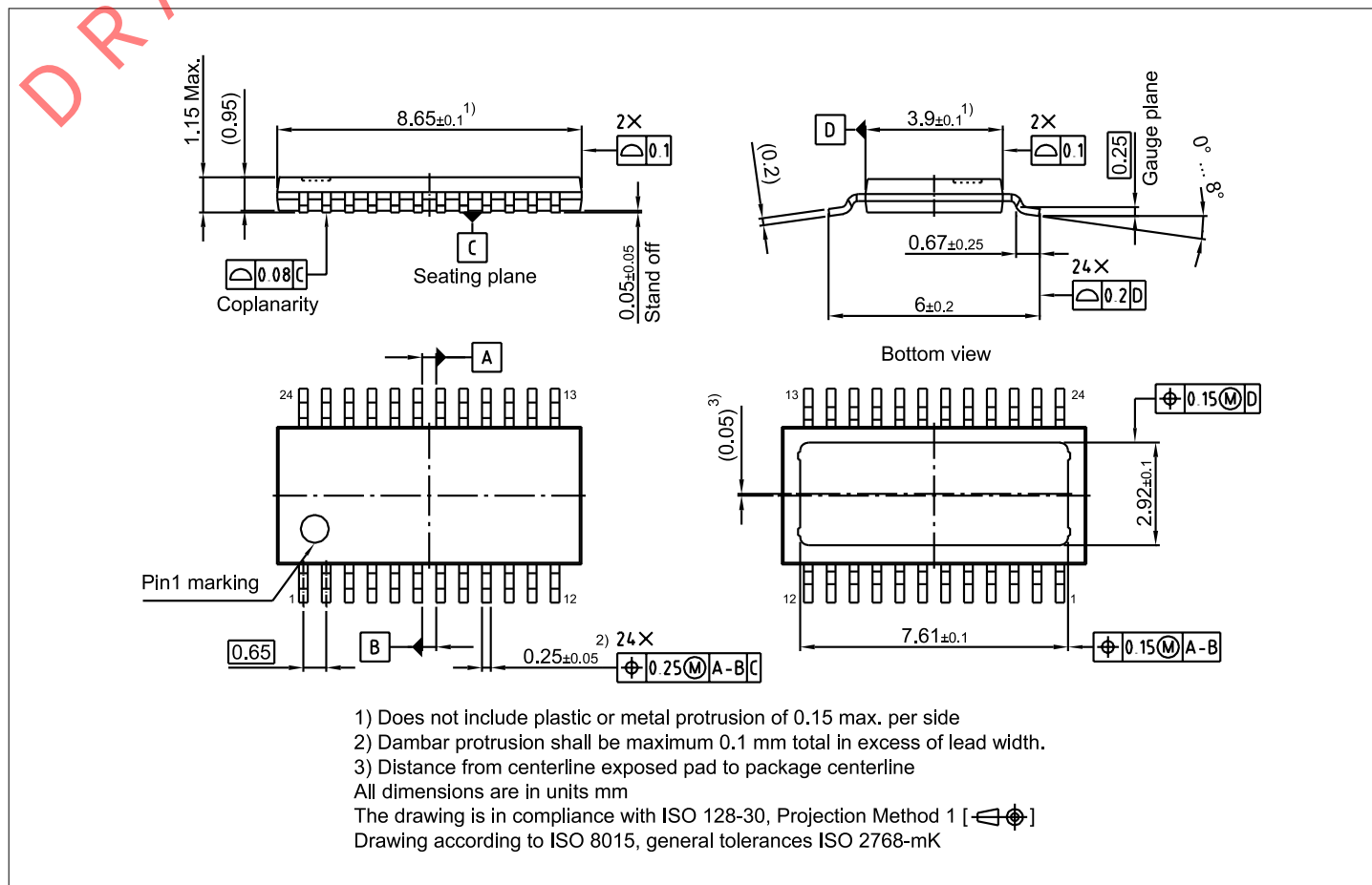
Figure 5 PG-TSDSO-24 package outlines
